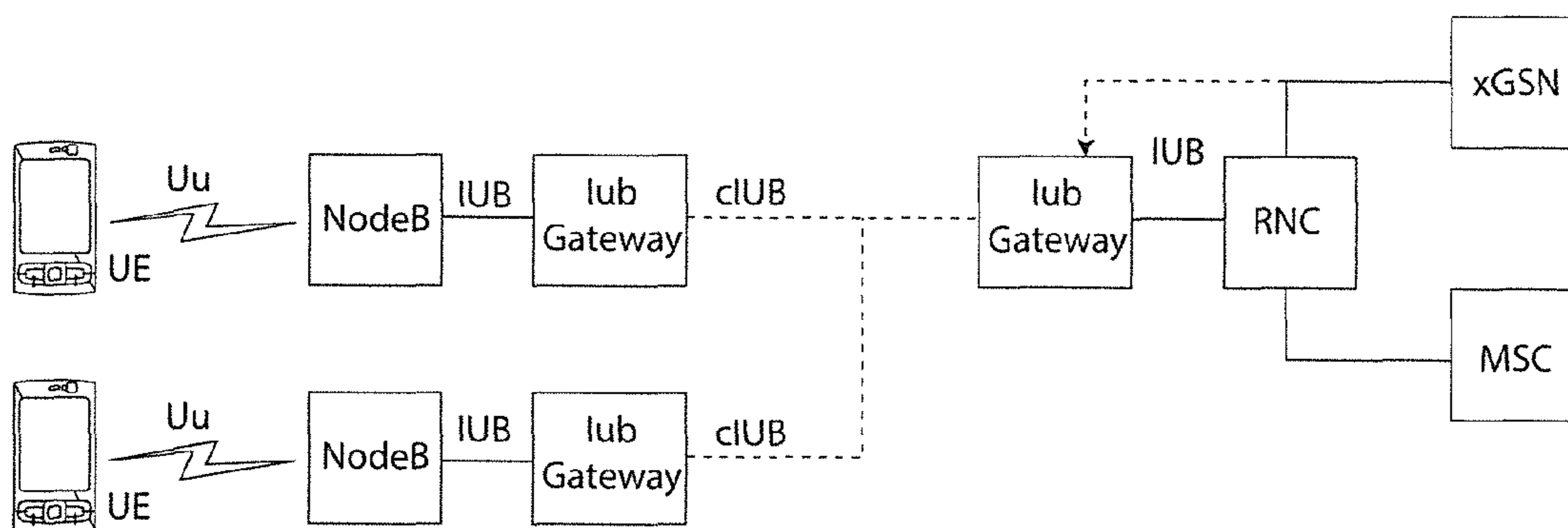
Iub Optimization via Iub Gateway
