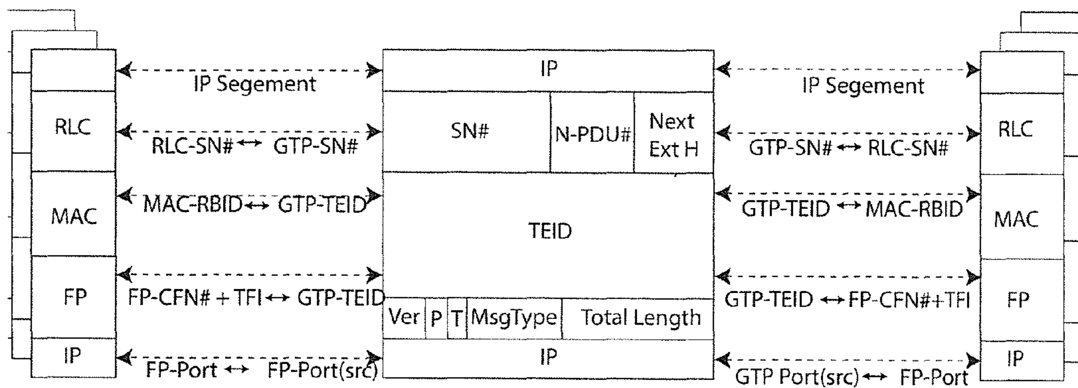
Iub Gateway GTP conversion Fig. 14
