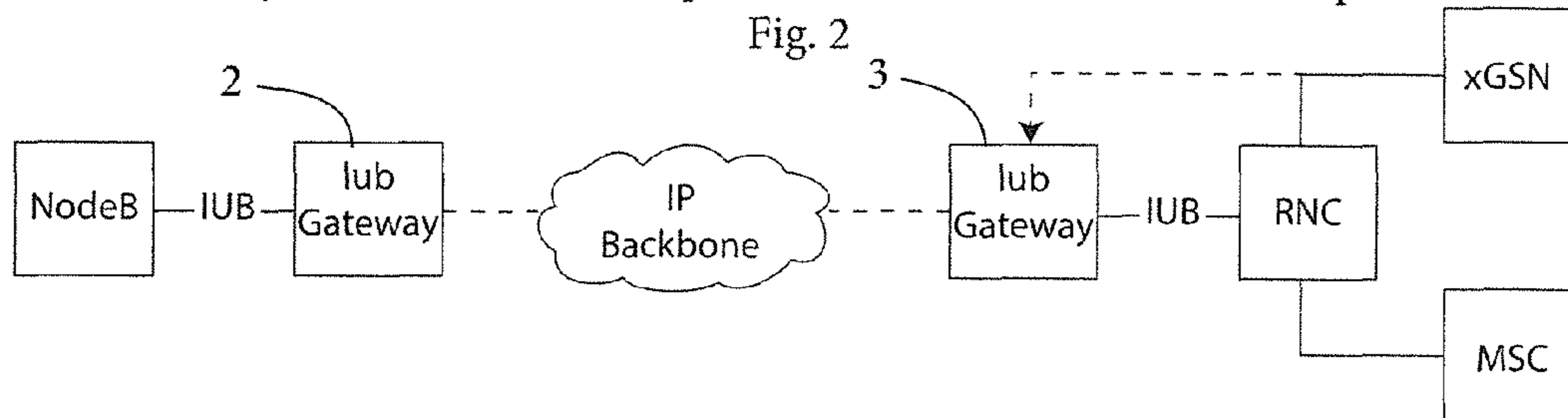
Symmetrical UrbanDate Iub Optimizer Gateway architecture
