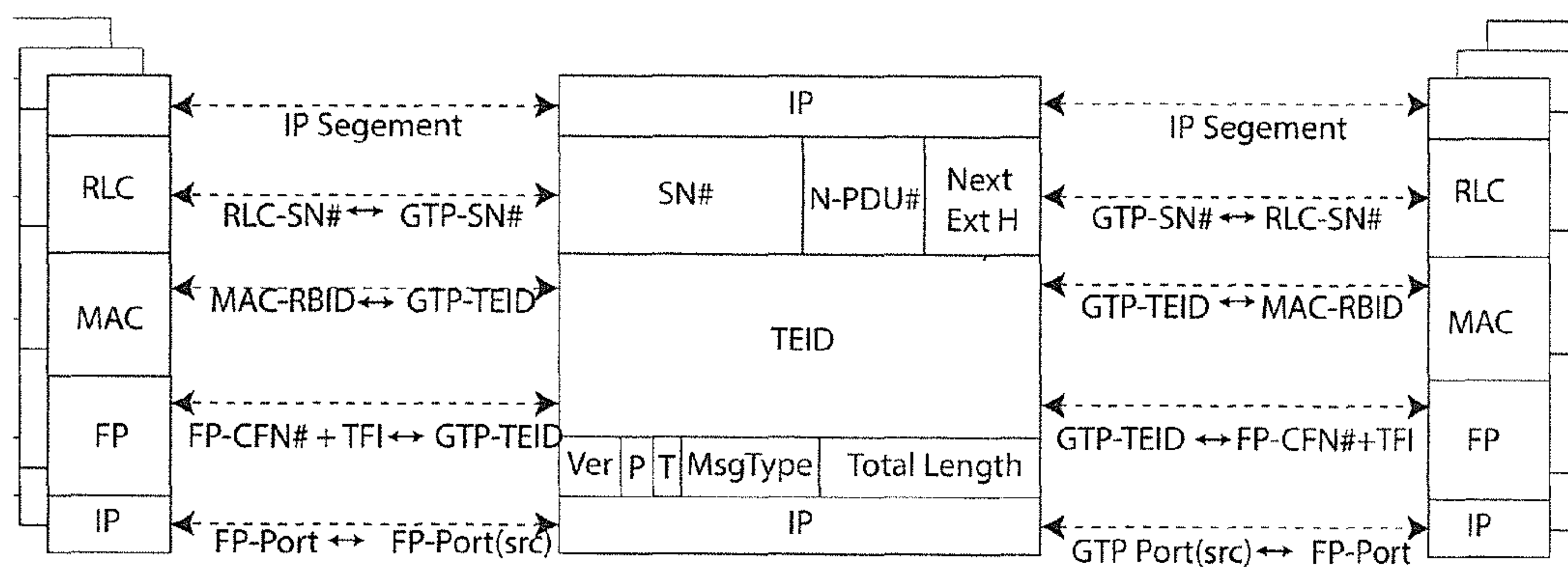
Iub Gateway GTP conversion
