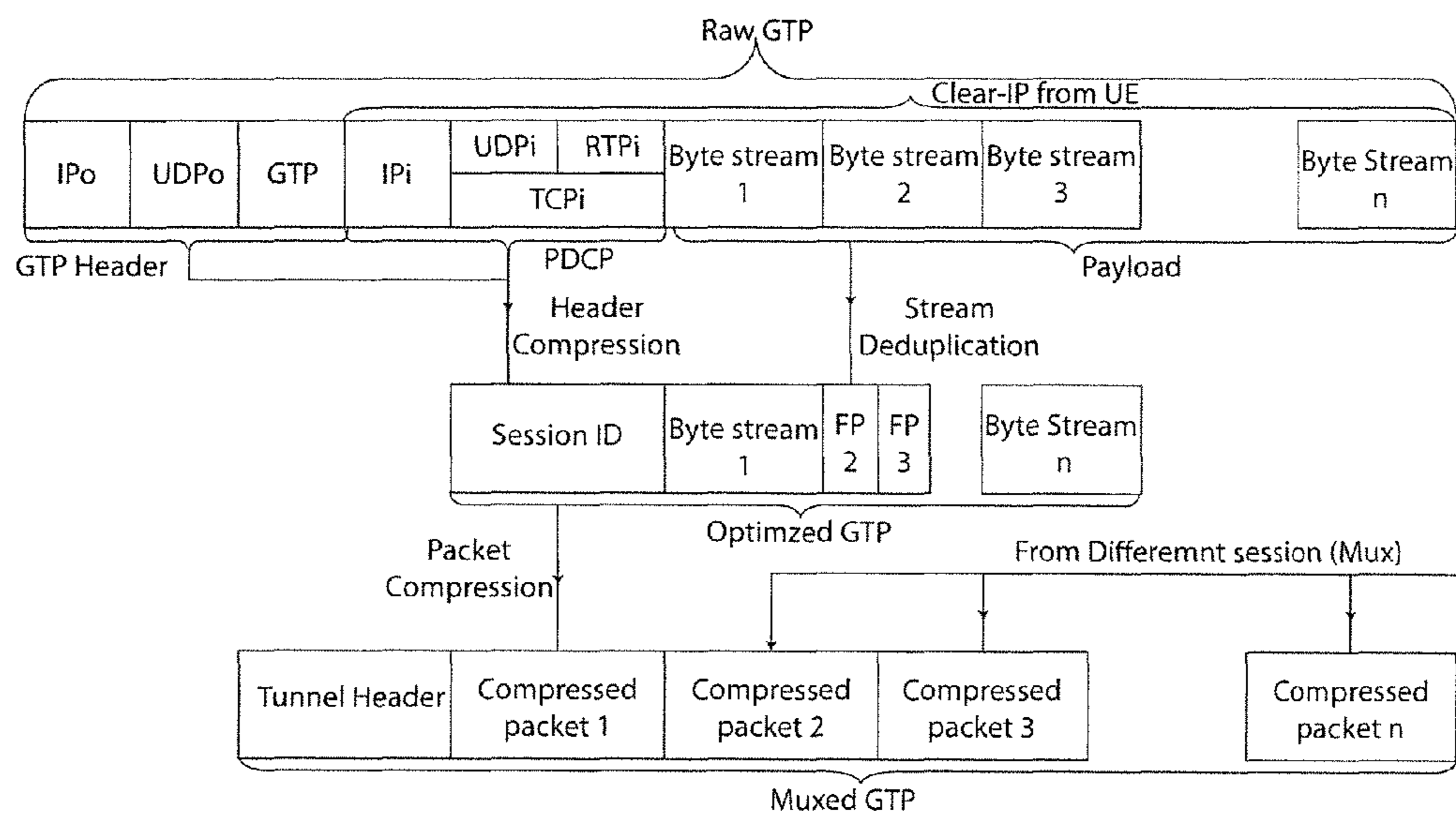
Iub Gateway Bandwidth Optimization
