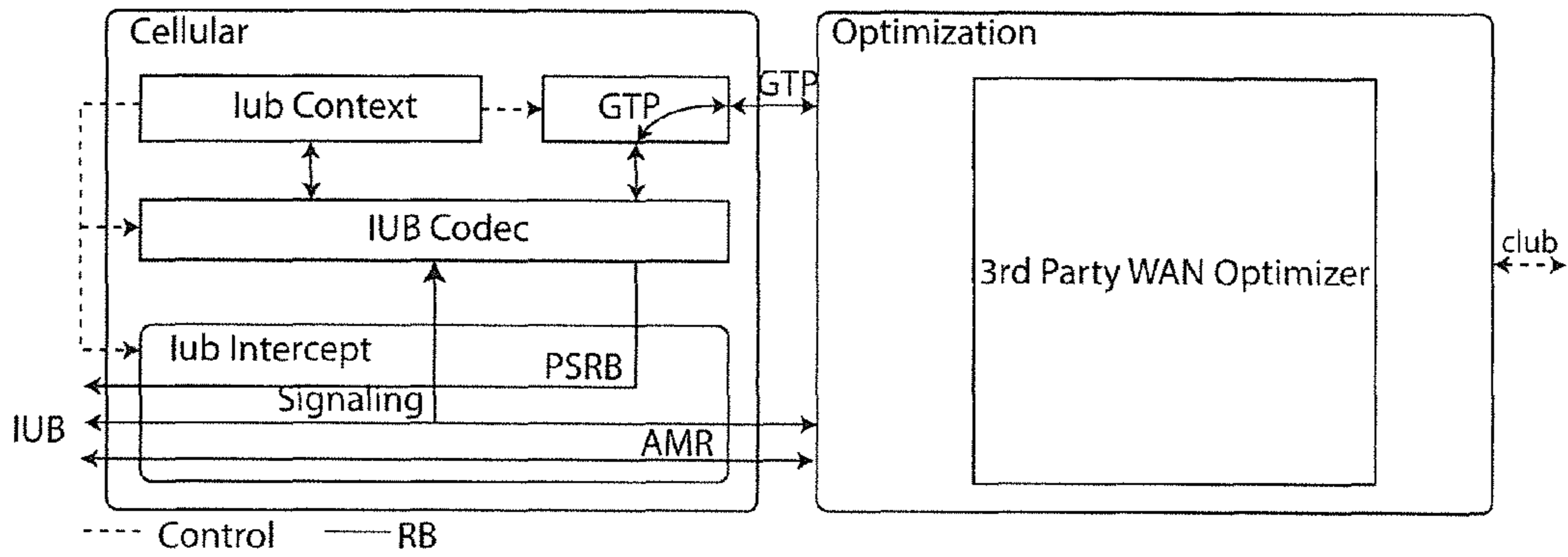
Iub Gateway with 3rd Party WAN Optimizer
