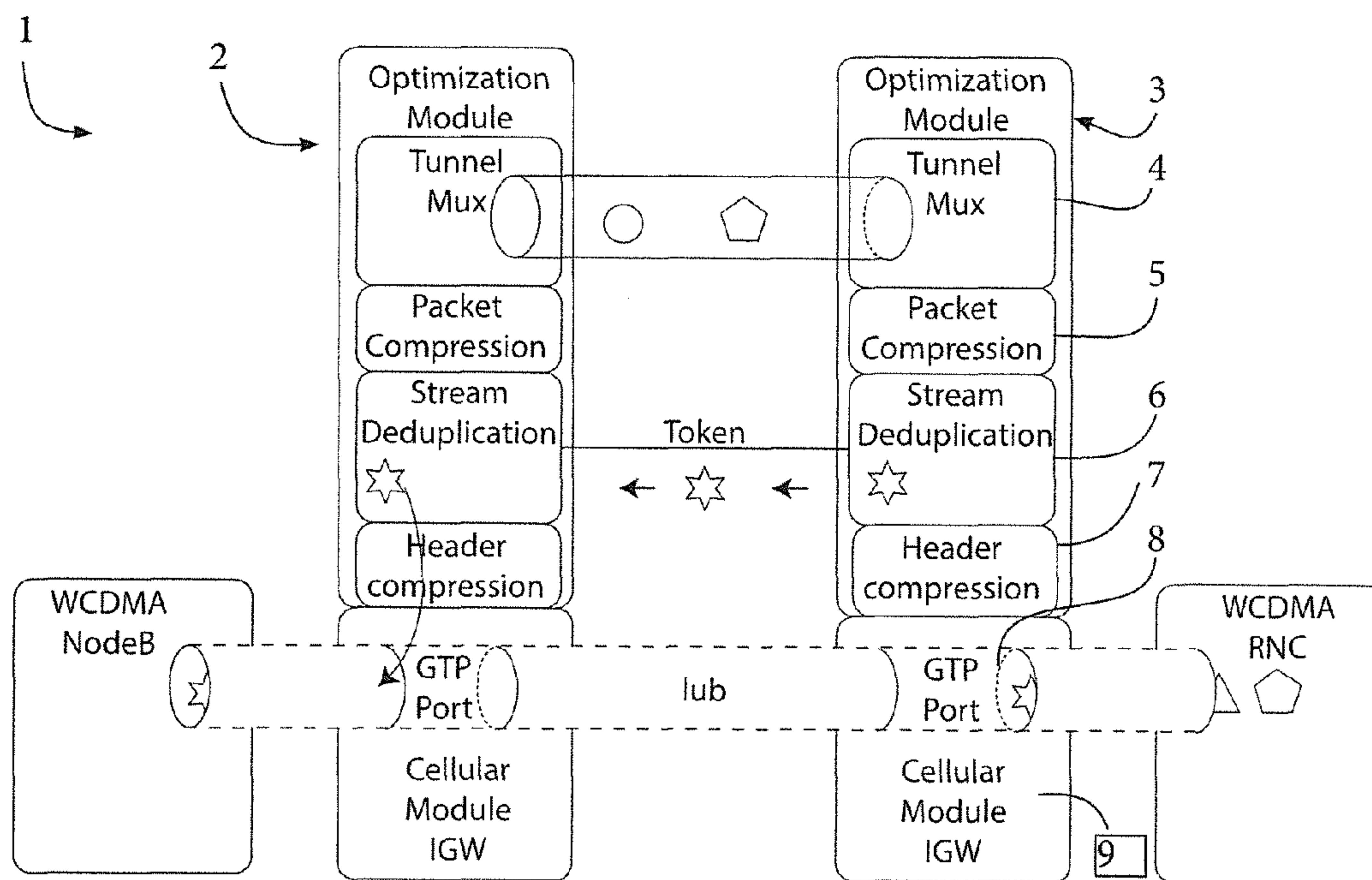
Fig. 1 Stream De-duplication (PRIOR ART)
