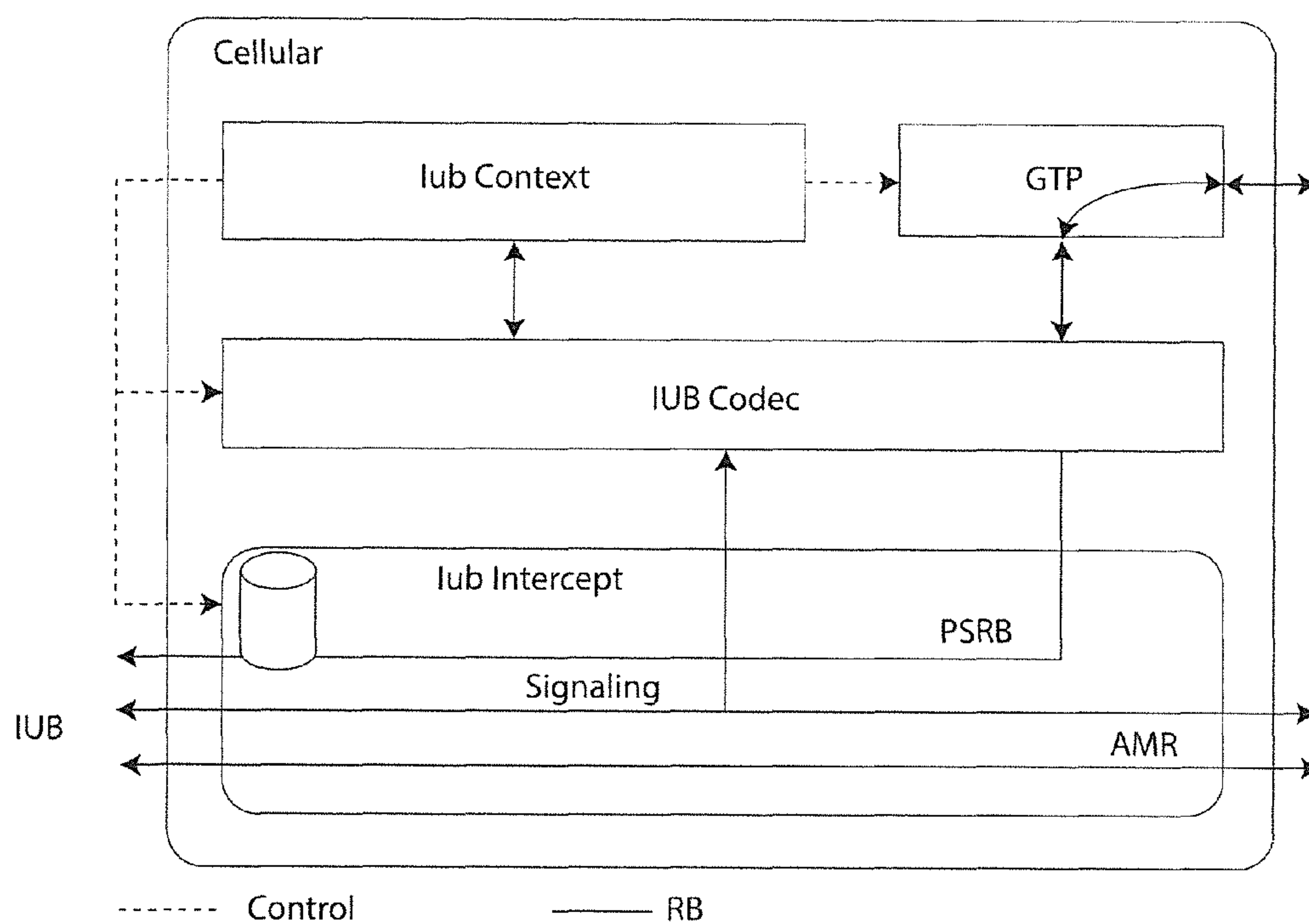
Iub Gateway Interceptor
