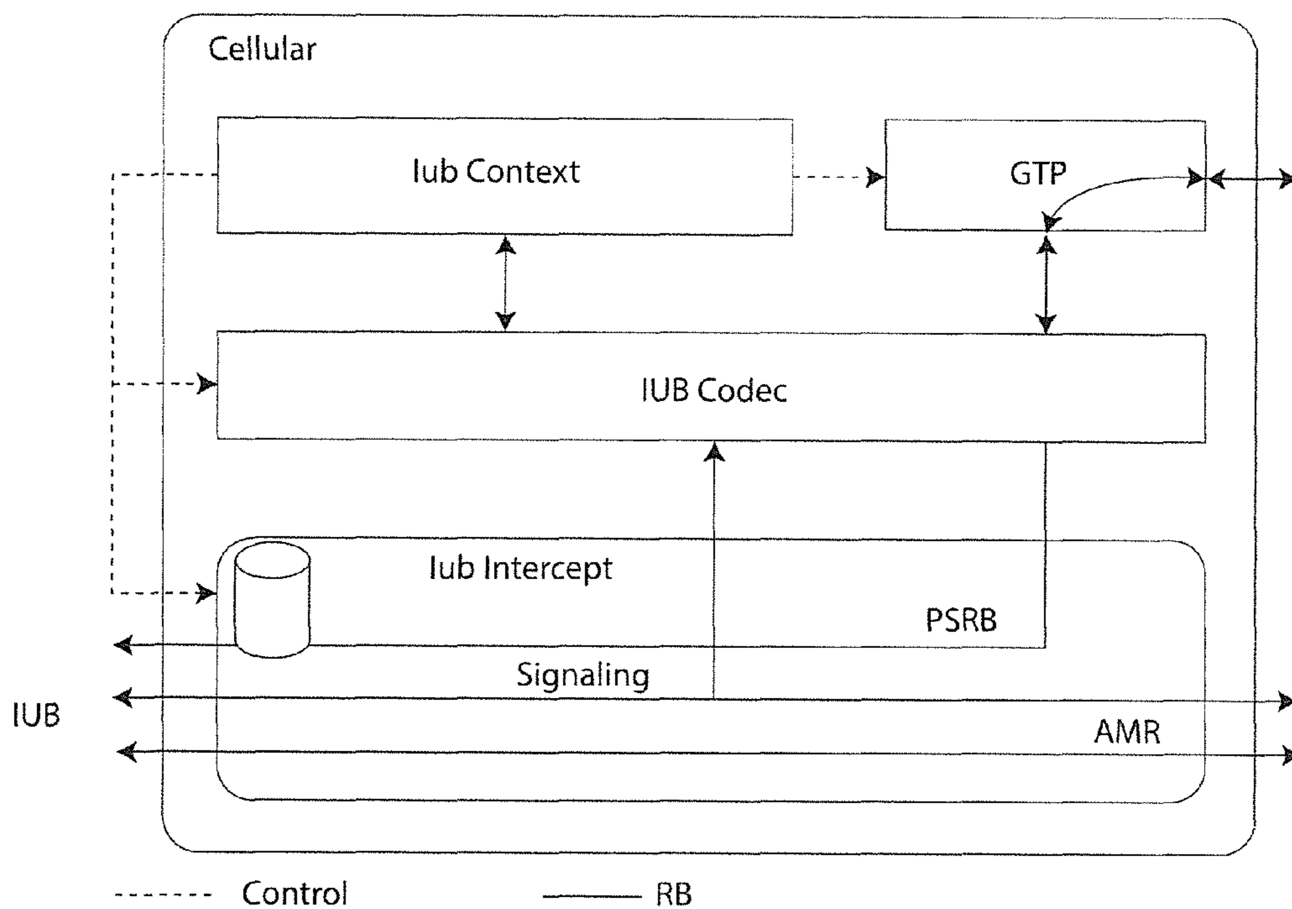
Iub Gateway Interceptor Fig. 15
