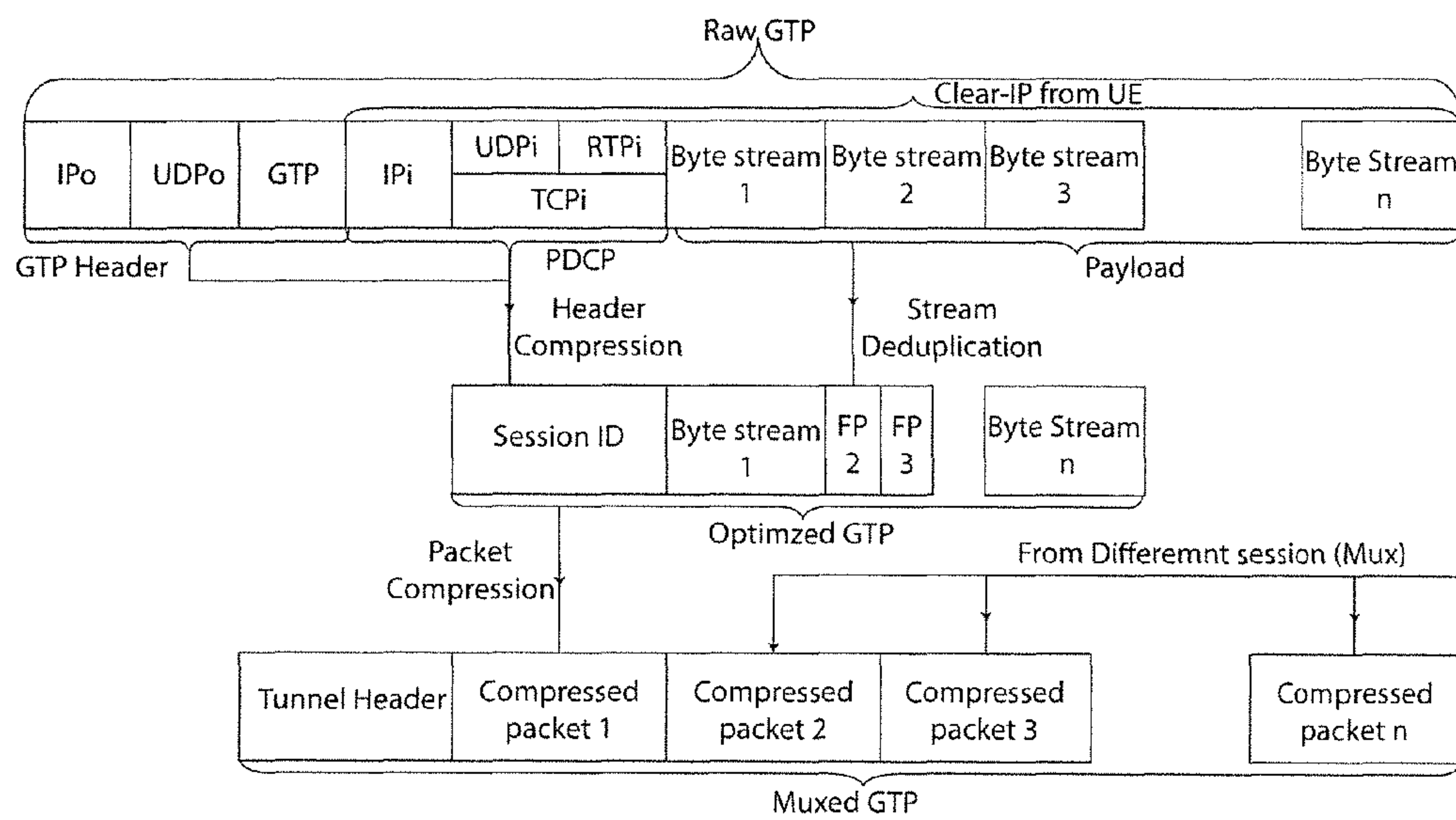
Iub Gateway Bandwidth Optimization Fig. 16
