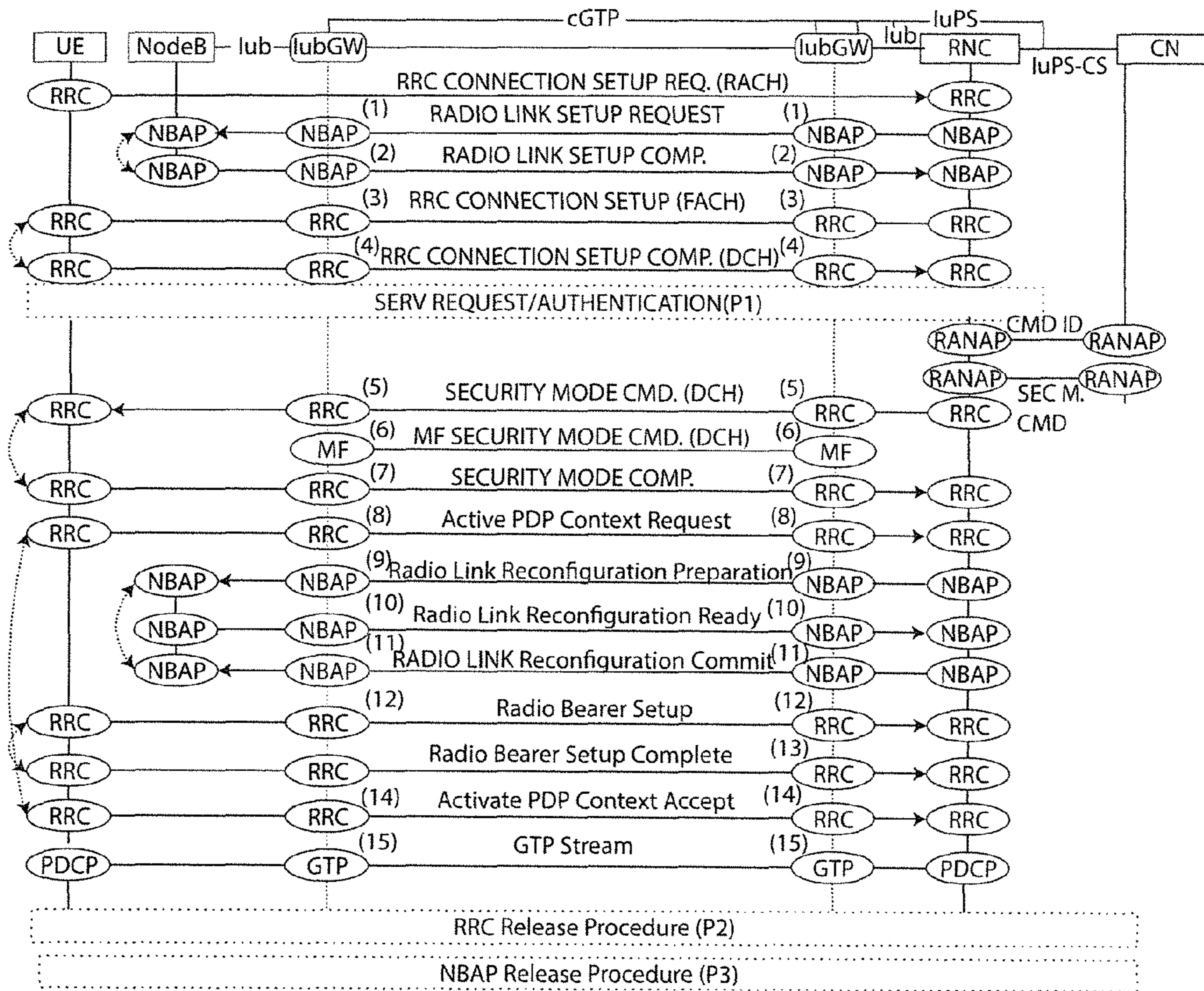
IGW intercepts RRC/NBAP signaling and builds context
