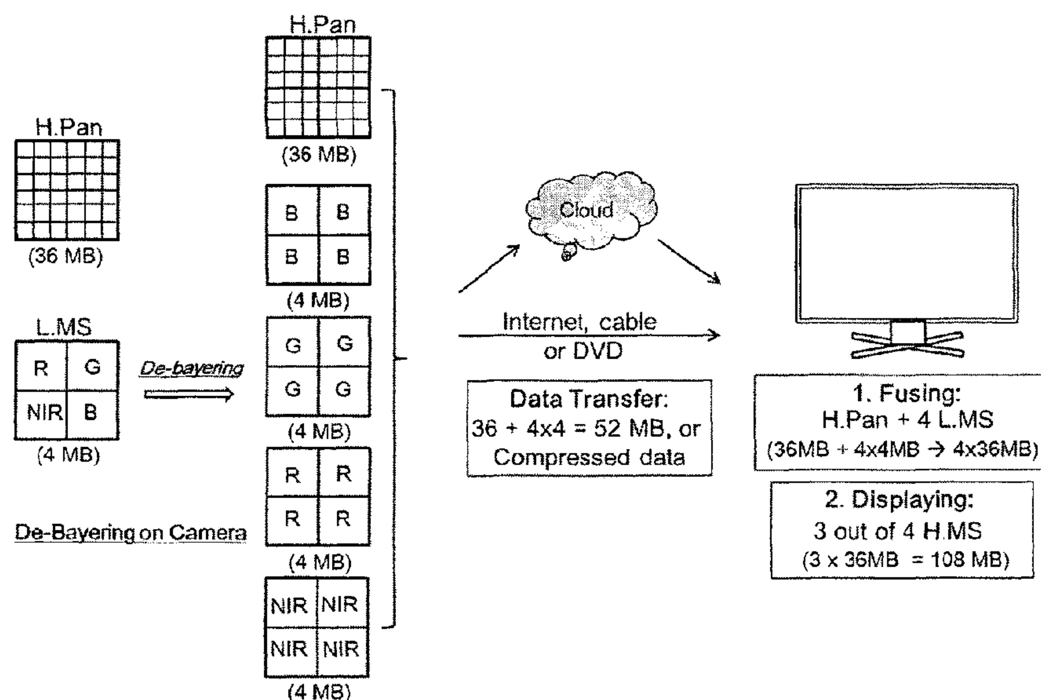
2-Chip Color Camera with H.Pan and L.MS
