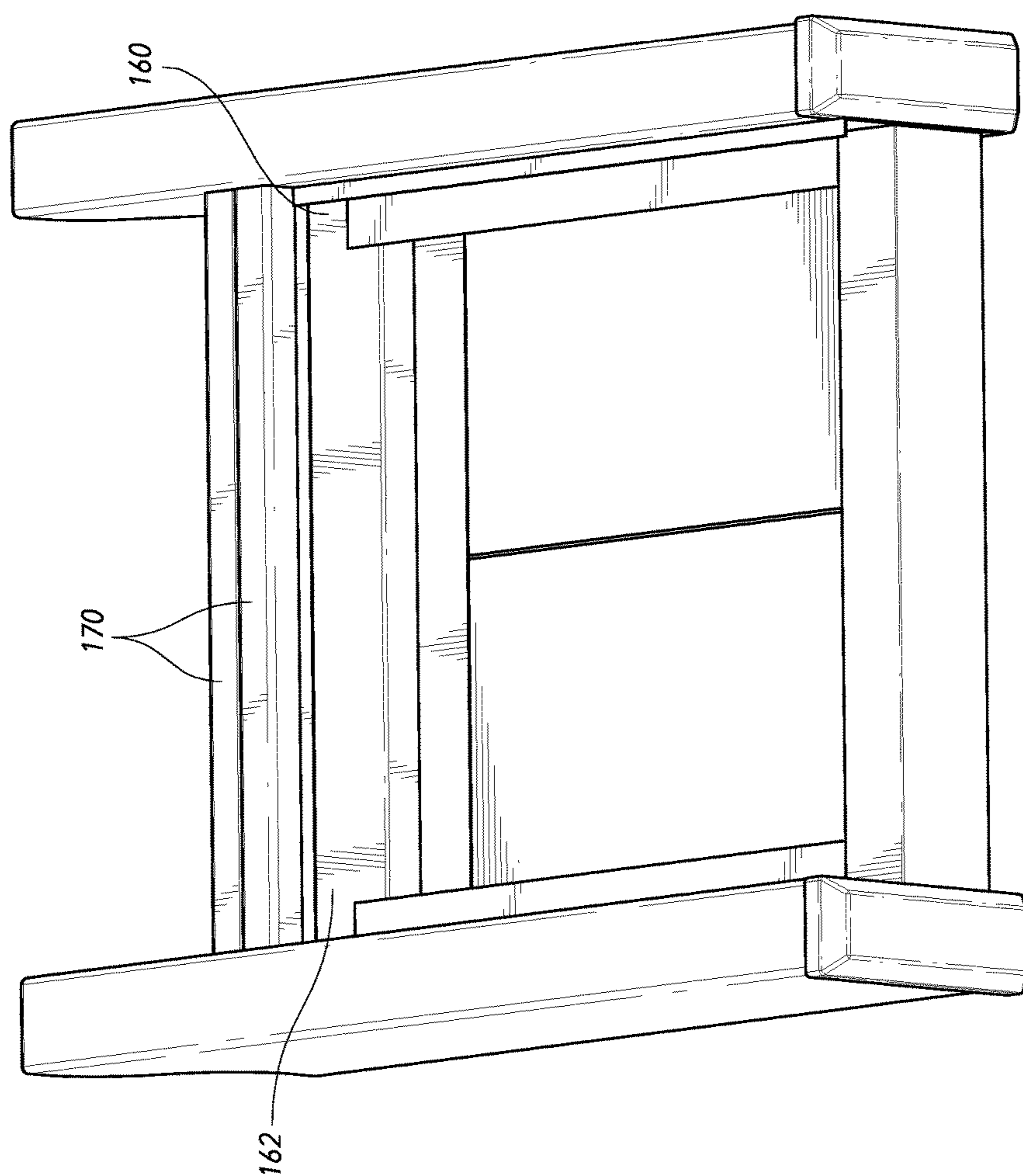
FIG. 17 (PRIOR ART)
