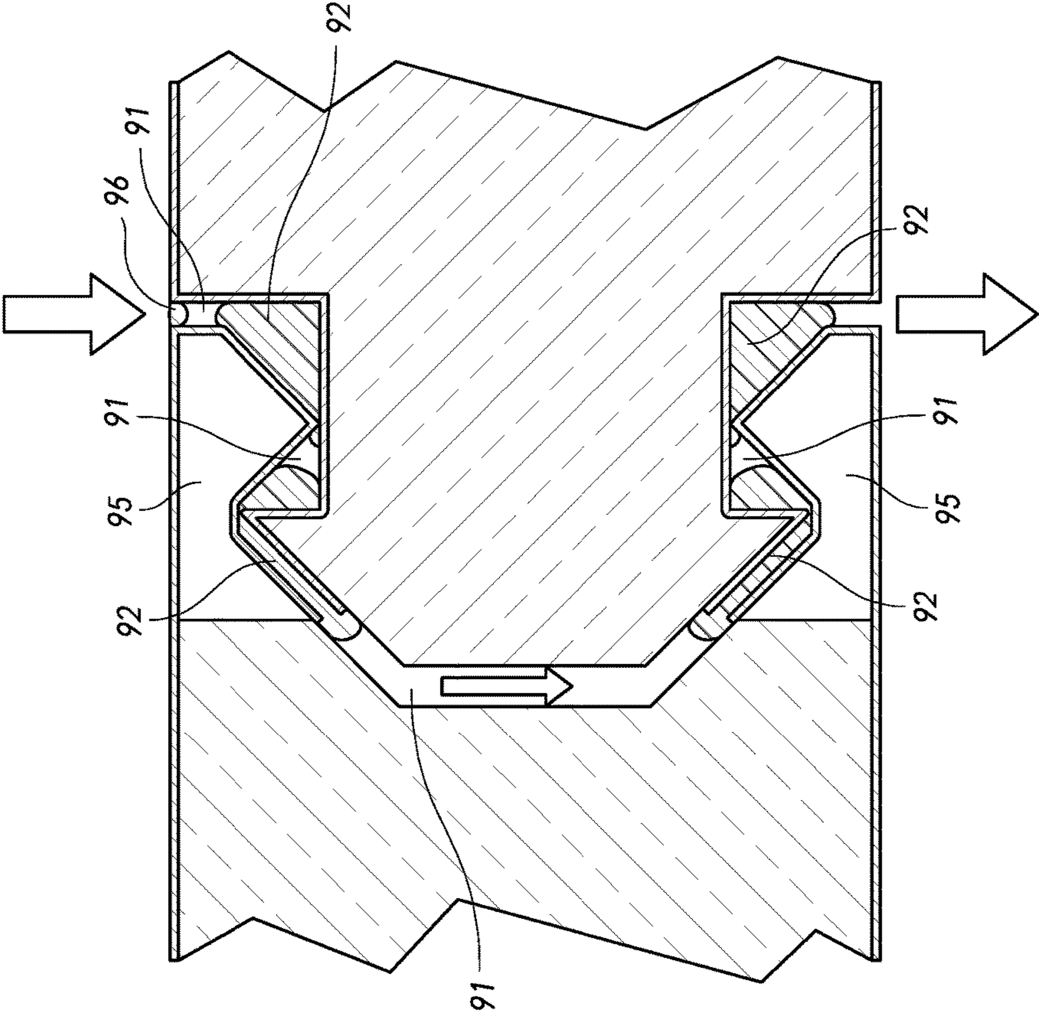
FIG. 9 (PRIOR ART)
