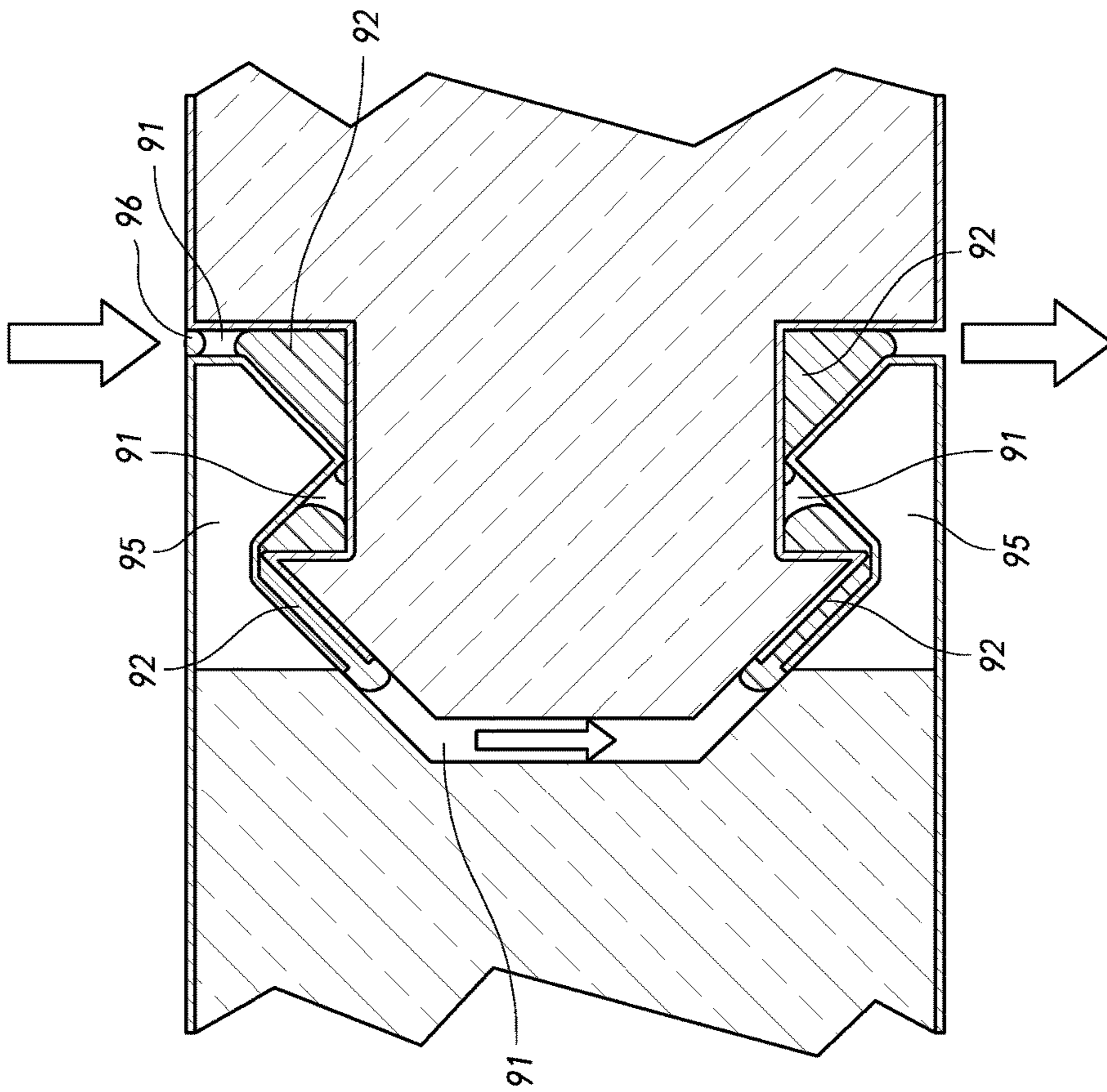
FIG. 9 (PRIOR ART)
