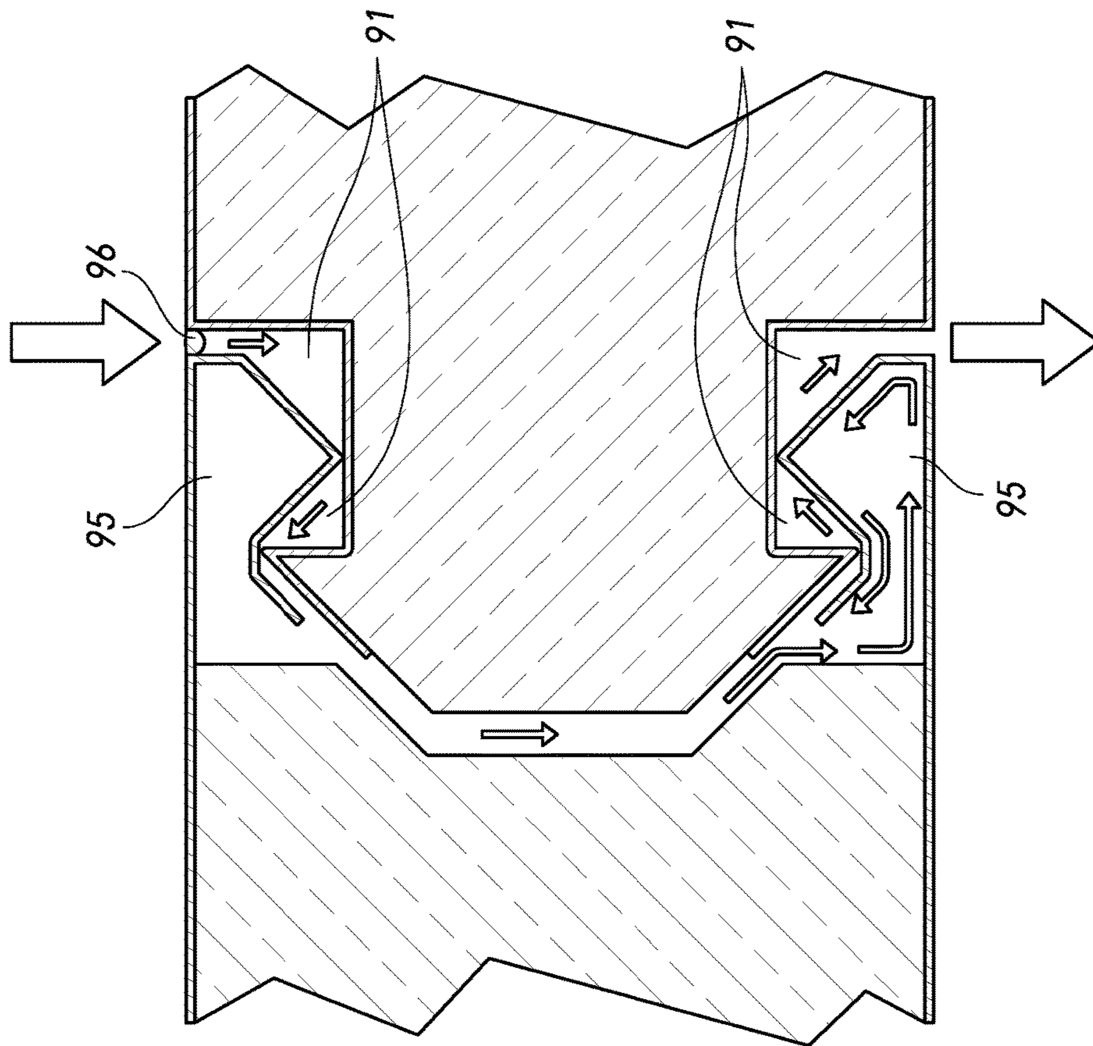
FIG. 10 (PRIOR ART)
