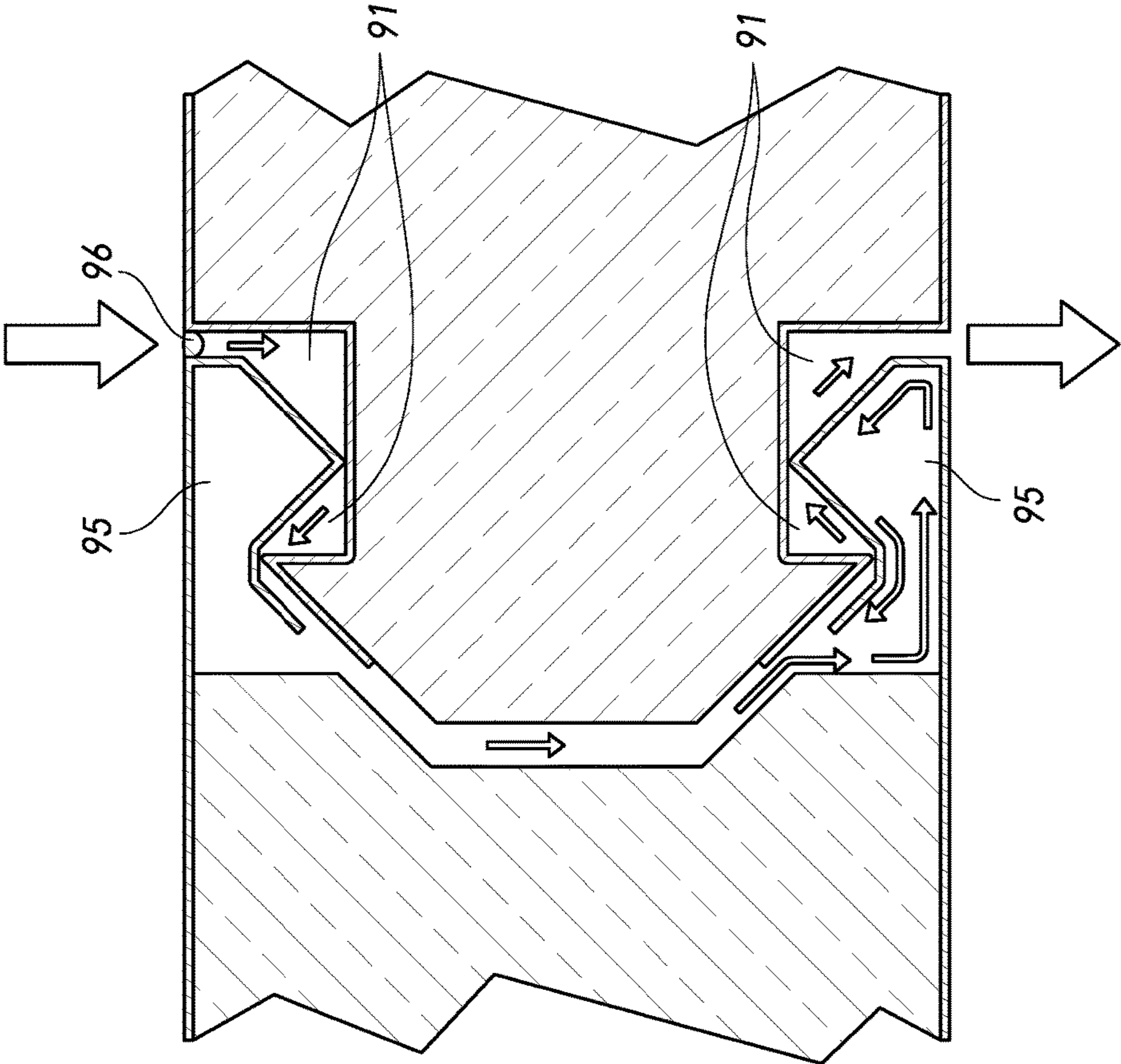
FIG. 10 (PRIOR ART)
