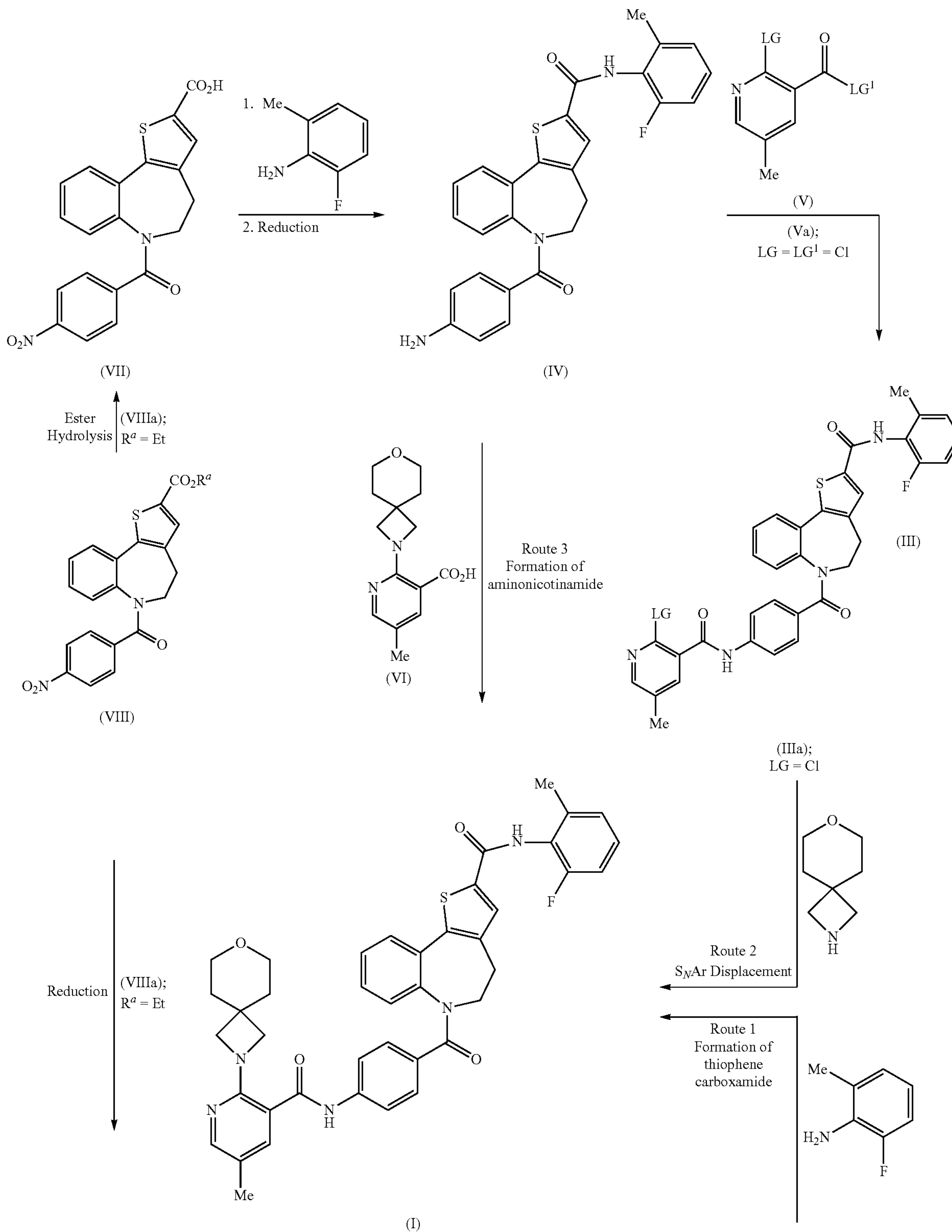
Scheme 1: Synthetic routes used for the preparation of Compound (I).
