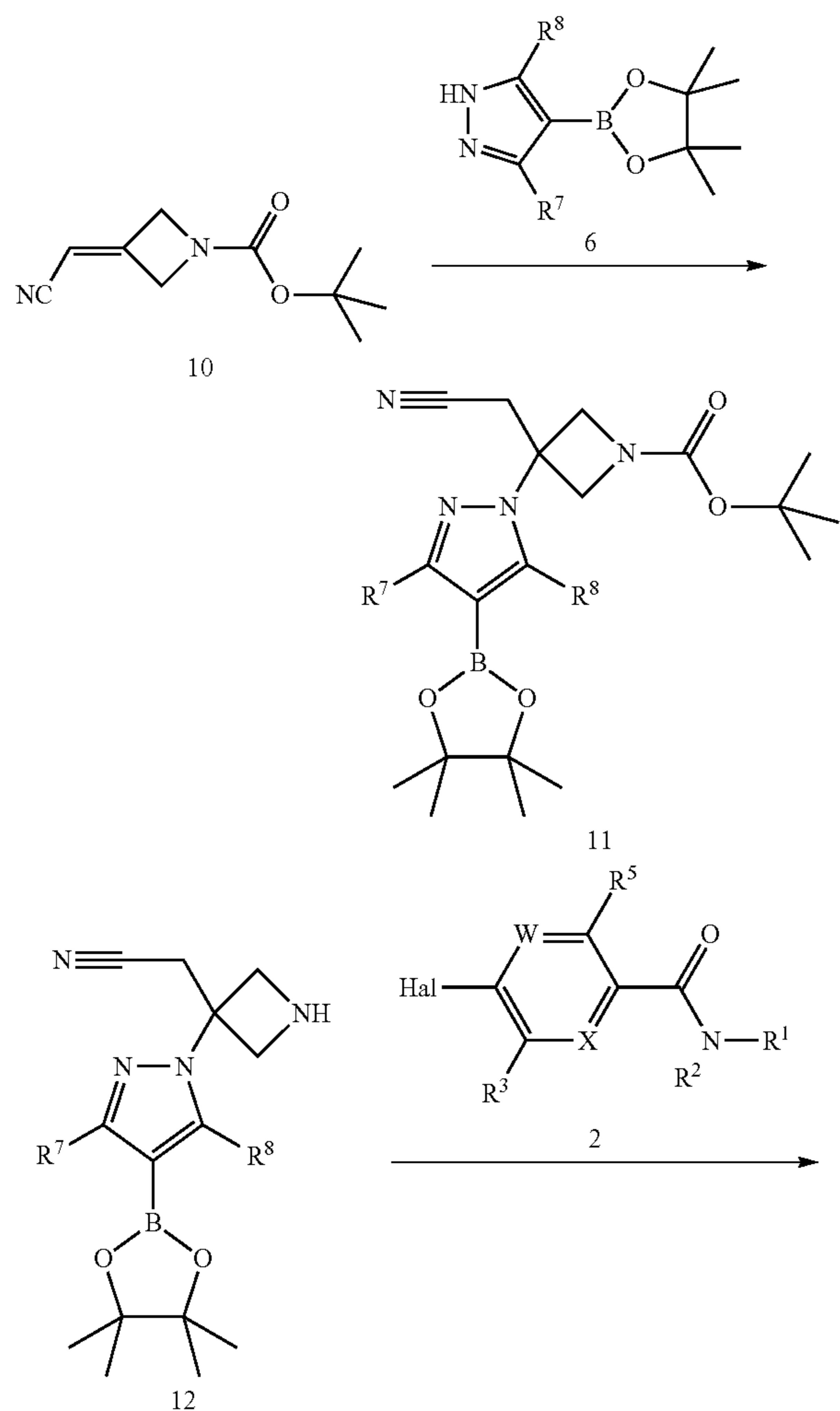
Scheme 2
