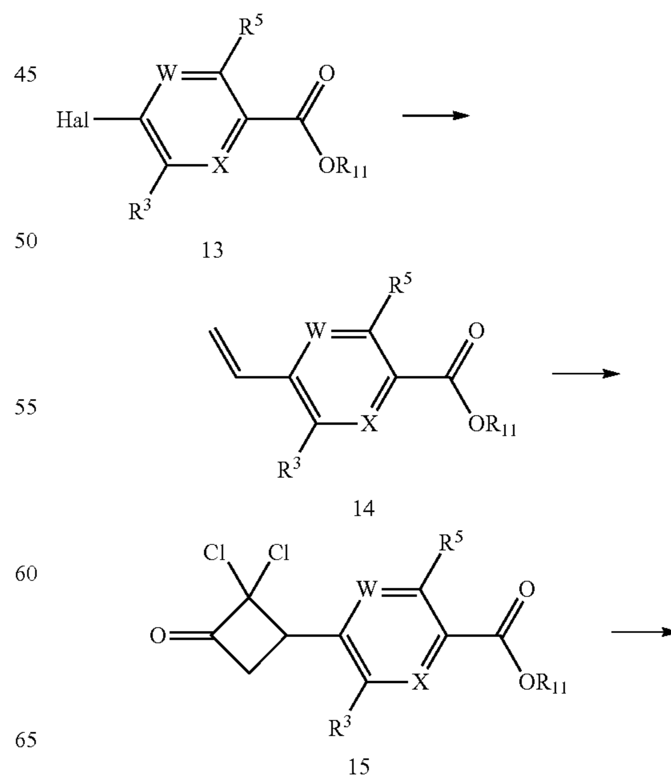
Scheme 3
