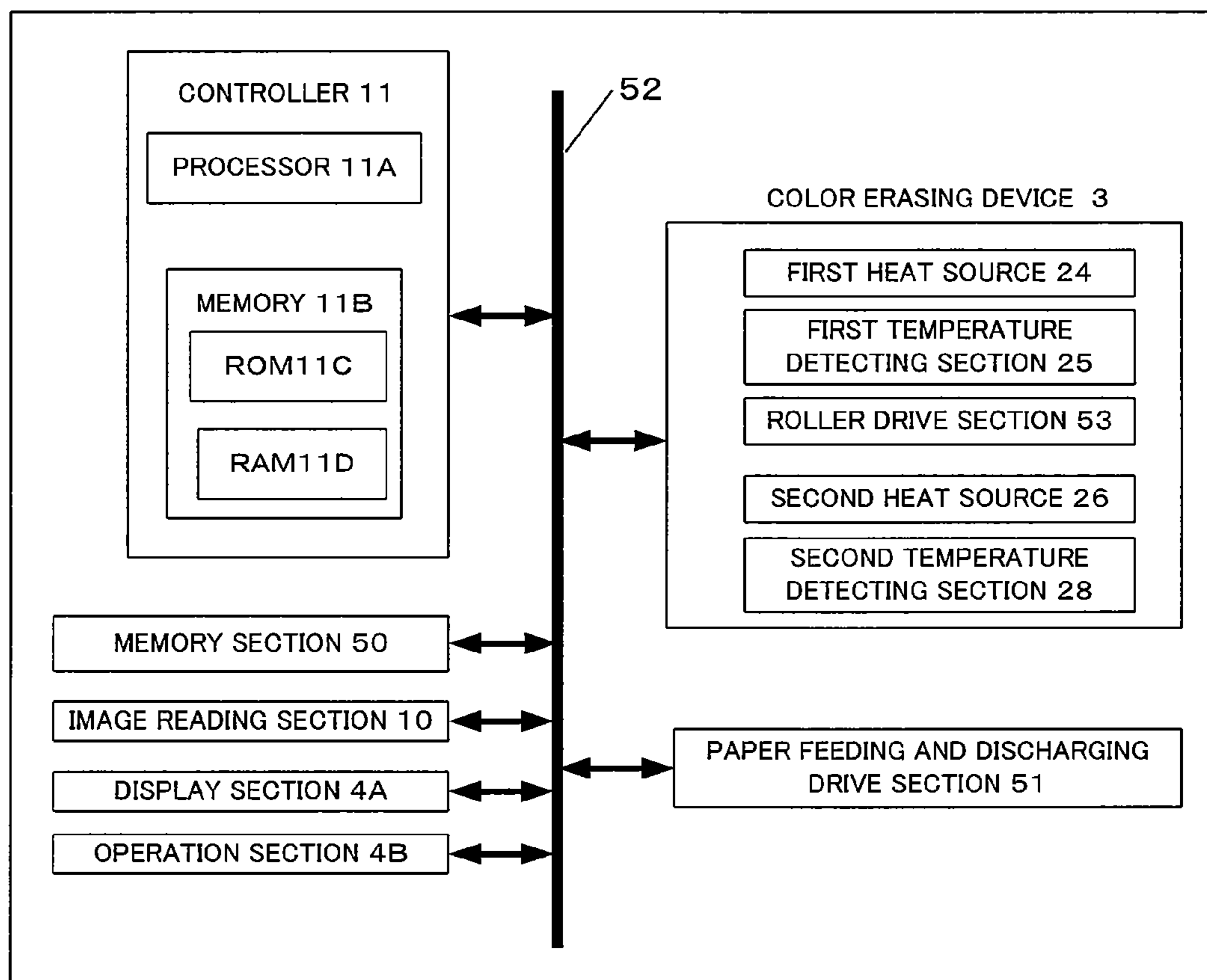
ERASING APPARATUS 1
