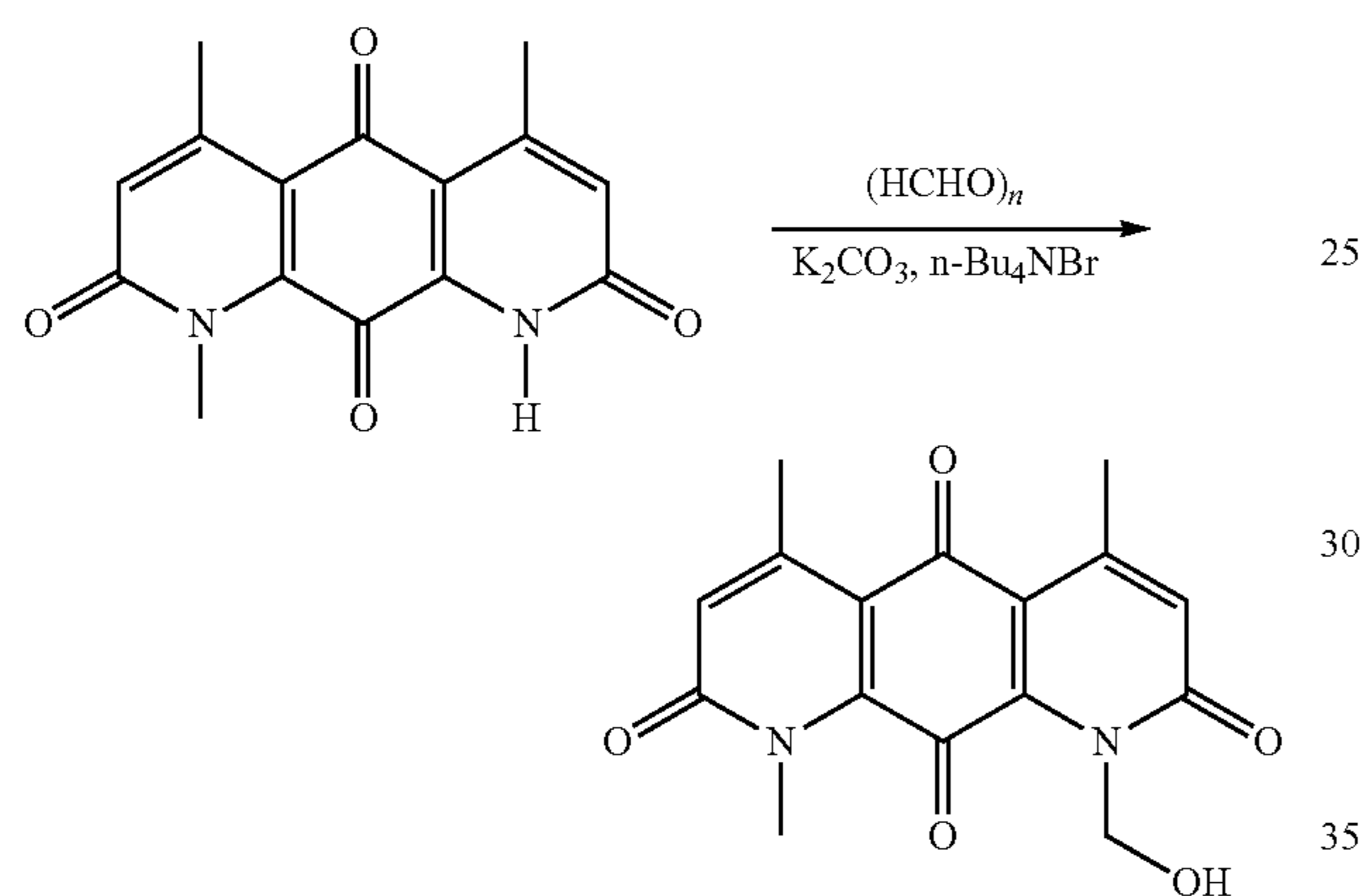
Scheme 7.1. Preparation of DNQ-P1.
