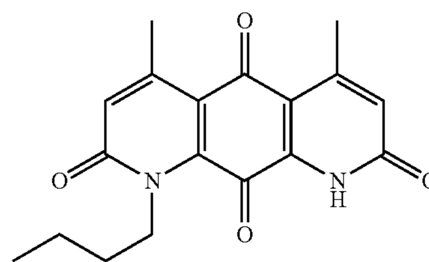
Scheme 4.3. New DNQ derivatives.
