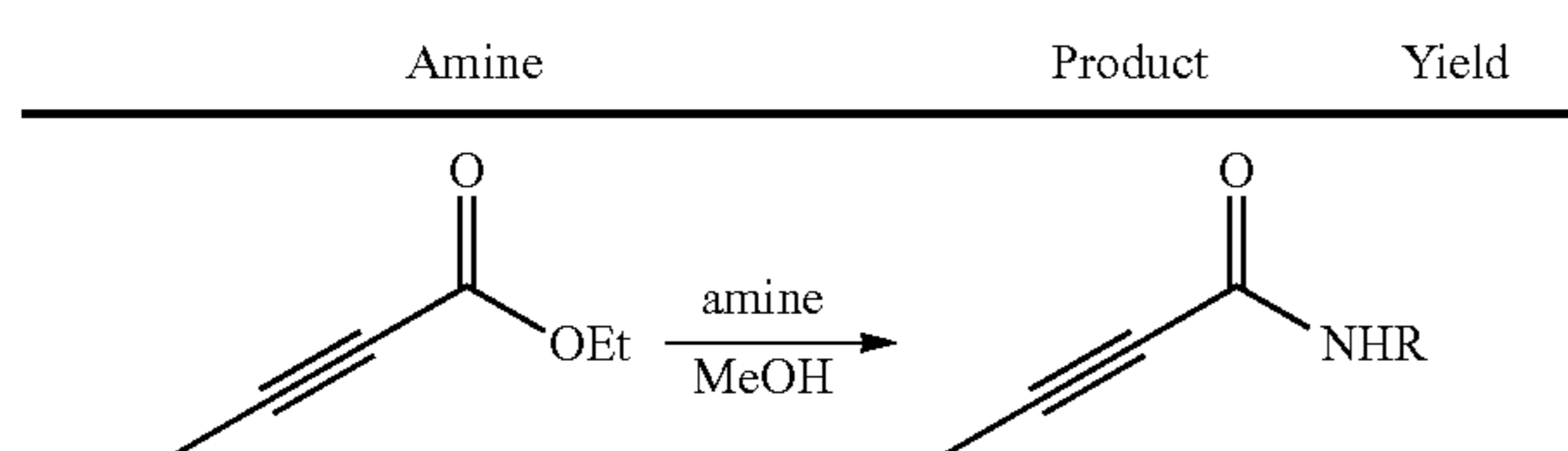
Scheme 4.4. Synthesis of amides bearing bulky substituents on nitrogen.
