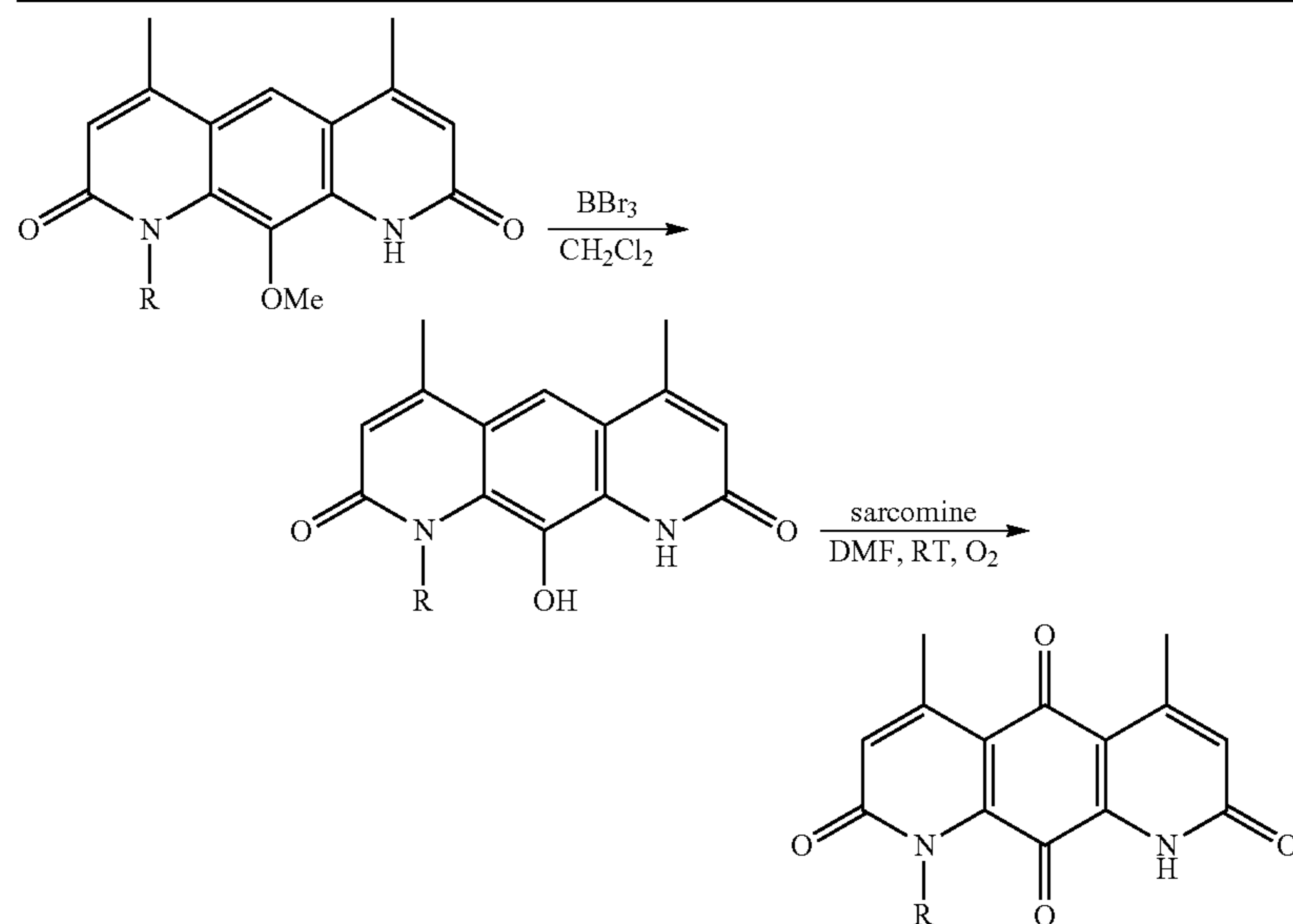
Scheme 4.5. Synthesis of DNQ derivatives bearing substituents sensitive to HBr-mediated deprotection.
