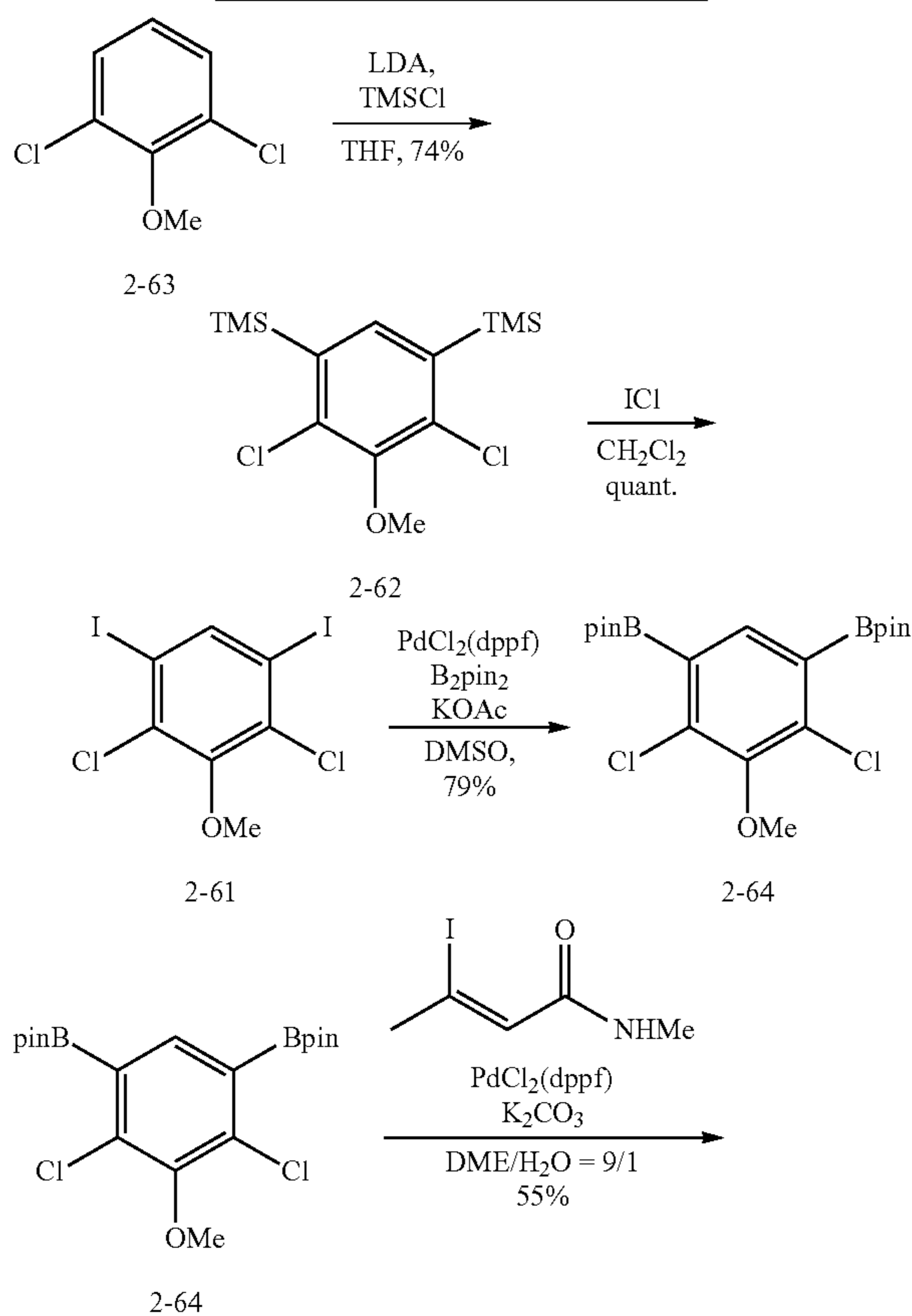
Scheme 1.12. Synthesis of SCH 538415.
