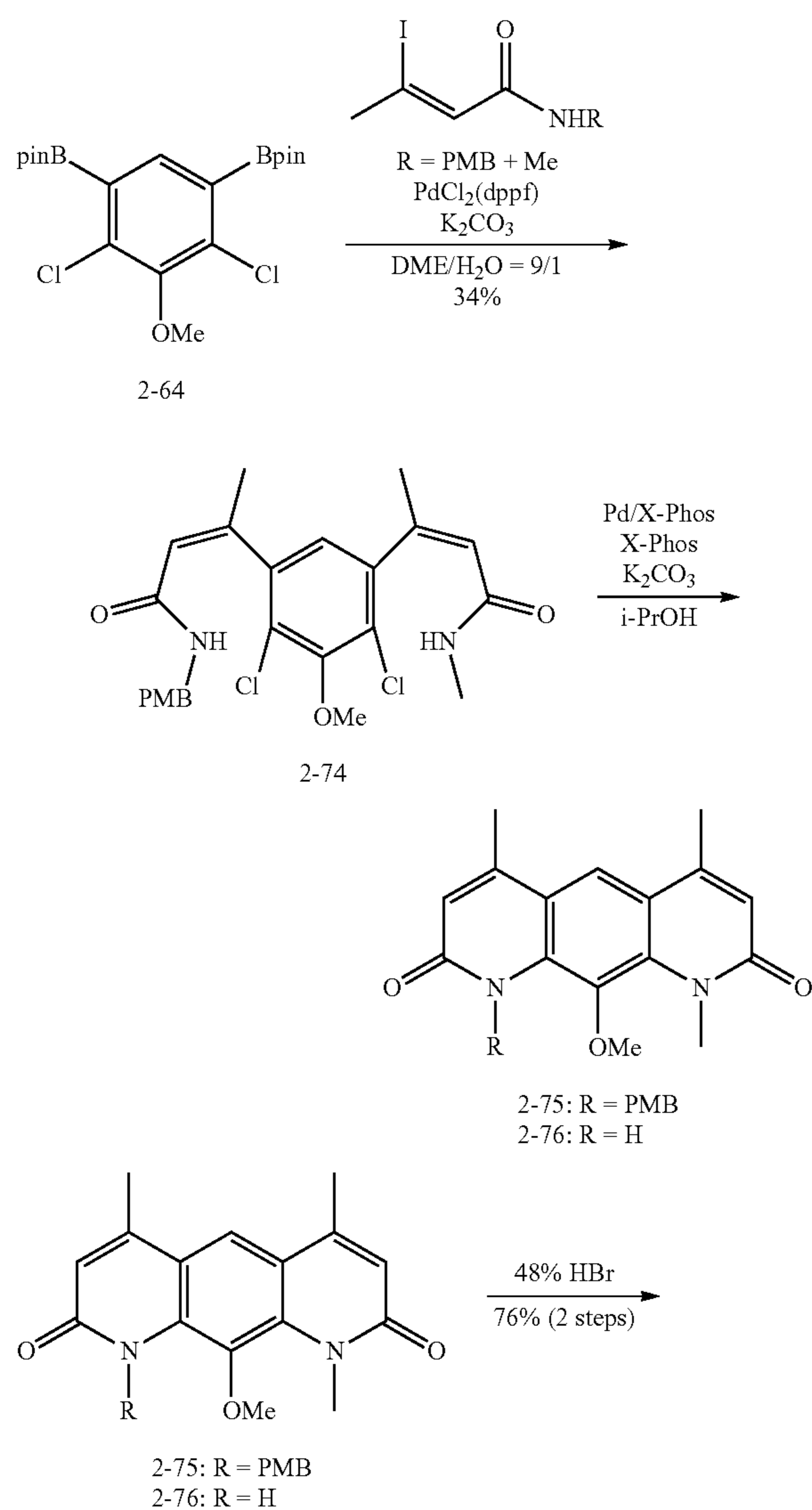
Scheme 1.14. Robust and scalable synthesis of DNQ.
