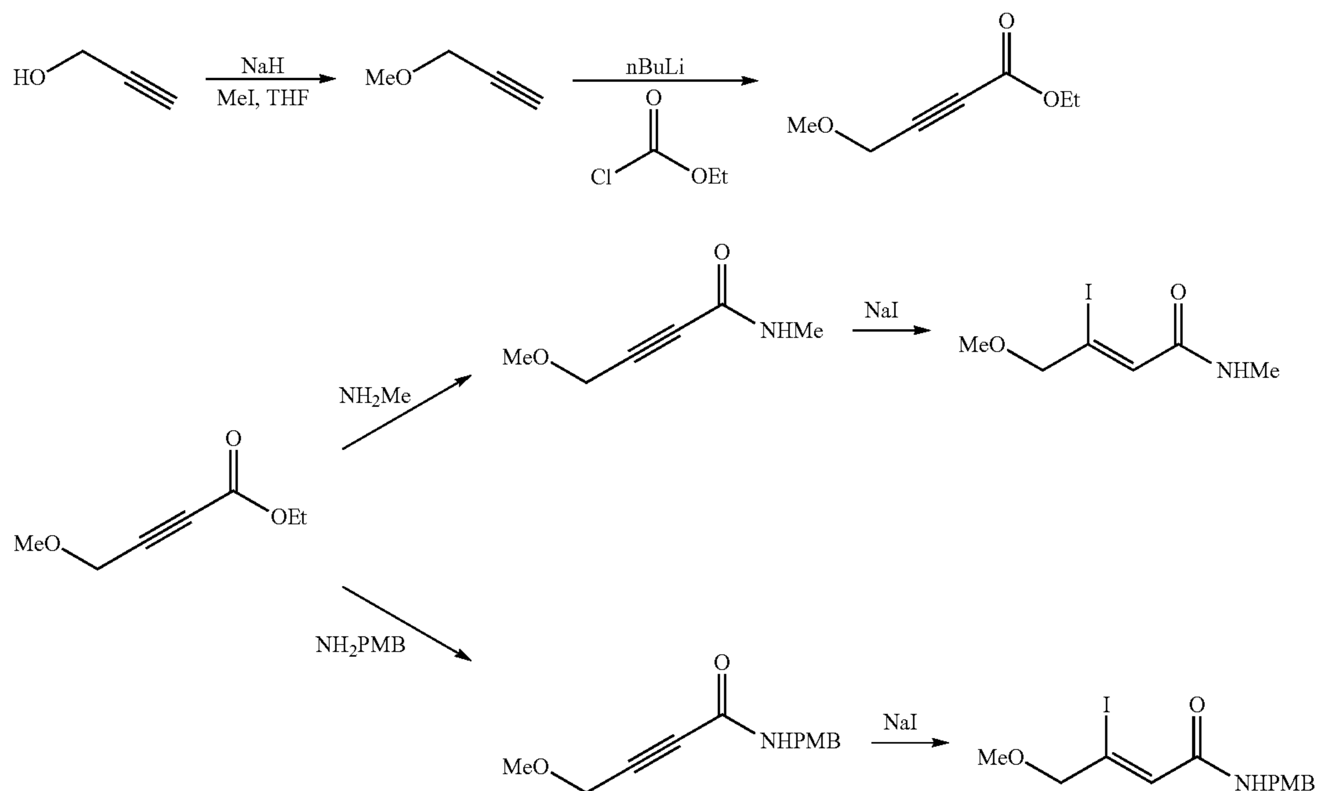
Scheme 7.2. Preparation of DNQ-P2 and DNQ-P3 Intermediates.
