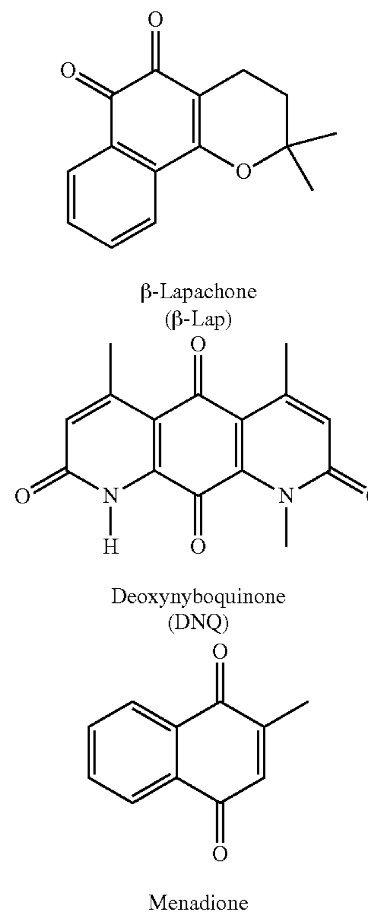
Scheme 1. Examples of Quinone Compounds.
