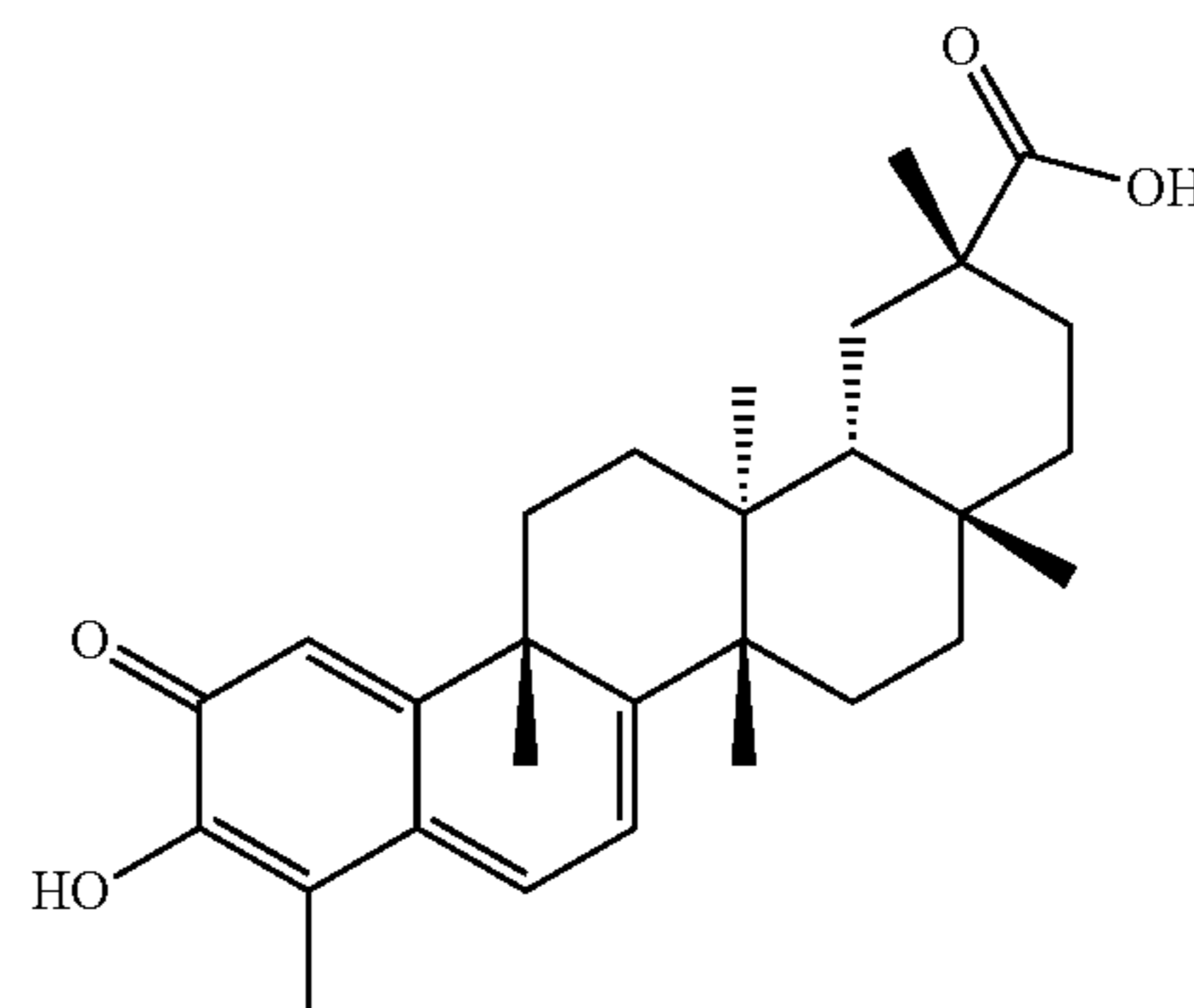
Celastrol
