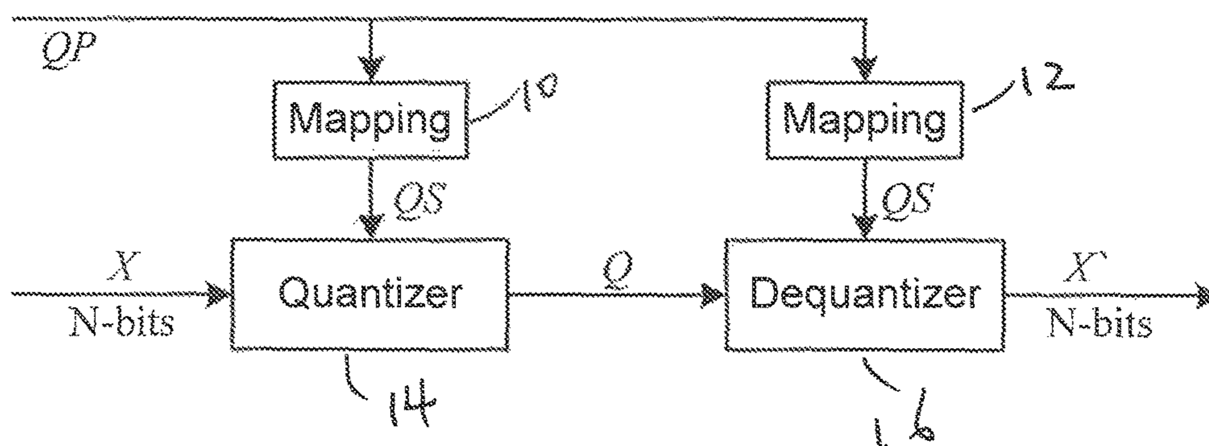
FIG. 4 Prior Art
