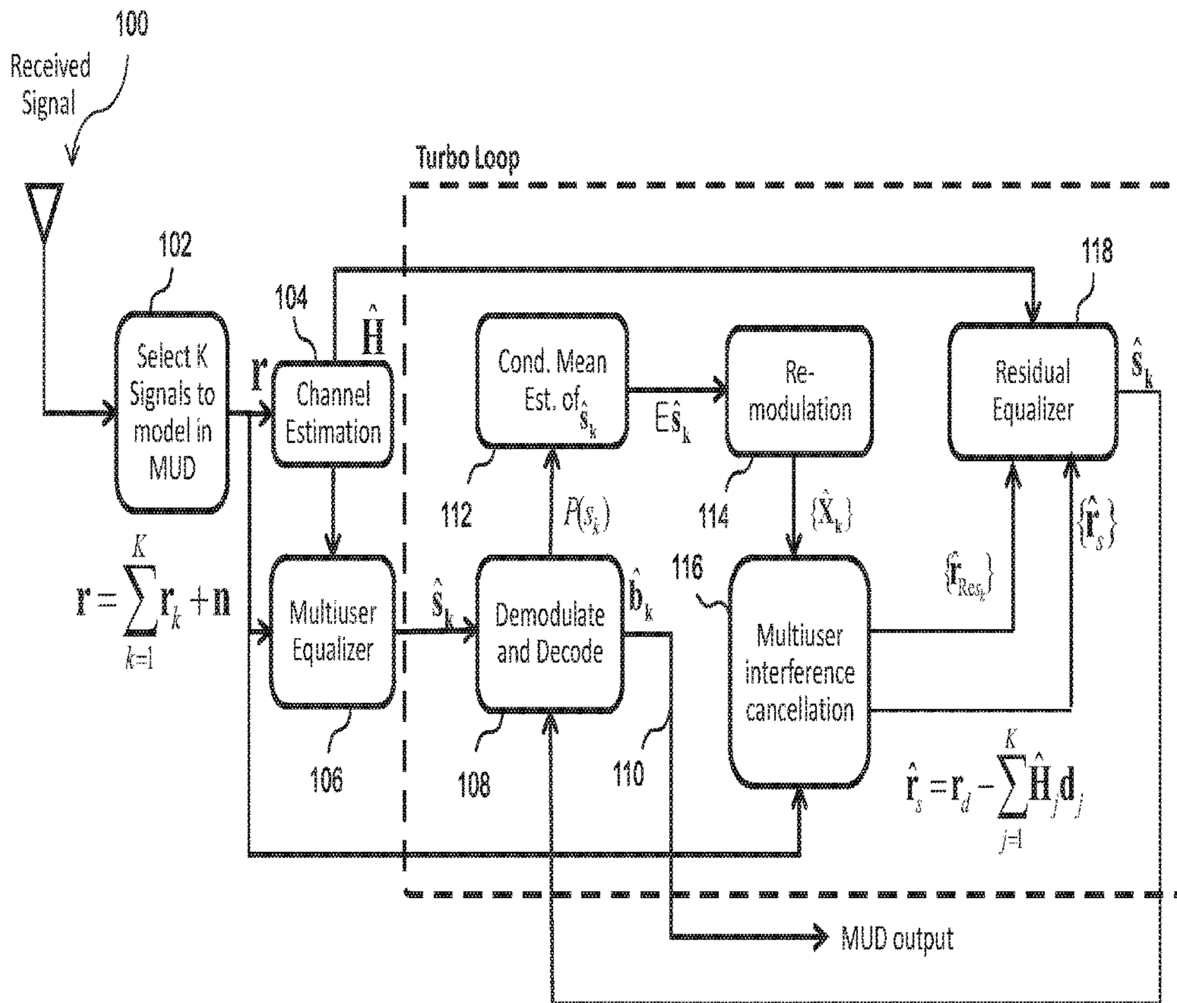
FIG. 1 (Prior art)
