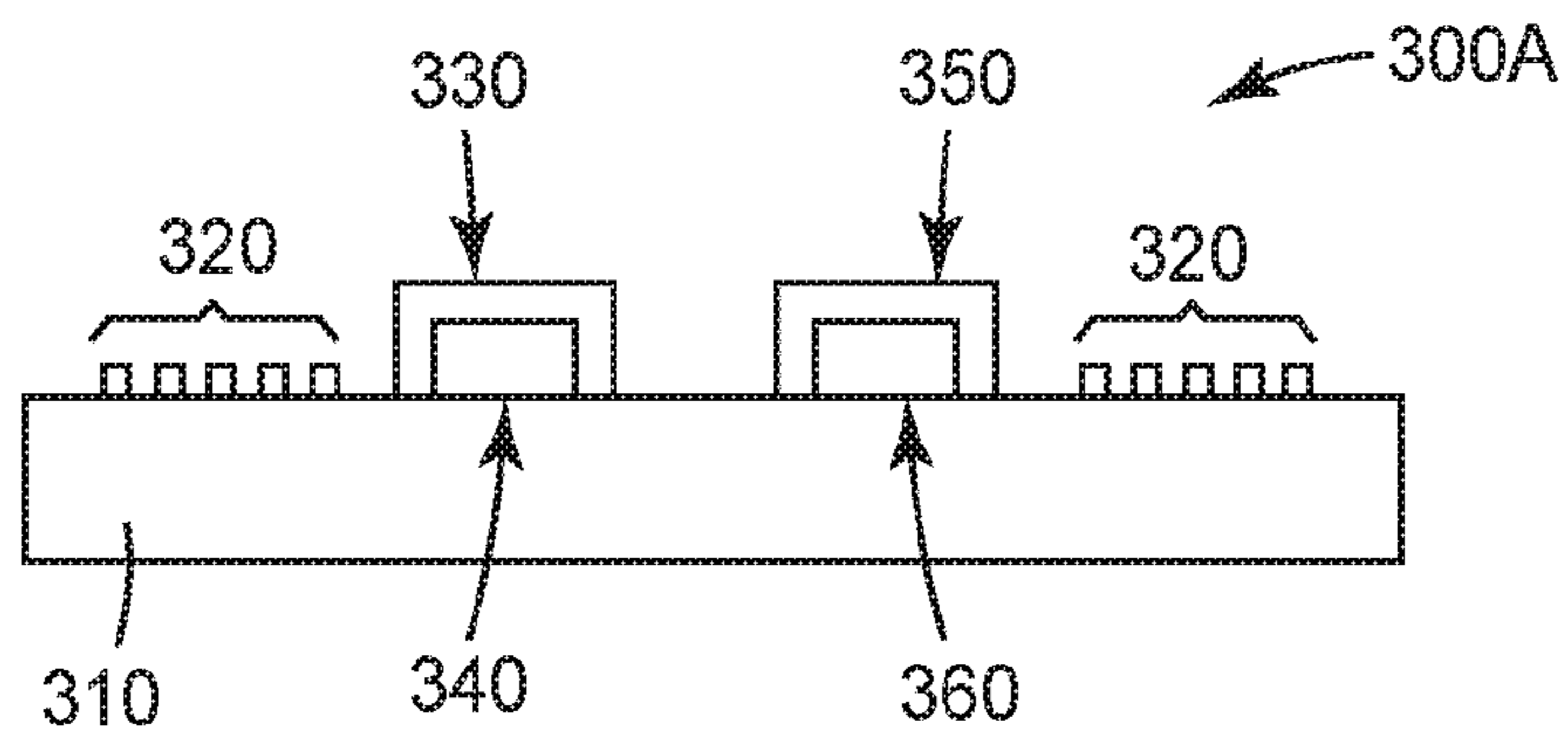
FIG. 3D
