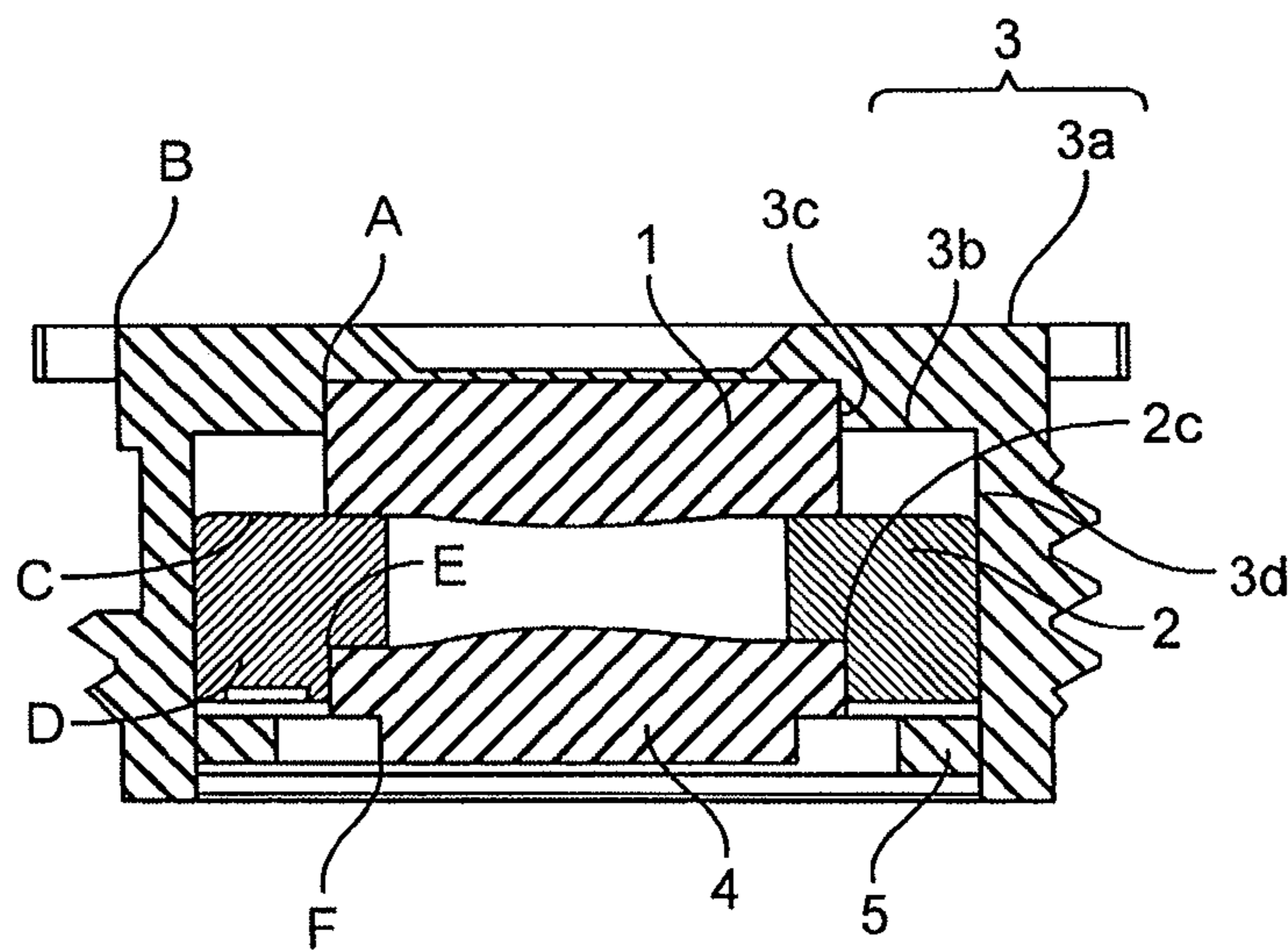
SECTION E-E
