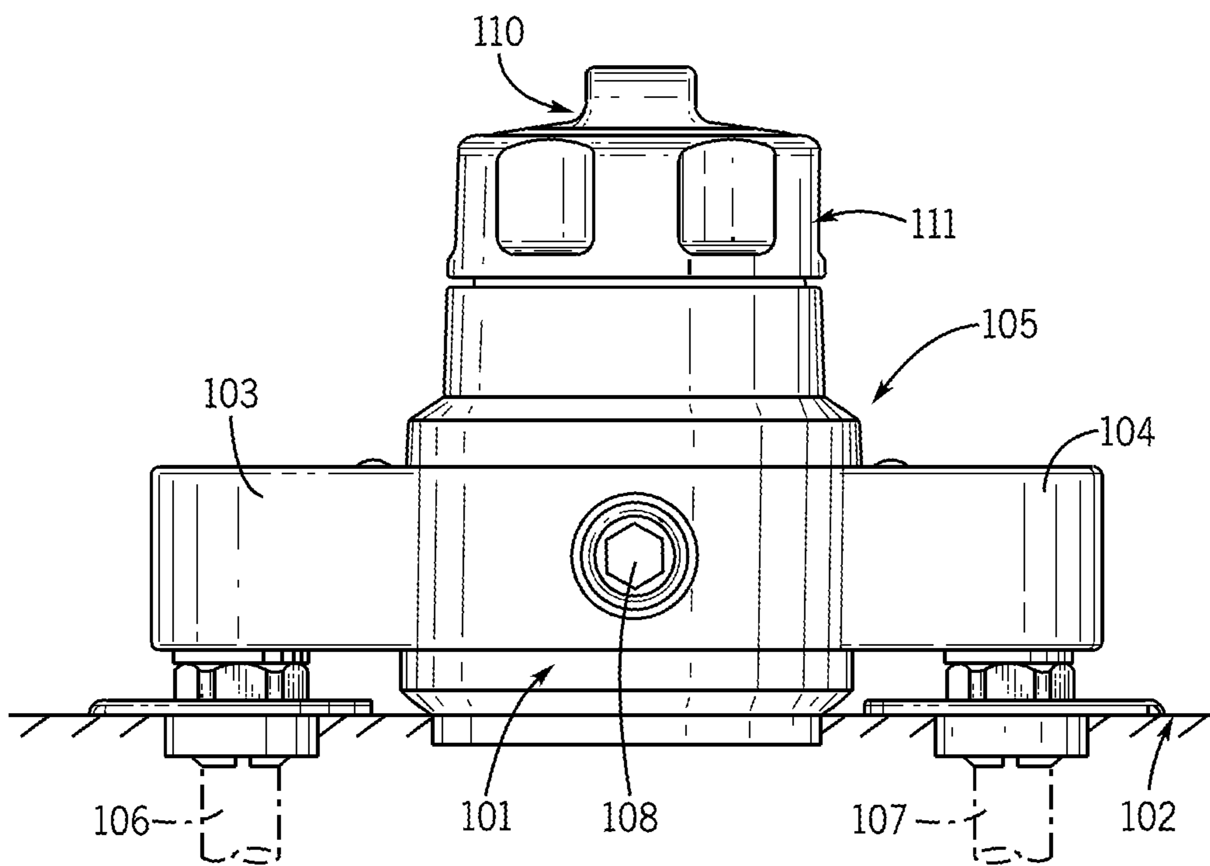
FIG. 13 PRIOR ART
