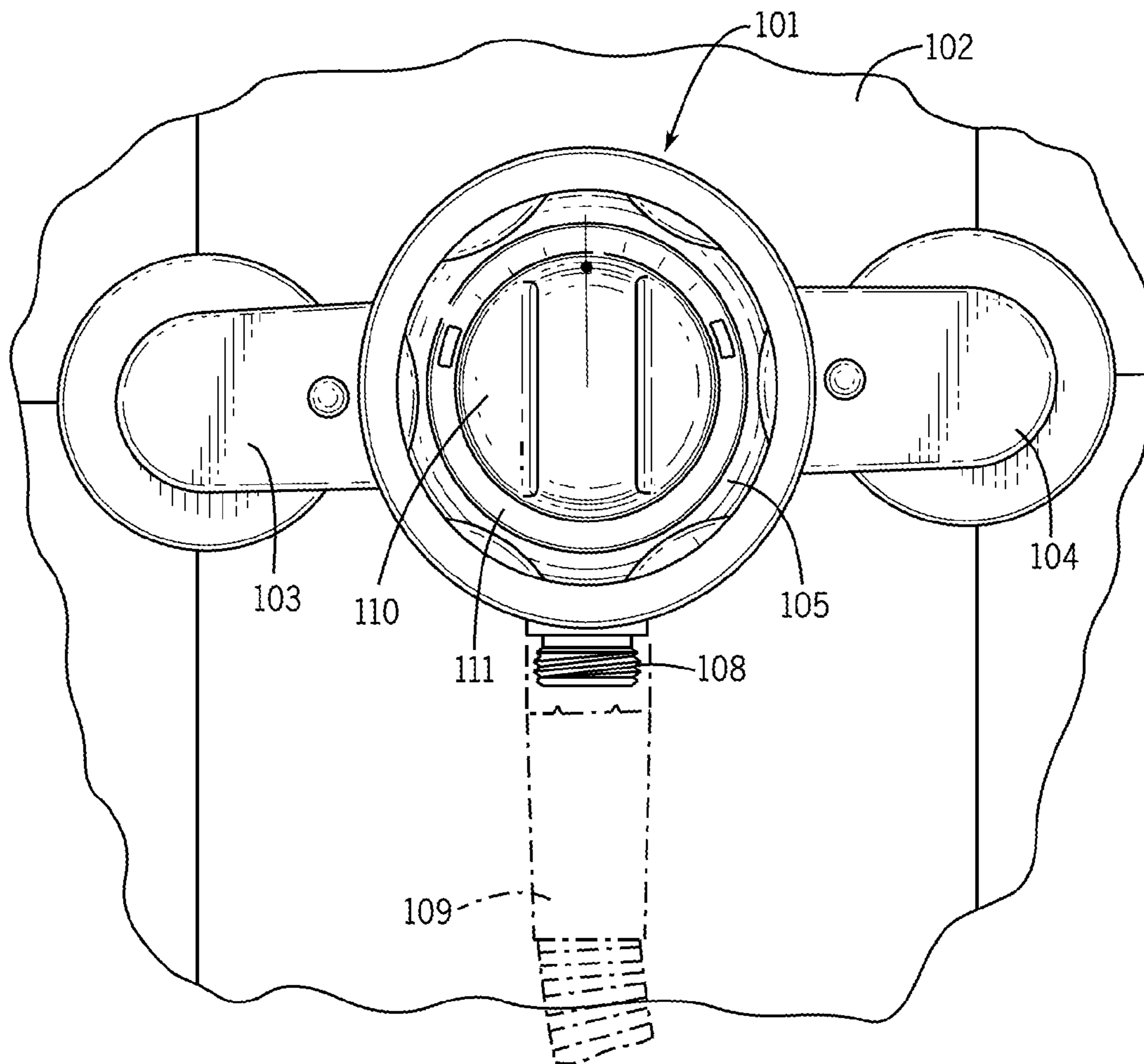
FIG. 12 PRIOR ART
