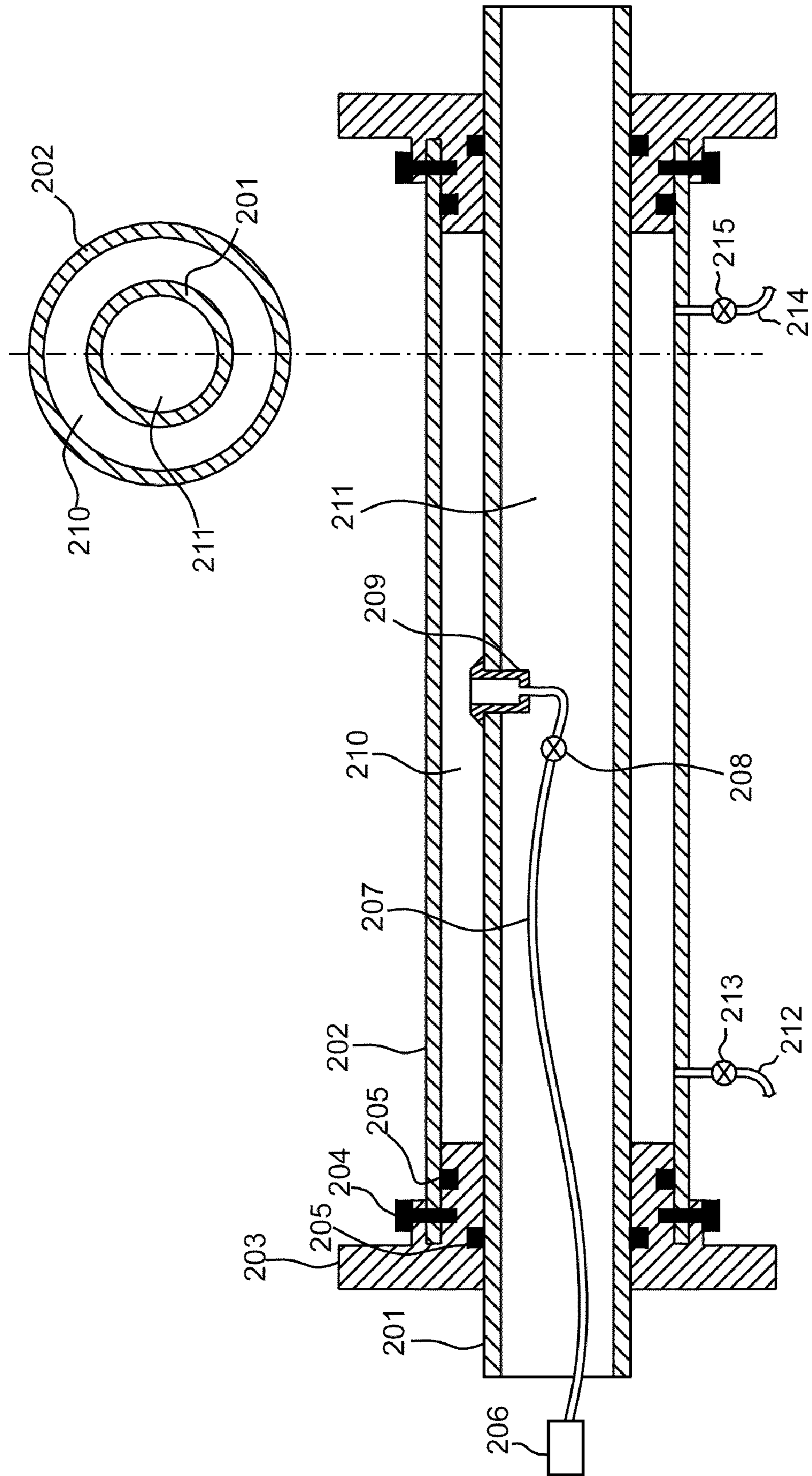
Figure 2 – Sealing fluid test assembly
