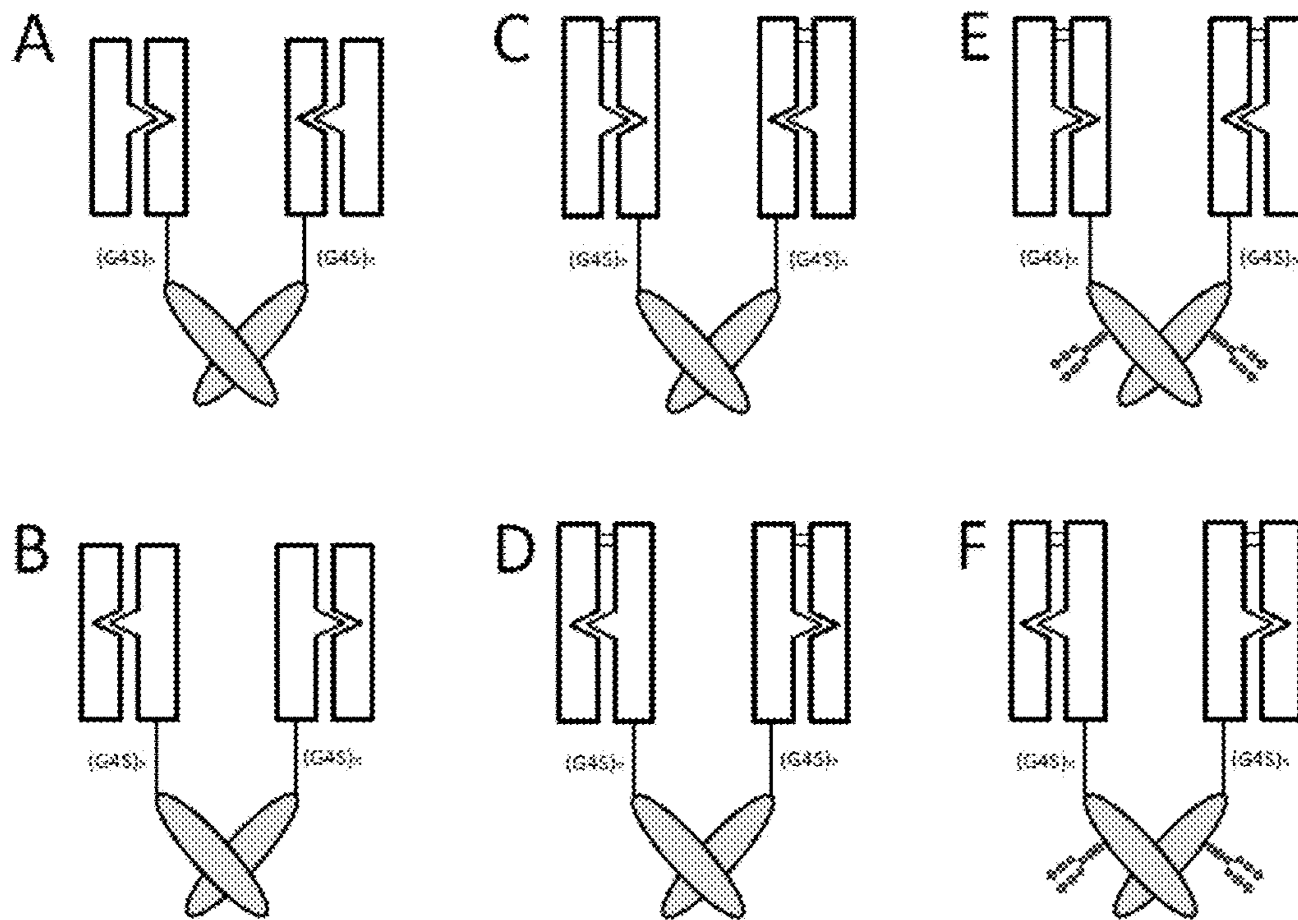
Figure 1 – Designs of knob-in-hole (Fc/Fc)-GDF15 molecules
