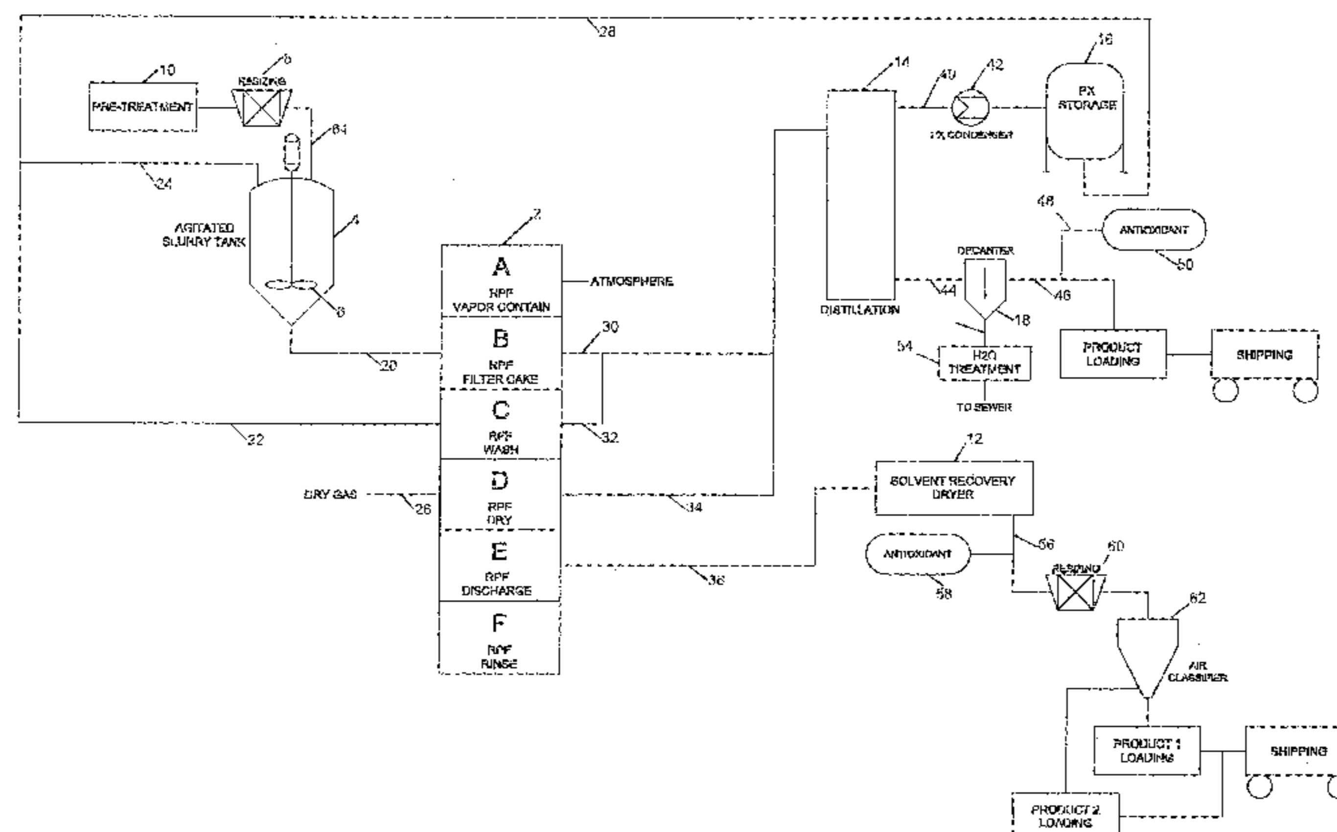
Process Flow Diagram
