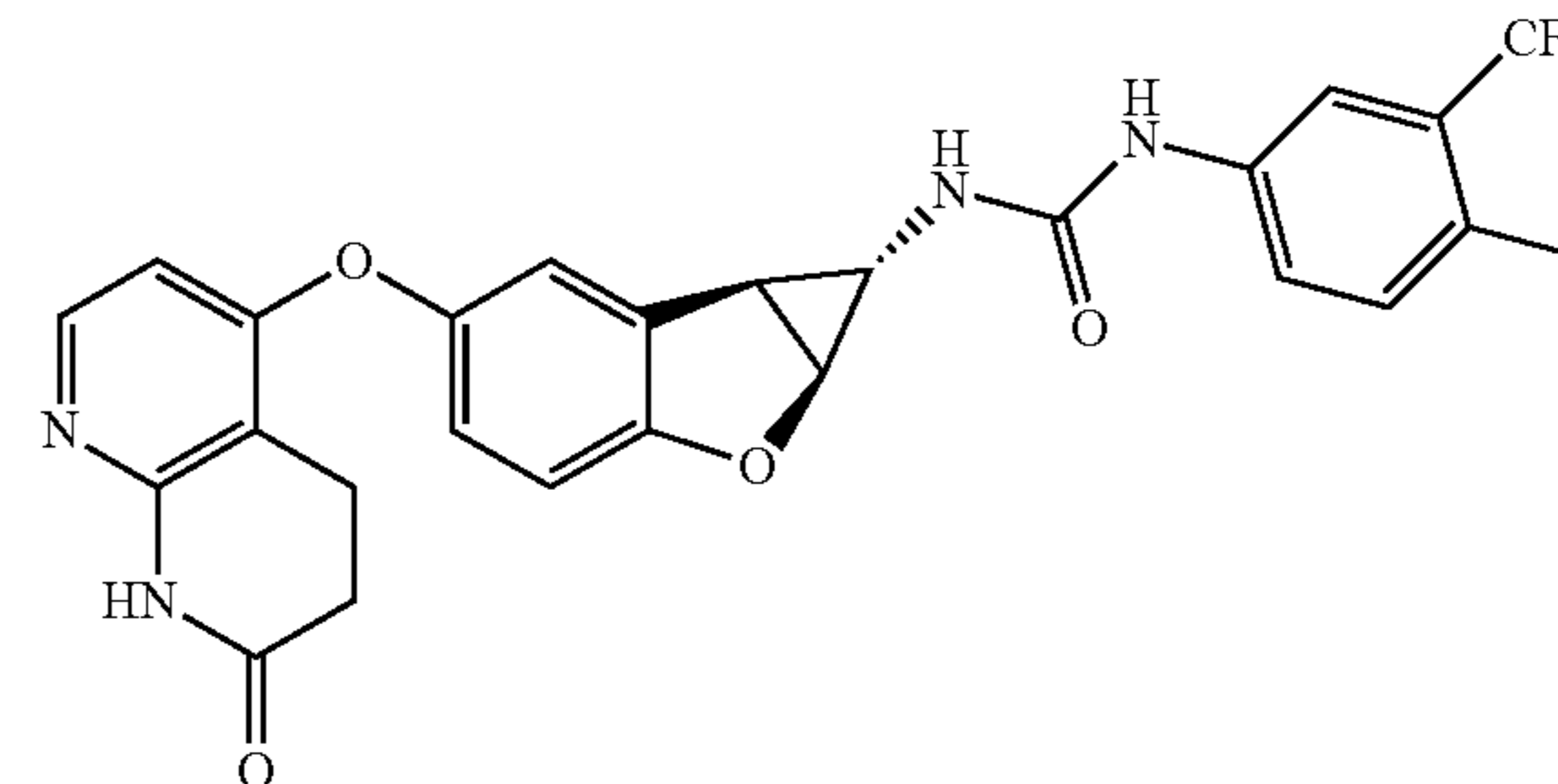
Compound 1.32
