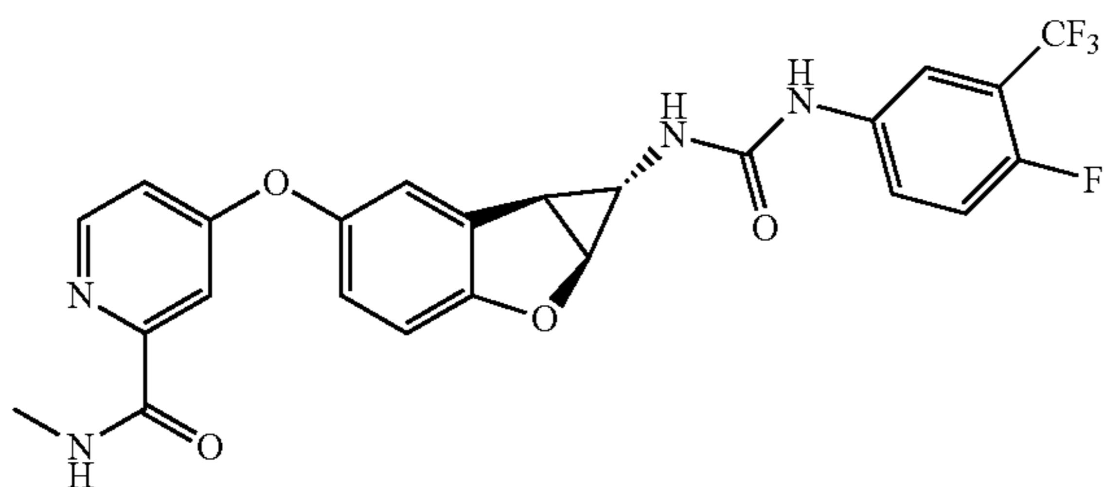
Compound 2.7
