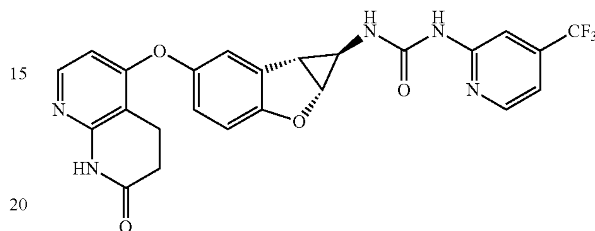
Compound 1.72
