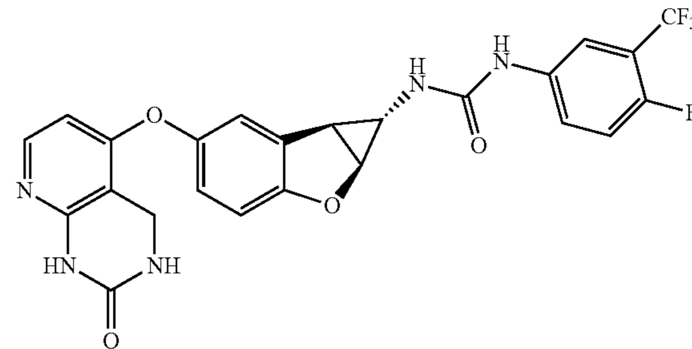
Compound 2.5
