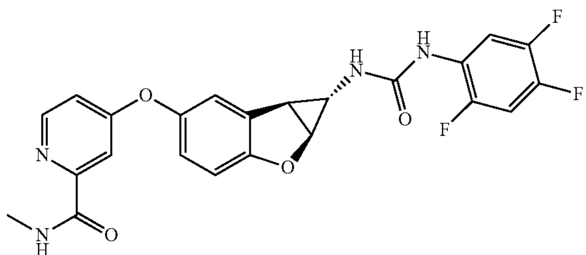
Compound 2.9
