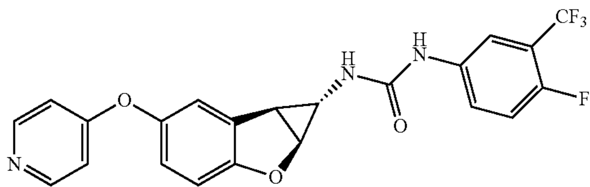
Compound 2.10
