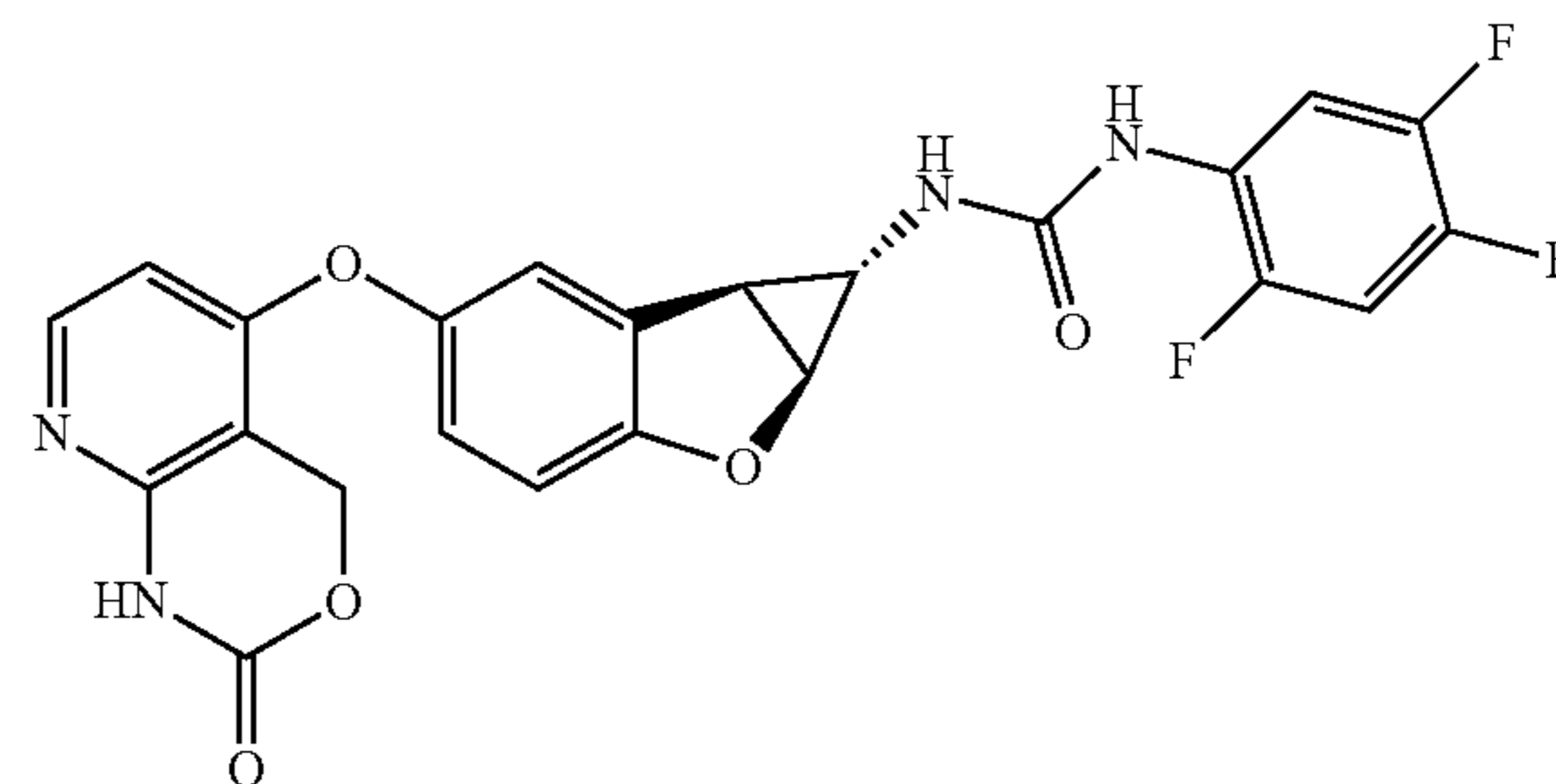
Compound 2.4
