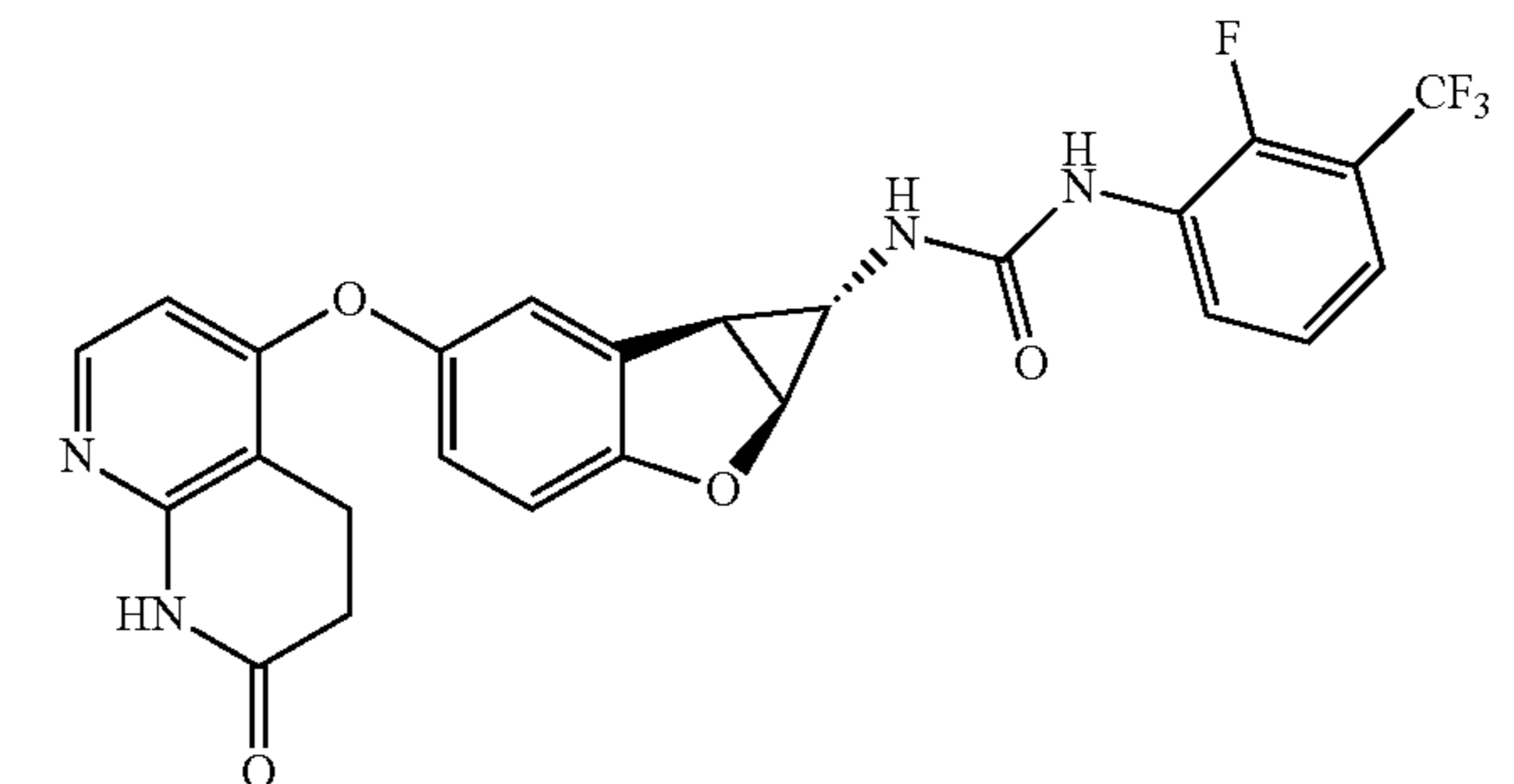
Compound 1.12
