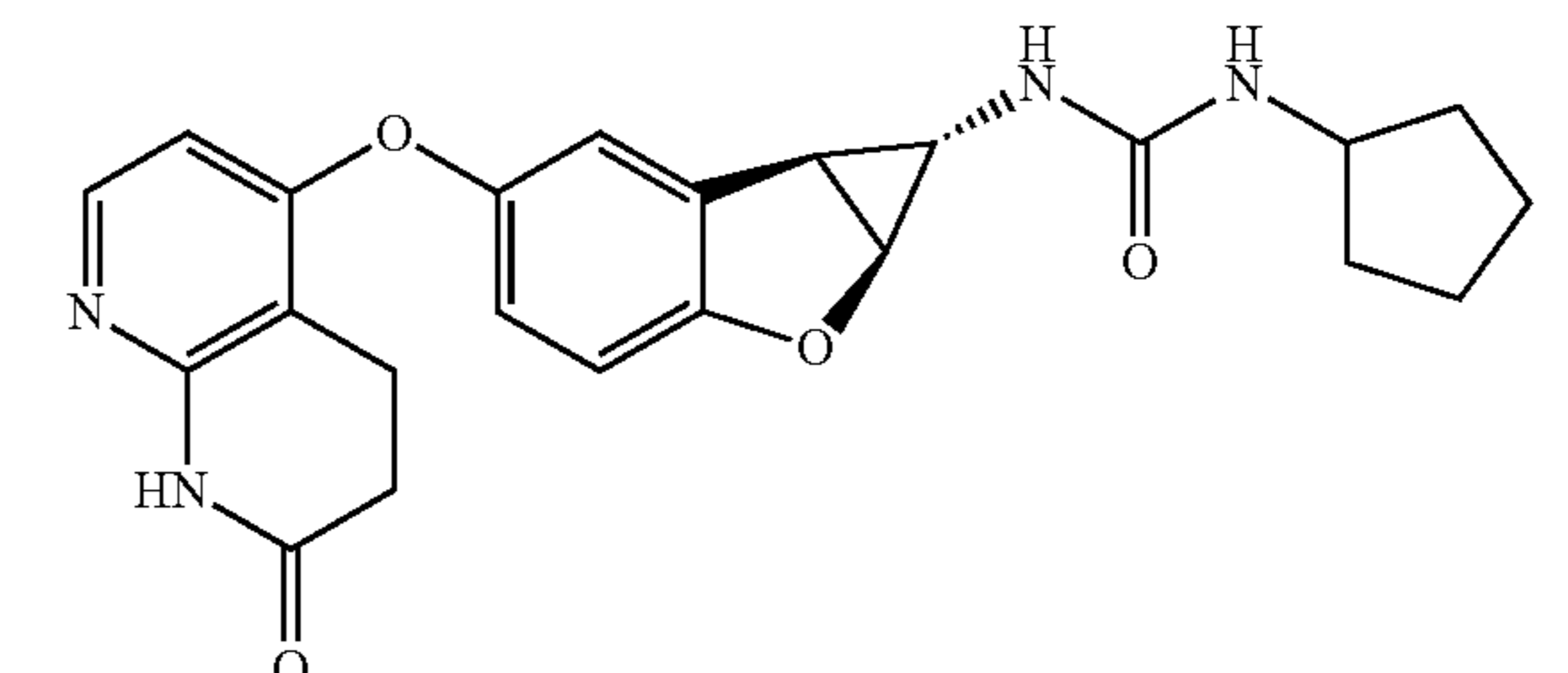
Compound 1.52
