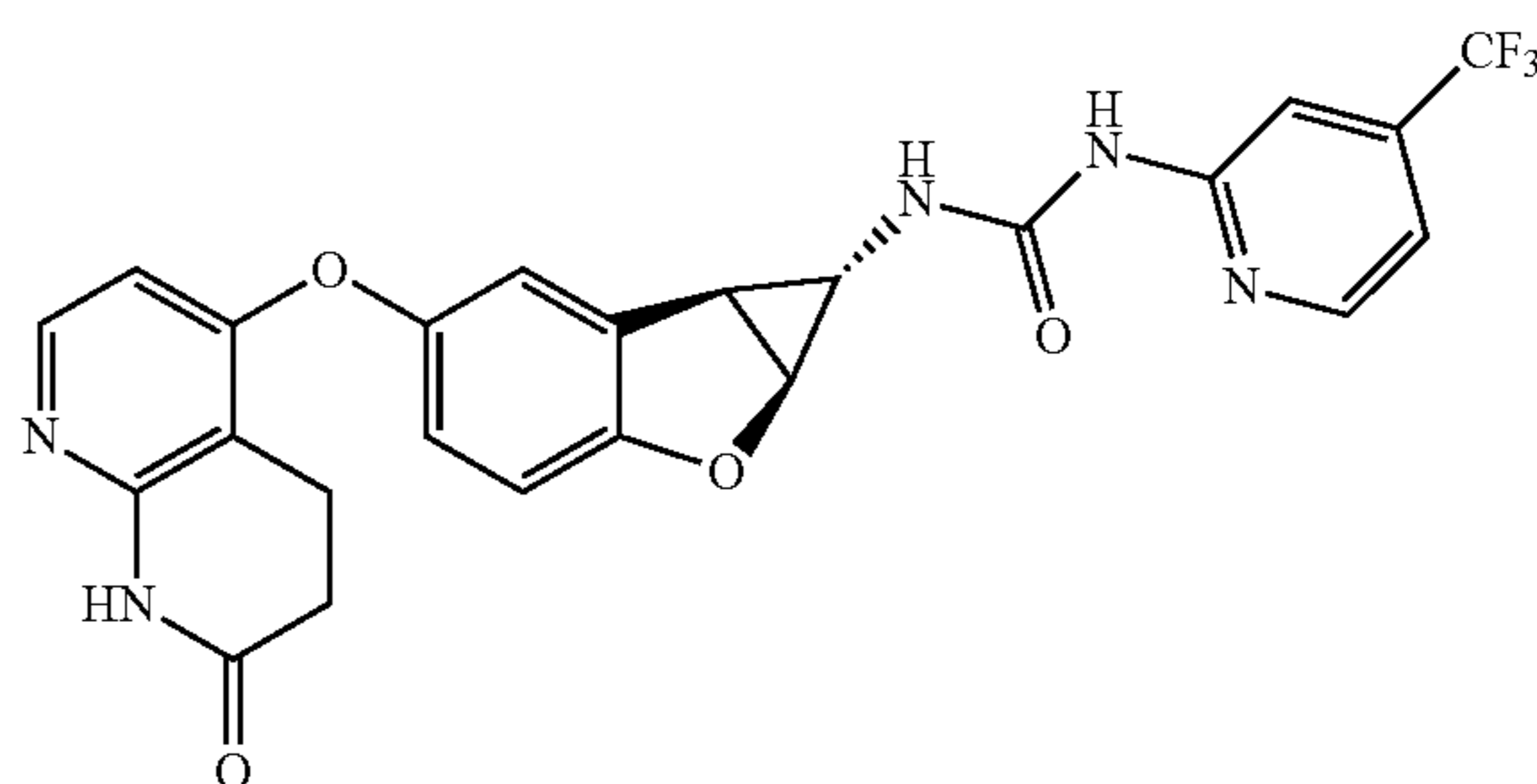
Compound 1.2
