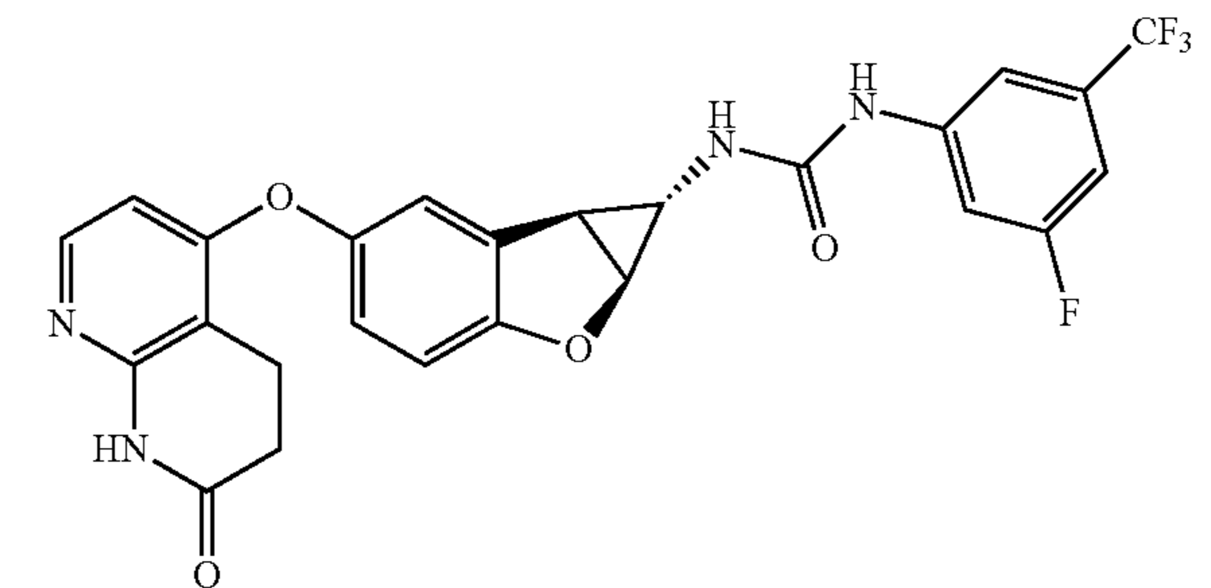
Compound 1.12
