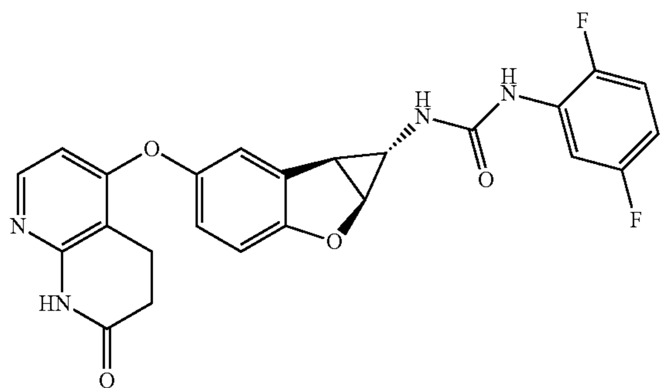
Compound 1.44
