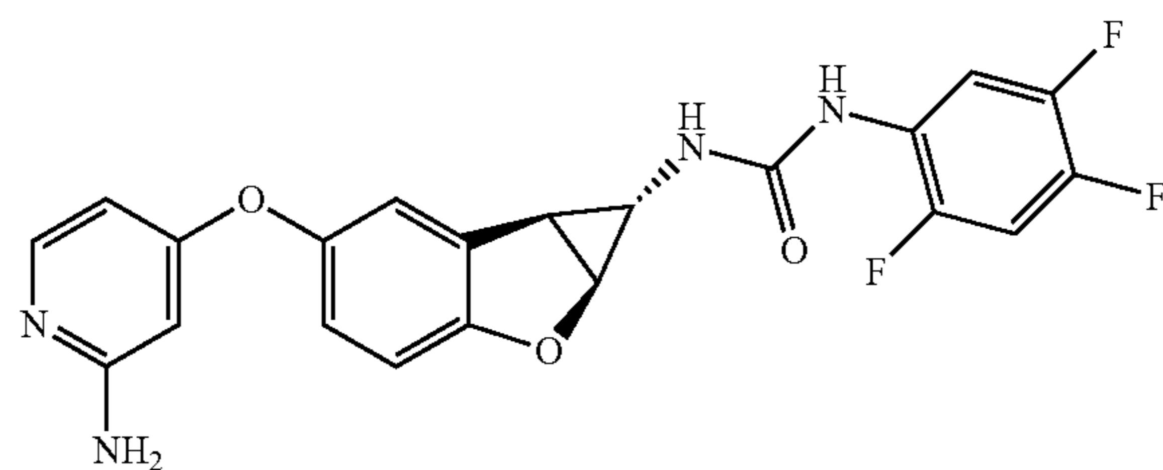
Compound 2.16
