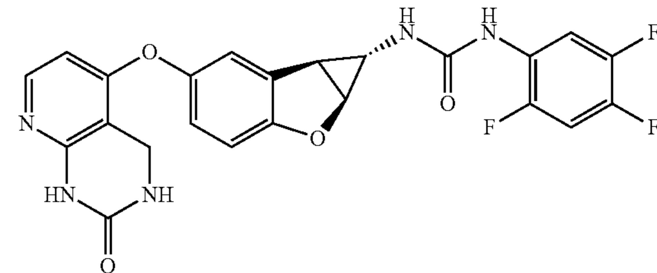
Compound 2.5
