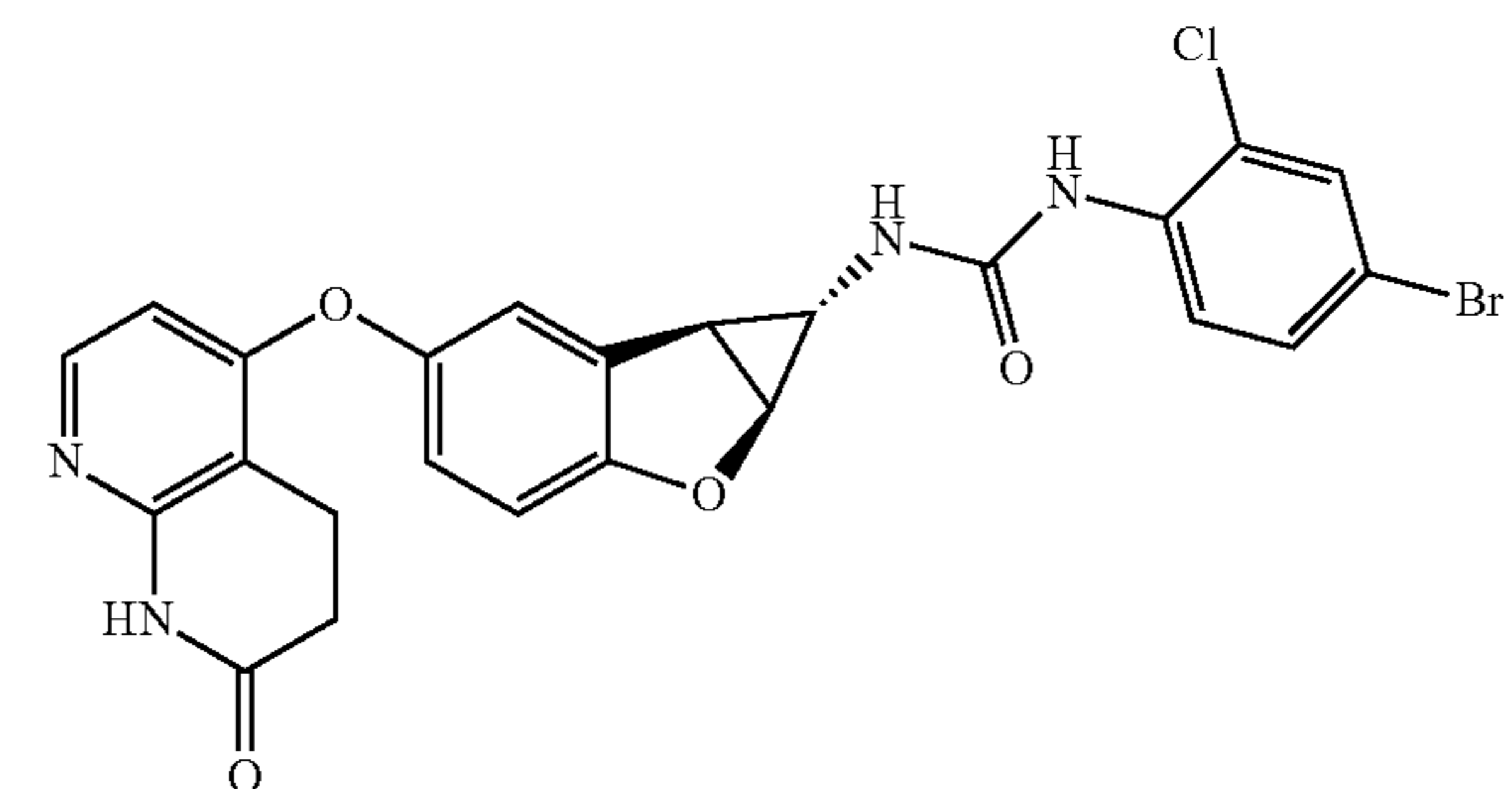
Compound 1.11
