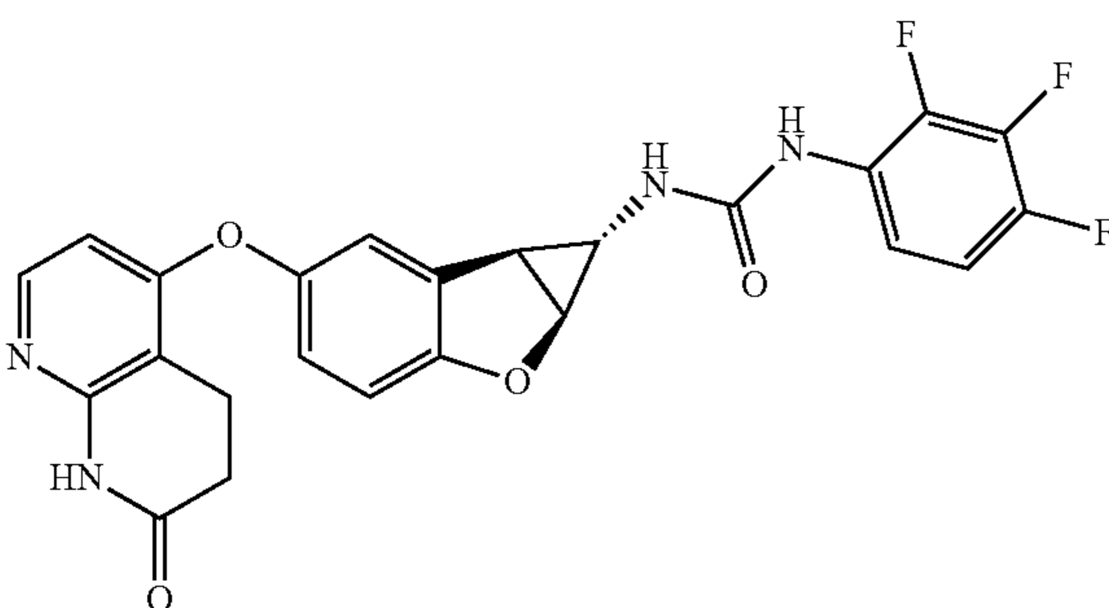
Compound 1.47
