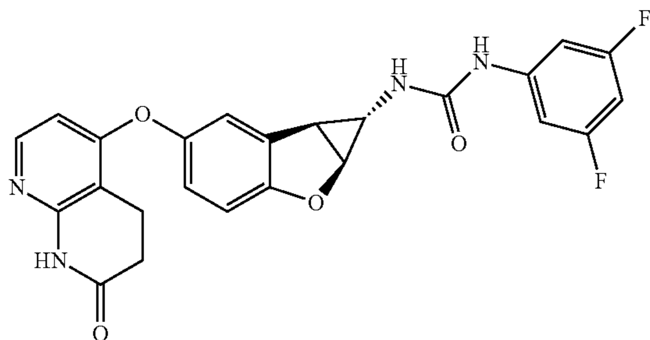
Compound 1.23
