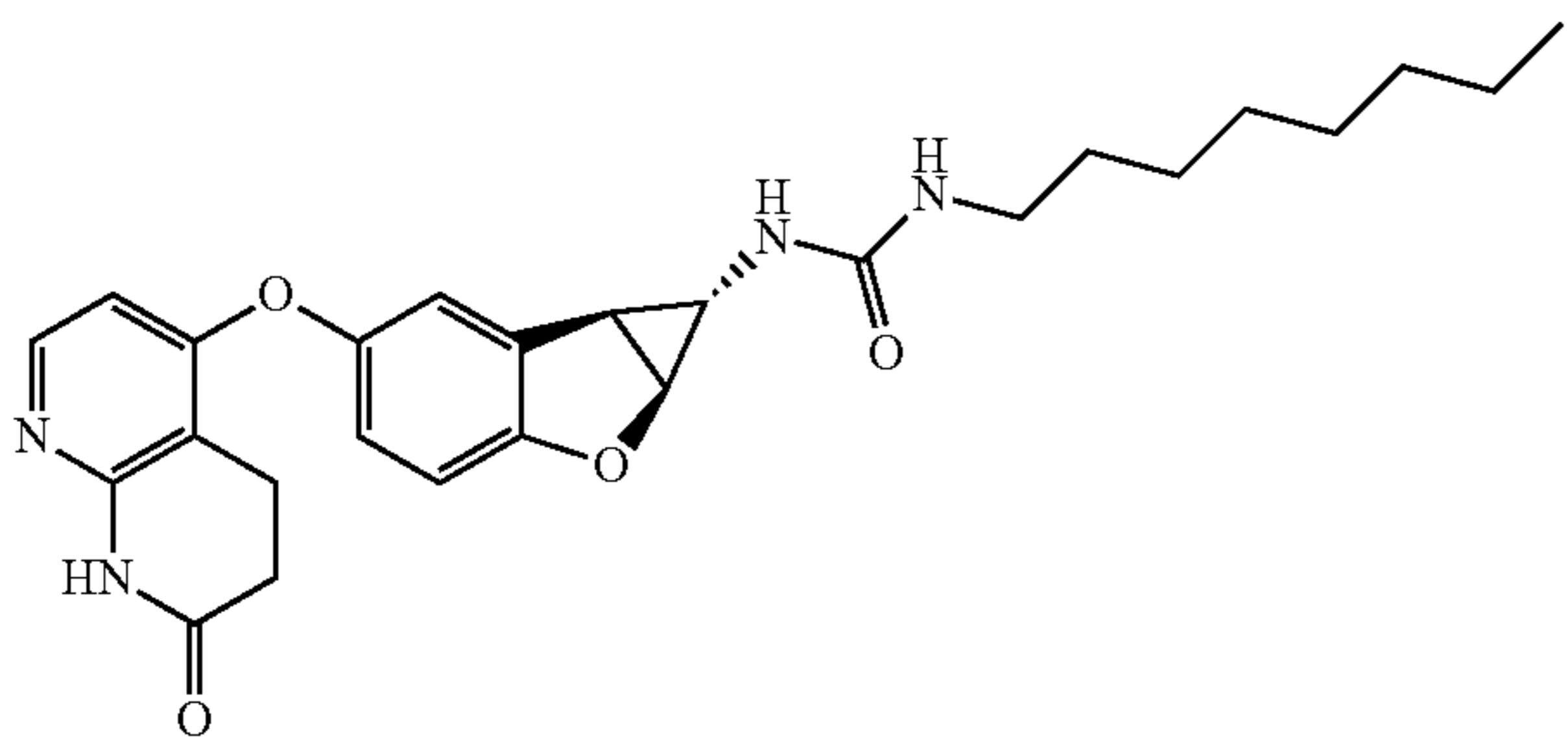
Compound 1.85
