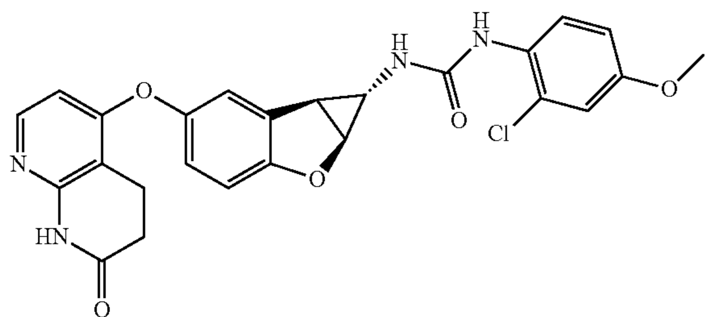
Compound 1.4
