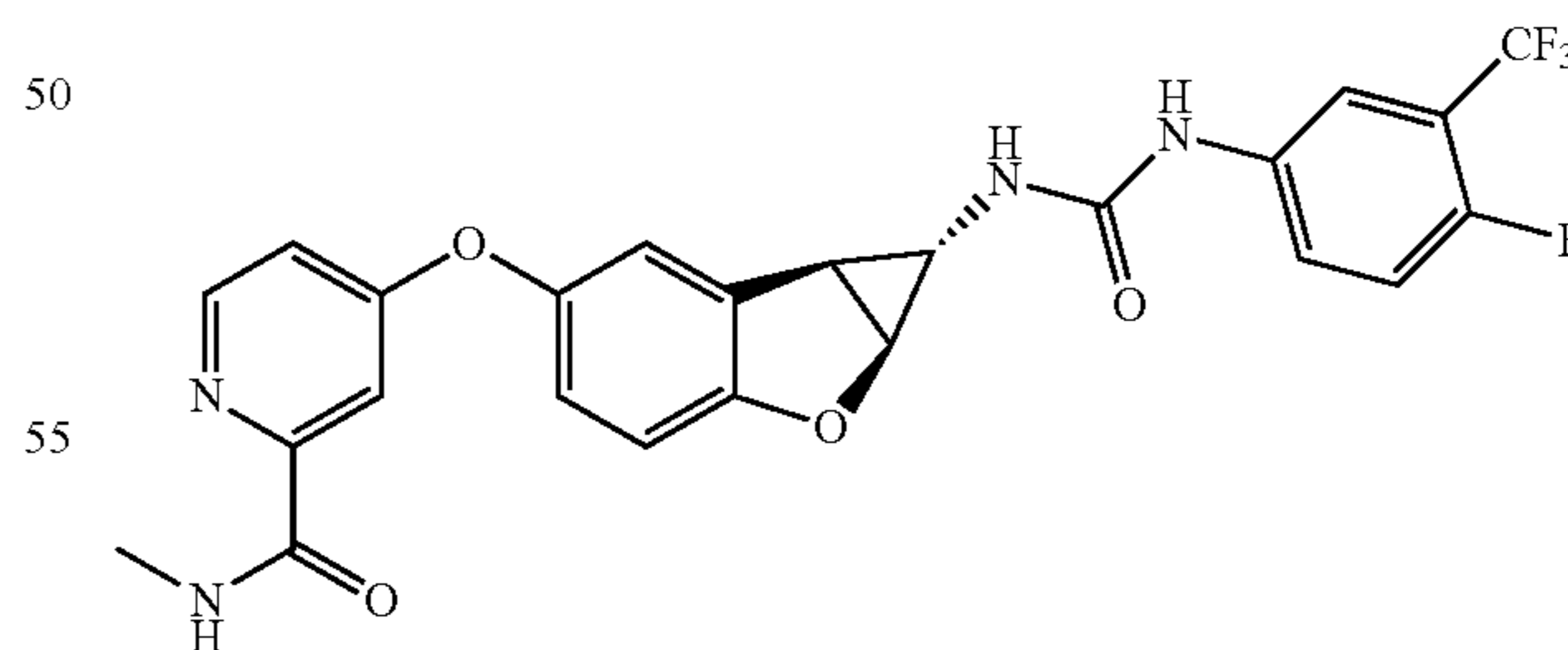
Compound 2.7
