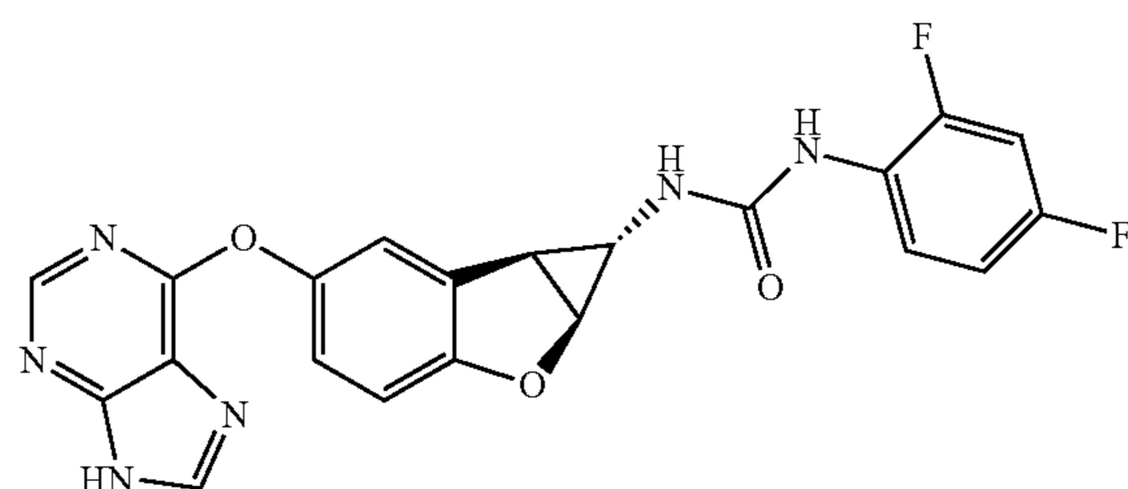
Compound 2.13
