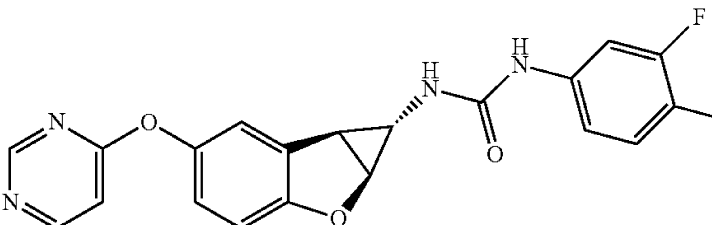
Compound 2.3
