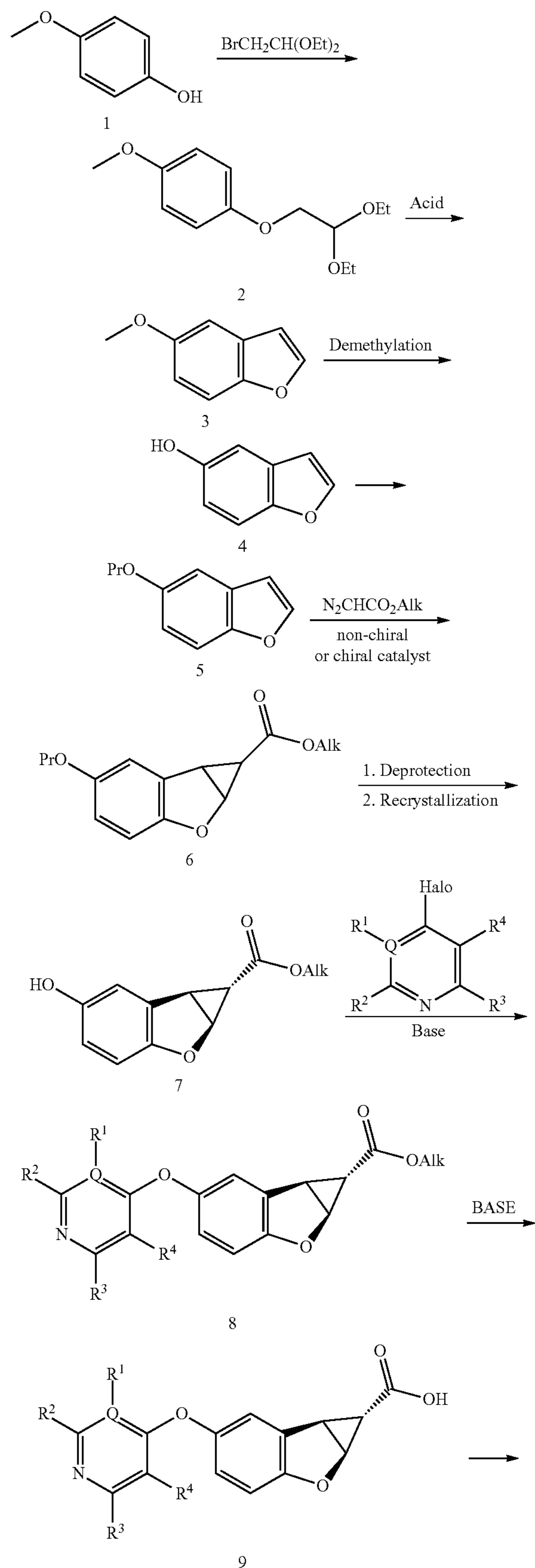
Scheme I
