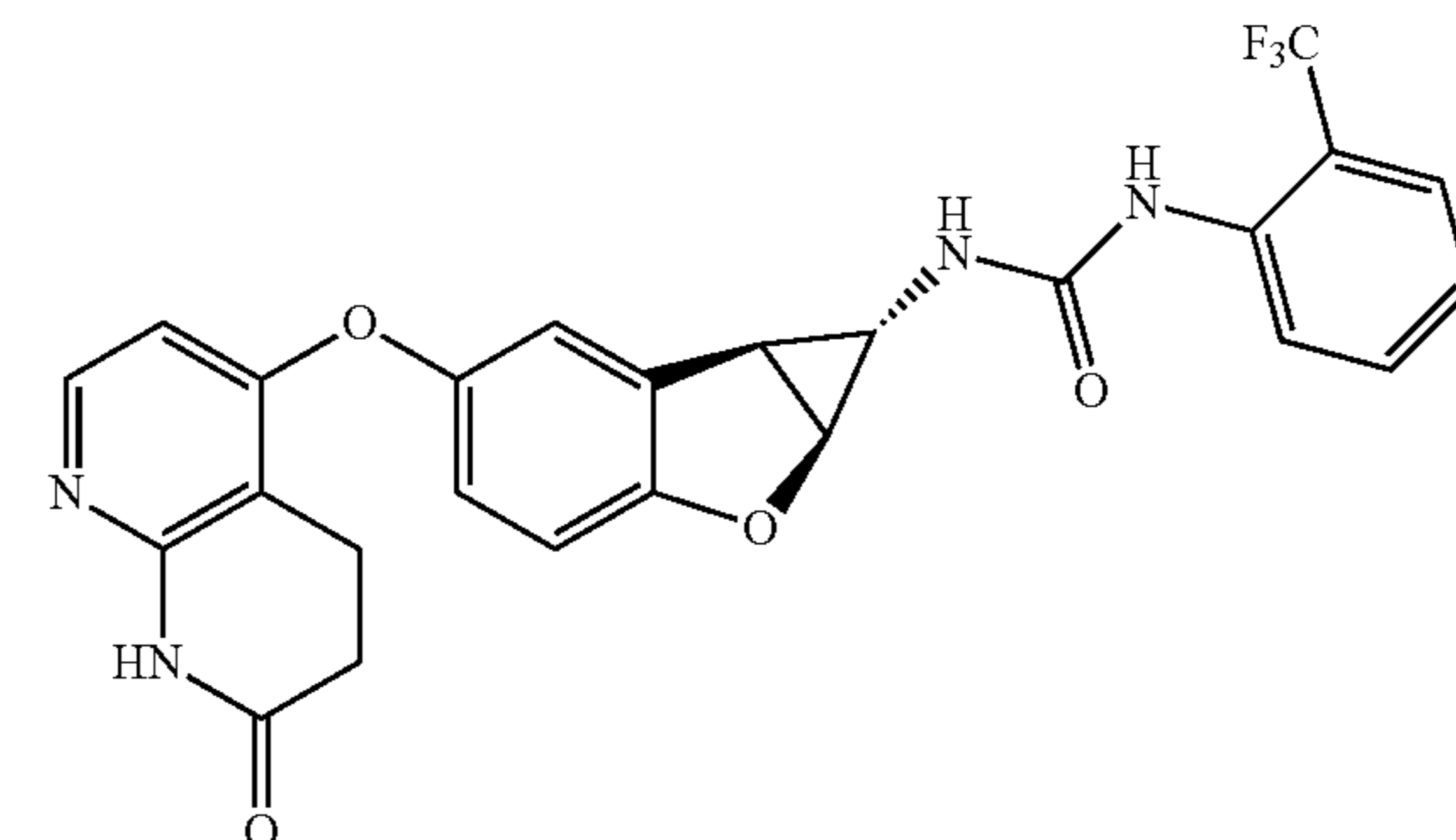
Compound 1.31
