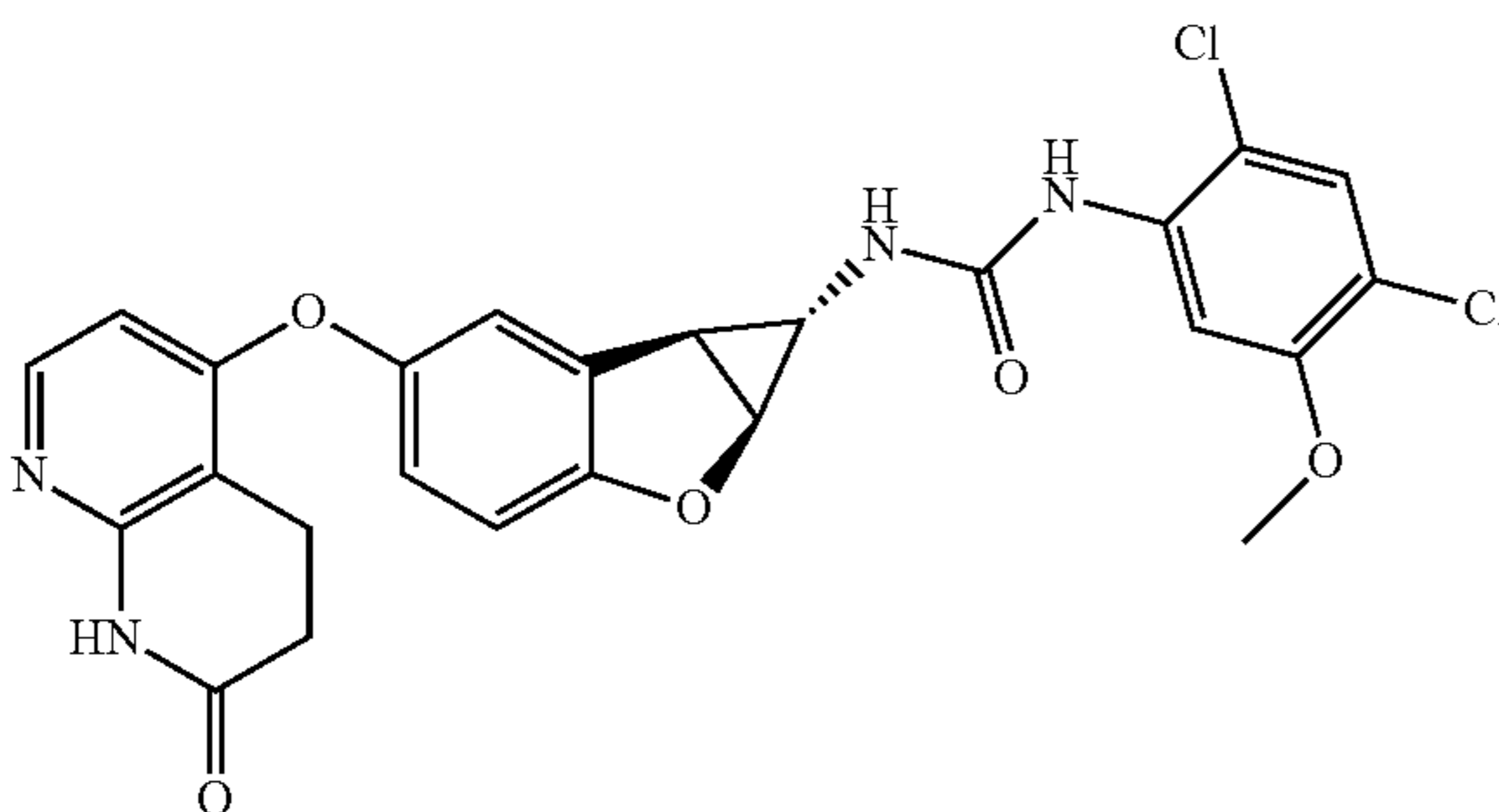
Compound 1.27
