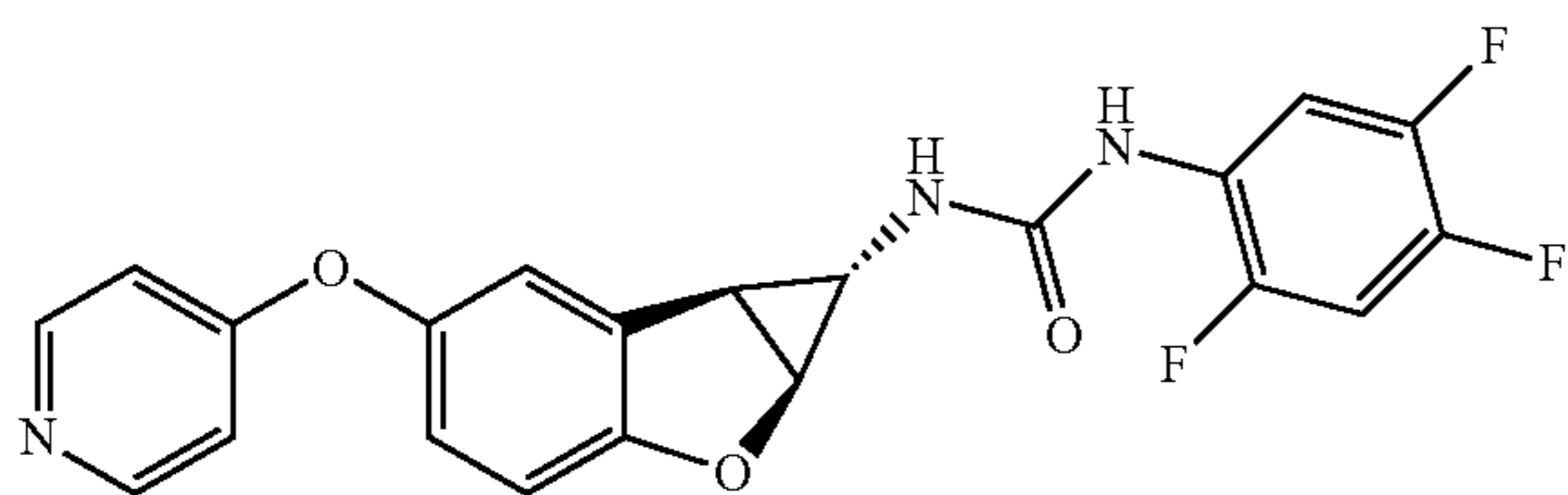
Compound 2.11
