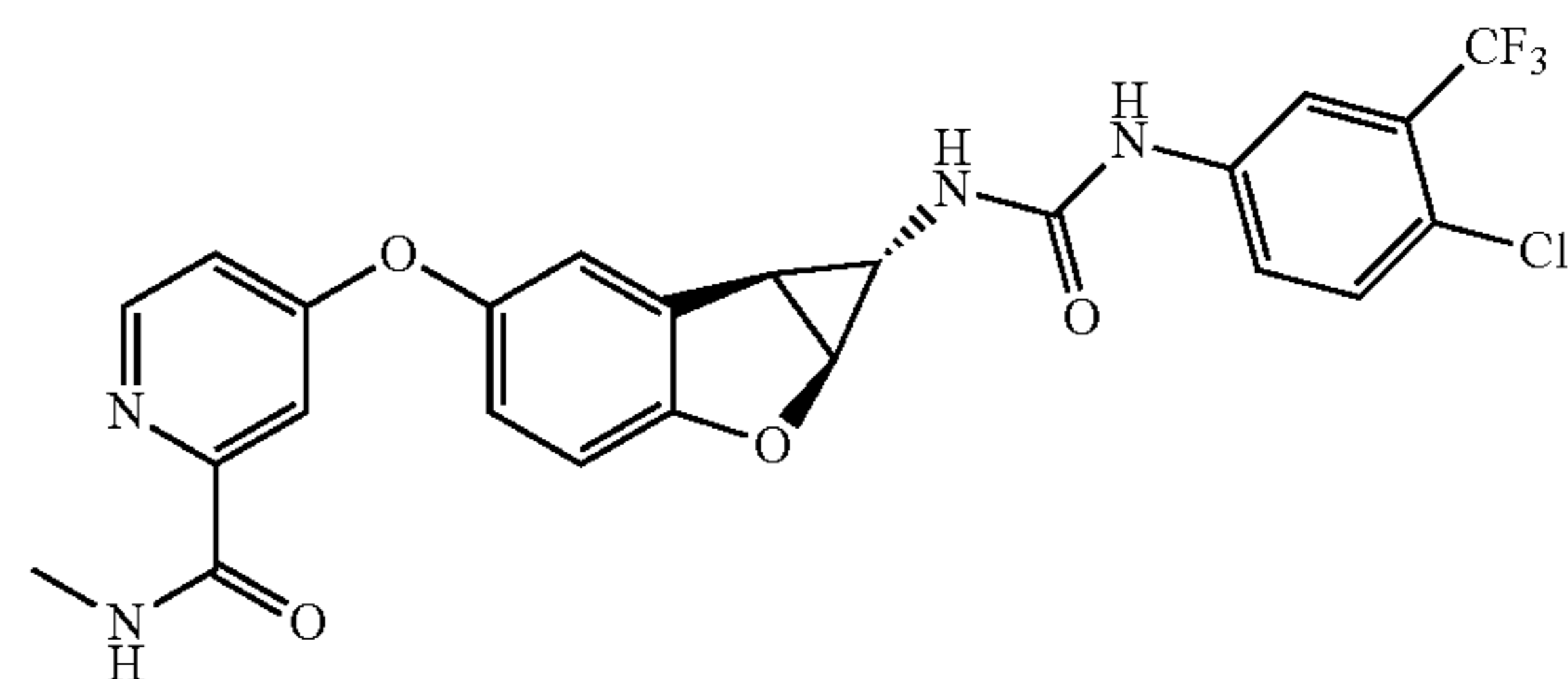
Compound 2.16
