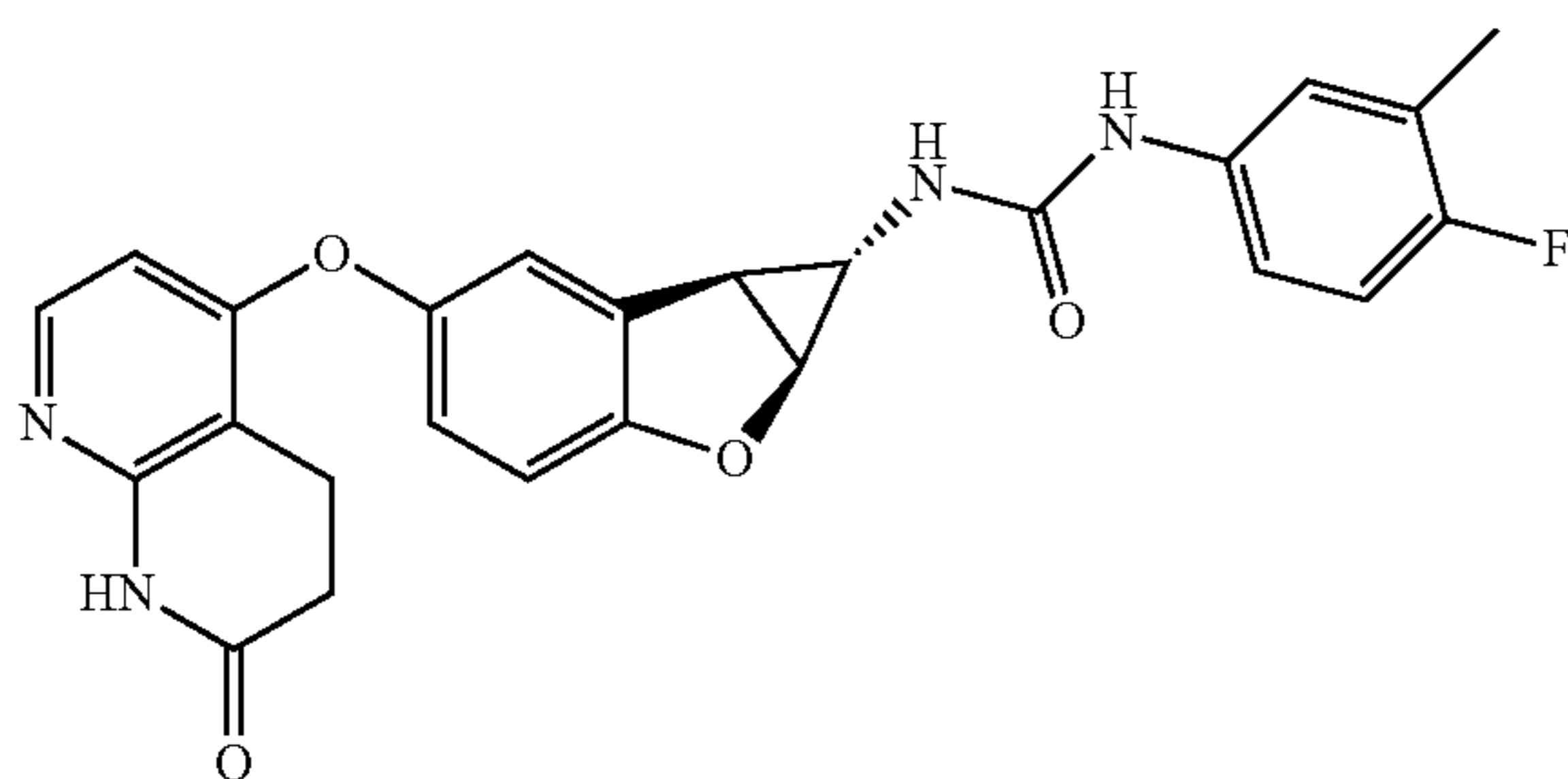
Compound 1.24
