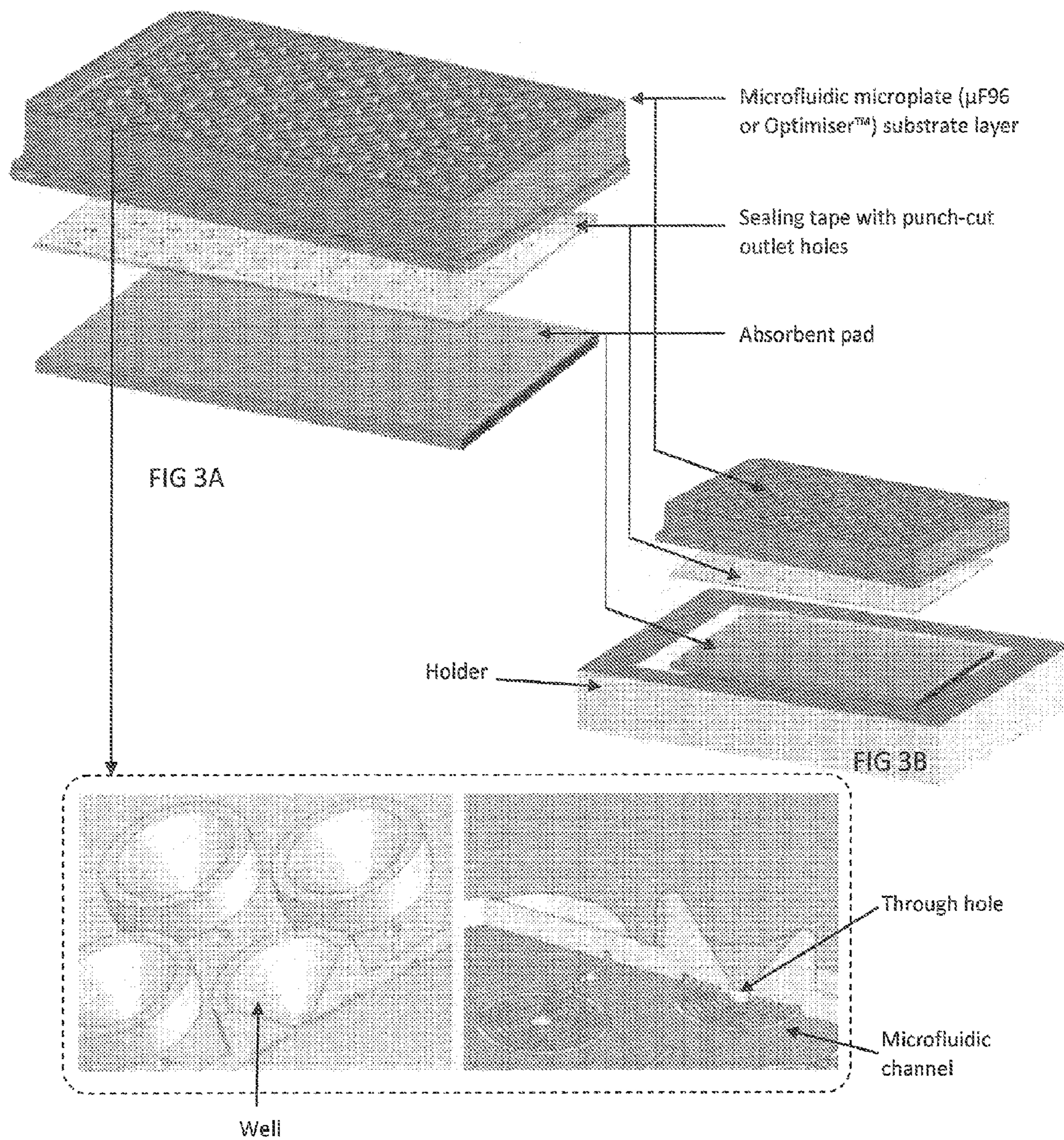
FIG 3. 3D schematic views of an embodiment of the microfluidic microplate. FIG 3A shows the basic constituents of the microfluidic microplate – namely the substrate layer, sealing layer and absorbent pad. FIG 3B shows the use of the microfluidic microplate with a suitable designed holder. Insert images at bottom show close up views of the substrate layer showing the well, through hole and microchannel structures.
