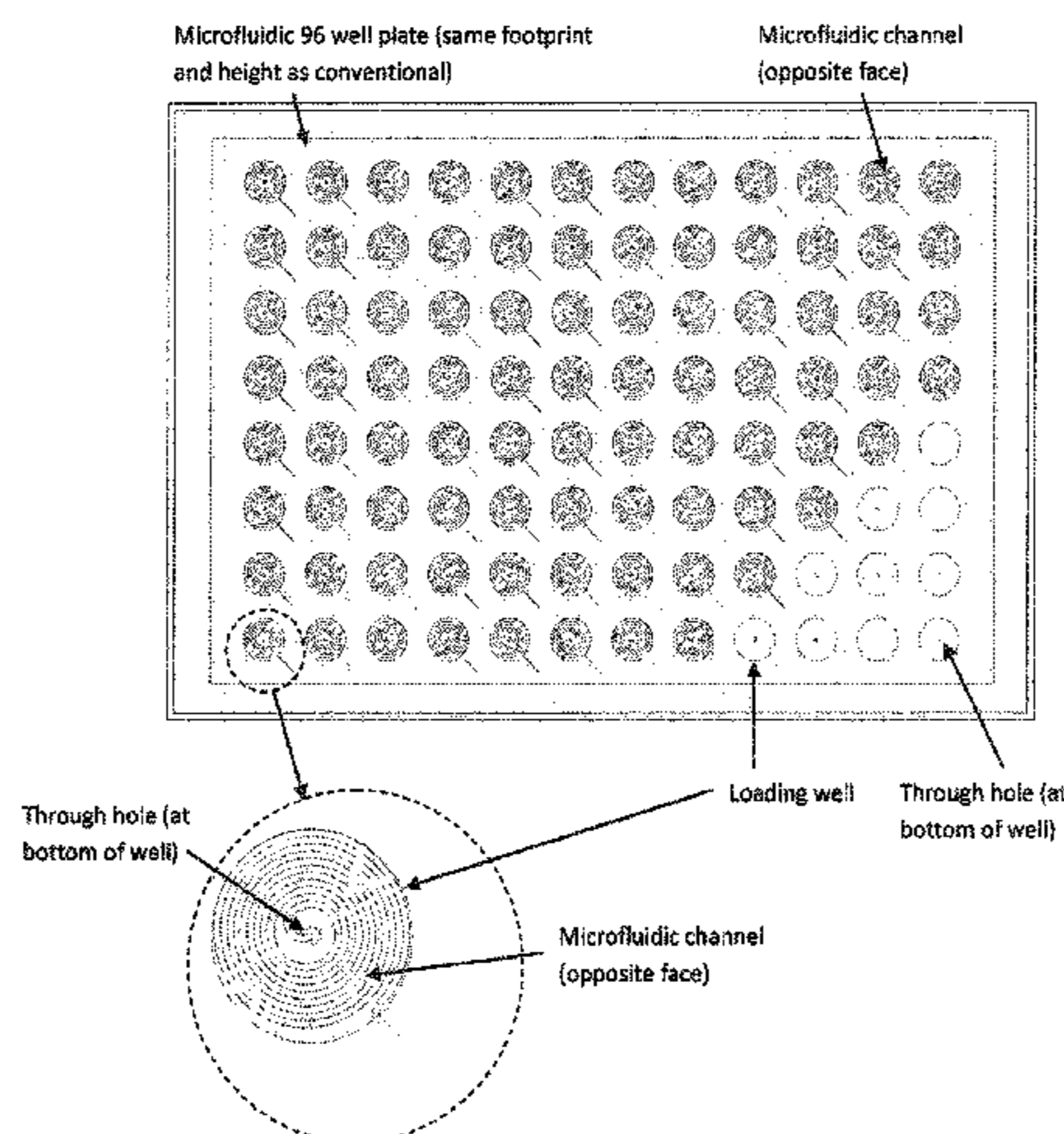
Microfluidic 96 well plate concept. The plate matches the dimensions of conventional microplates (as defined by accepted ANSI standards). The positions of the wells also matches ANSI standards. Each well is connected to a microchannel on the opposing face of the substrate. Figure does not show sealing layer (for microchannels) and absorbent pad for clarity. Also, selected wells in lower right hand corner of top figure do not show microchannel pattern for ease of explanation.
