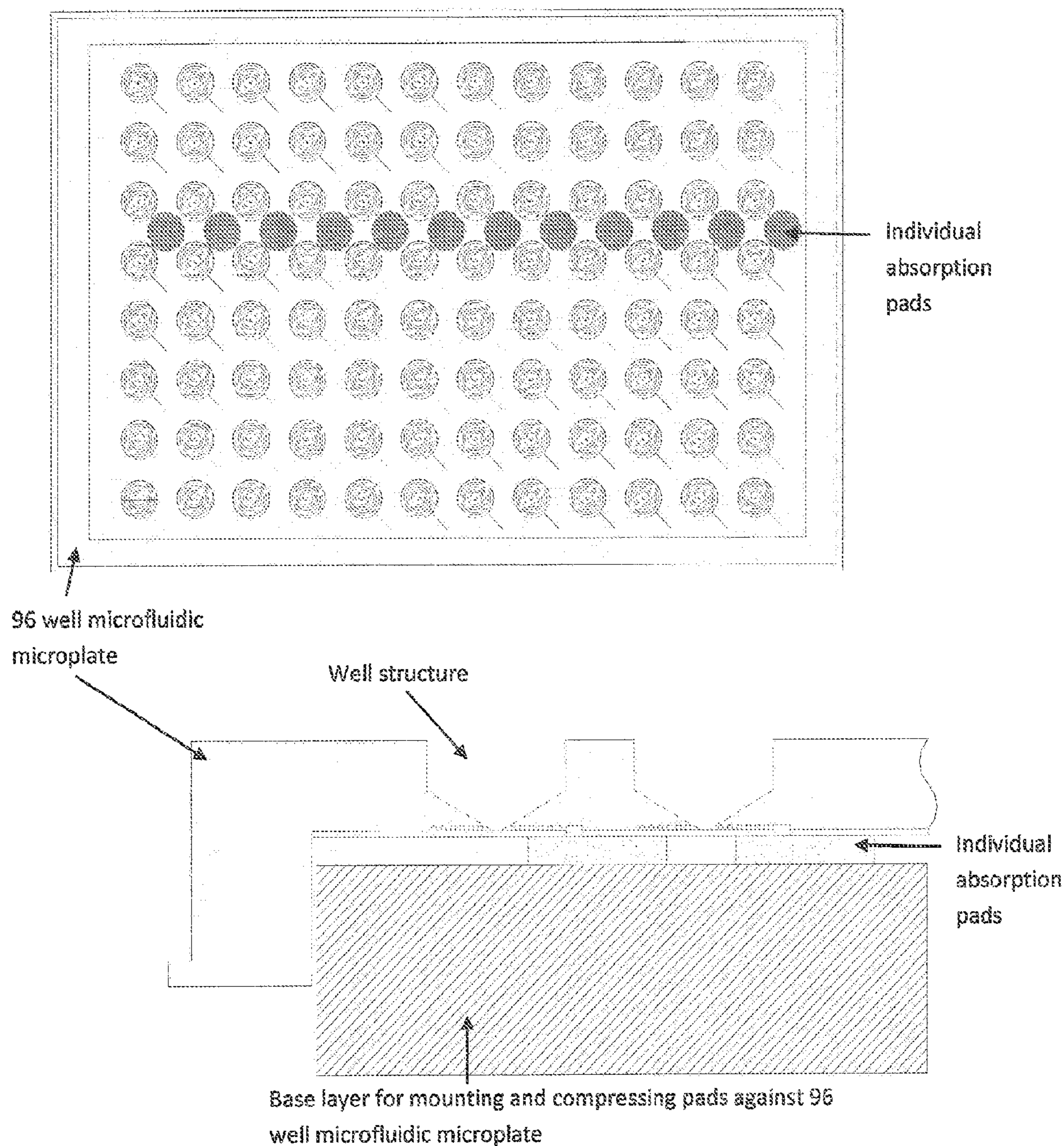
FIG 13. In this configuration, a separate absorption pad is used for each of the 96 wells. Furthermore, the absorptions pads are not physically attached to the microplate; instead they are attached to a base layer over which the microplate is positioned for operation. Furthermore, the pads are not in the same vertical line-of-sight as the wells and the microchannels. For ease of explanation, only one row of absorbent pads is shown; whereas the actual device would contain 96 distinct pads.
