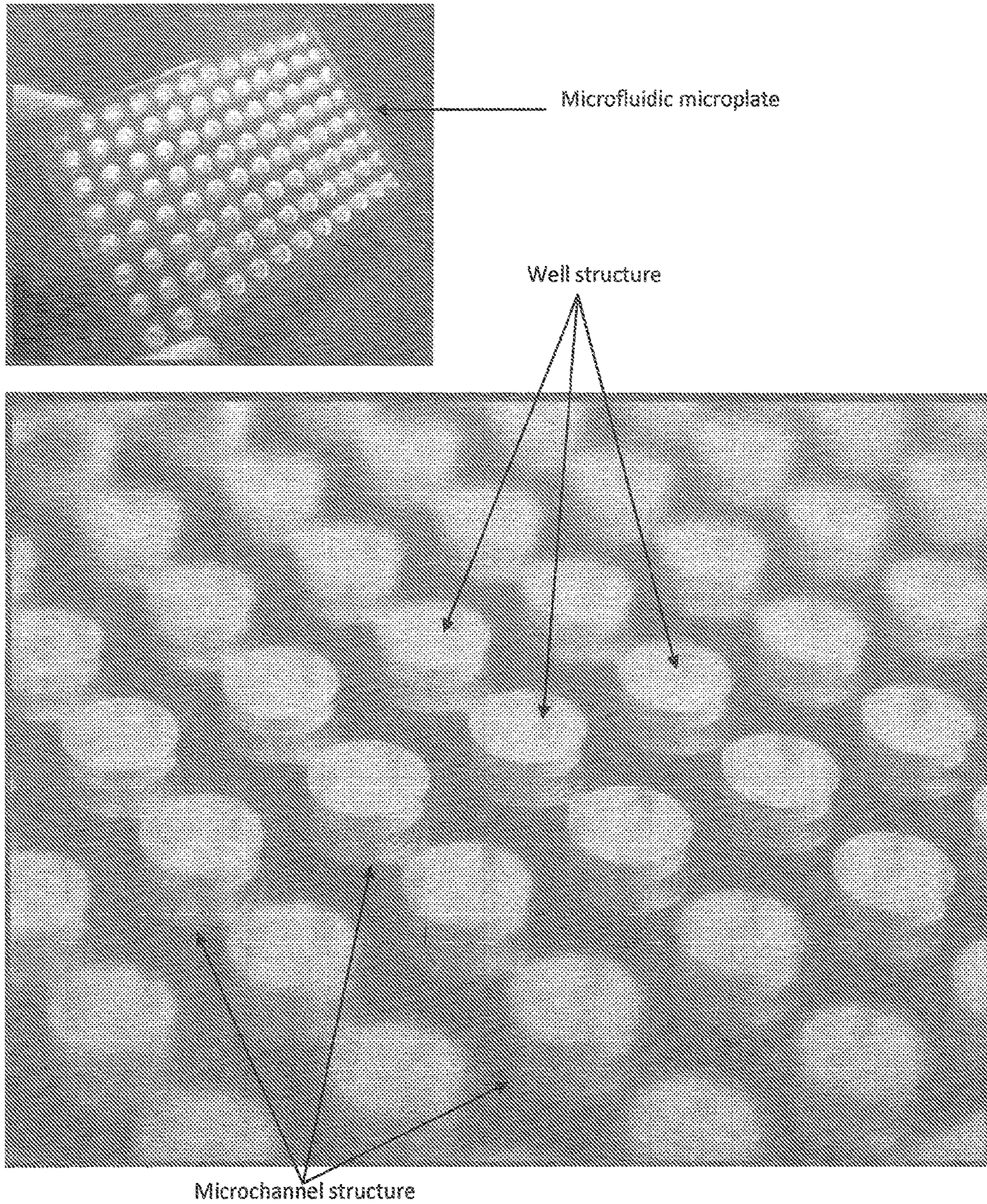
FIG 25. Microfluidic microplate. Note sealing tape and absorbent pad are not shown for clarity.
