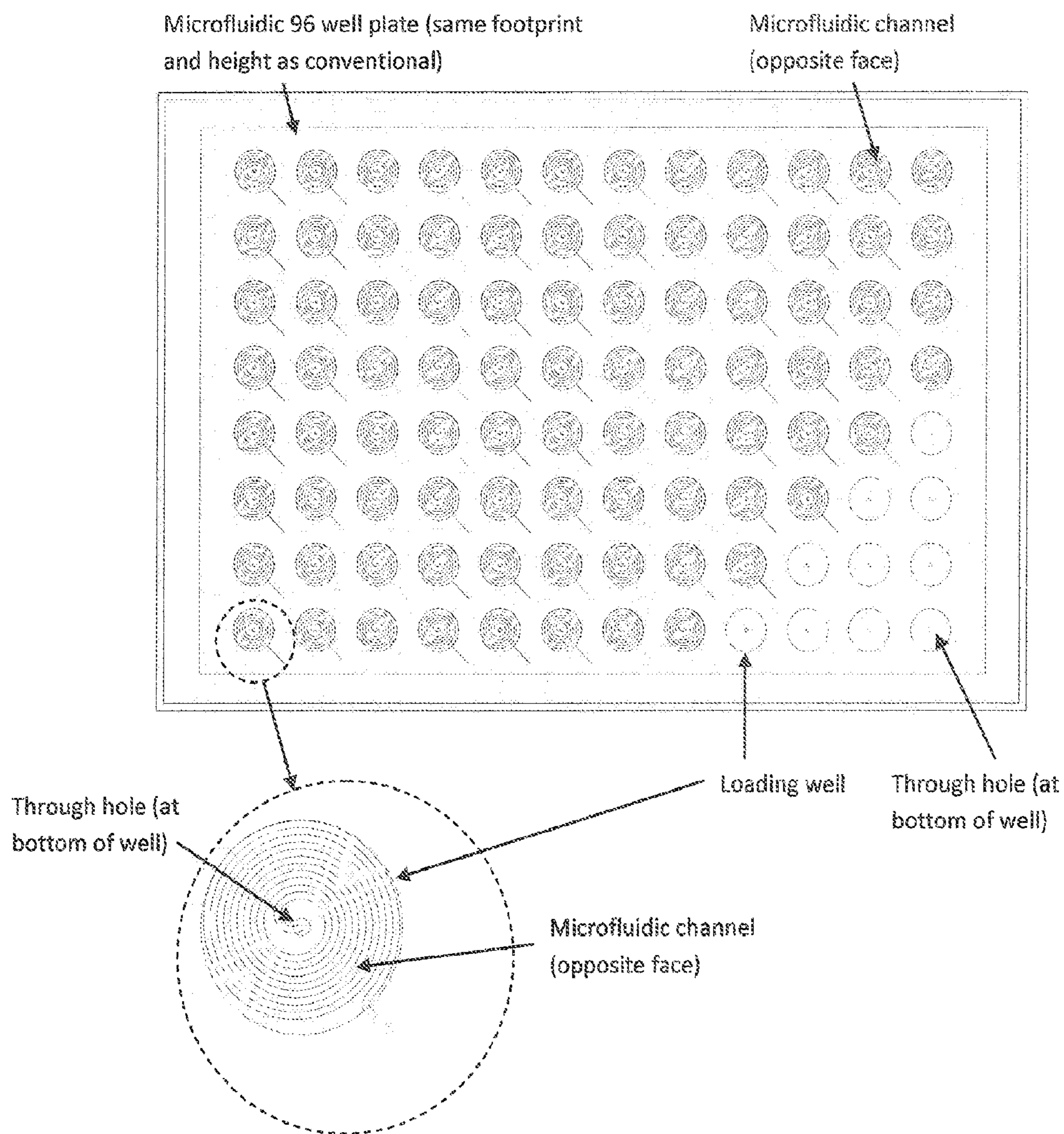
FIG 1. Microfluidic 96 well plate concept. The plate matches the dimensions of conventional microplates (as defined by accepted ANSI standards). The positions of the wells also matches ANSI standards. Each well is connected to a microchannel on the opposing face of the substrate. Figure does not show sealing layer (for microchannels) and absorbent pad for clarity. Also, selected wells in lower right hand corner of top figure do not show microchannel pattern for ease of explanation.
