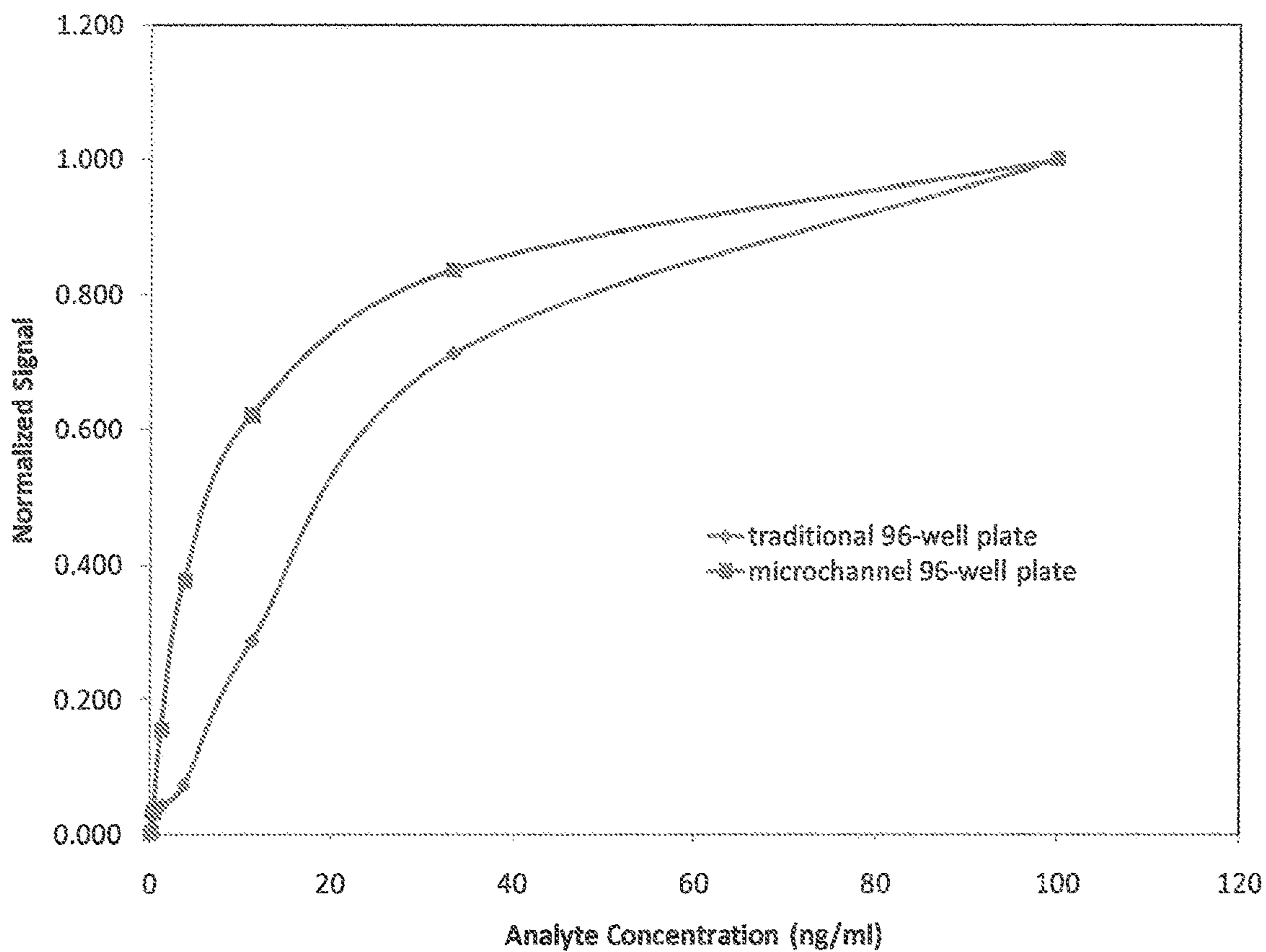
FIG 28. Test results comparing the performance of a conventional (traditional 96-well plate) 96 well plate with the microfluidic microplate of the present invention using chemiluminescence based detection. The Y-axis is normalized to facilitate comparison.
