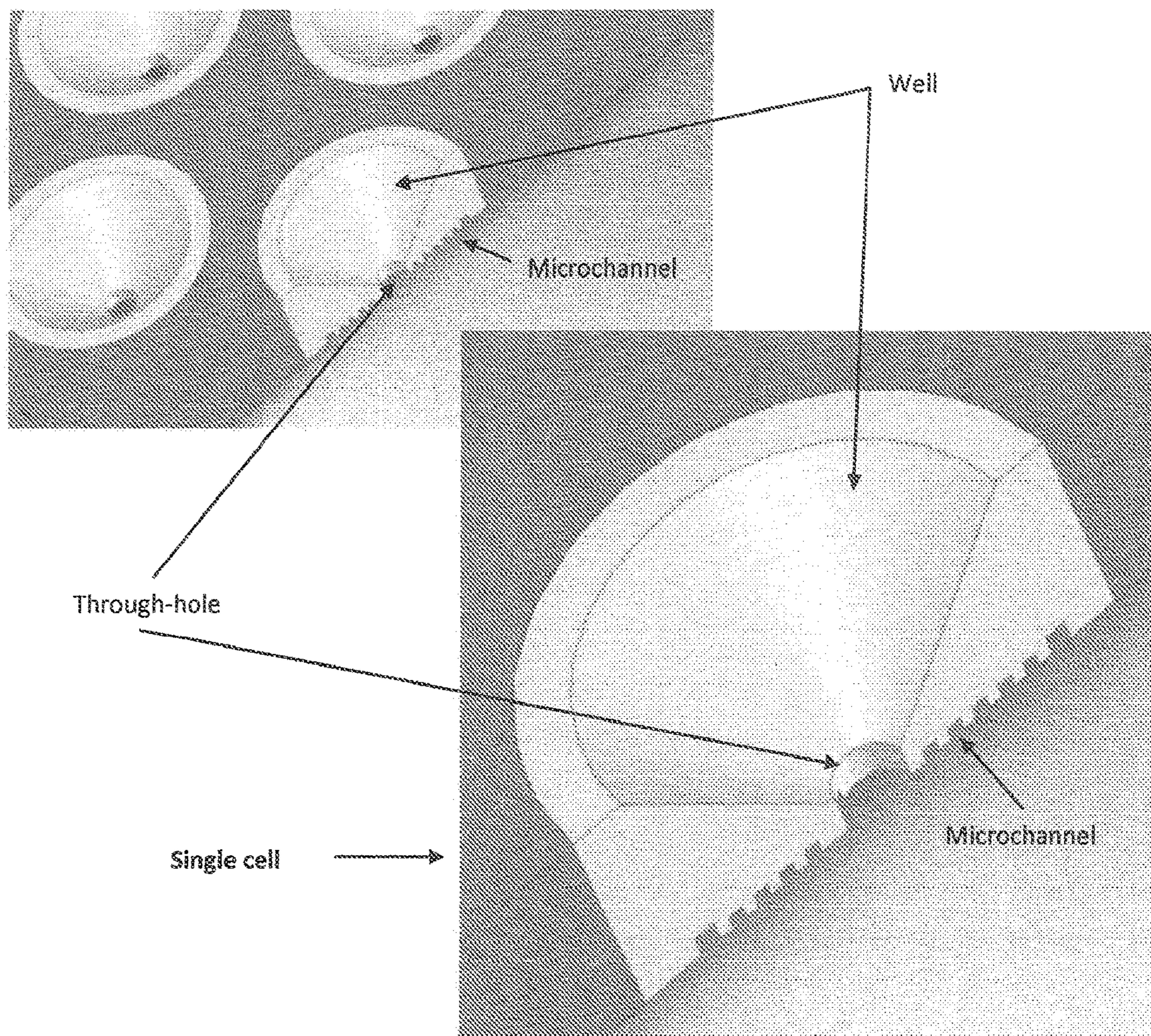
FIG 23. Embodiment particularly well suited for chemiluminescence based detection (note that only a partial view of the microfluidic microplate is shown in the above FIG to illustrate the concept clearly). In this embodiment, each cell (wherein a cell composes of one well with a through-hole connecting to a single microchannel) is physically isolated from the adjoining cells by a substantially opaque substrate. The “microfluidic substrate” is in actuality an array of physically distinct substrates.
