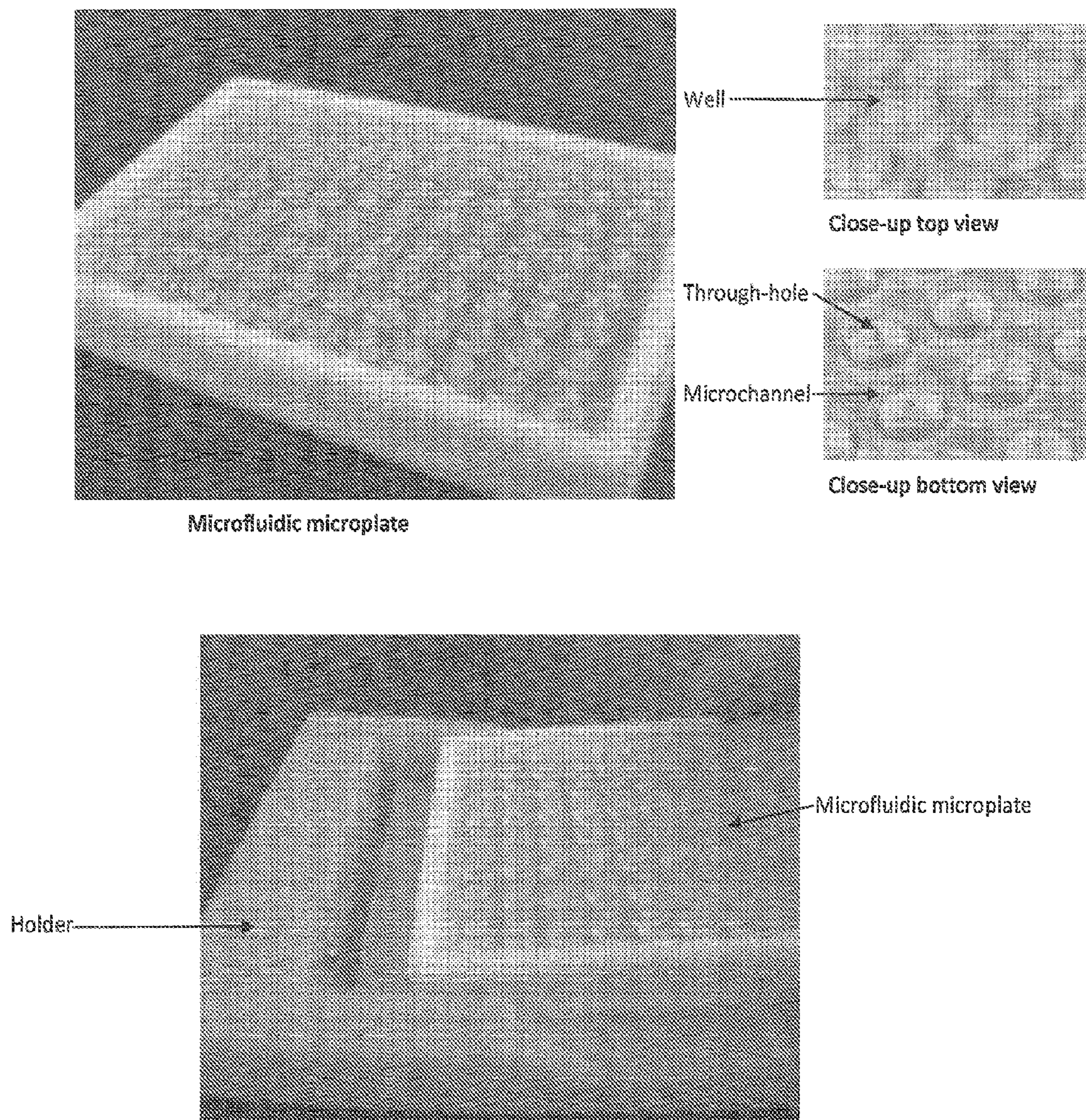
FIG 26. Alternate embodiment of the Microfluidic microplate of the invention. Note sealing tape and absorbent pad are not shown for clarity. The image on the bottom shows the microfluidic microplate being positioned in a holder for liquid handling steps -- in actual operation; the holder would also house the absorbent pad in the embodiments wherein the pad is a disposable element.
