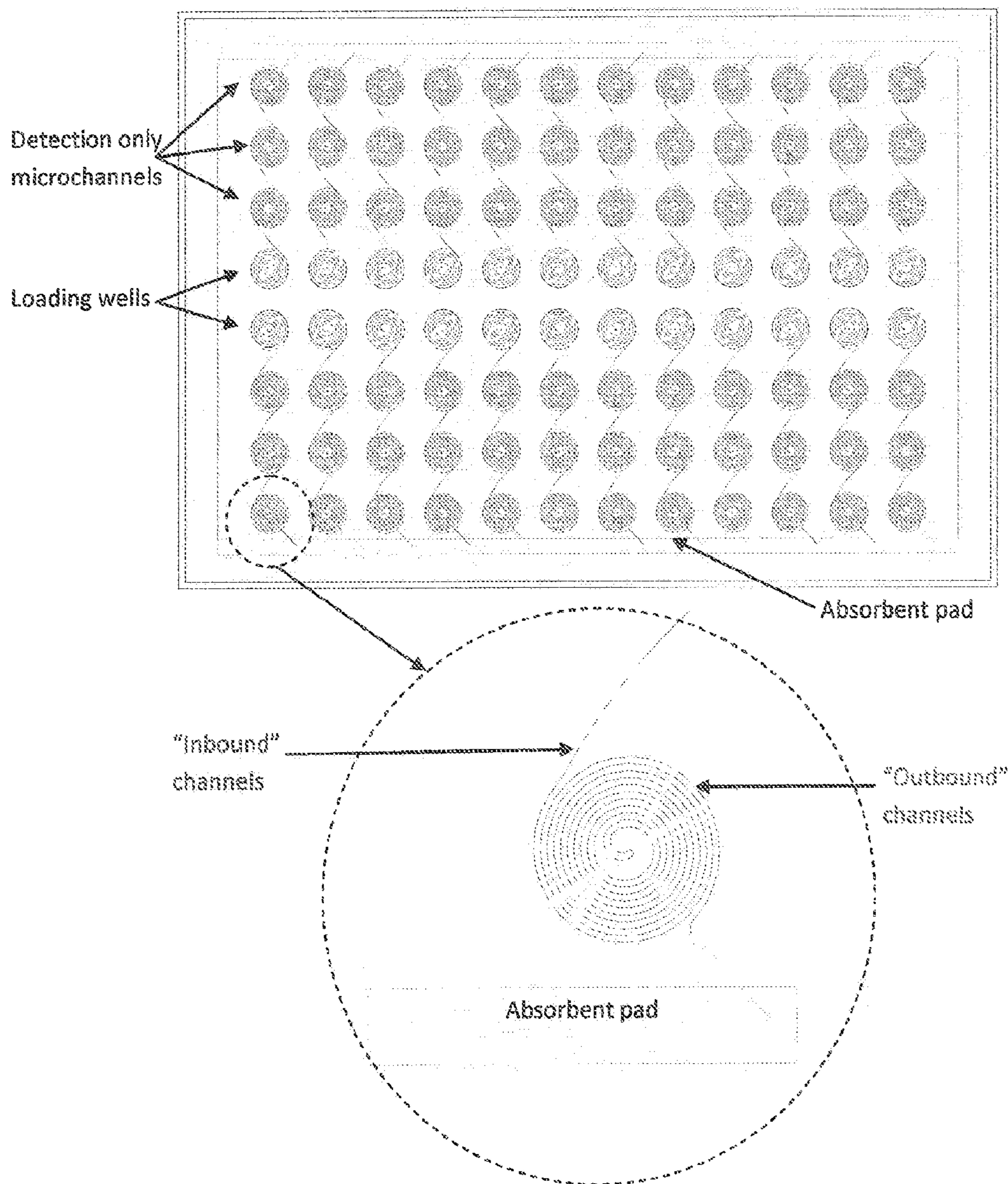
FIG 21A. In this configuration, one loading well is connected to a microchannel path on the opposing surface and is additionally connected to other microchannel sections not directly underneath the loading well. When a liquid is loaded into the well, it will flow through all the microchannel sections (4 sections in fig above) connected in series. In the Figure shown above, a total of 24 distinct loading wells connect to a total of 4 reaction chambers each. The microchannel configuration may be modified to another embodiment to accommodate the series connection of the channel sections.
