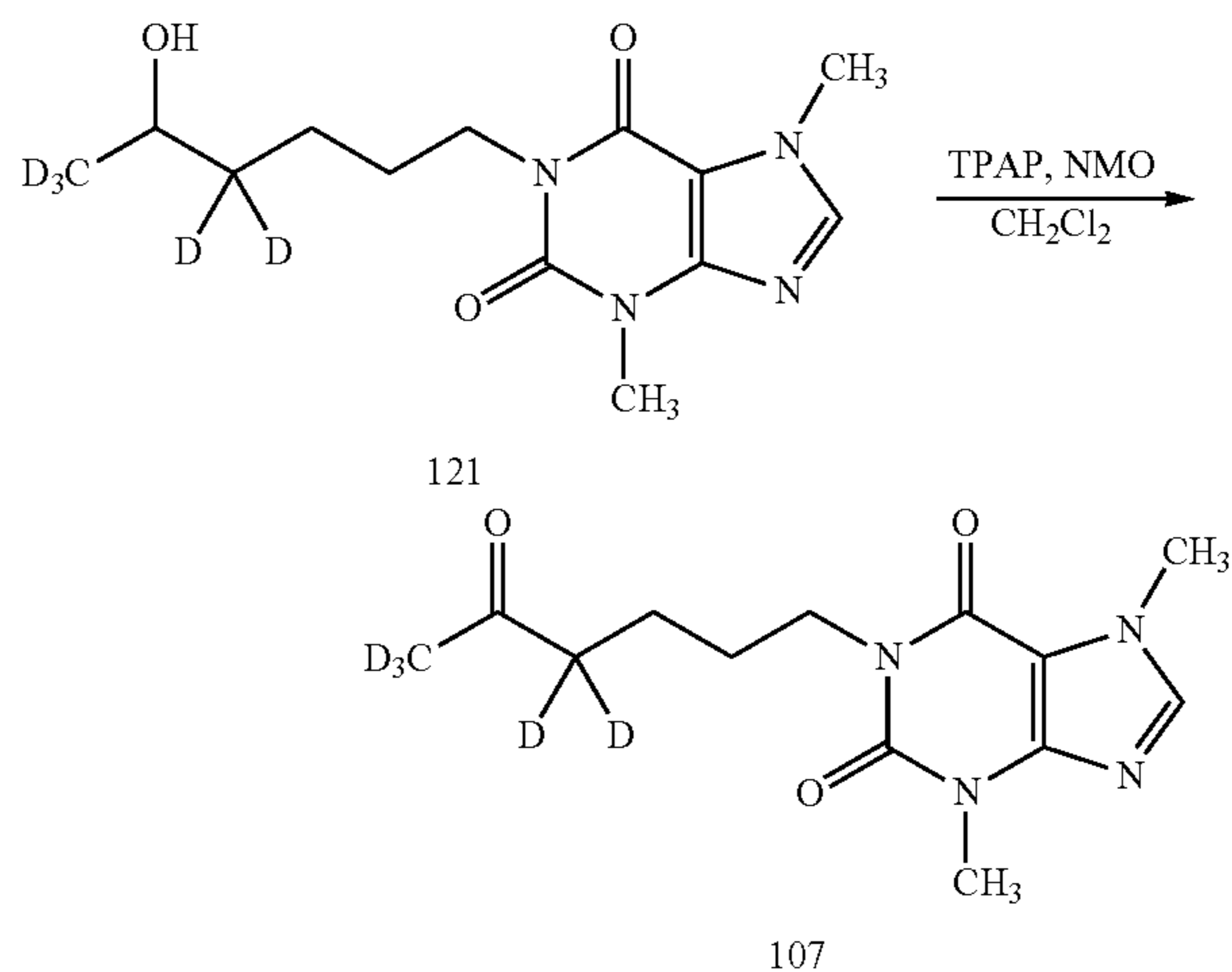
Scheme 25. Preparation of Compound 107.
