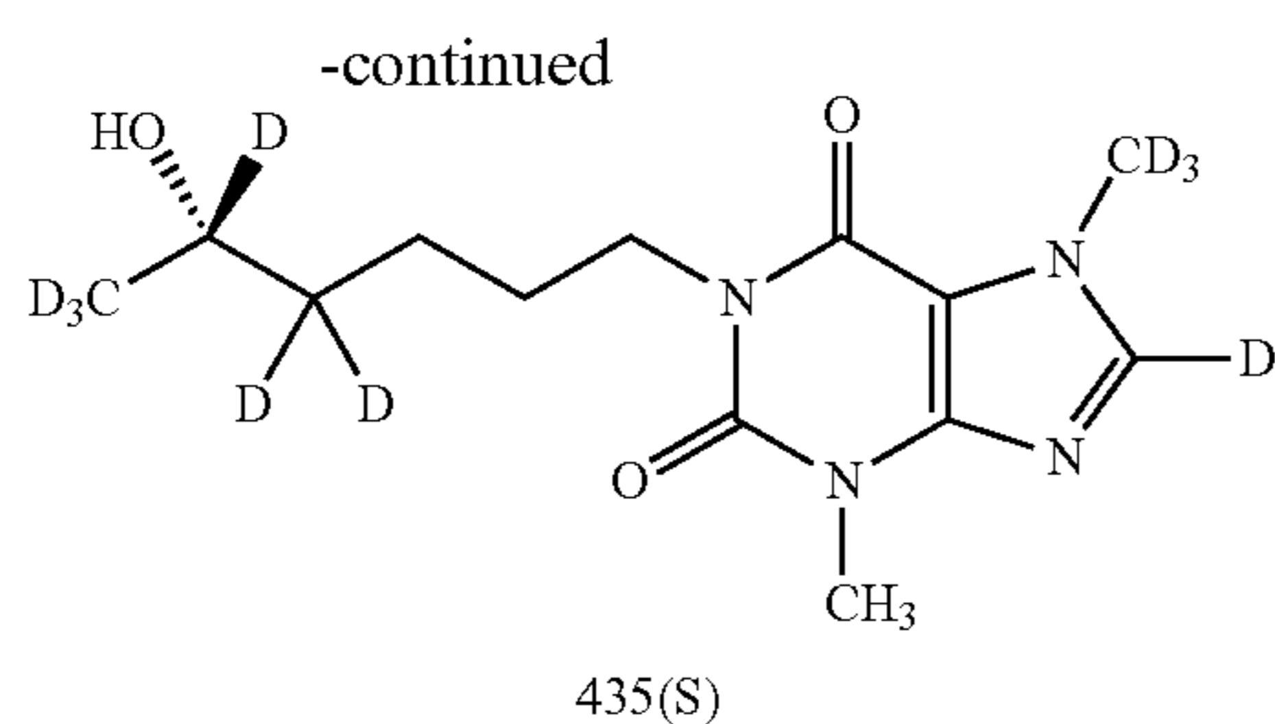
(±)8-d 1 -1-(4,4,5,6,6,6-d 6 -5-Hydroxyhexyl)-3-methyl-7-(methyl-d 3 )-1H-purine-2,6(3H,7H)-dione (Compound 435)
