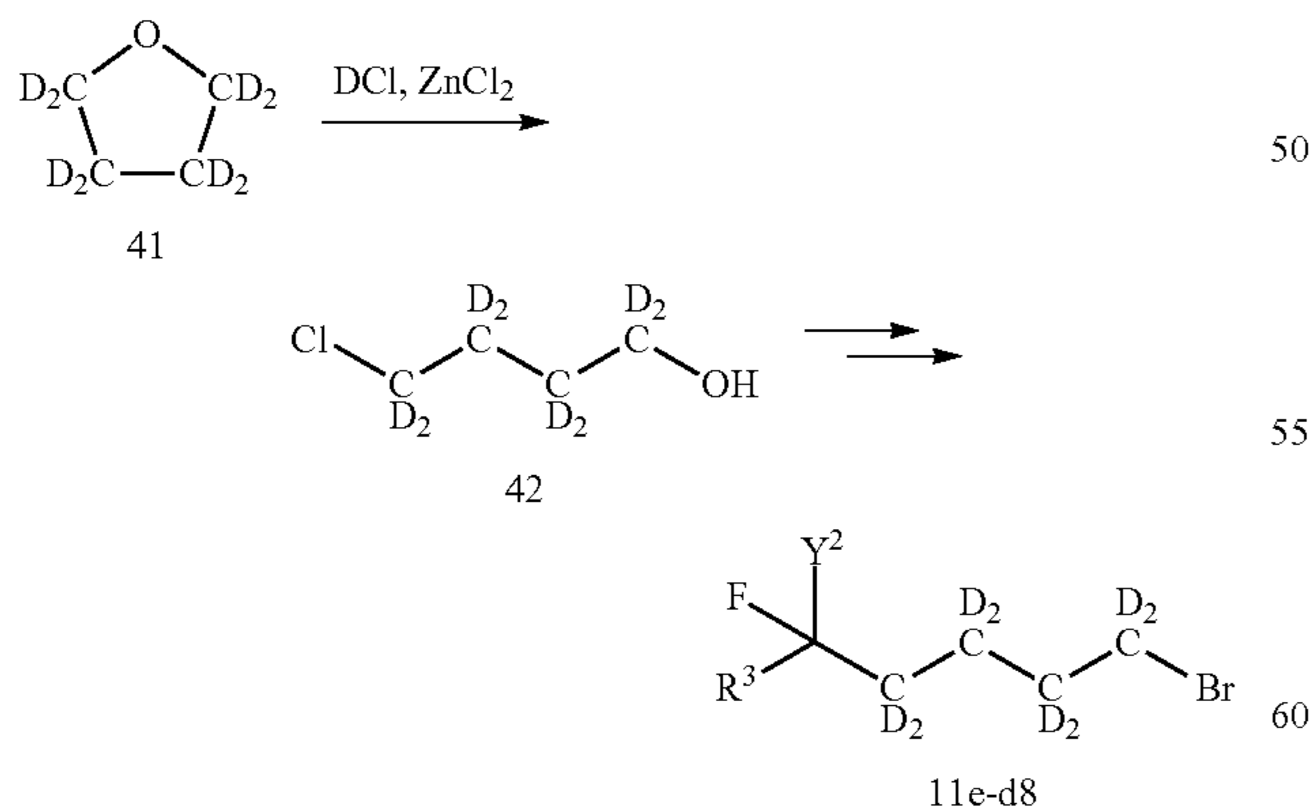
Scheme 8. Synthesis of Intermediates 11e-d 8 (X=Br)
