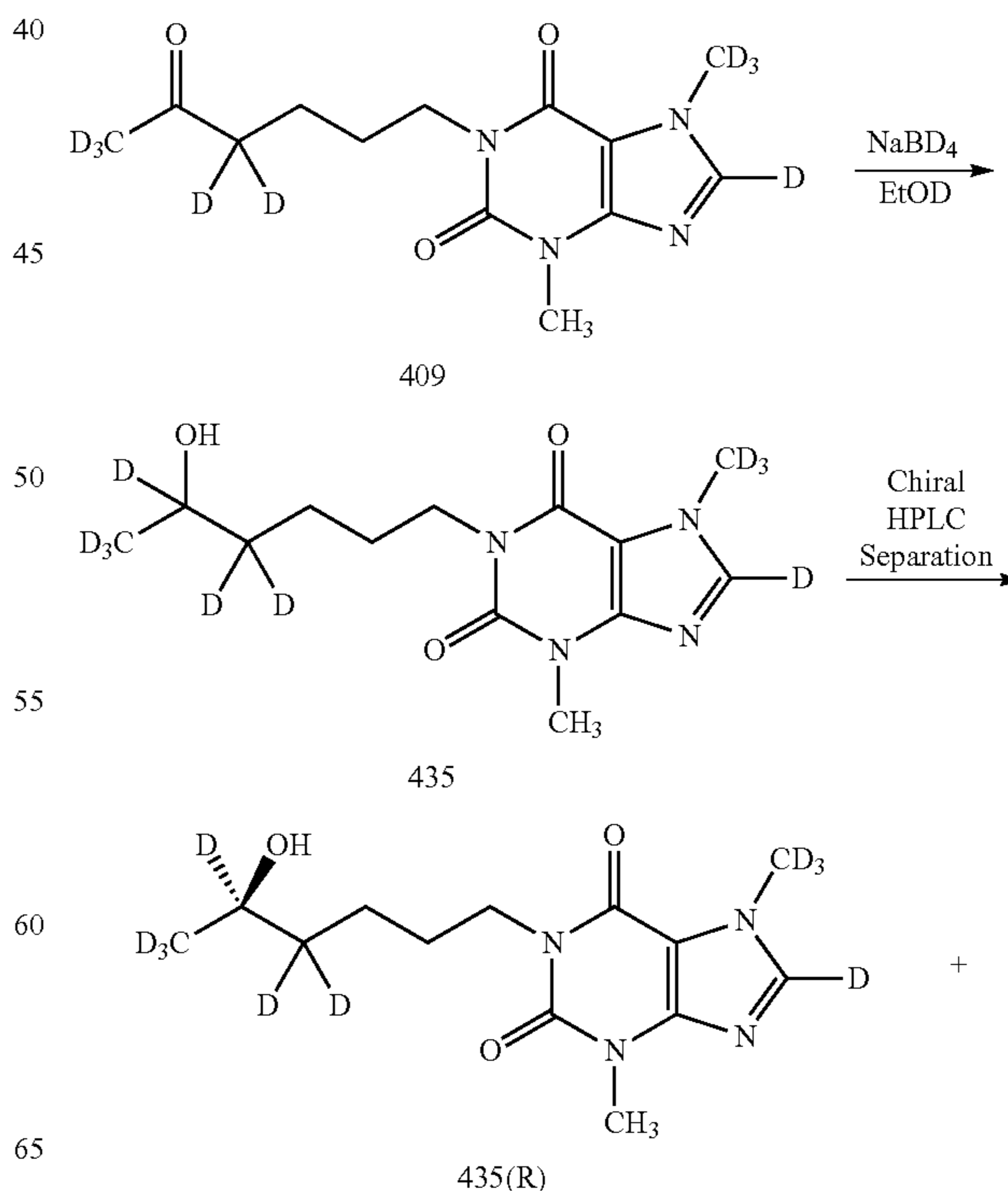
Scheme 17. Preparation of Compounds 435, 435(R), and 435(S).
