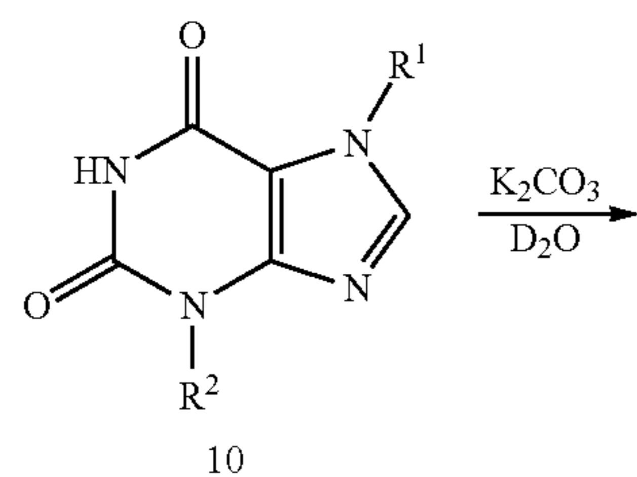
Scheme 12. Alternative Synthesis of Compounds of Formula A1
