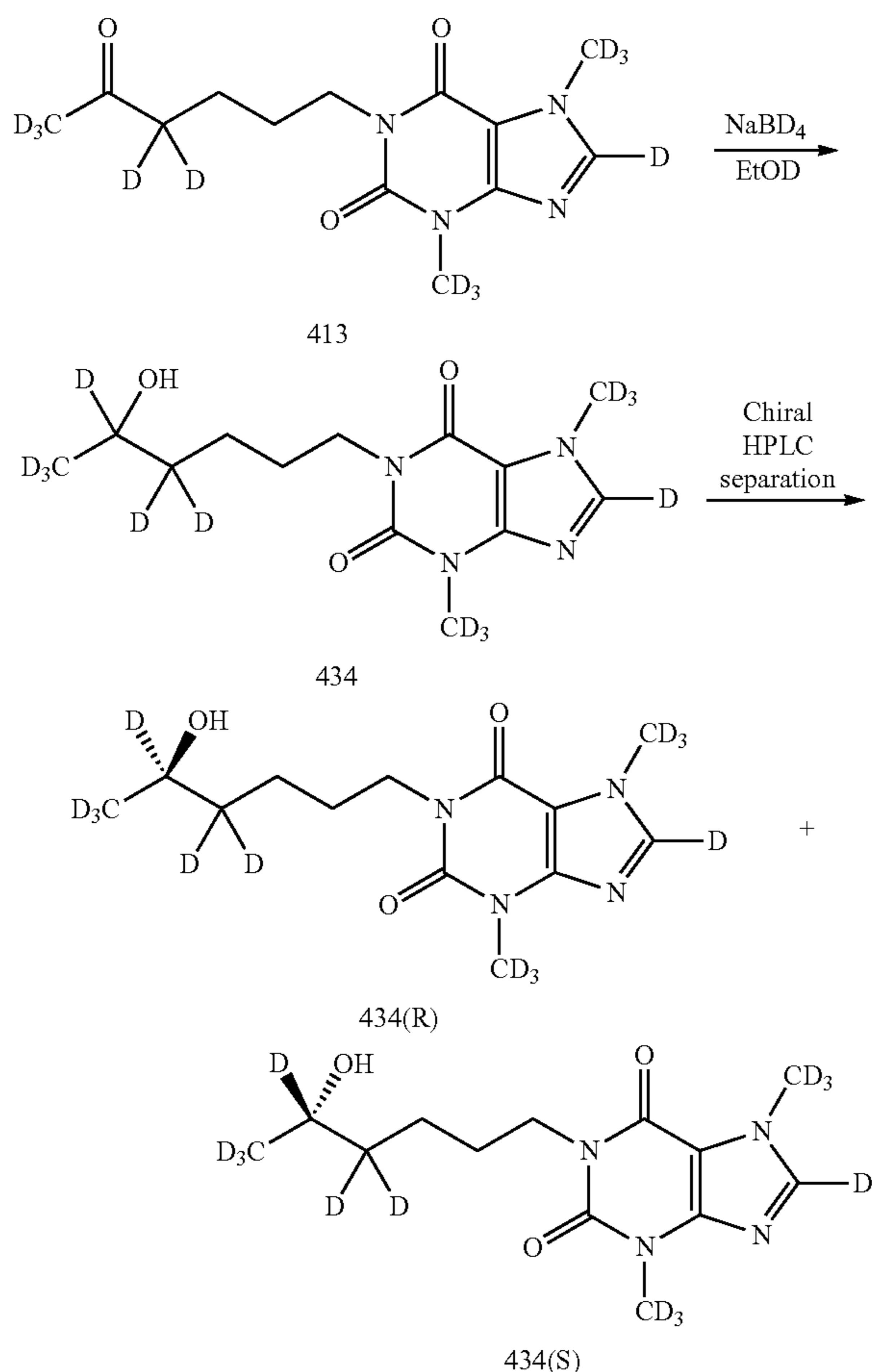
Scheme 26. Preparation of Compounds 434, 434(R) and 434(S).
