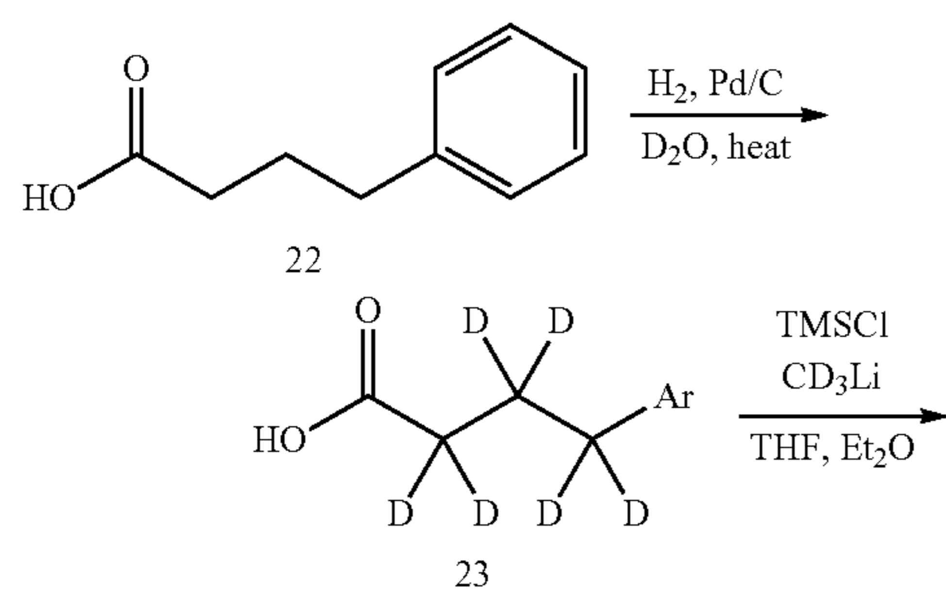
Scheme 4. Synthesis of Intermediates 11A-d 9 and 11a-d 11
