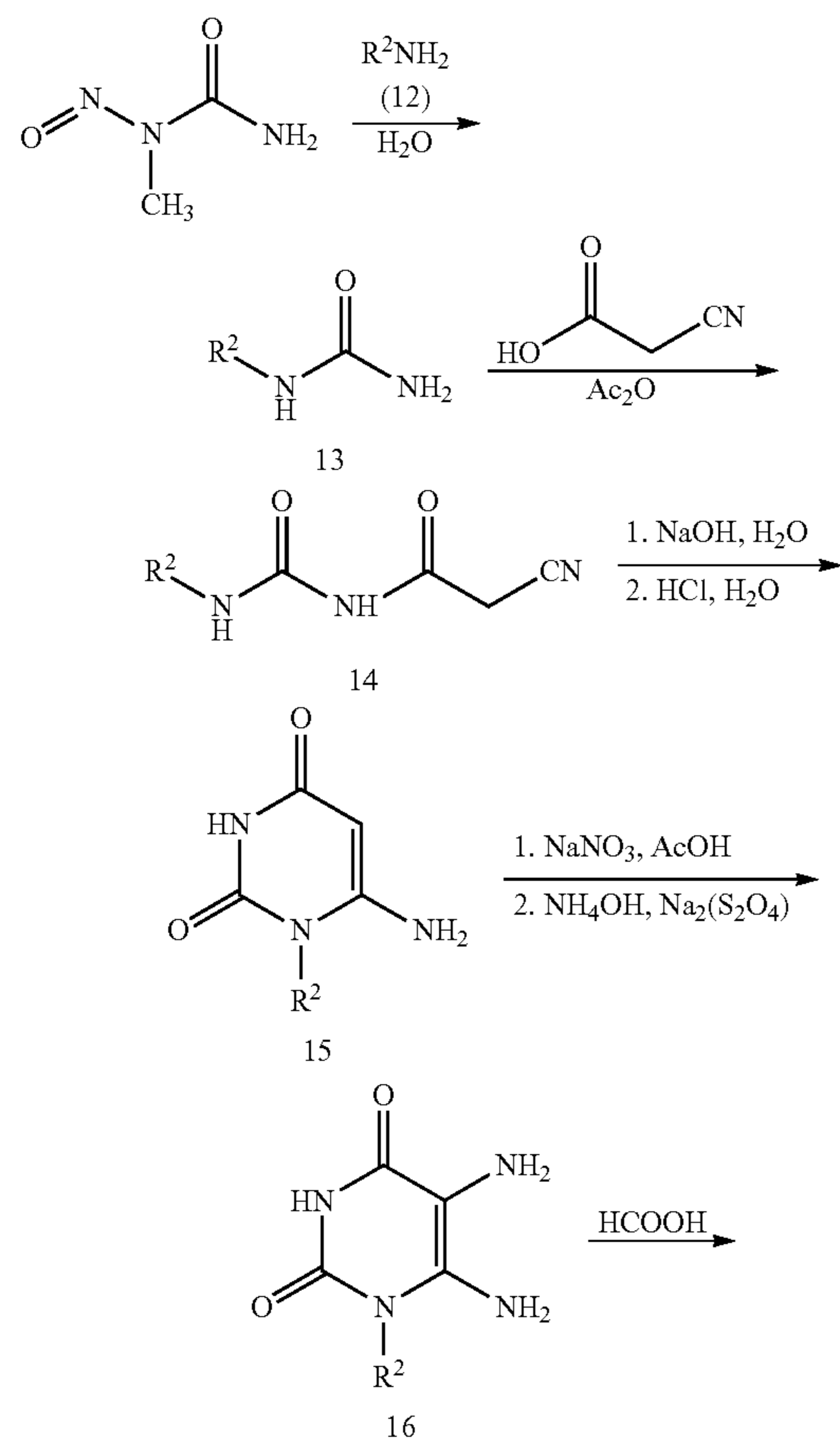
Scheme 2. Synthesis of Compound 10
