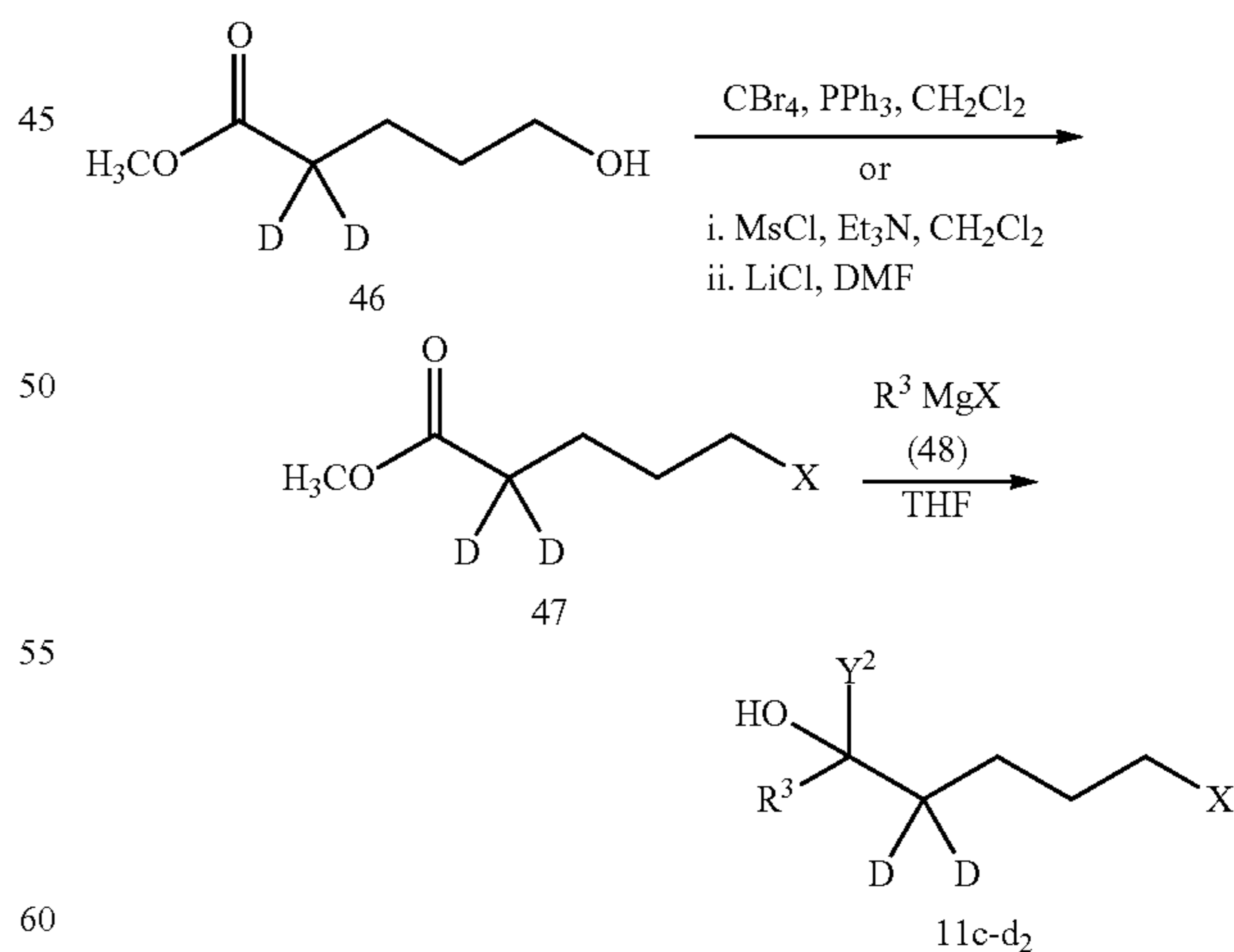
Scheme 10. Synthesis of Intermediates 11c-d 2 .
