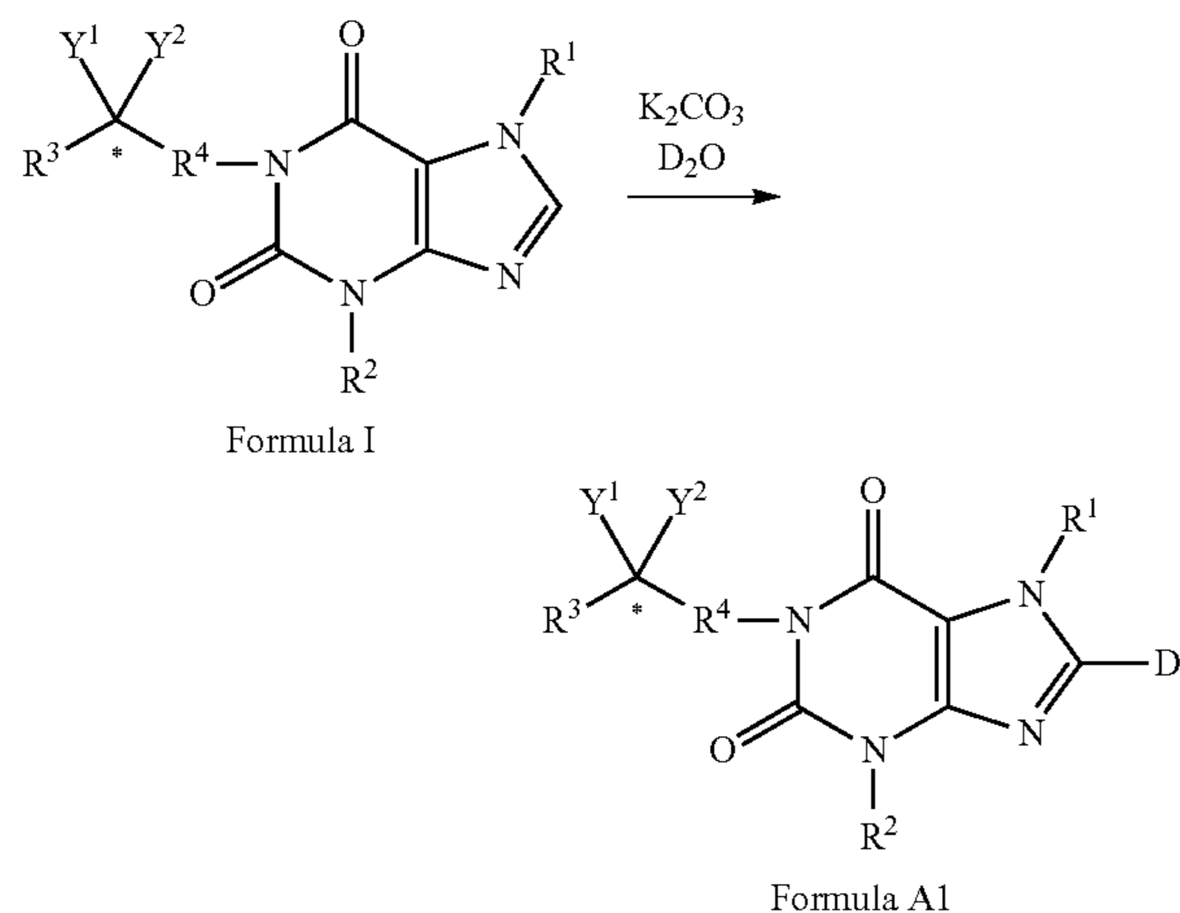
Scheme 11. Synthesis of Compounds of Formula A1
