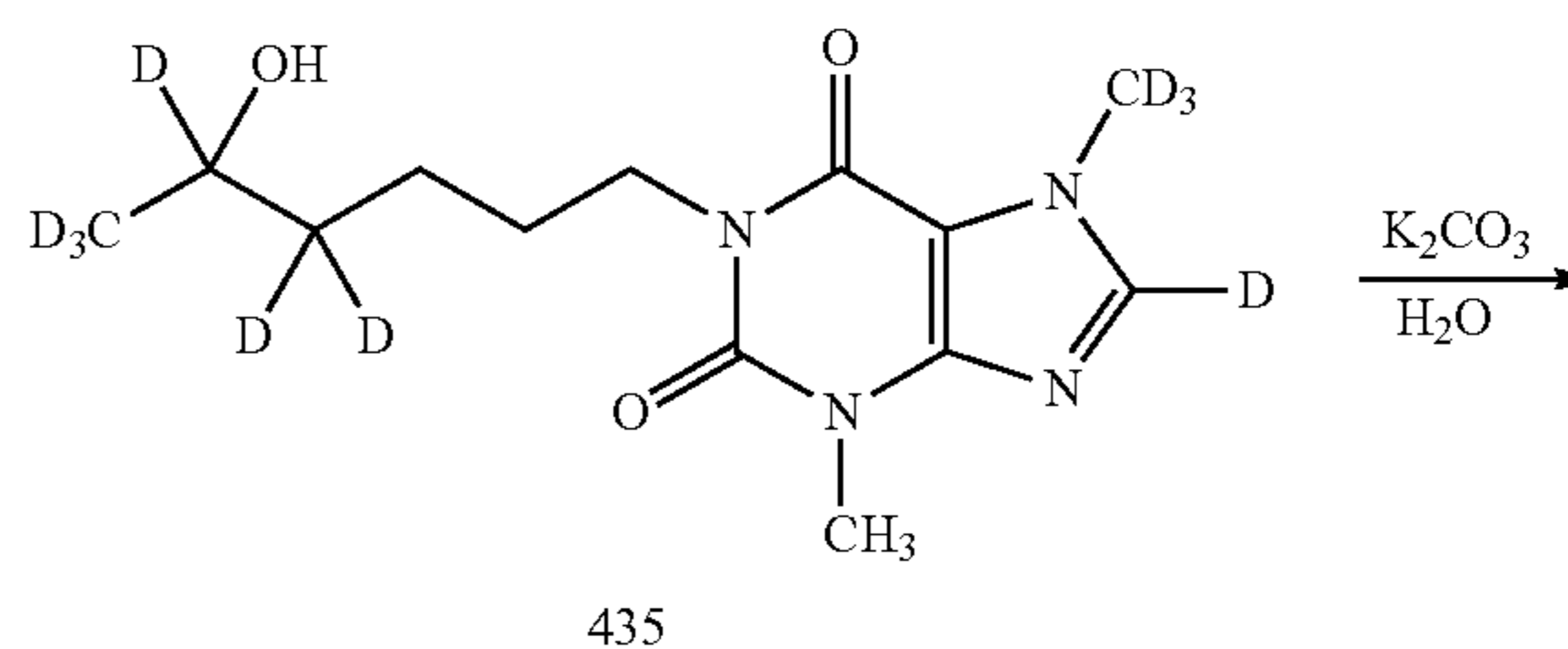
Scheme 27. Preparation of Compounds 135, 135(R) and 135(S).
