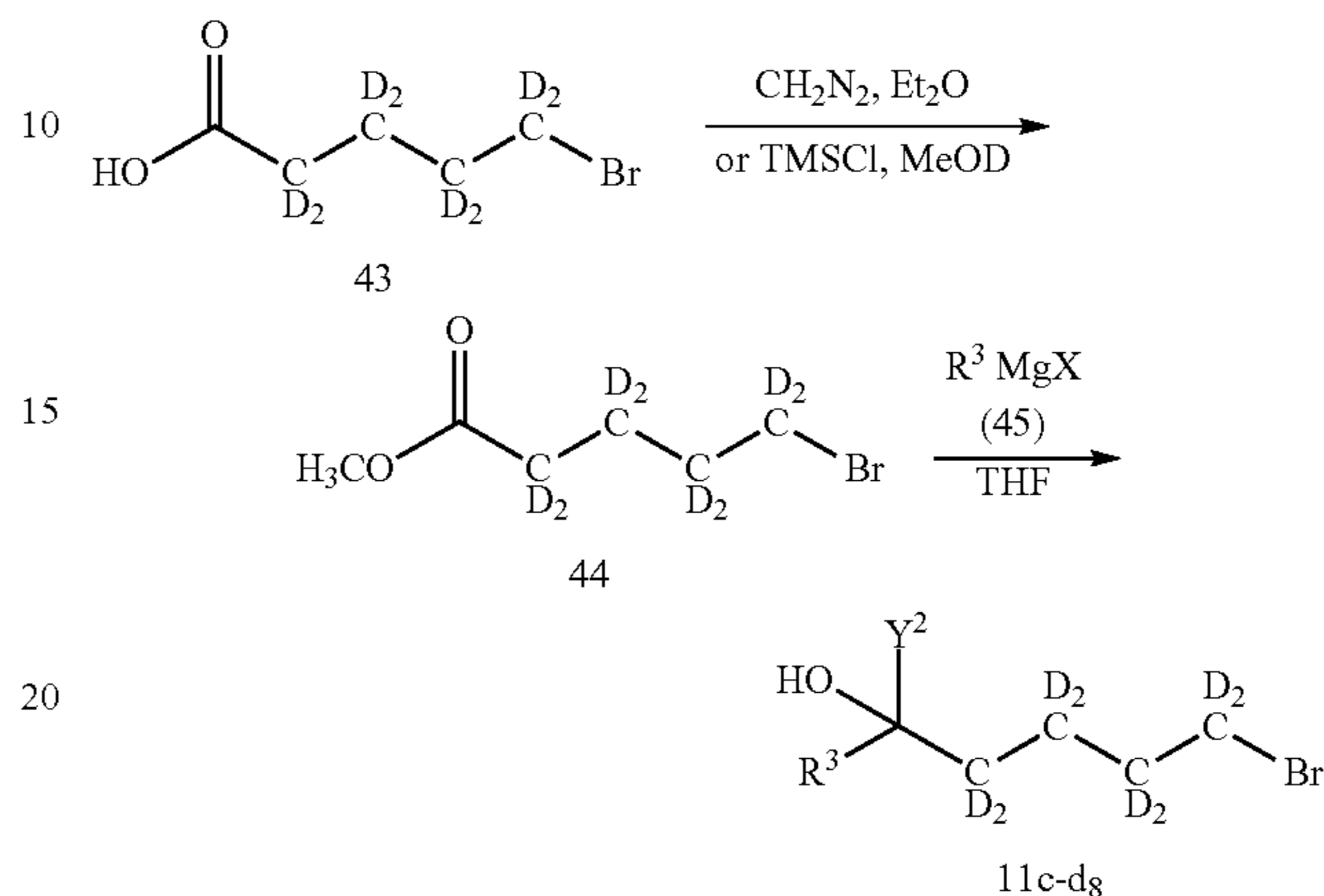
Scheme 9. Synthesis of Intermediates 11c-d 8 (X=Br)
