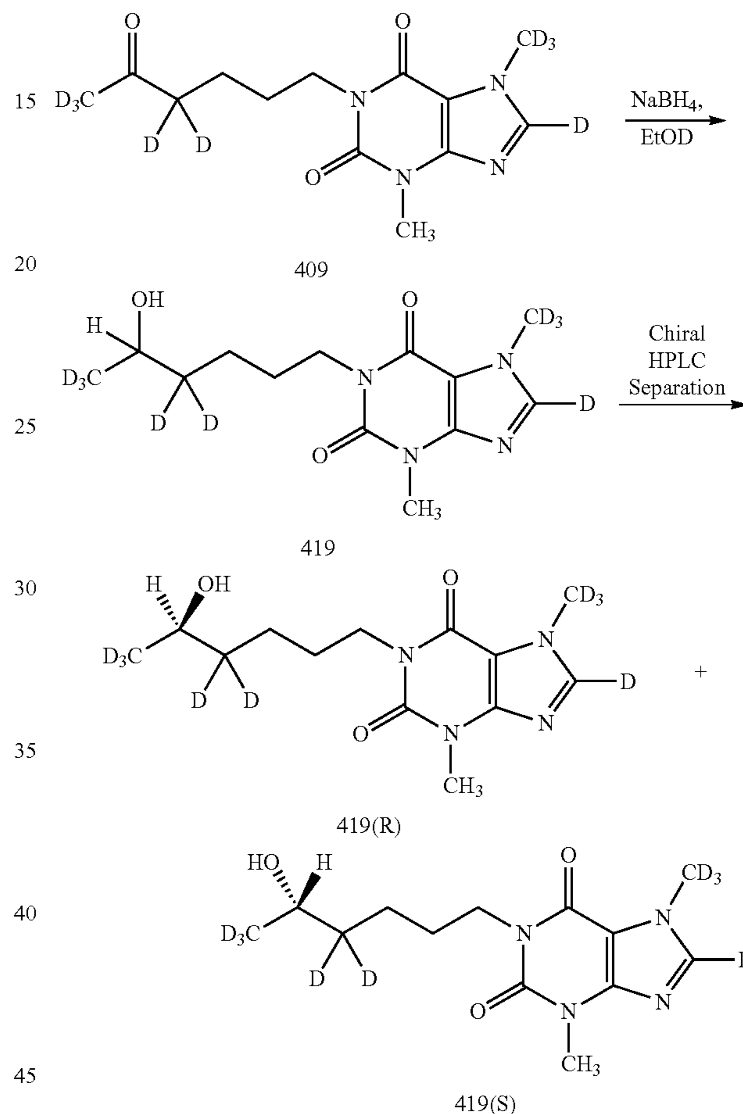
Scheme 16. Preparation of Compounds 419, 419(R), and 419(S).
