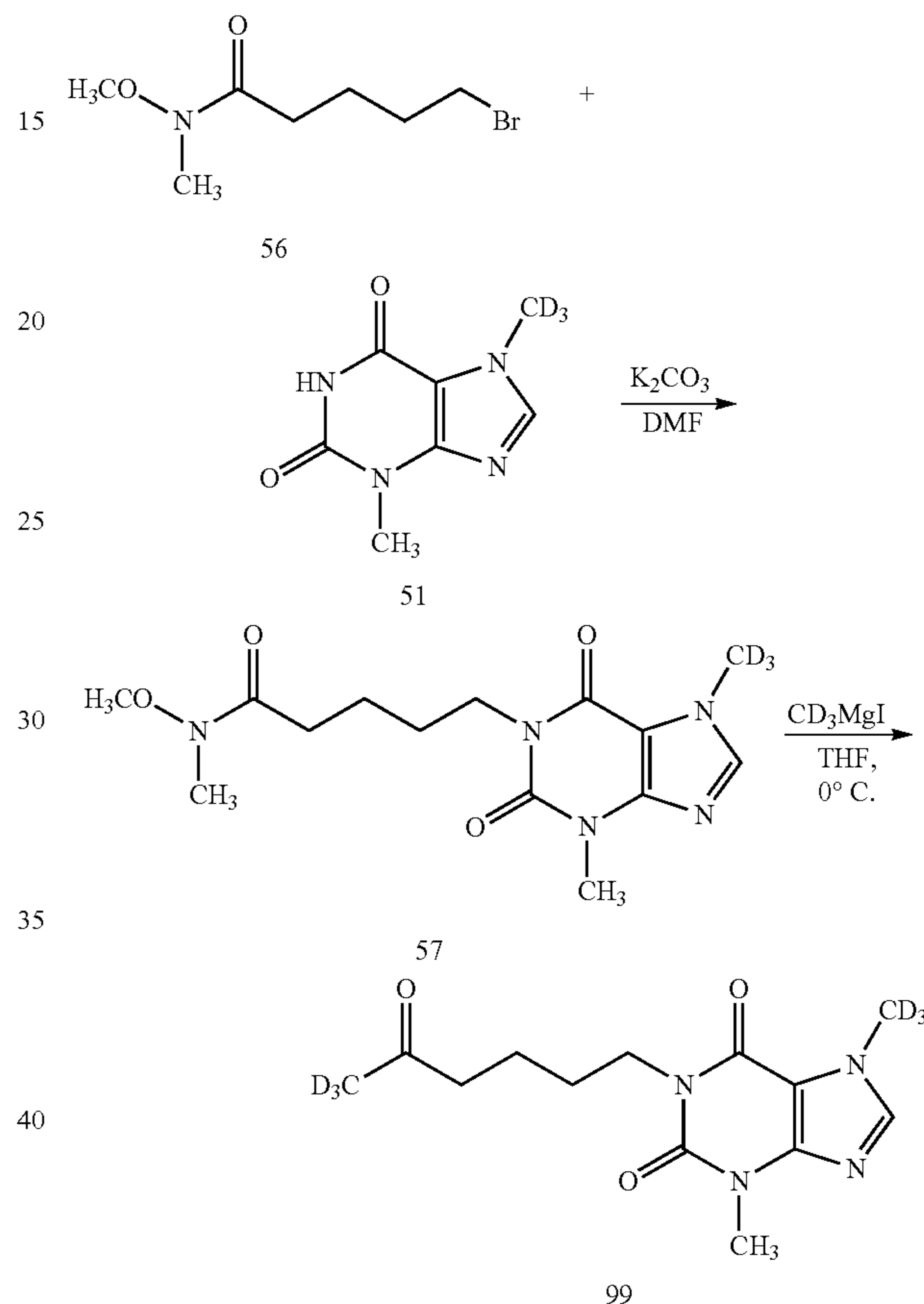
Scheme 15. Preparation of Compound 99.
