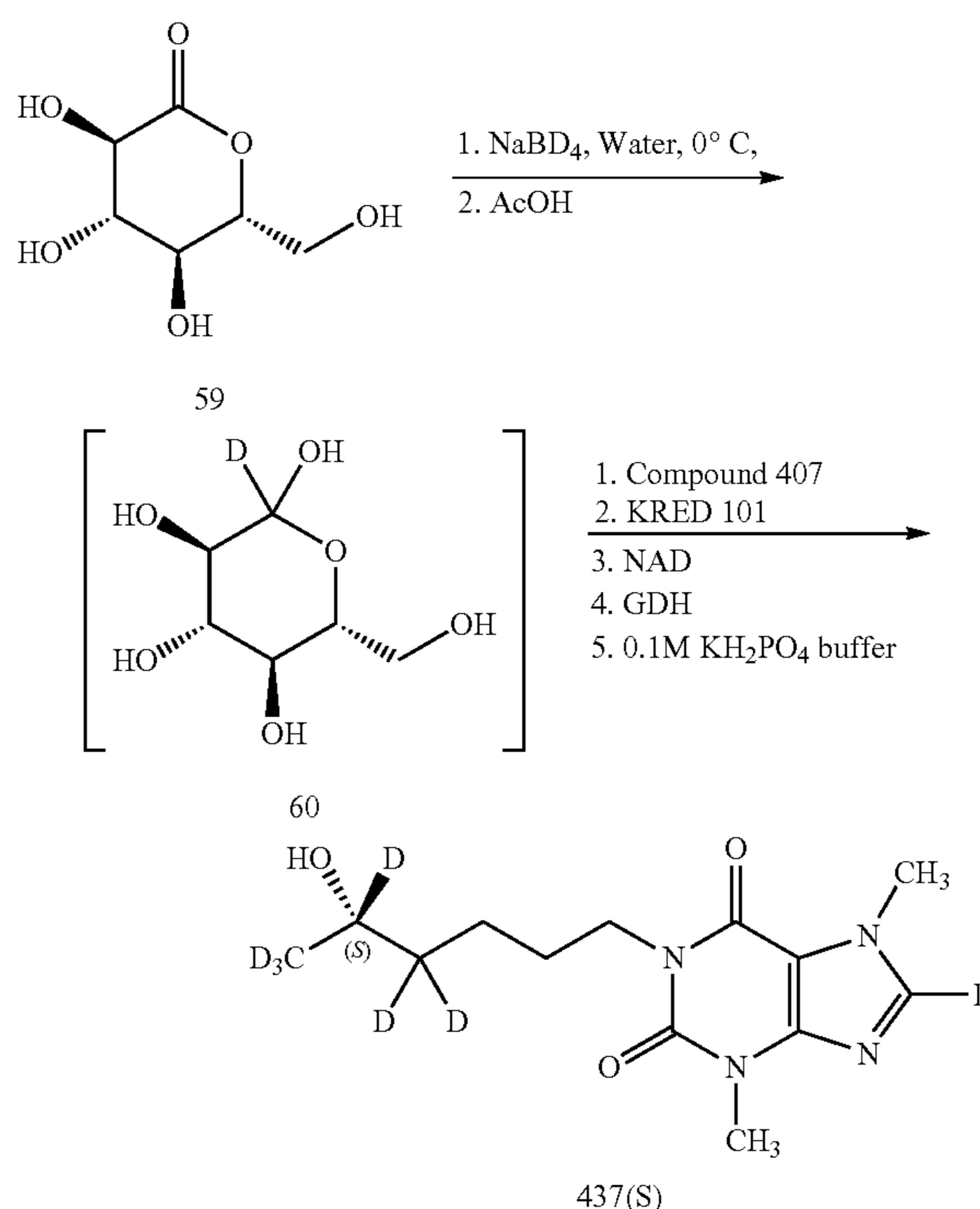
Scheme 19. Preparation of Compound 437(S).
