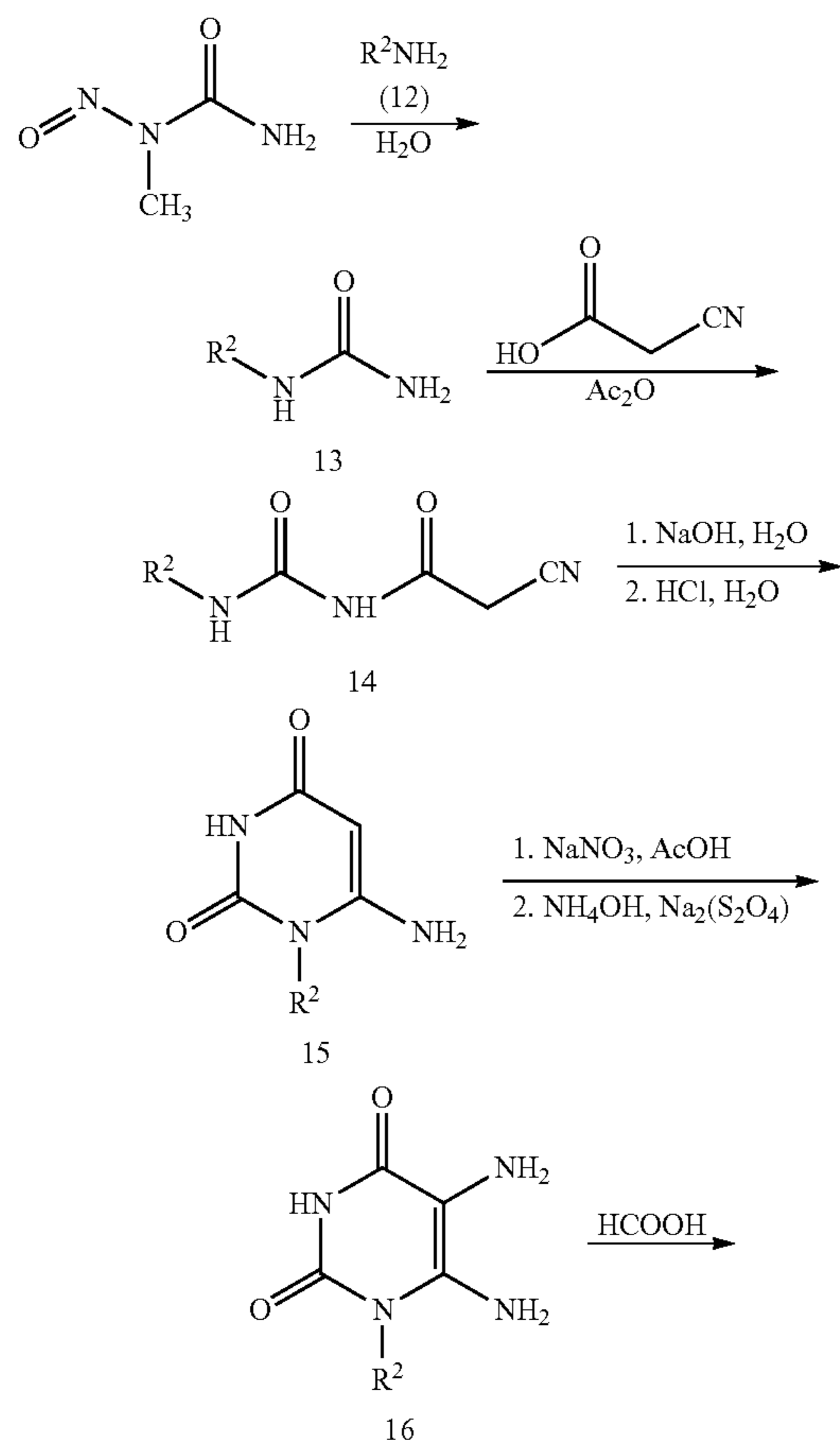
Scheme 2. Synthesis of Compound 10
