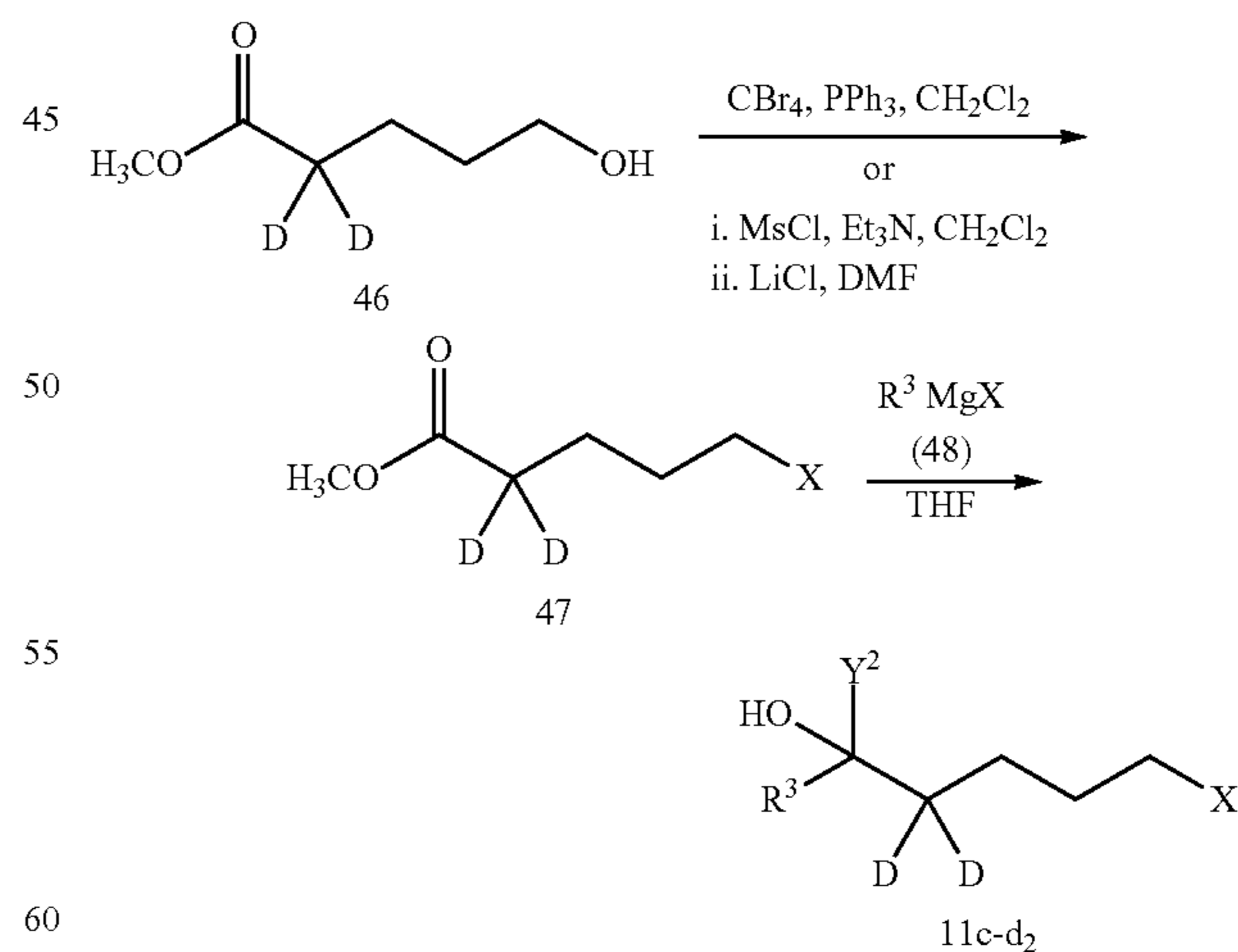
Scheme 10. Synthesis of Intermediates 11c-d 2 .
