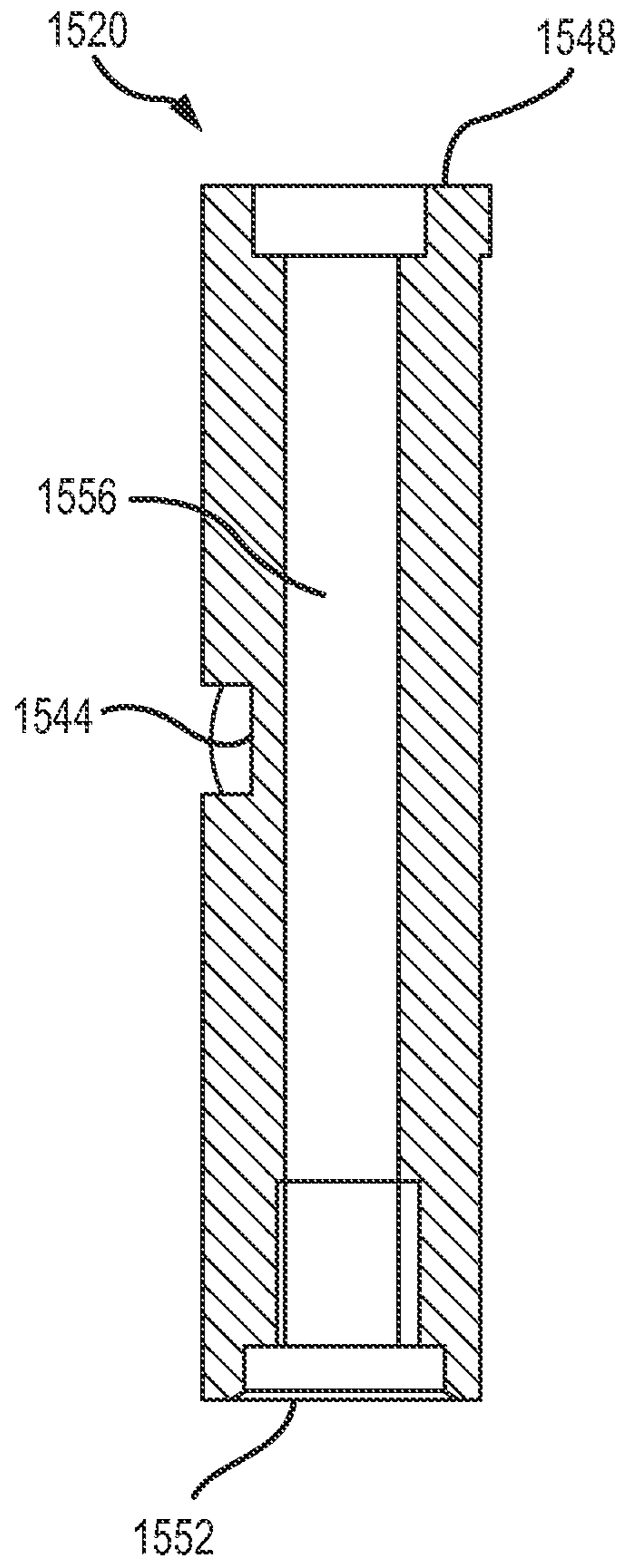
SECTION F-F
