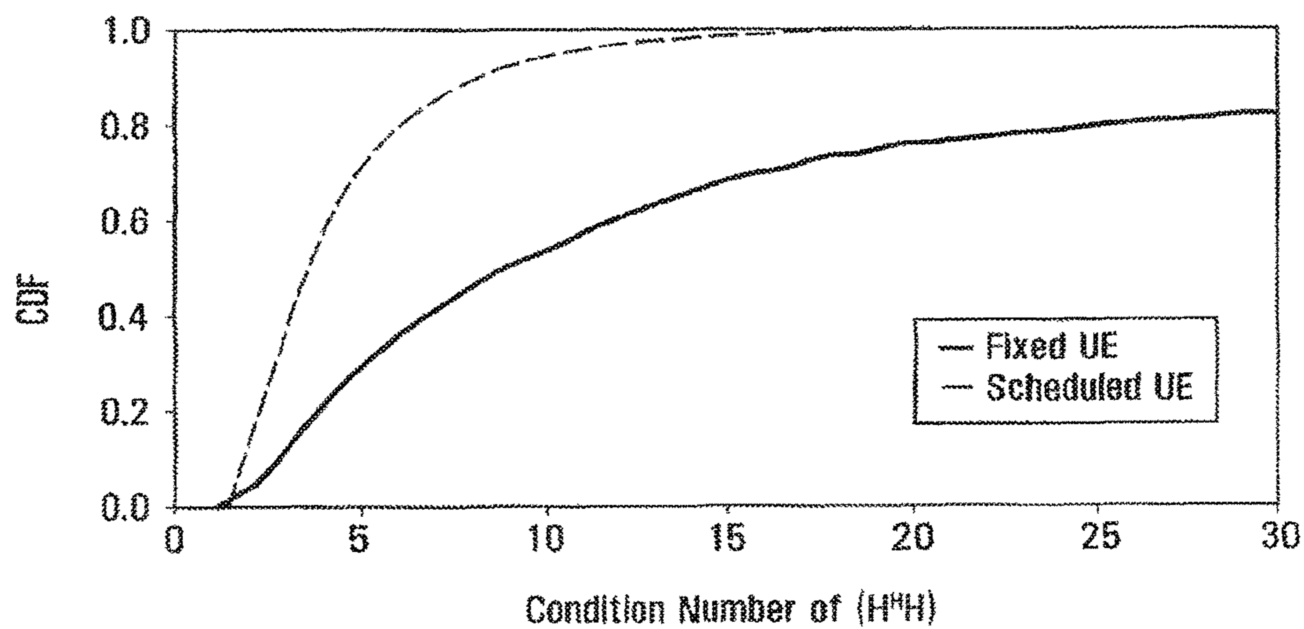
Minimum Conditional Number Scheduling (SM 2x2 MLD, 16 UEs, ITU-VA, Turbo R=1/2, 10MHz 1024-FFT, 2-Baud)
