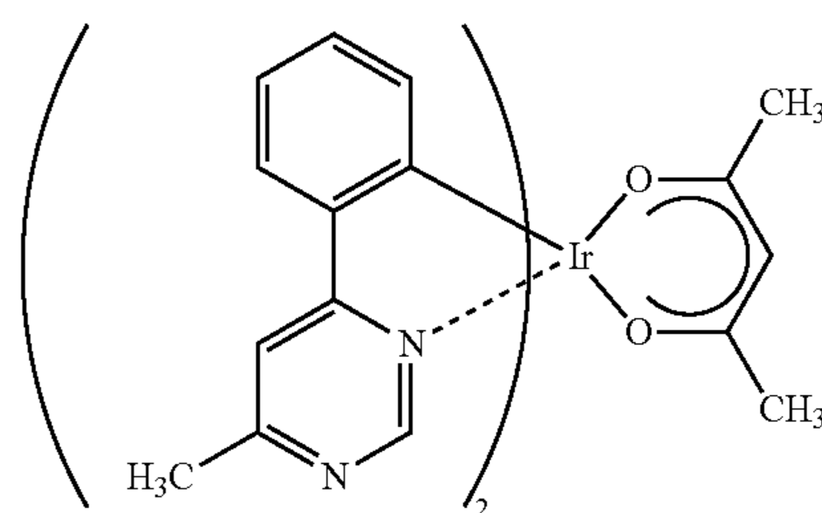
[\text{Ir}(\text{mppm})_2(\text{acac})]
