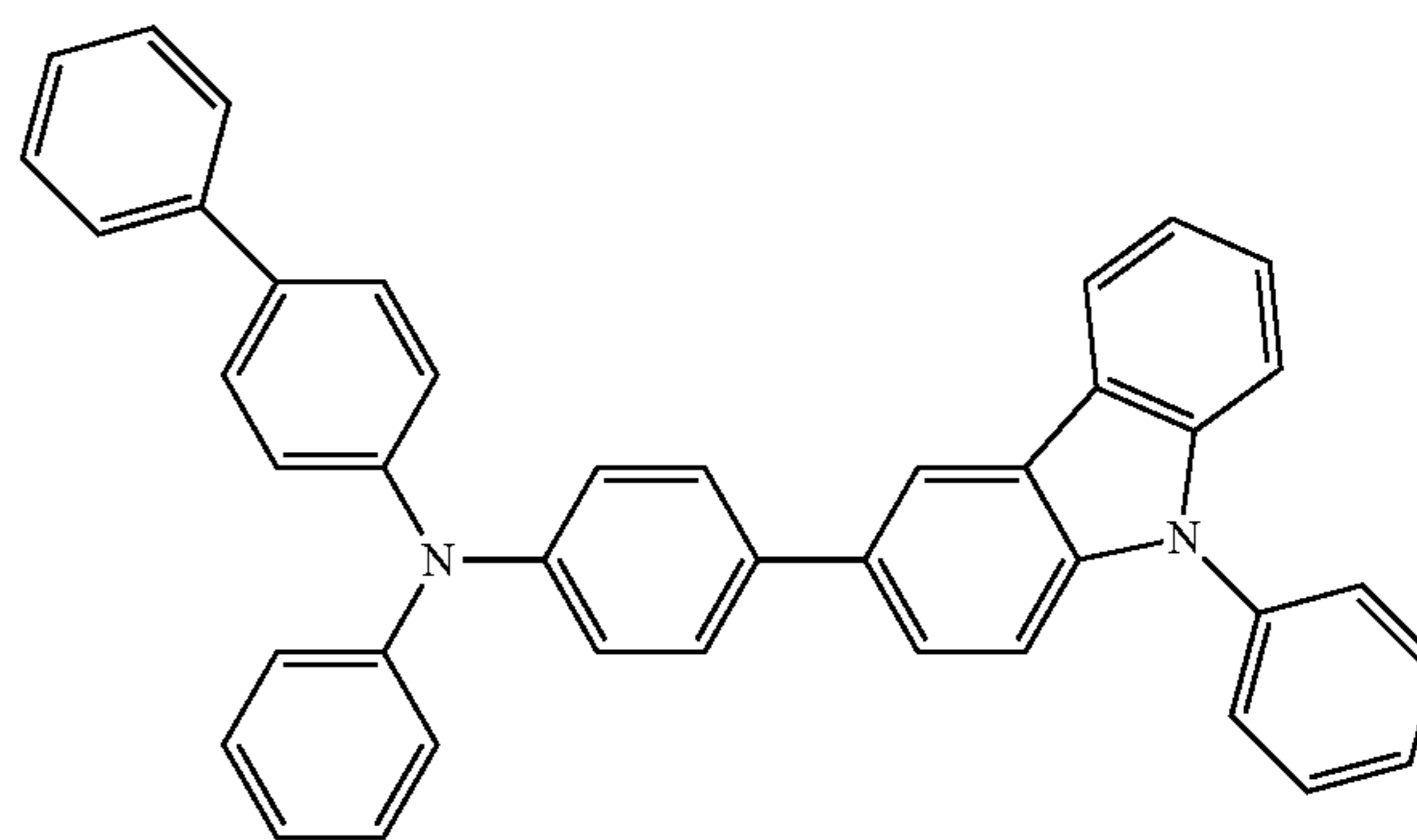
PCBA1BP
