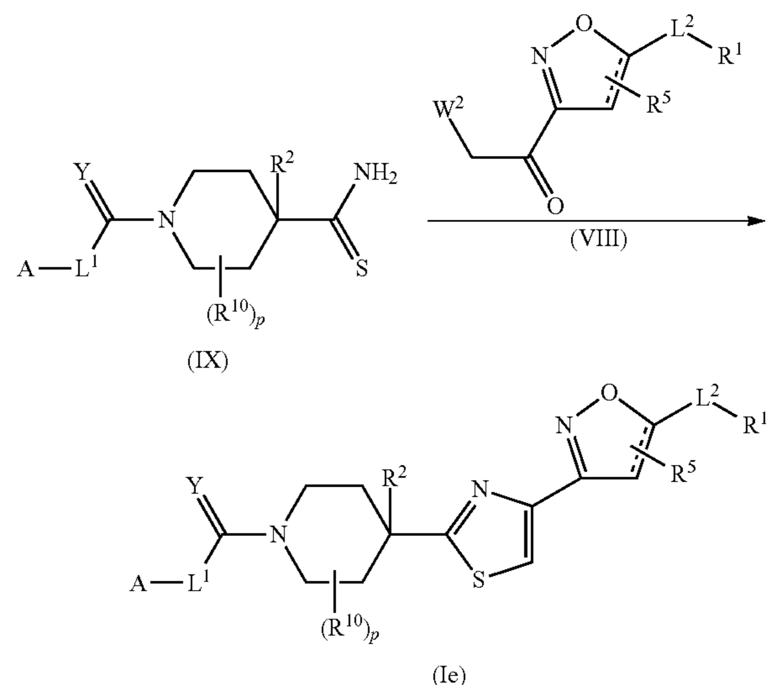
Scheme 5: Process E
