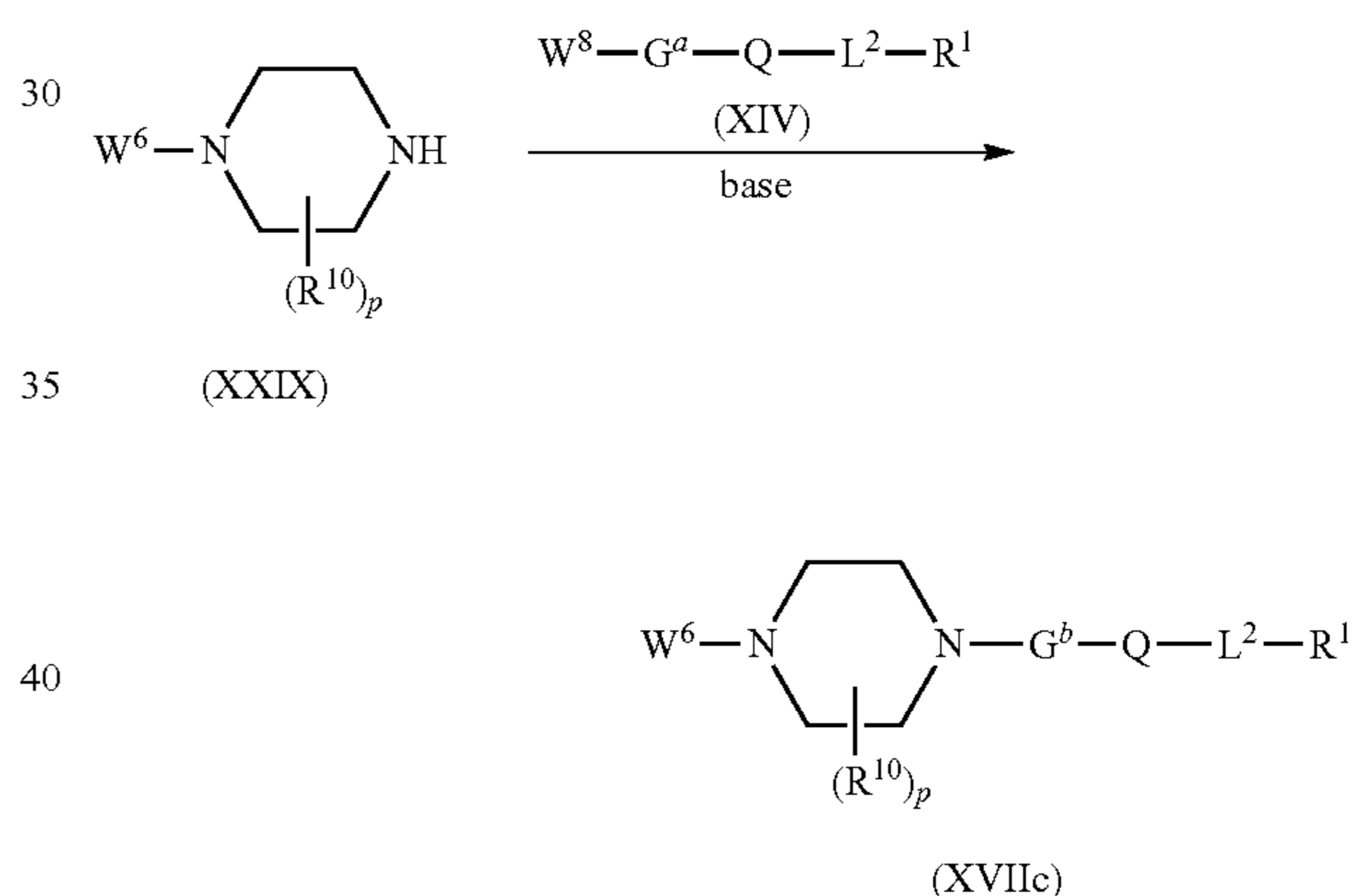
Scheme 16: Process O
