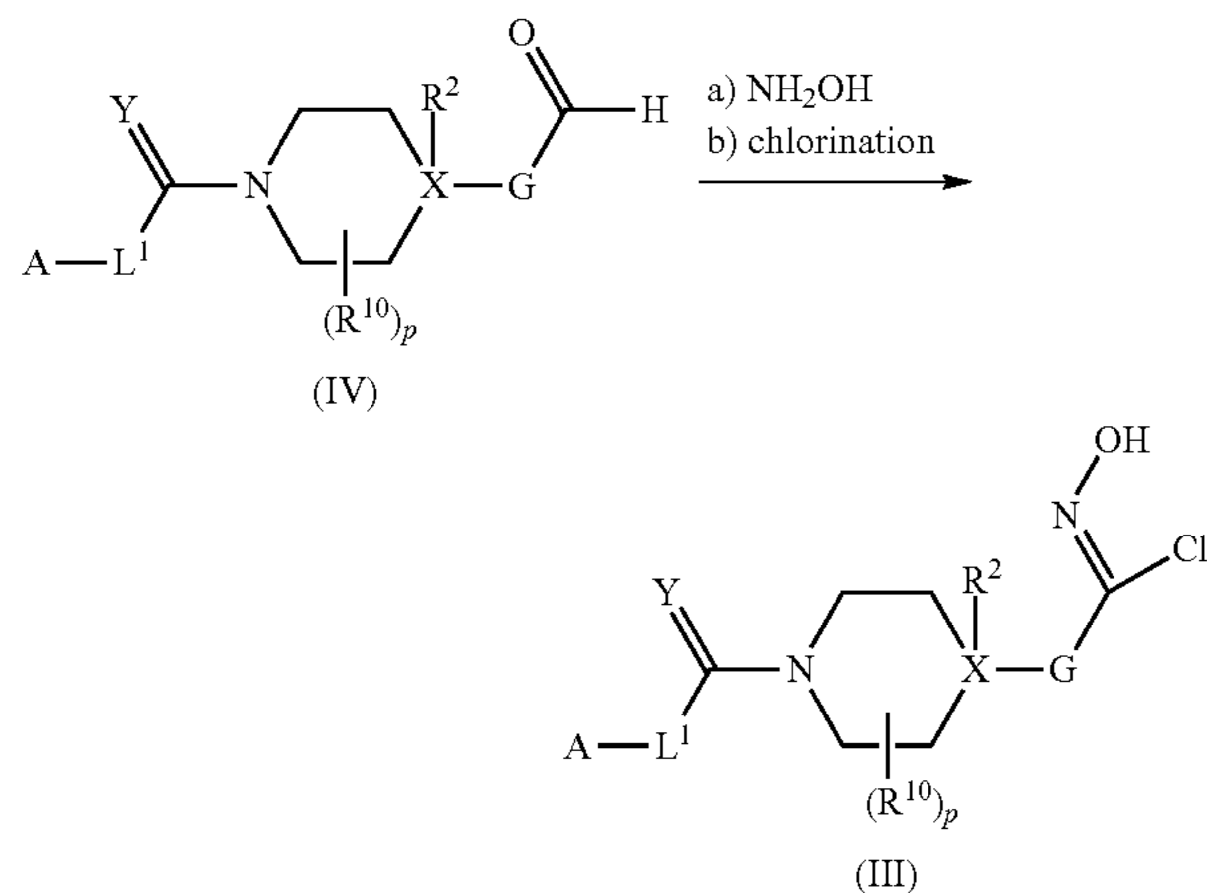
Scheme 3: Process C
