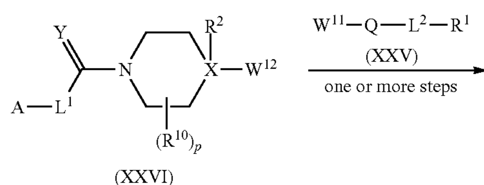
Scheme 4: Process D
