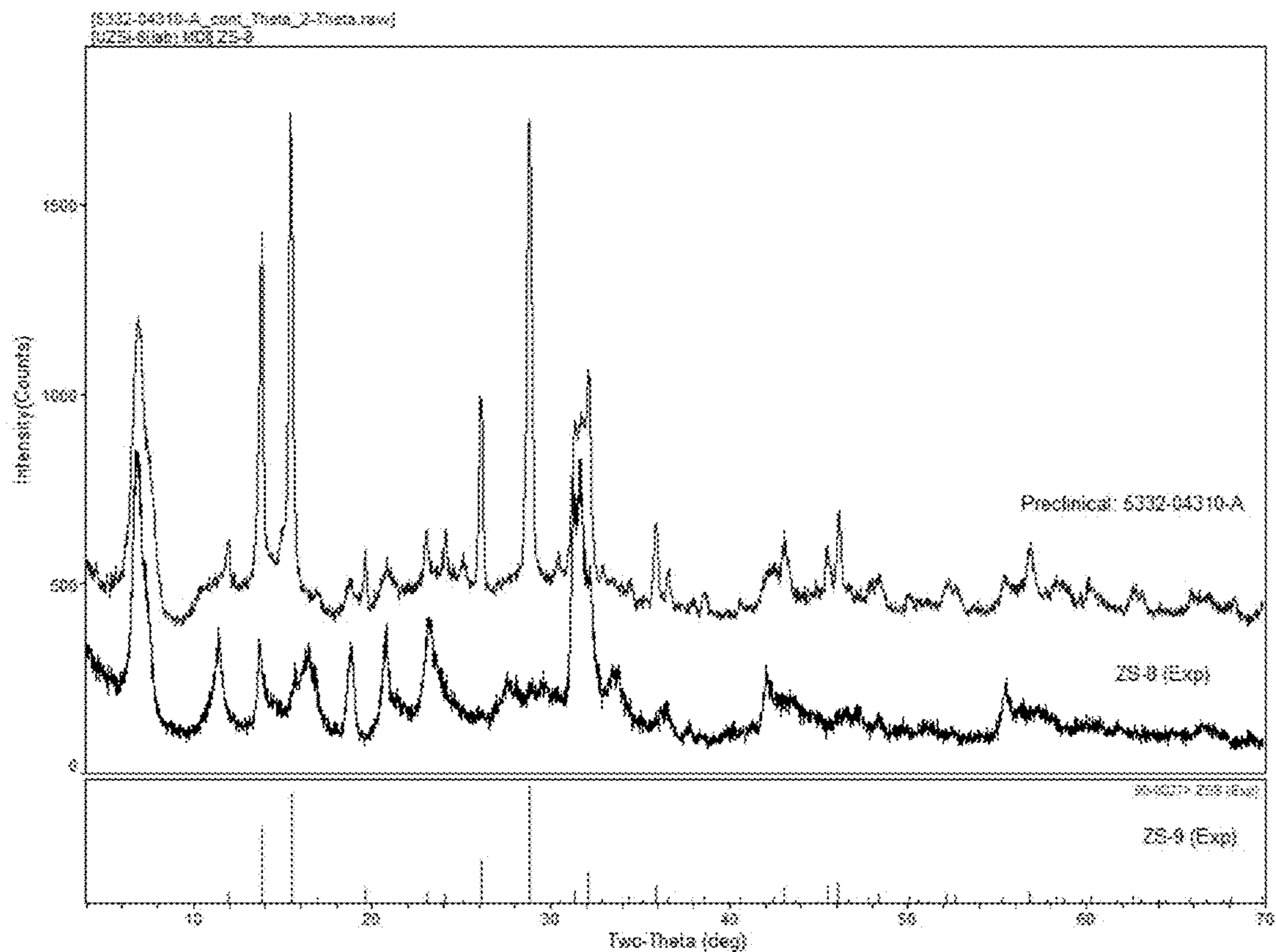
Fig. 30: XRD data showing ZS-8 impurities.
