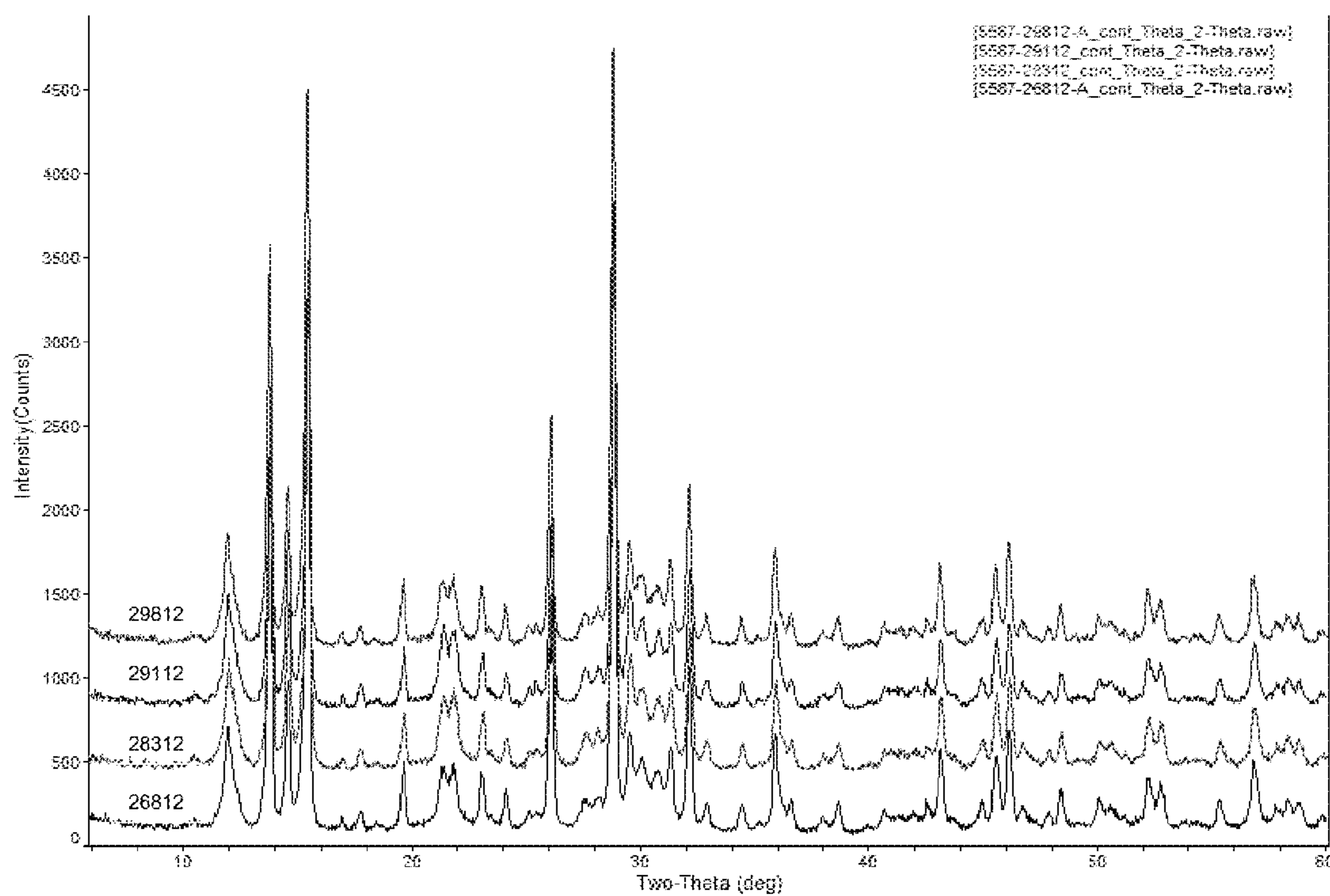
Fig. 29: XRD data for ZS crystals produced according to Example 20.
