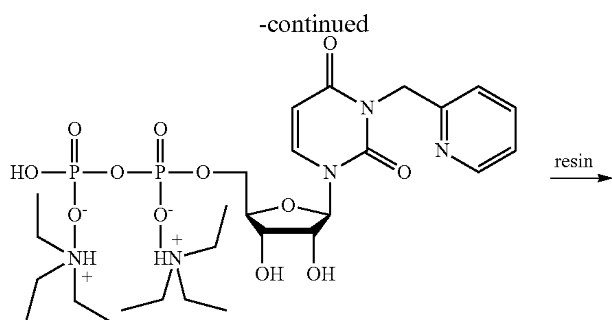
TEA salt of compound 3
