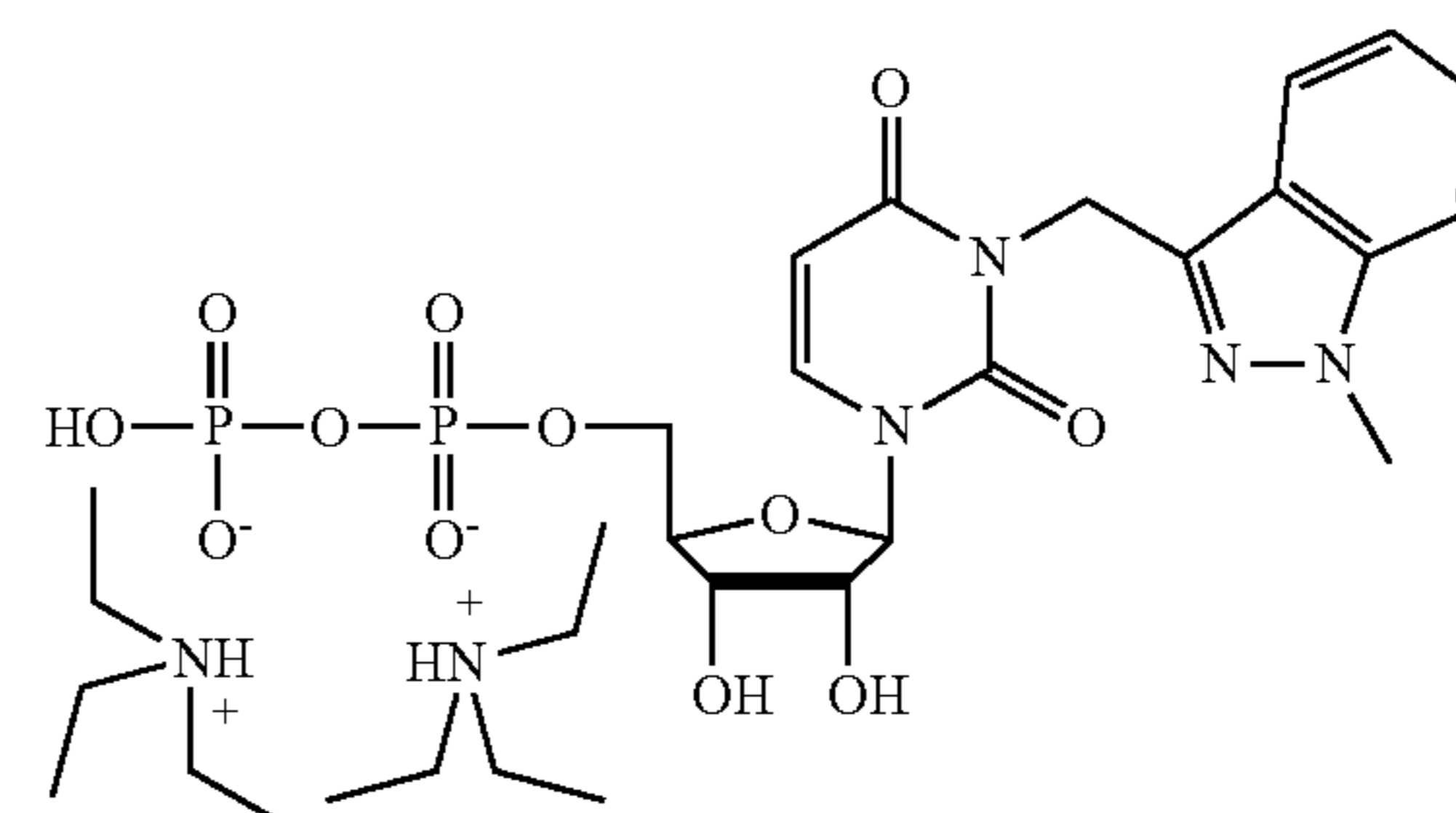
TEA salt of compound 4
