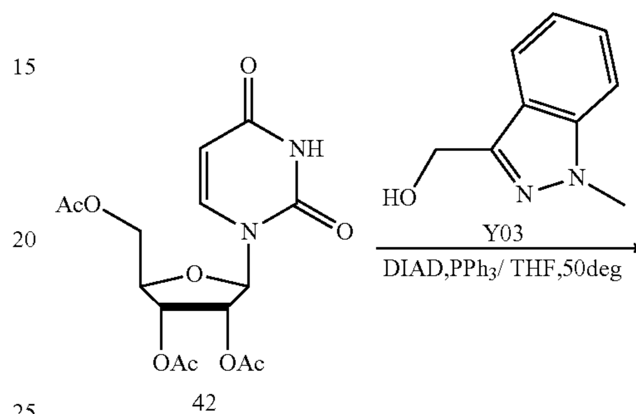
Scheme 4
