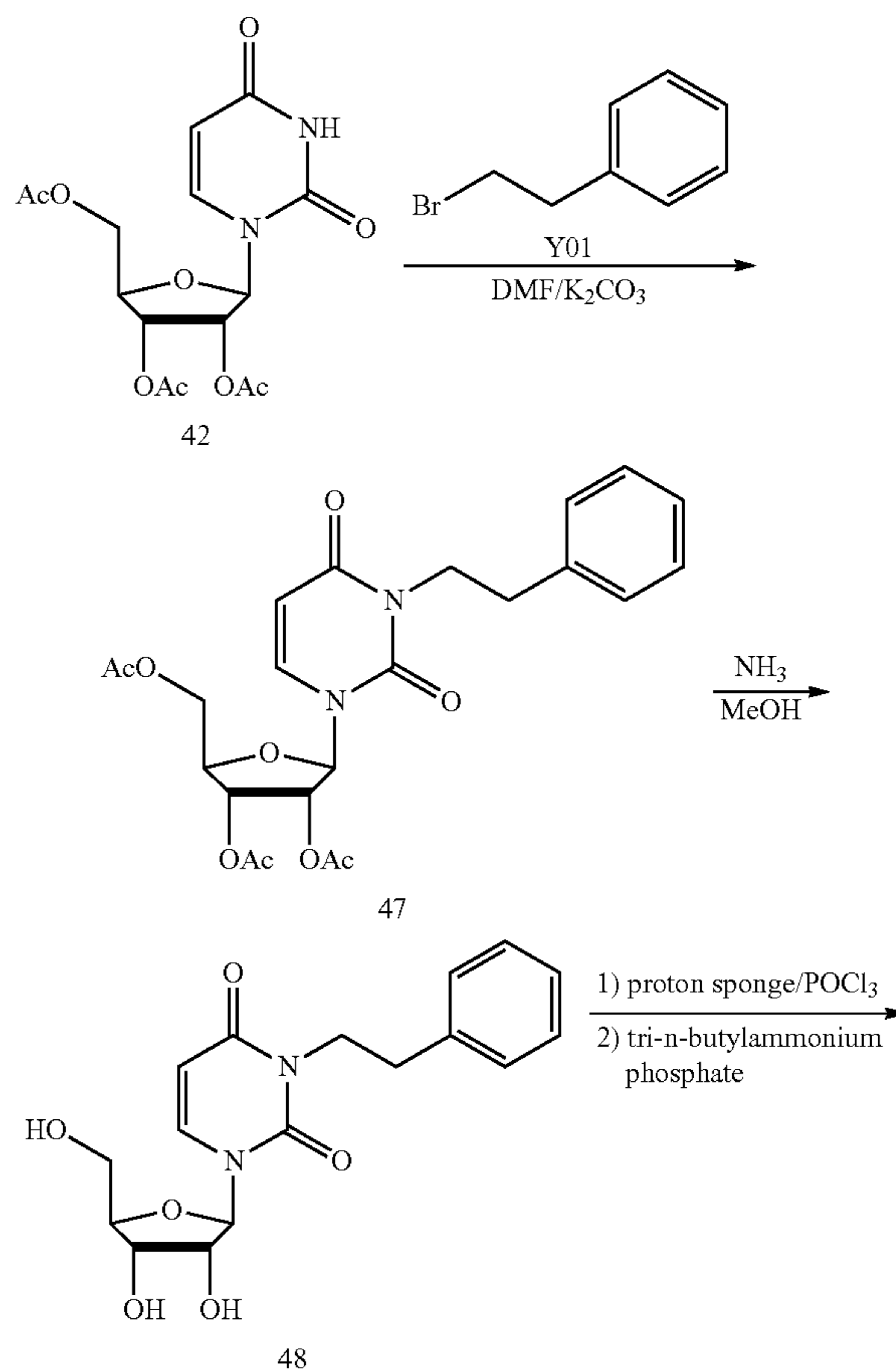
Scheme 2
