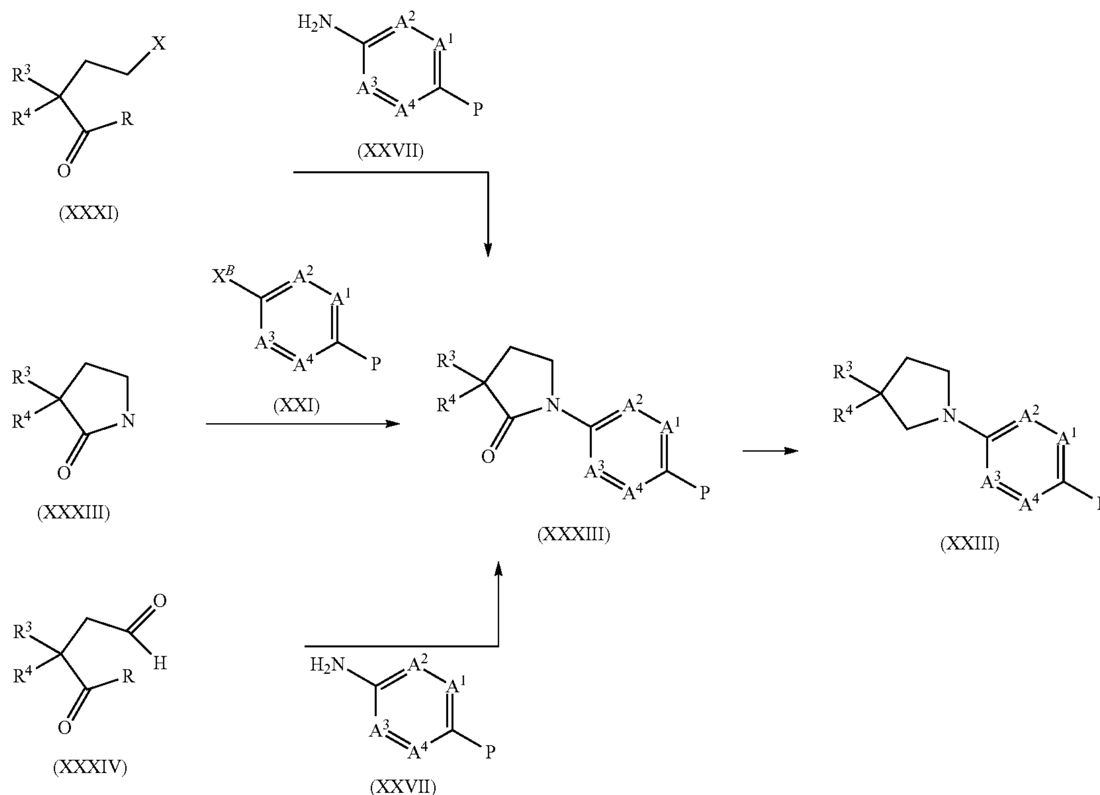
Scheme 10
