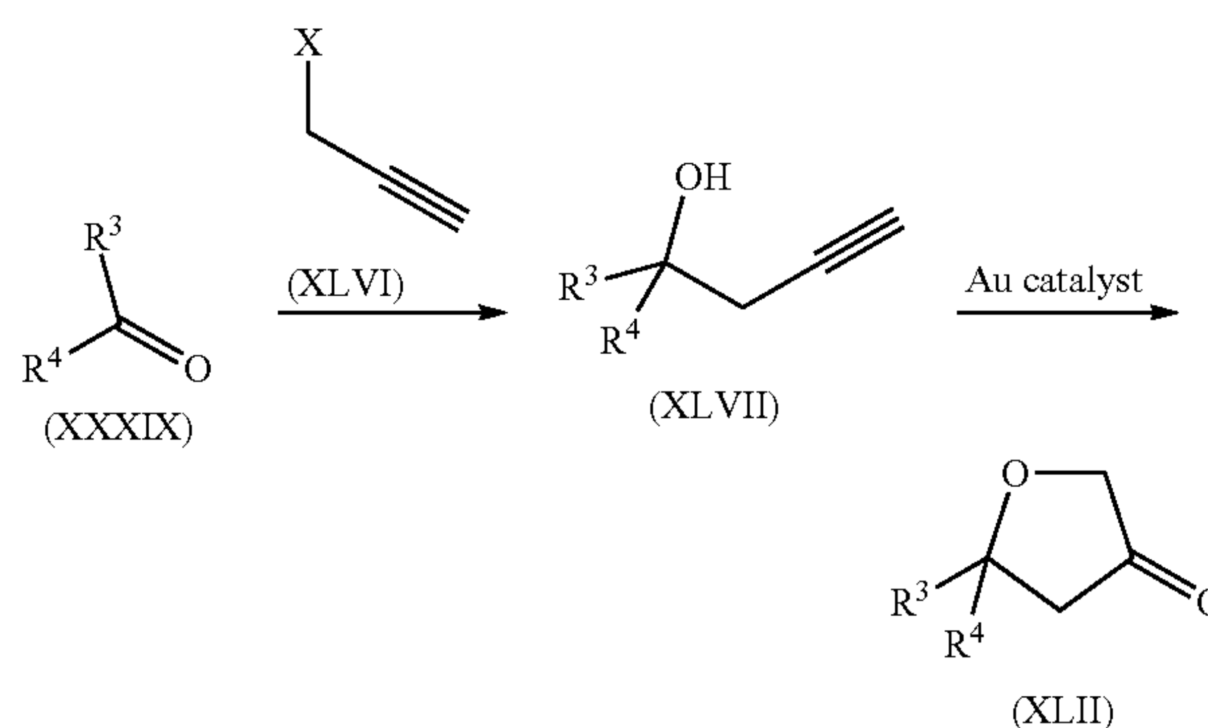
Scheme 14
