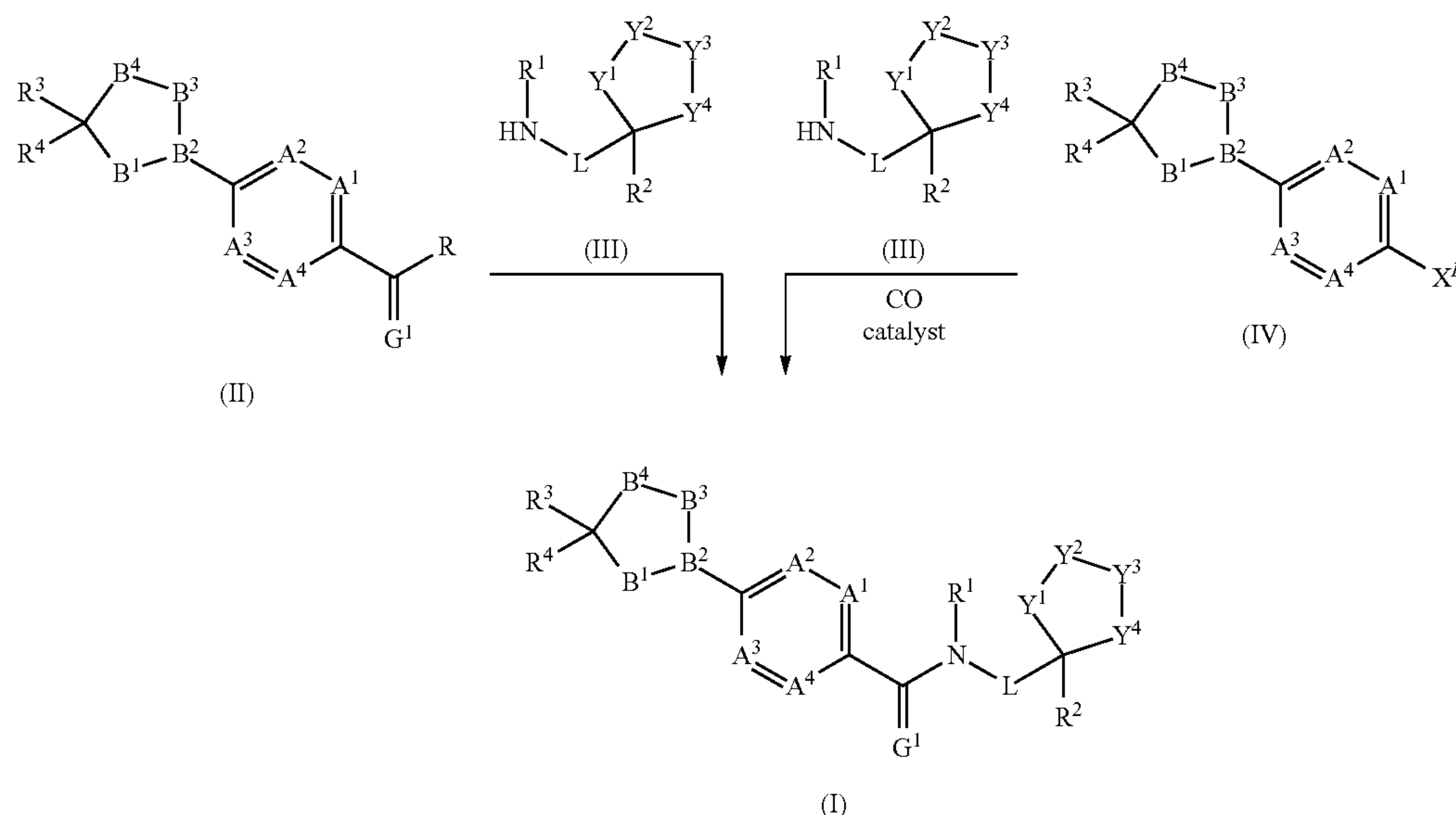
Scheme 1
