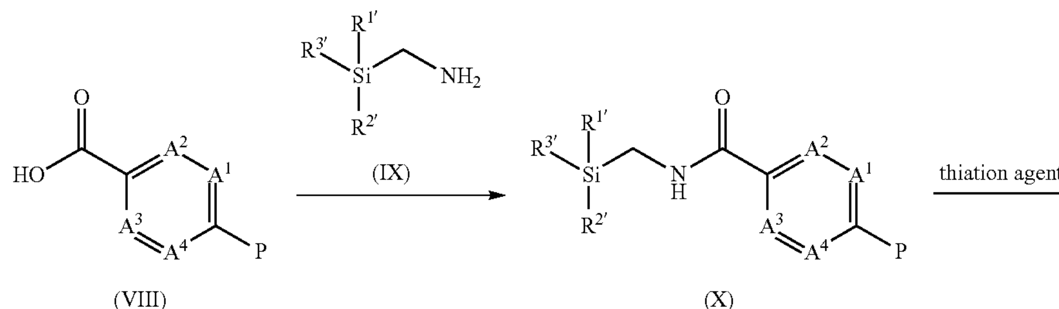
Scheme 3
