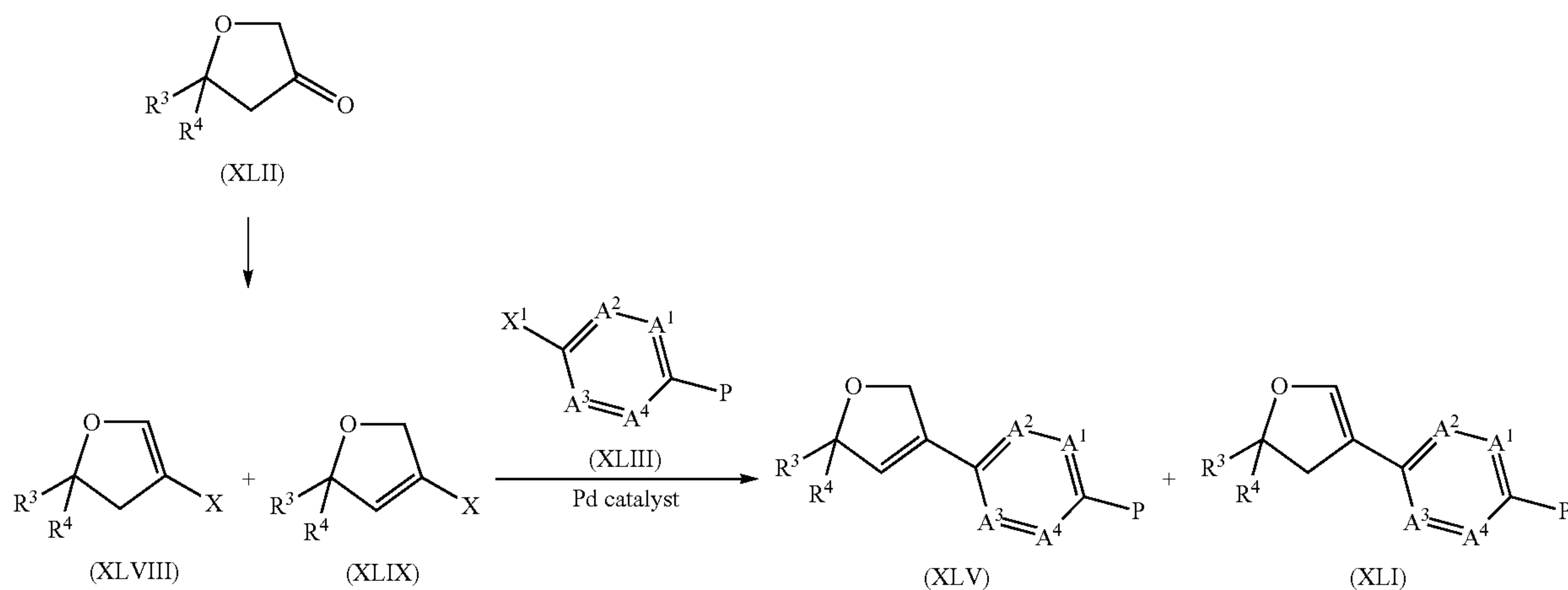
Scheme 15
