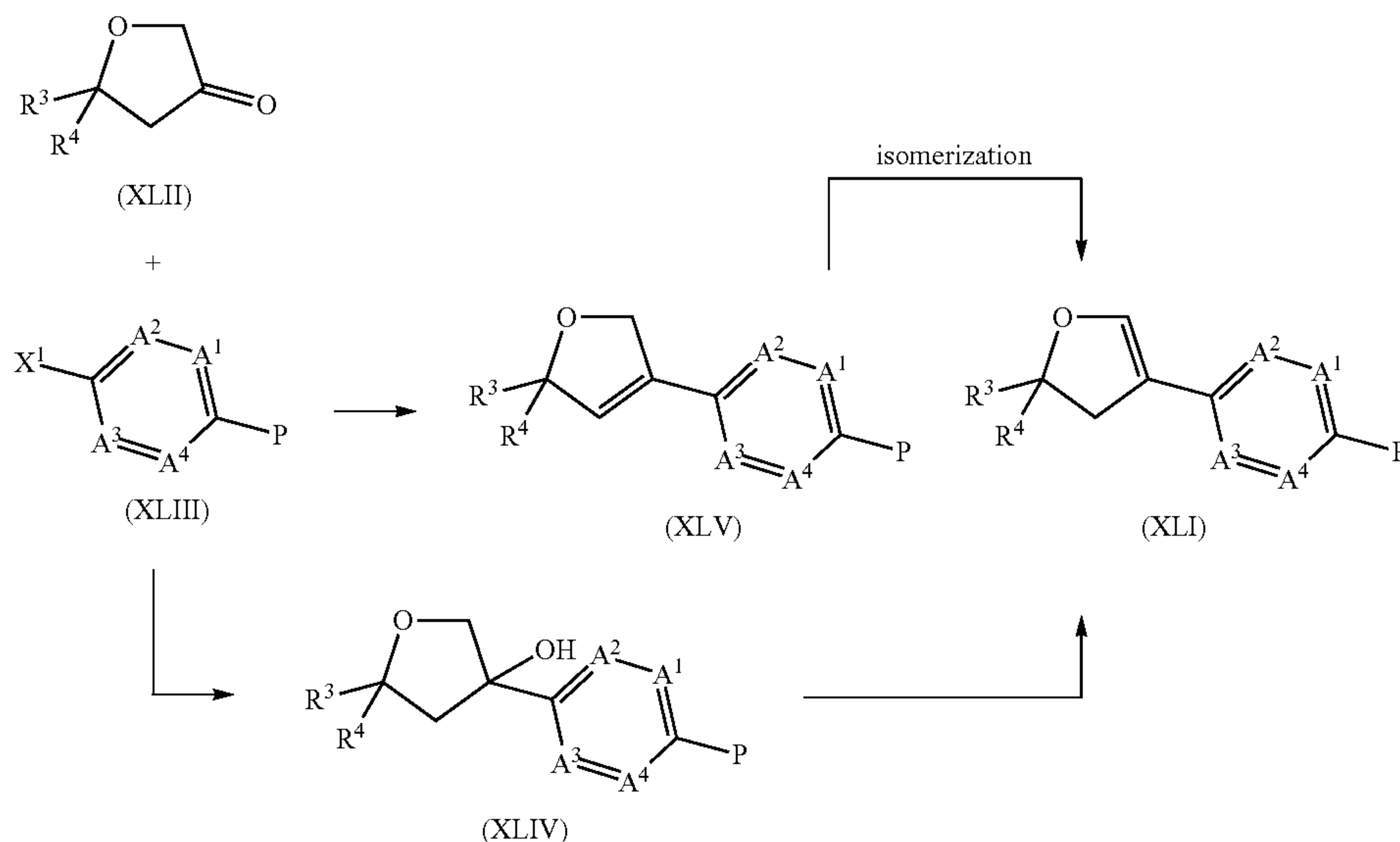
Scheme 13
