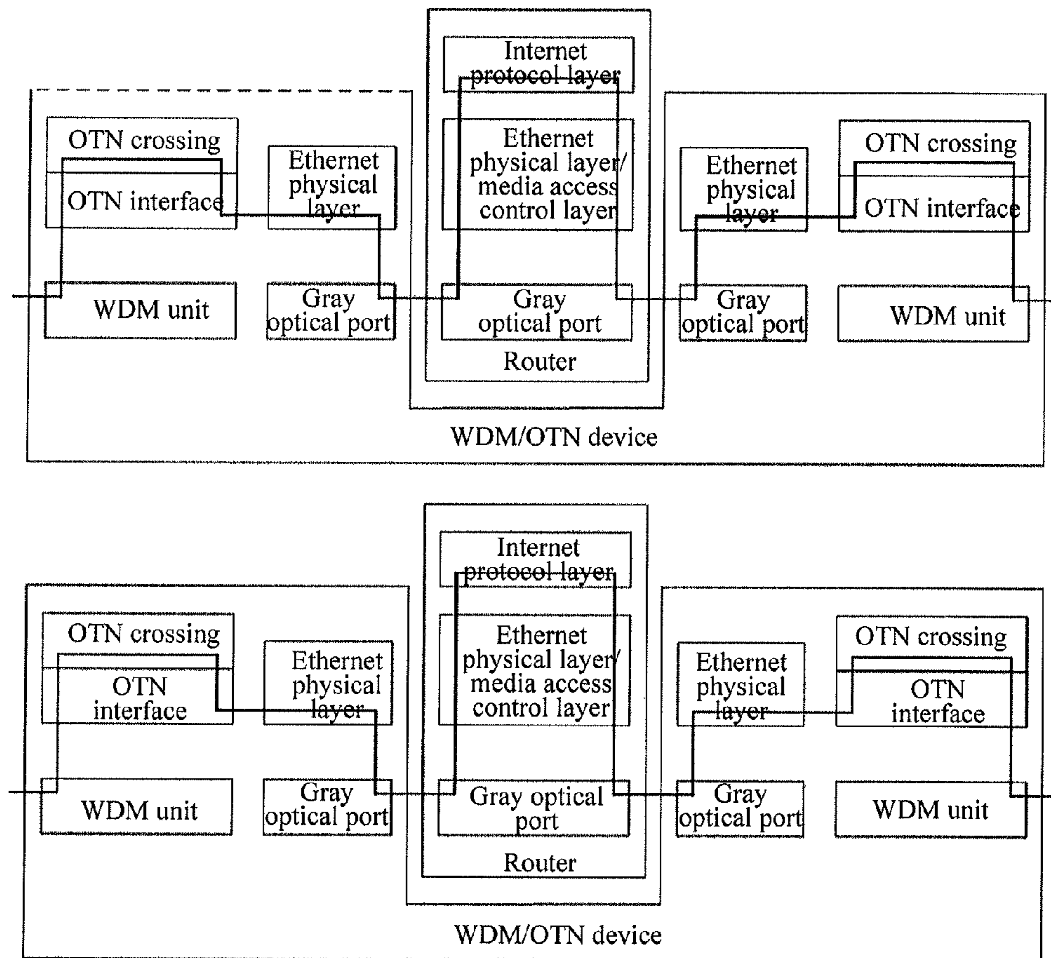
FIG. 2 (PRIOR ART)
