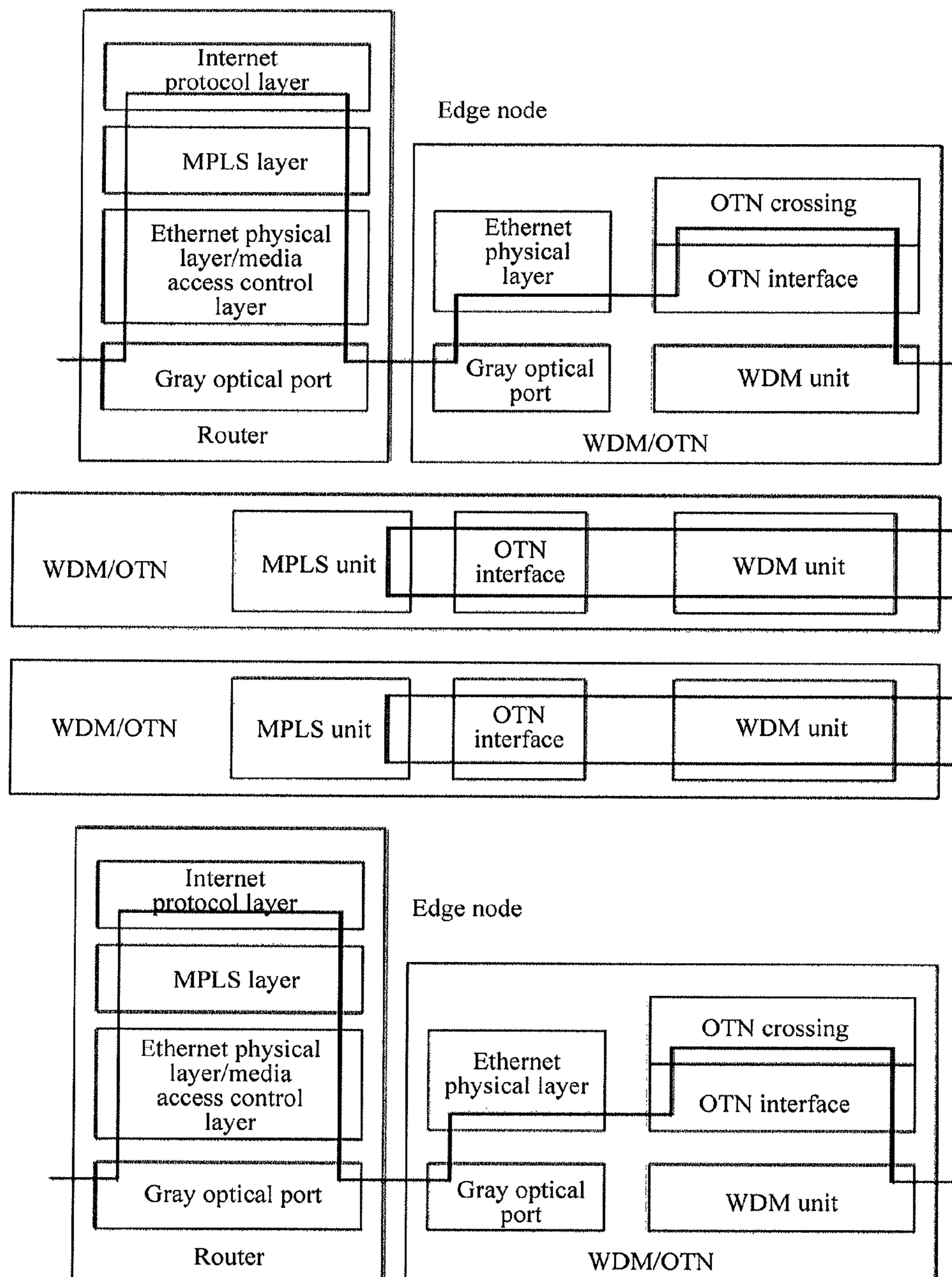
FIG. 4 (PRIOR ART)
