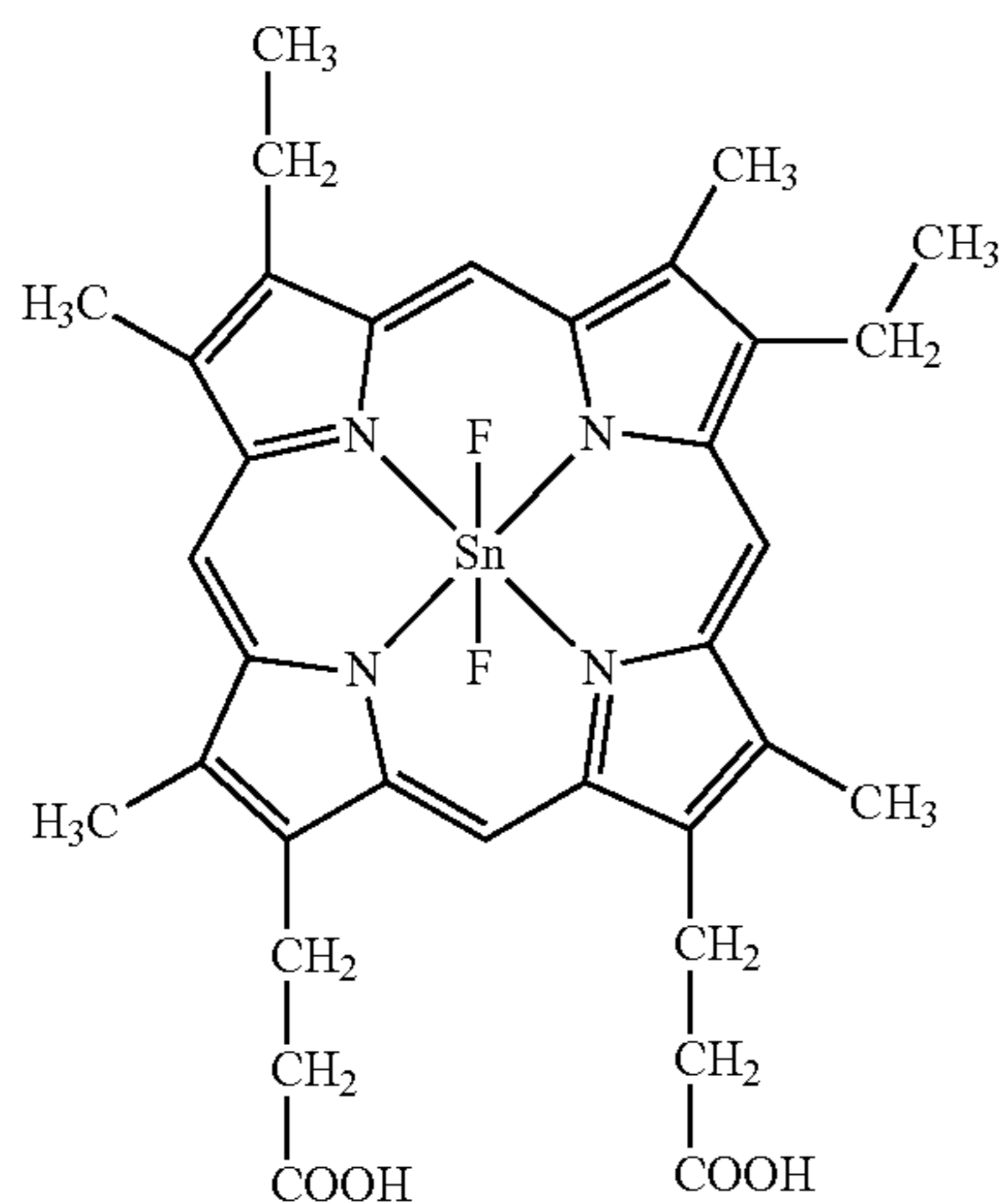
\text{SnF}_2(\text{Meso IX})
