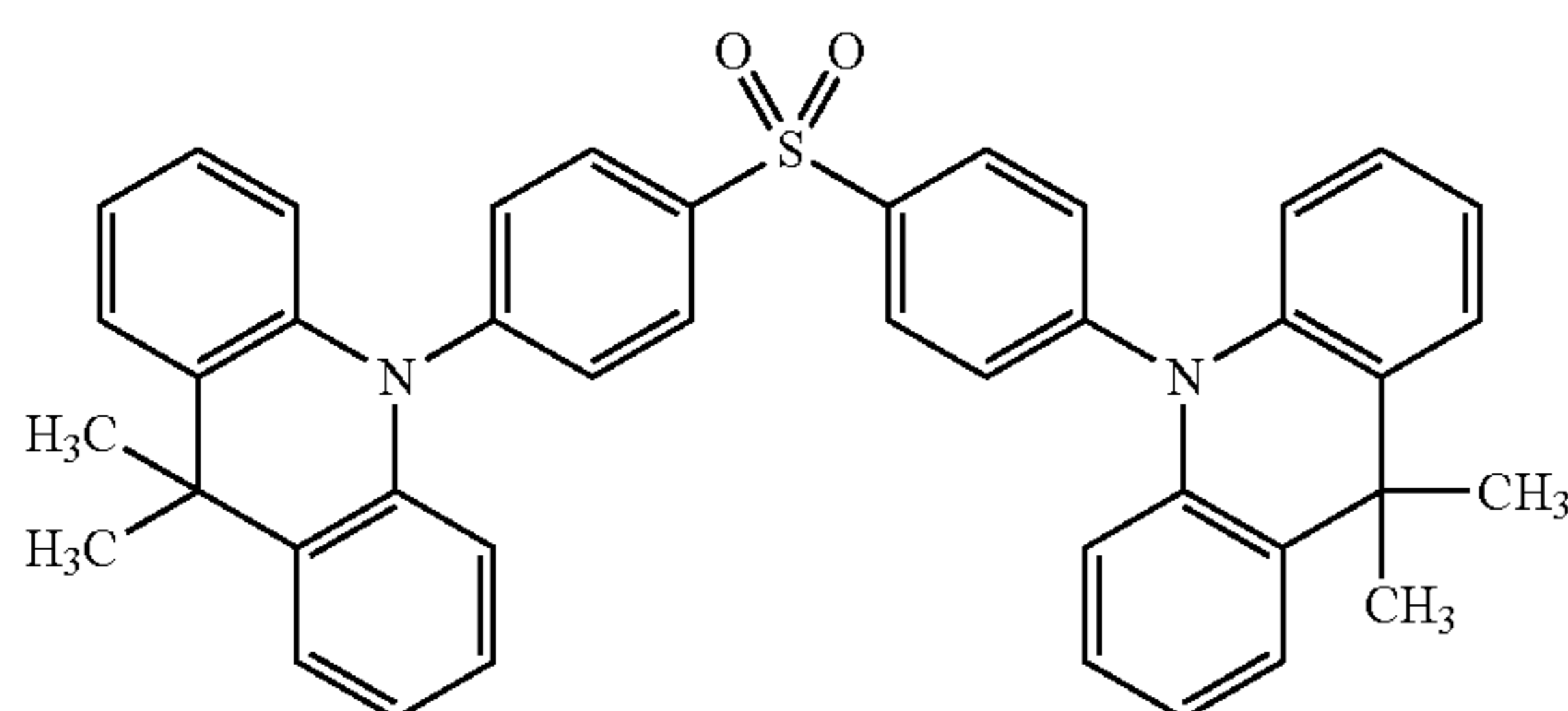
DMAC-DPS
