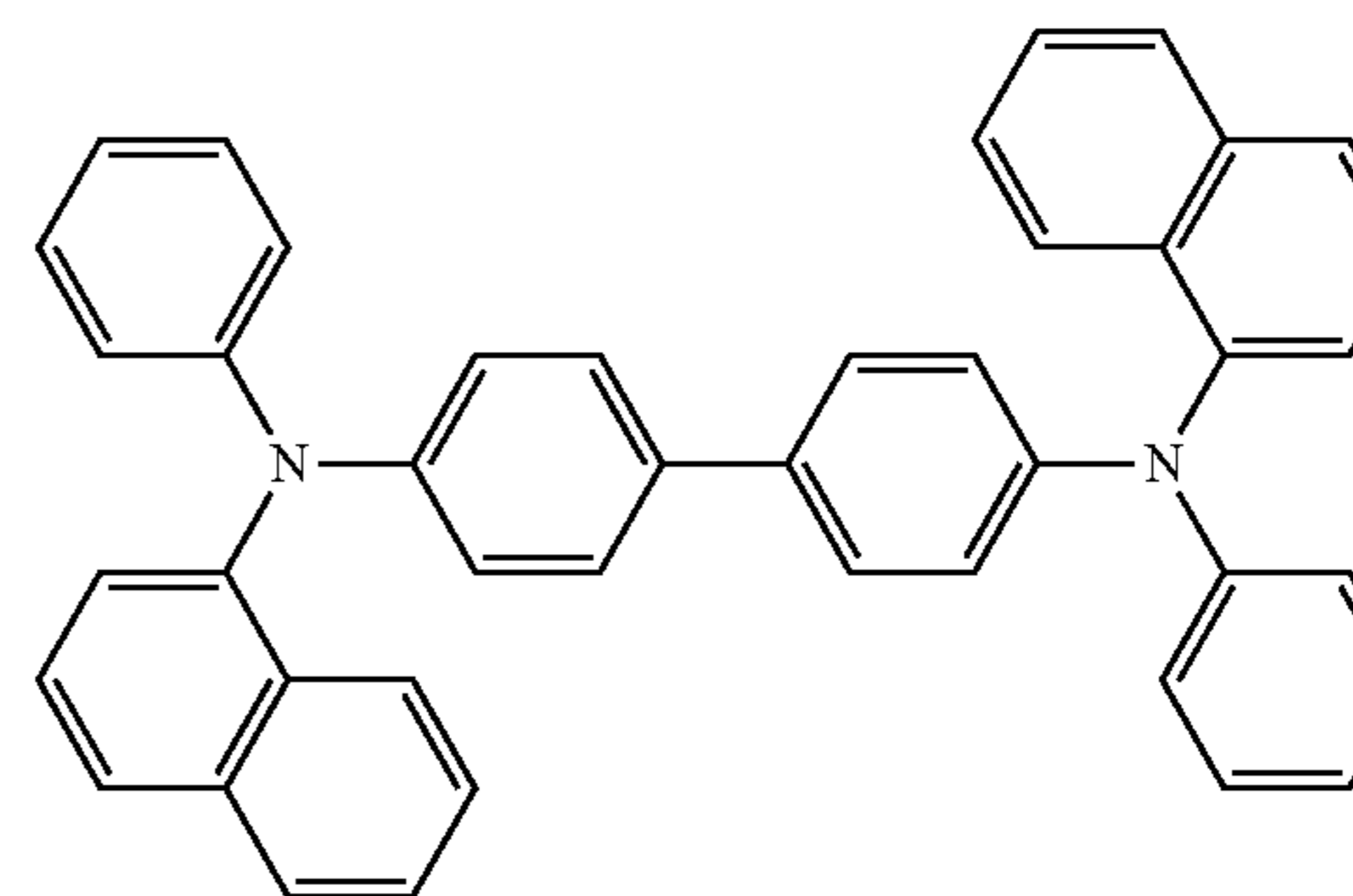
NPB
