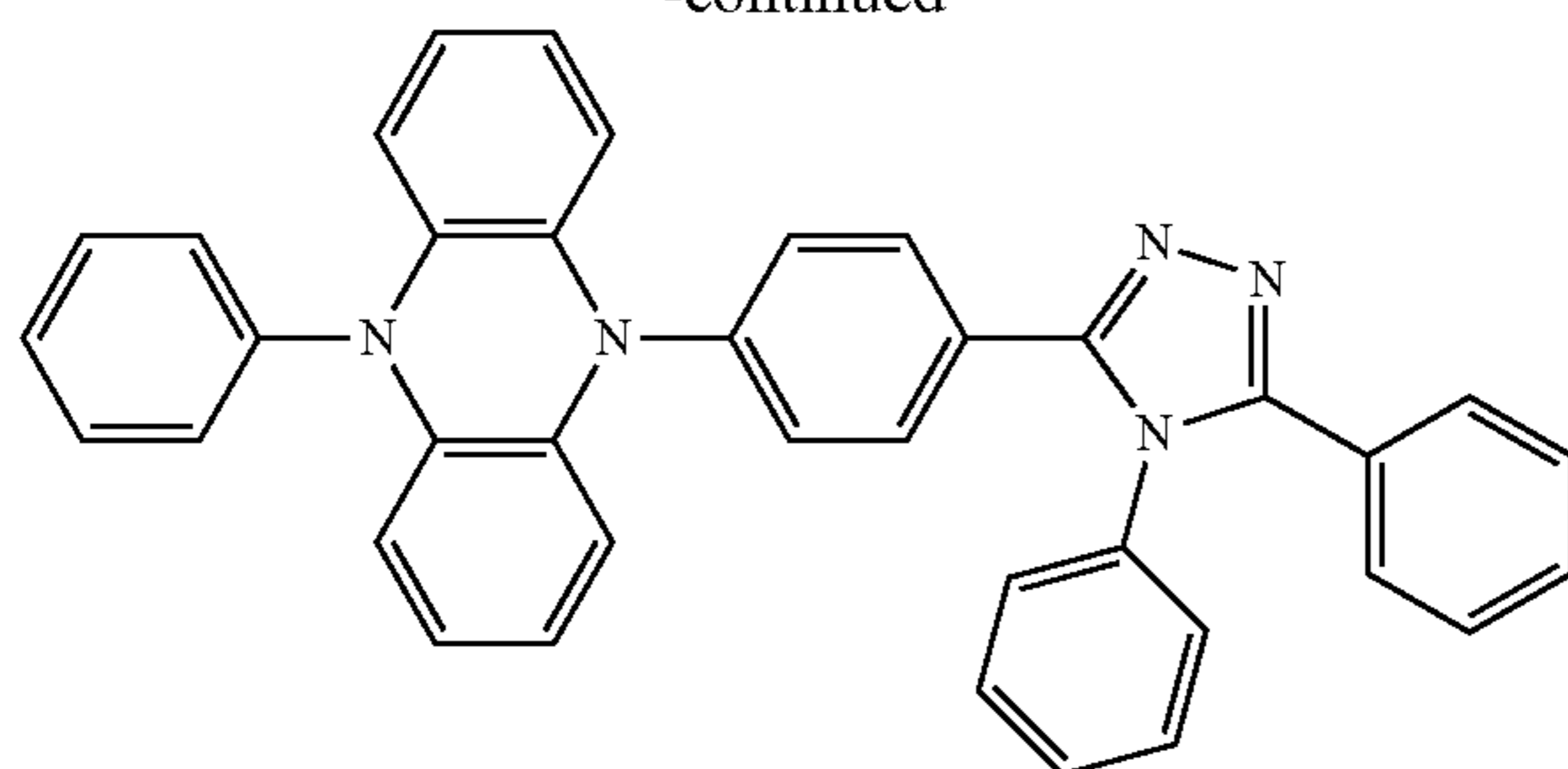
PPZ-3TPT
