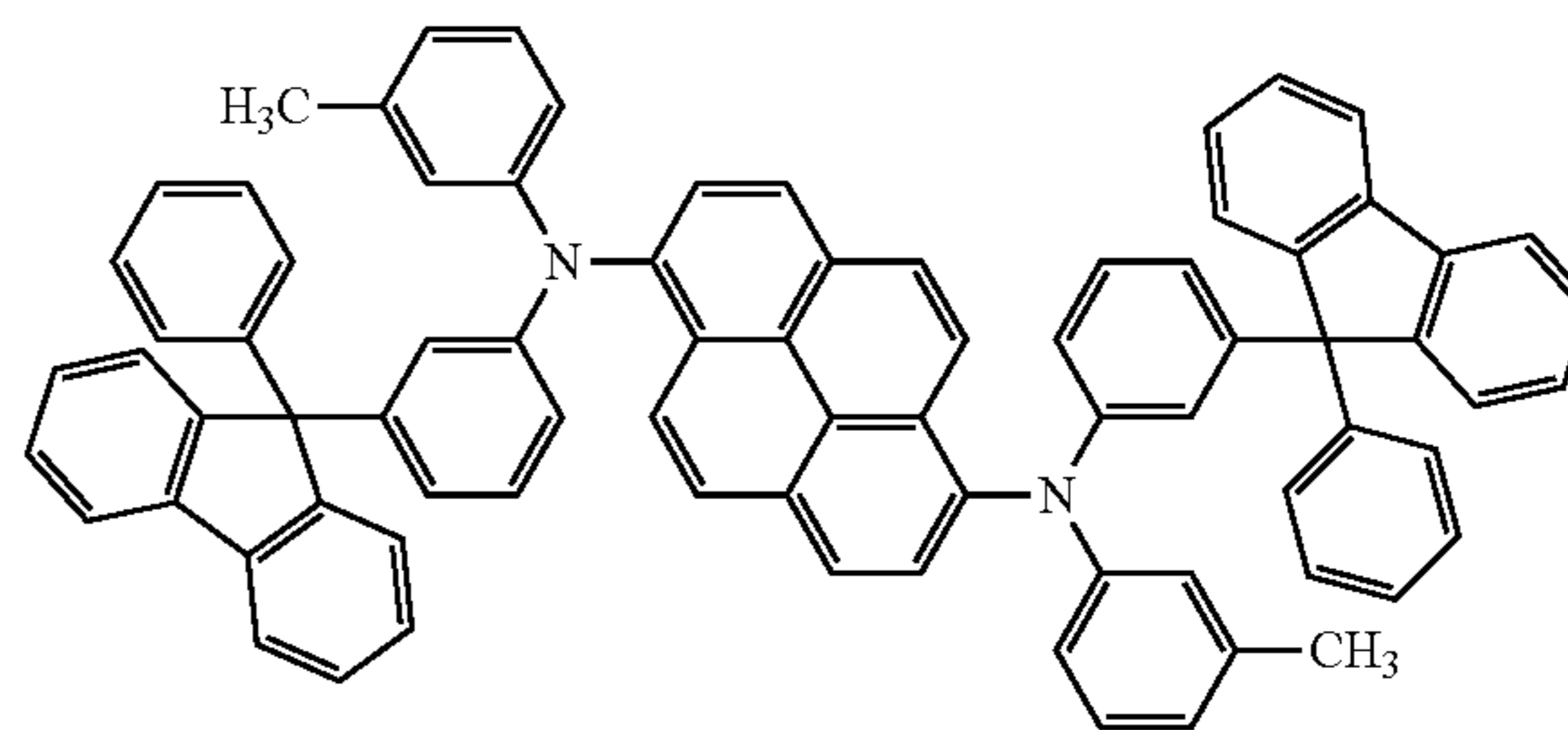
1,6mMemFLPAPrn
