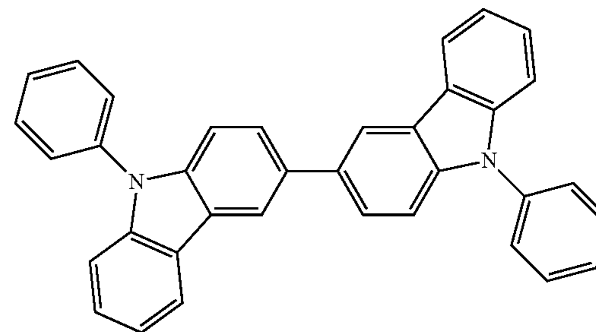
PCCP
