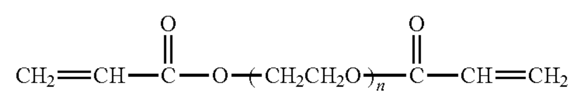
PEG diacrylate
