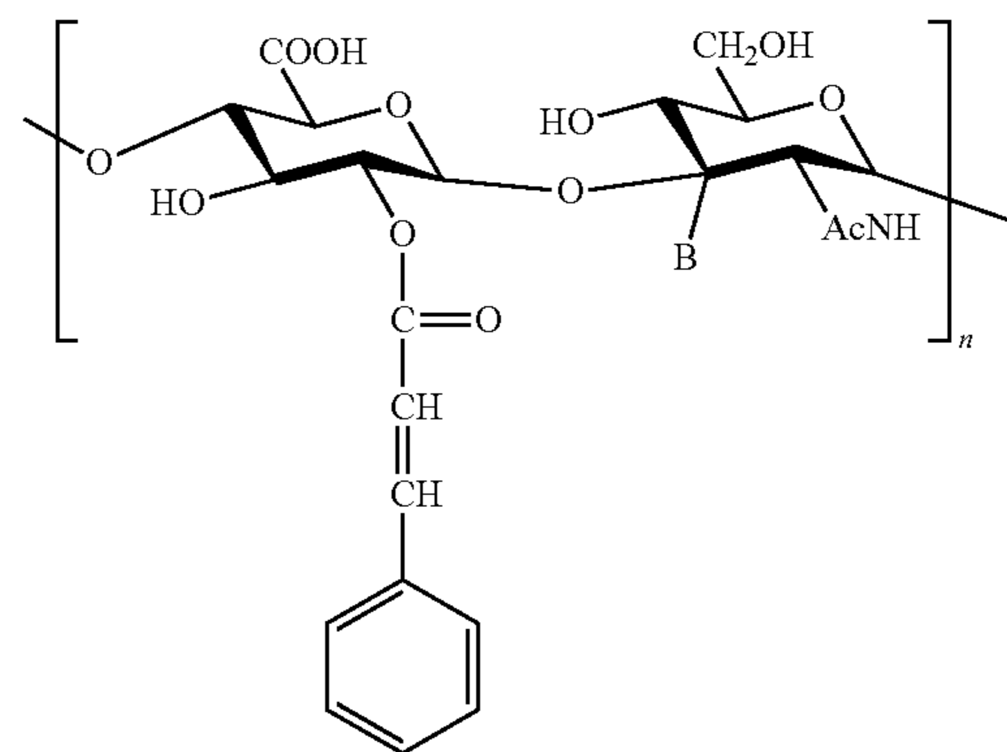
Commuted hyaluronic acid
