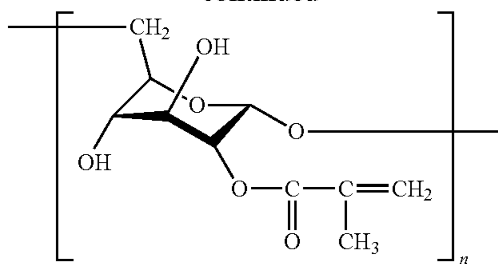
Methacrylate-modified Dextran
