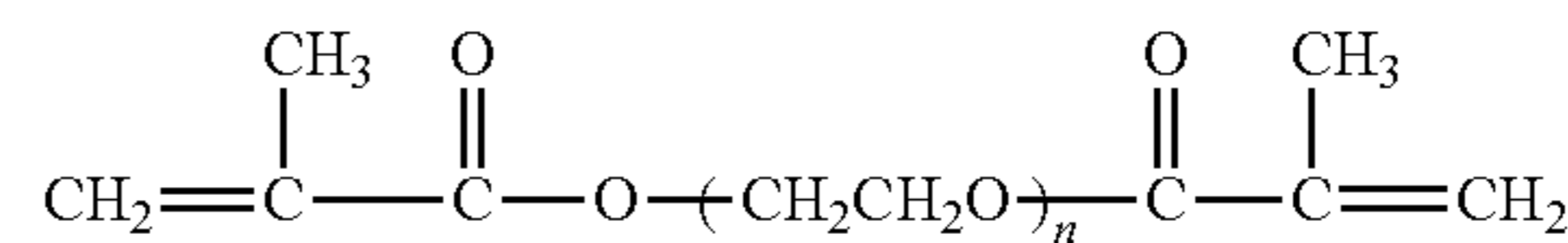
PEG diamethacrylate
