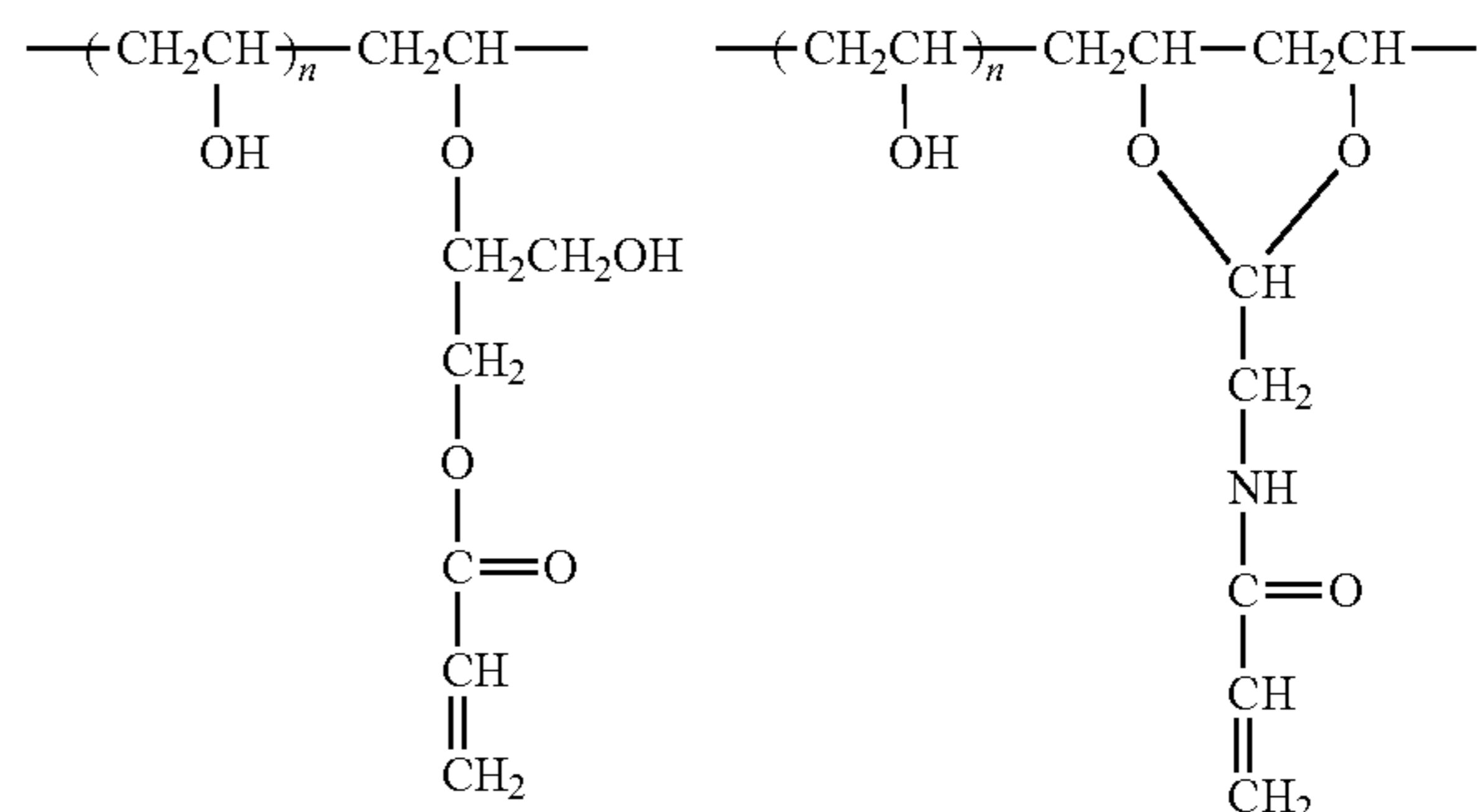
Acrylic modified PVA
