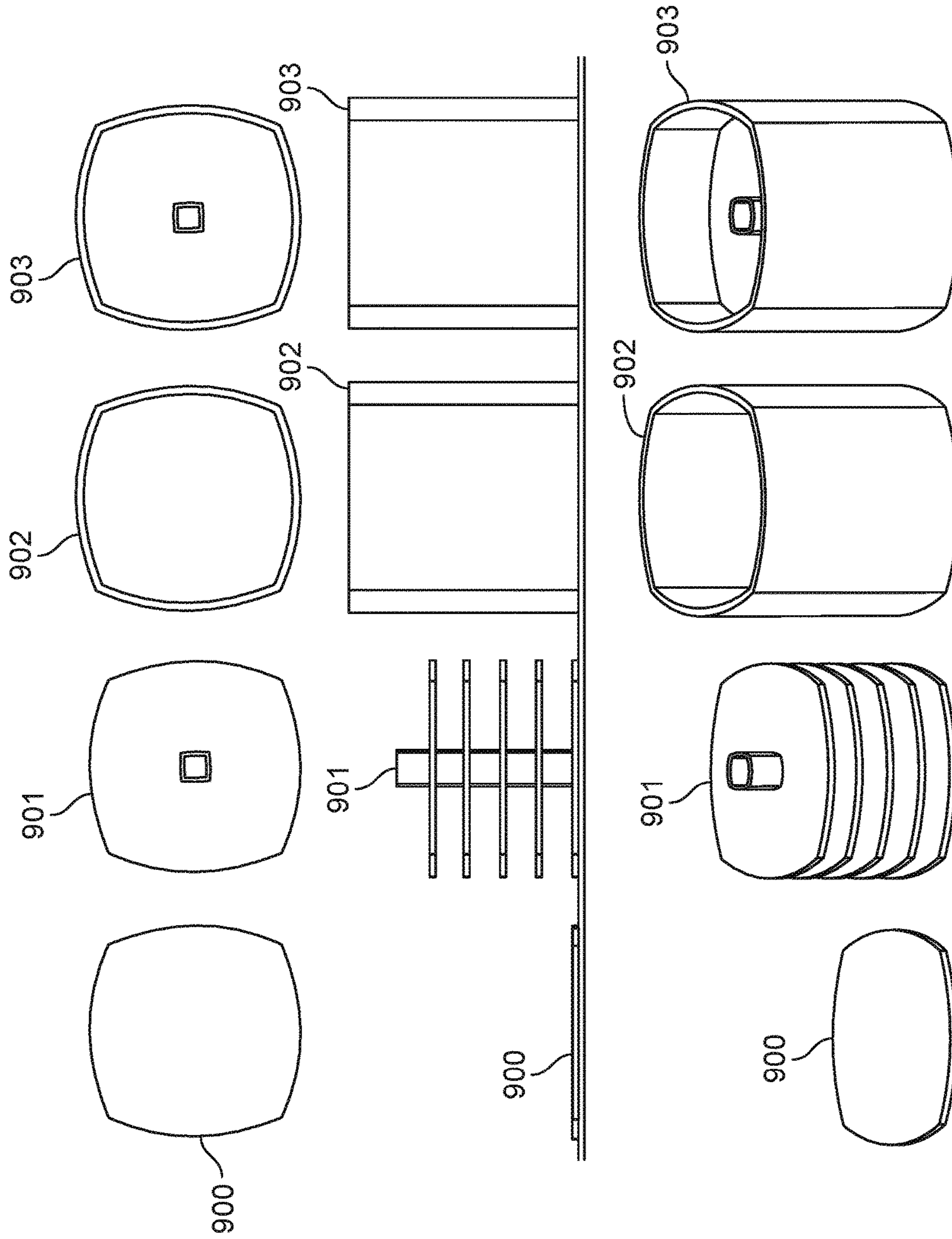
FIG. 9 Plates and Structural Elements - Four-sided Curvilinear Polygon
