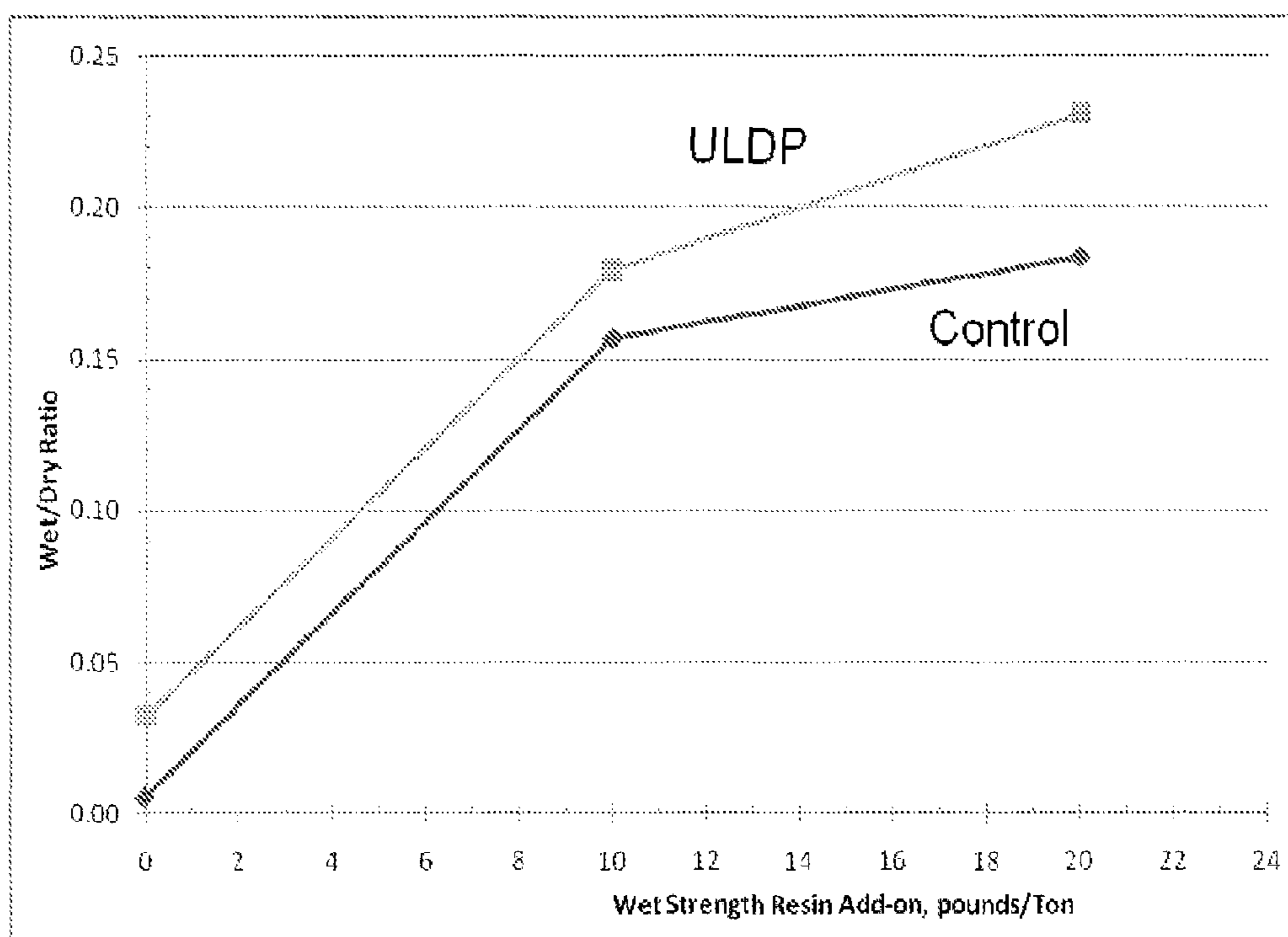
Figure 2. Wet/Dry strength ratio given as a function of wet strength resin level.
