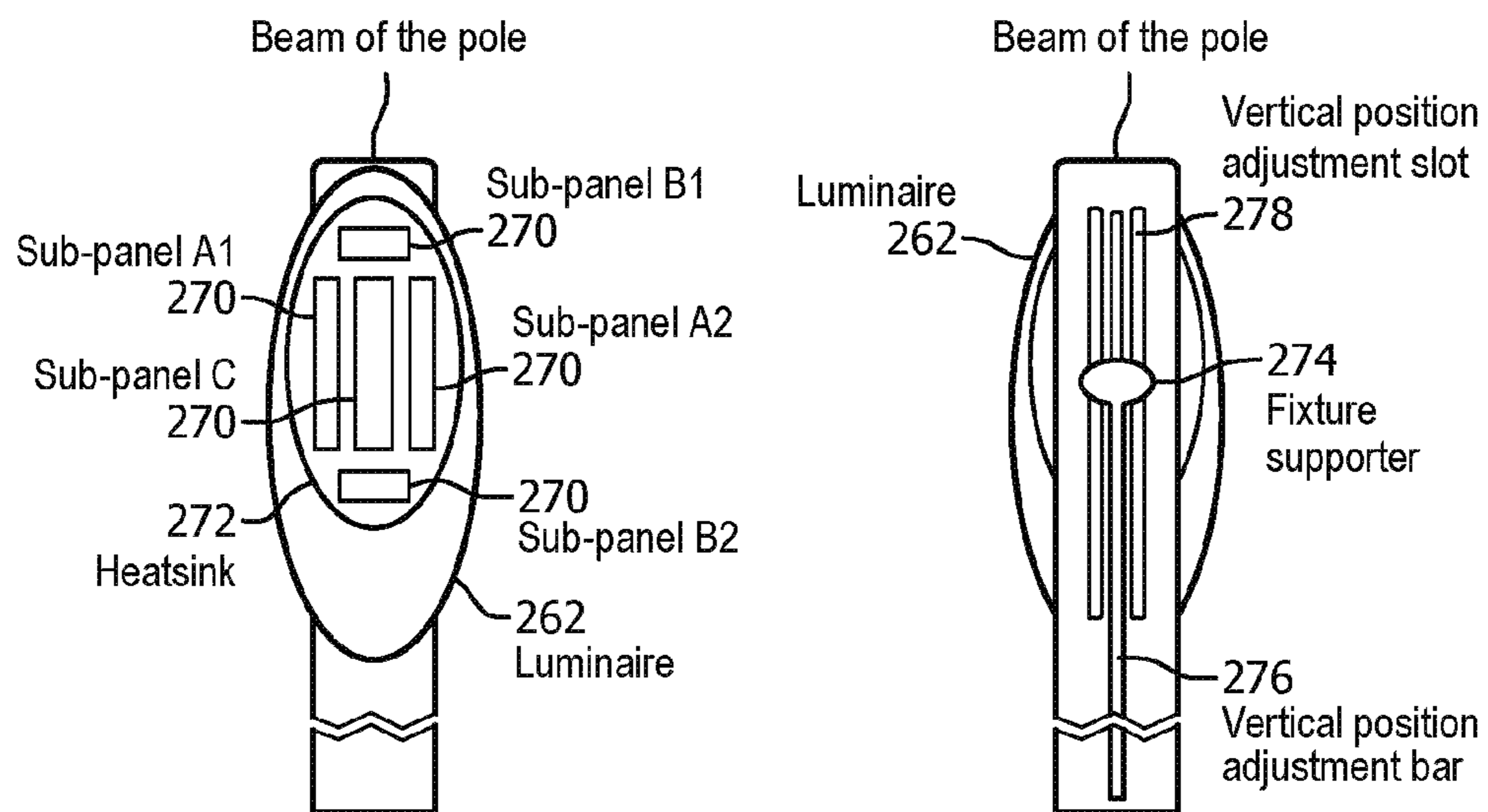
Bottom view
