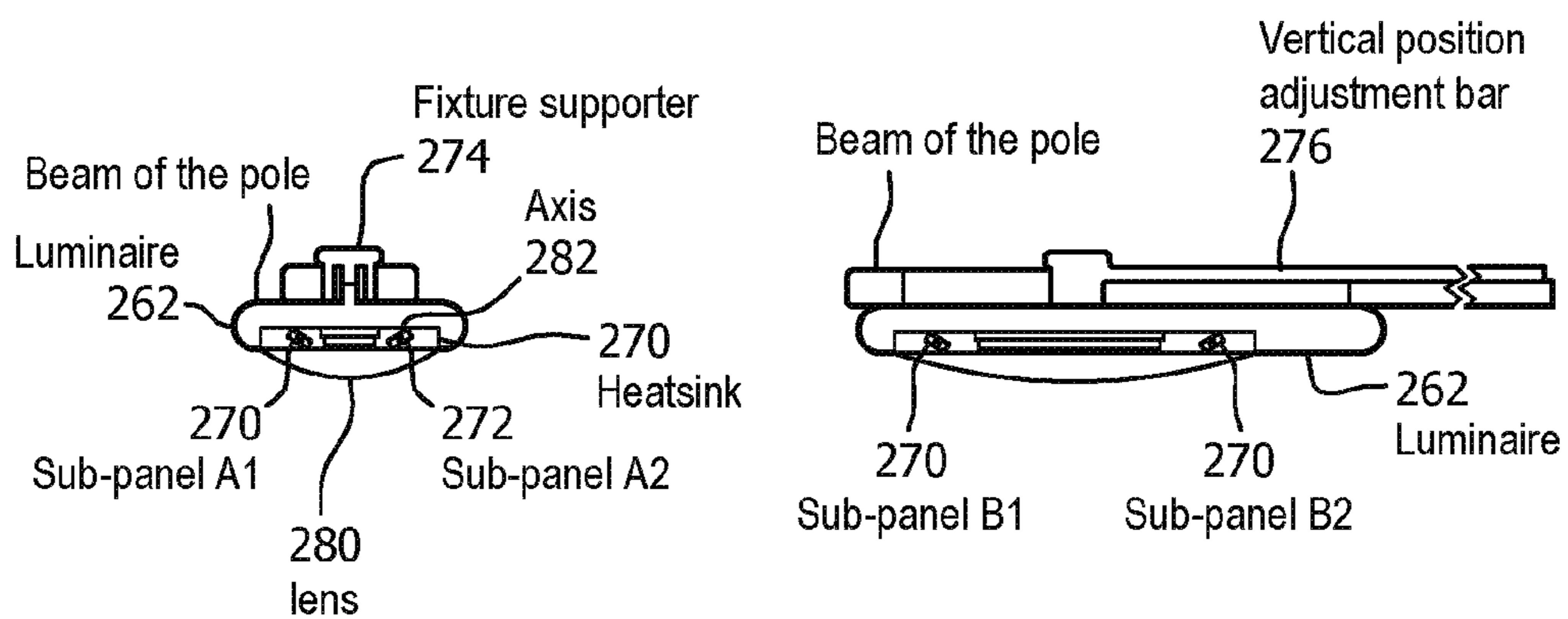
Front view
