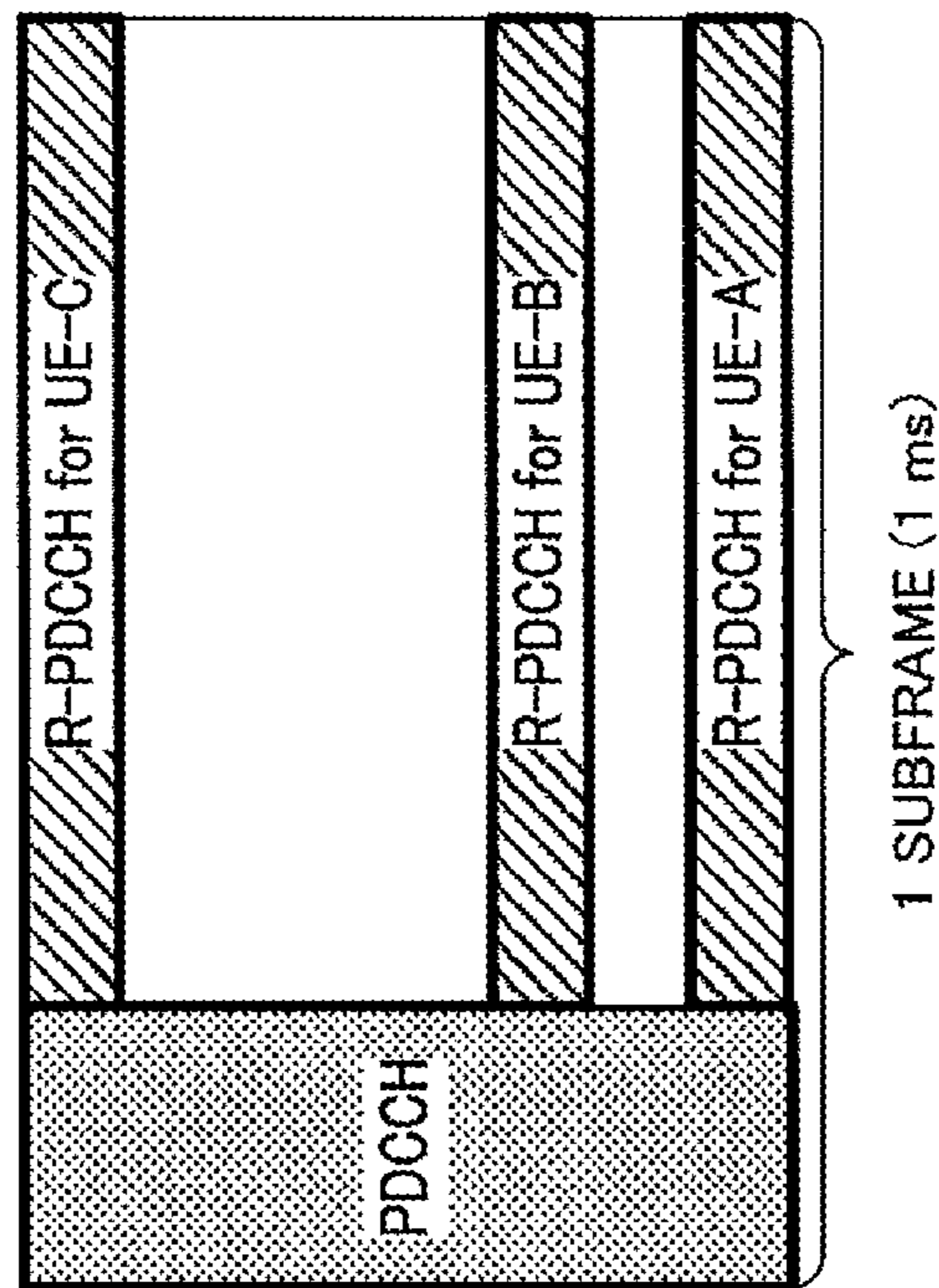
FIG.1A(FDM)
