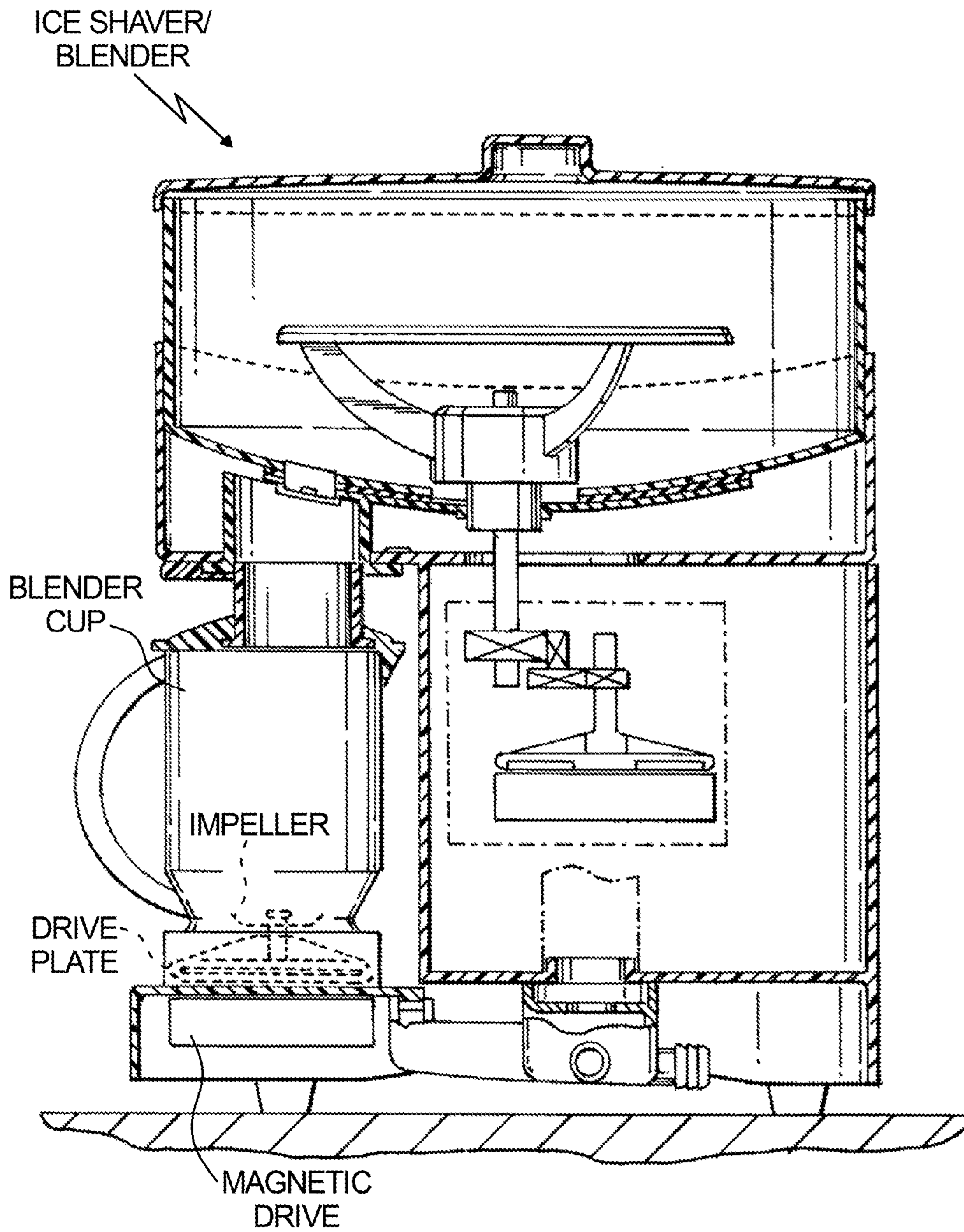
Fig. 2 (Prior Art)
