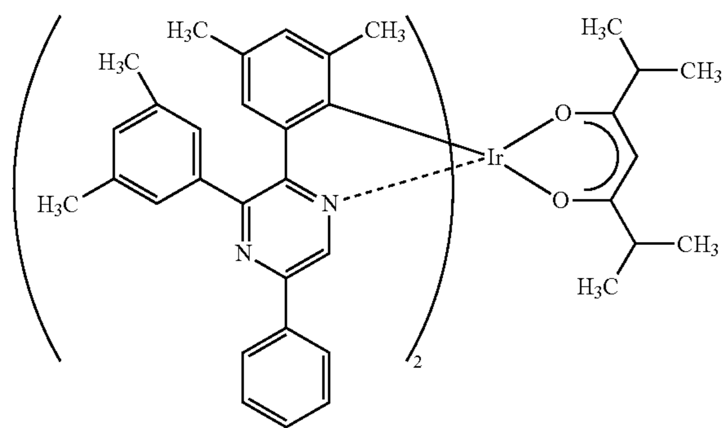
[Ir(dmdppr-P)_2(dibm)]
