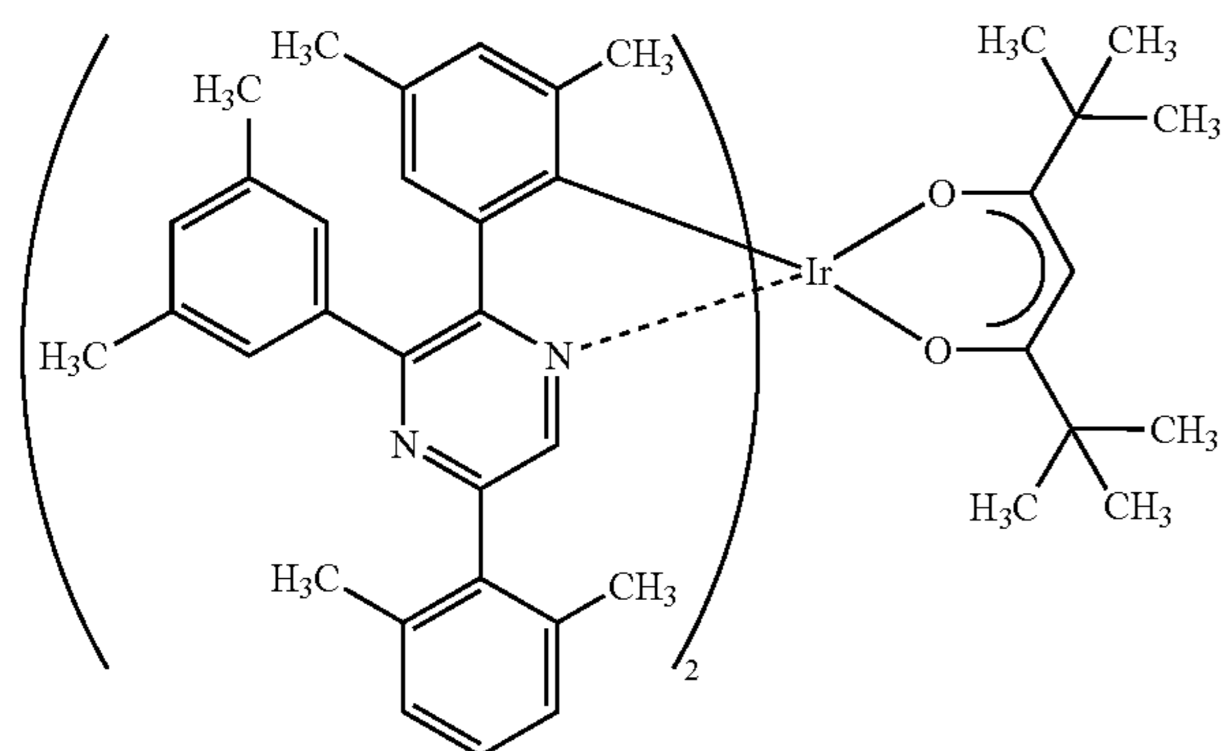
[Ir(dmdppr-dmp) 2 (dpm)]
