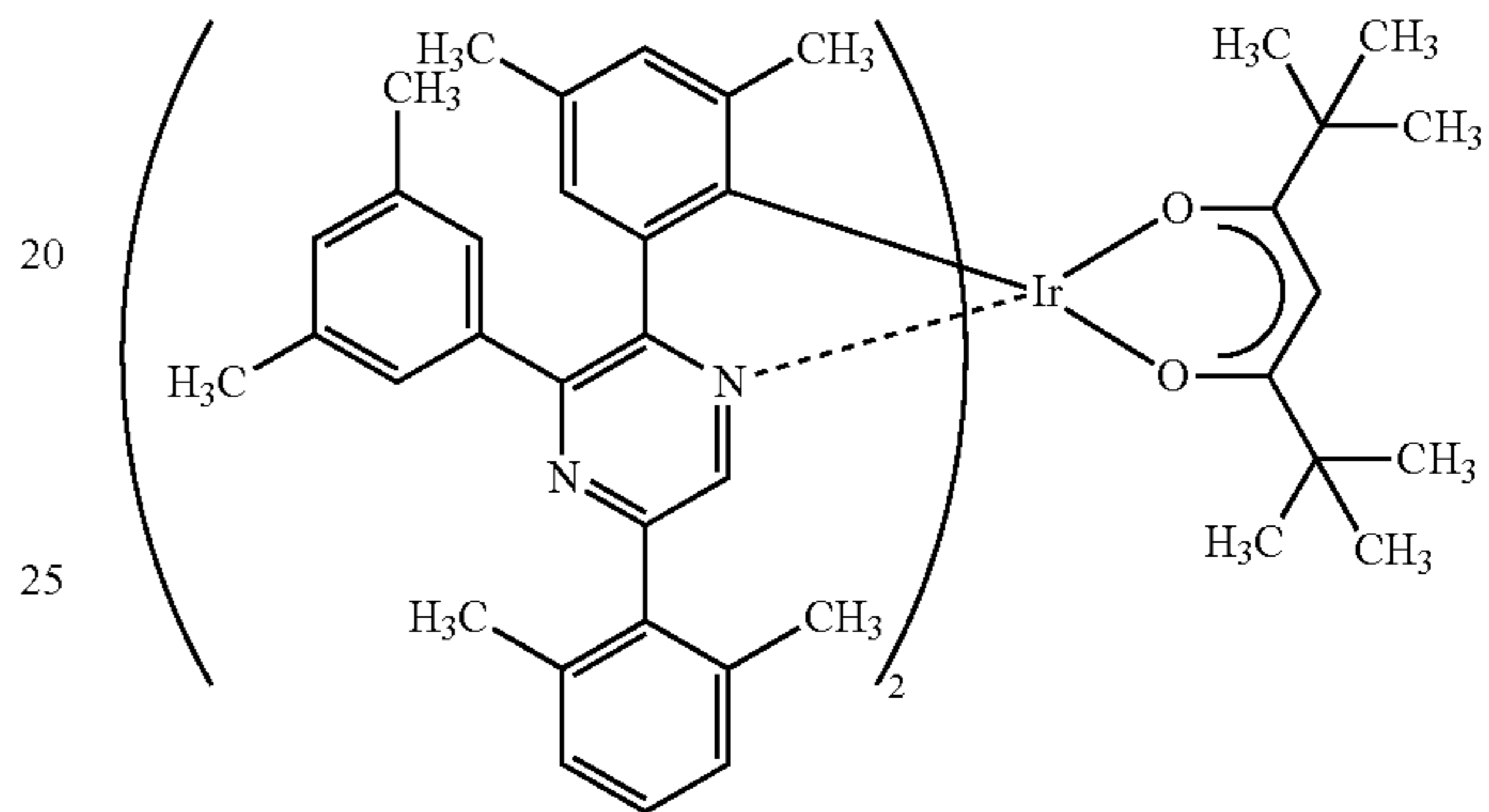
[Ir(dmdppr-dmp) 2 (dpm)]
