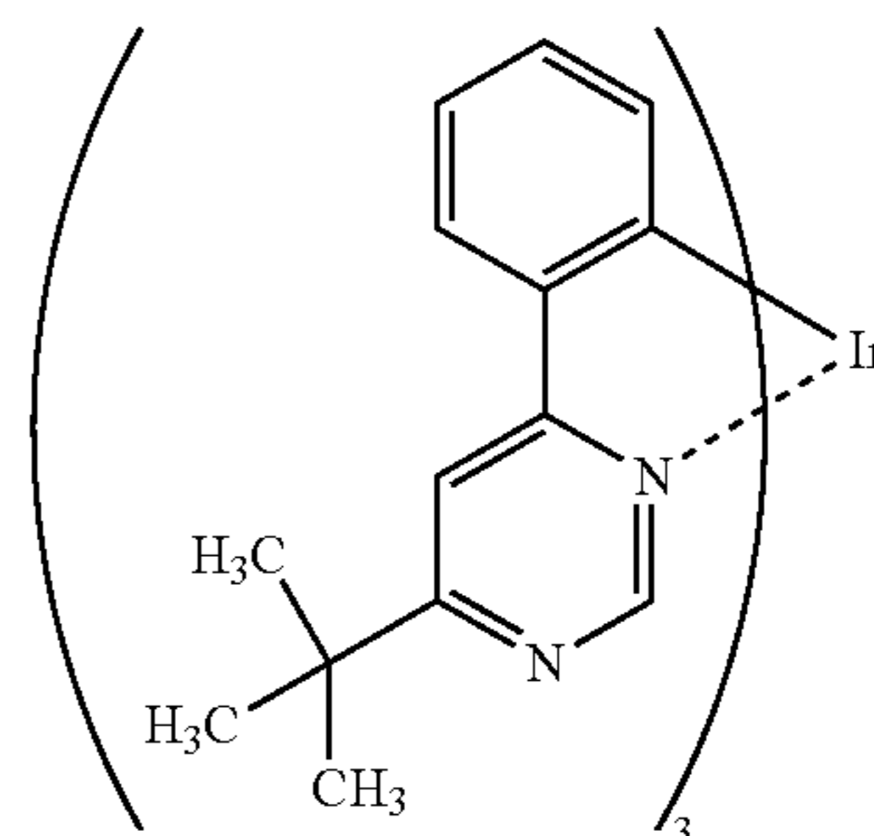
[Ir(tBuppm) 3 ]
