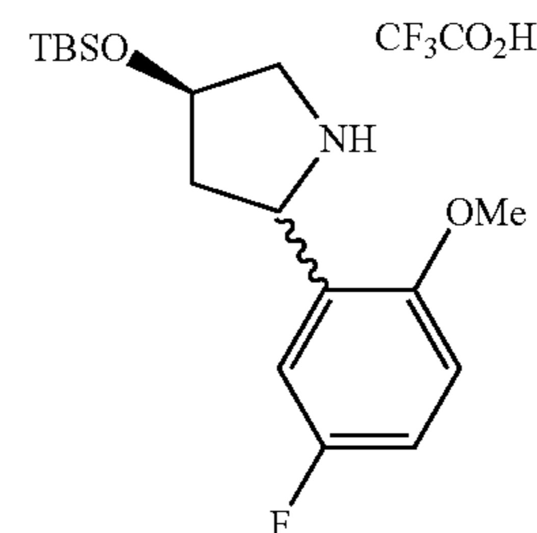
(R)-4-((tert-butyldimethylsilyloxy)-2-(5-fluoro-2-methoxyphenyl)pyrrolidine 2,2,2-trifluoroacetate
