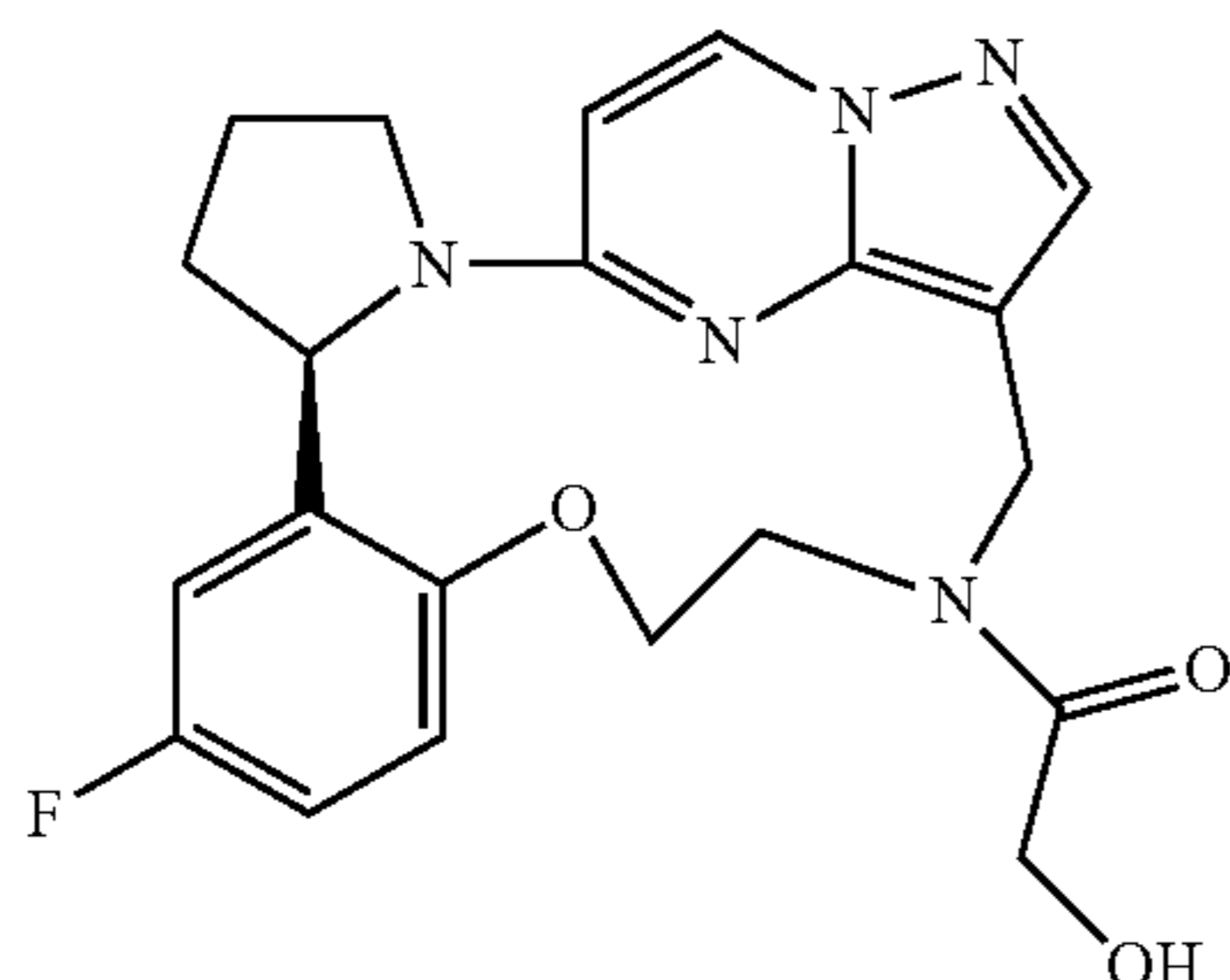
1-[(6R)-9-fluoro-13-oxa-2,16,20,21,24-pentaazapentacyclo[16.5.2.0 2,6 .0 7,12 .0 21,25 ]pentacos-1(24),7,9,11,18(25),19,22-heptaen-16-yl]-2-hydroxyethan-1-one
