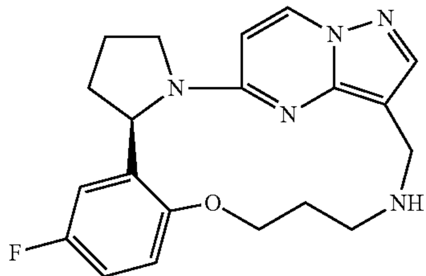
(6R)-9-fluoro-13-oxa-2,17,21,22,25-pentaazapentacyclo[17.5.2.0 2,6 .0 7,12 .0 22,26 ]hexacos-1(25),7,9,11,19(26),20,23-heptaene
