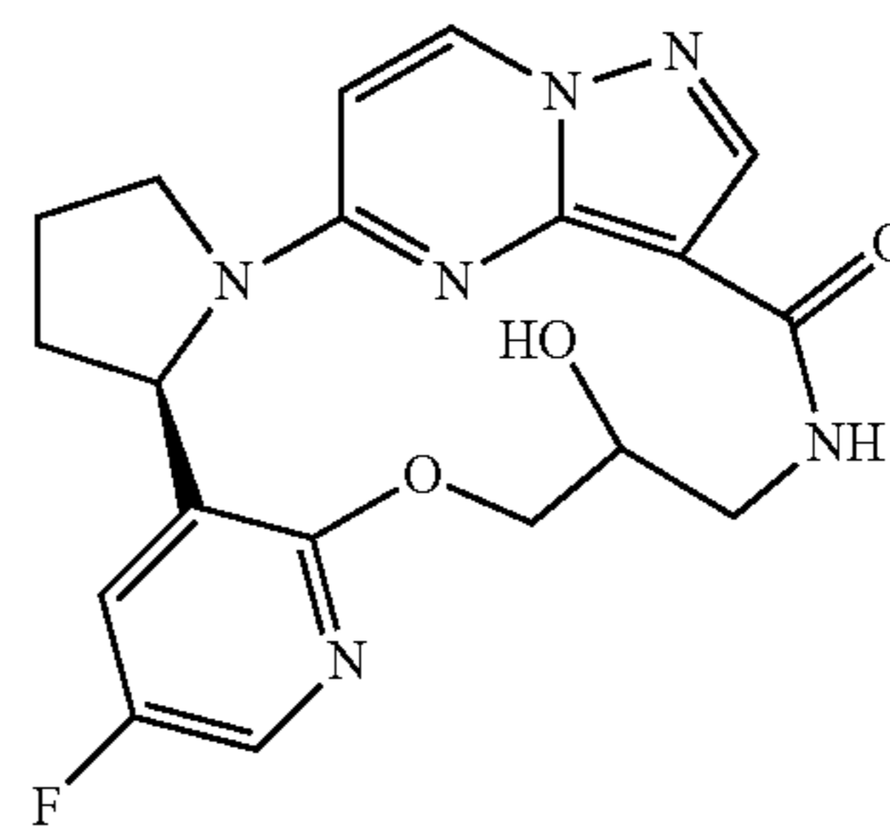
(6R)-9-fluoro-15-hydroxy-13-oxa-2,11,17,21,22,25-hexaazapentacyclo[17.5.2.0 2,6 .0 7,12 .0 22,26 ]hexacos-1(25),7,9,11,19(26),20,23-heptaen-18-one
