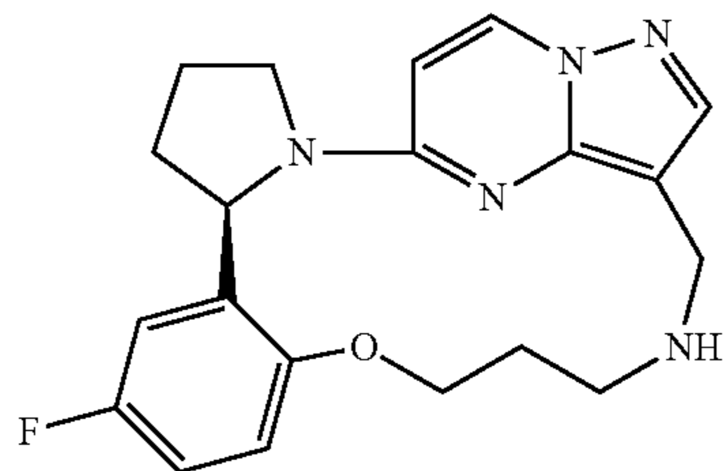
(6R)-9-fluoro-13-oxa-2,17,21,22,25-pentaazapentacyclo[17.5.2.0 2,6 .0 7,12 .0 22,26 ]hexacos-1(25),7,9,11,19(26),20,23-heptaene
