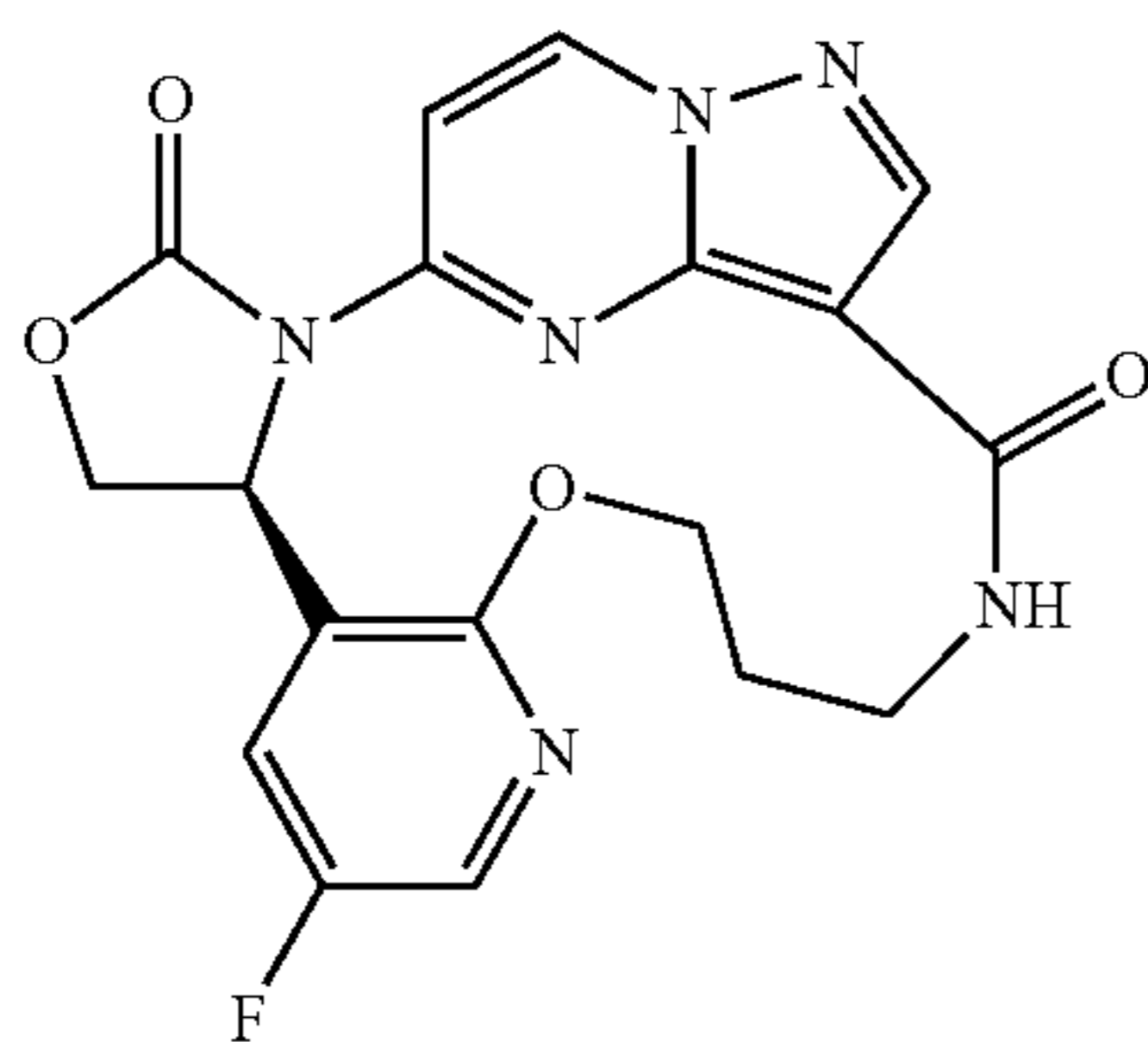
(6S)-9-fluoro-4,13-dioxo-2,11,17,21,22,25-hexaazapentacyclo[17.5.2.0 2,6 .0 7,12 .0 22,26 ]hexacos-1(25),7(12),8,10,19(26),20,23-heptaene-3,18-dione
