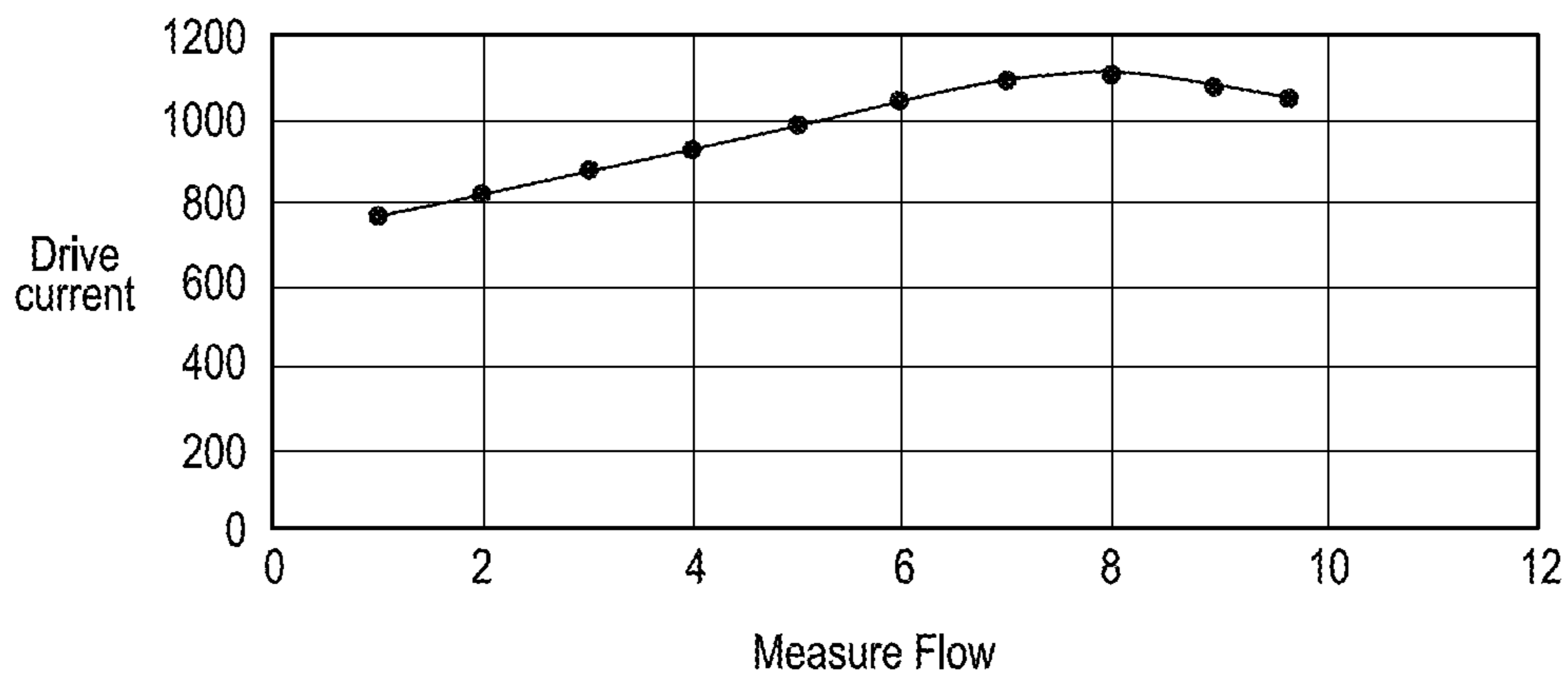
Driving Current
