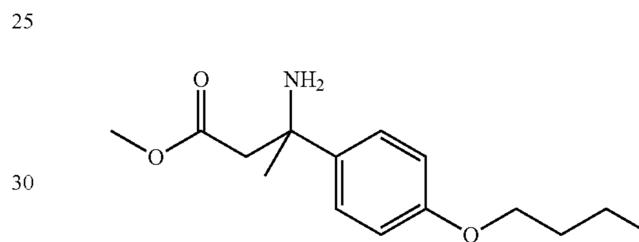
Intermediate 107C. Methyl 3-amino-3-(4-butoxyphenyl)butanoate
