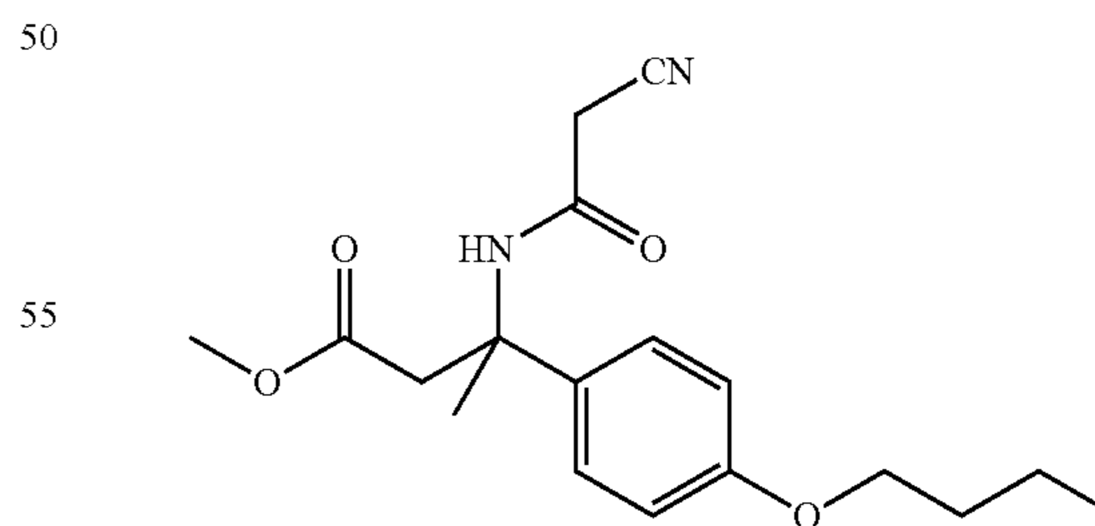
Intermediate 107B. Methyl 3-(4-butoxyphenyl)-3-(1,1-dimethylethylsulfonamido)butanoate
