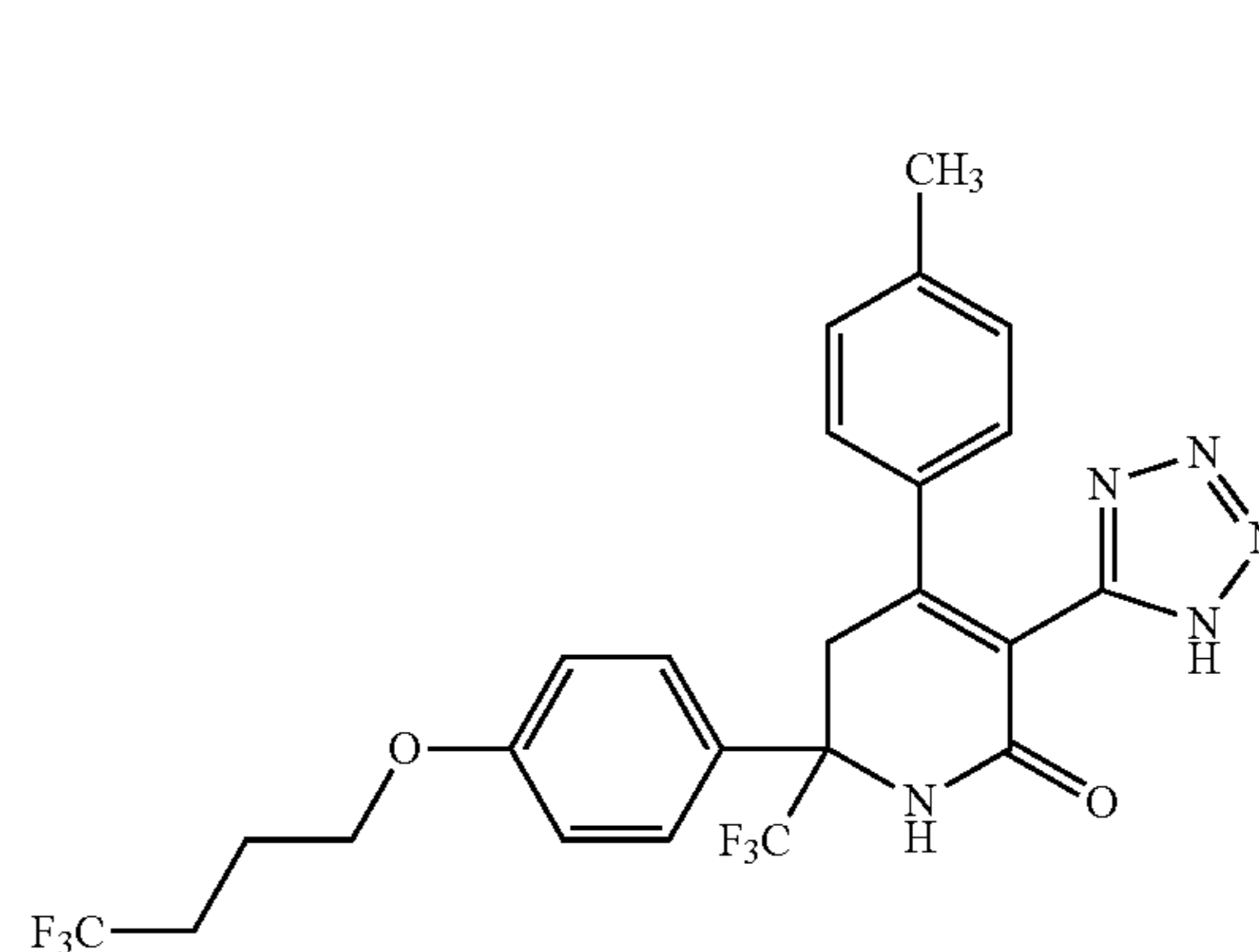
Intermediate 2A. 4-(4,4,4-Trifluorobutoxy)benzaldehyde
