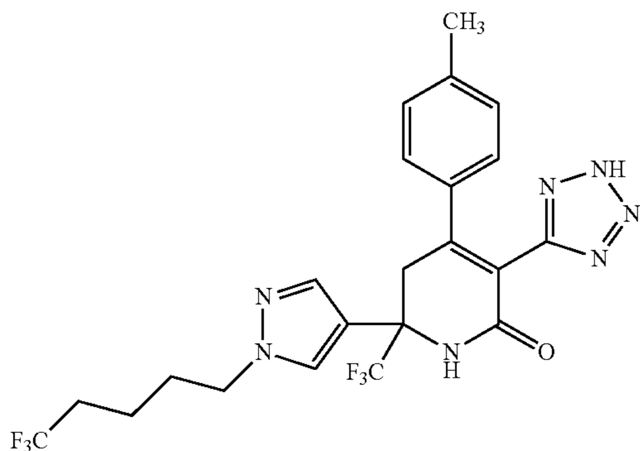
Intermediate 12A. 4-Iodo-1-(5,5,5-trifluoropentyl)-1H-pyrazole
