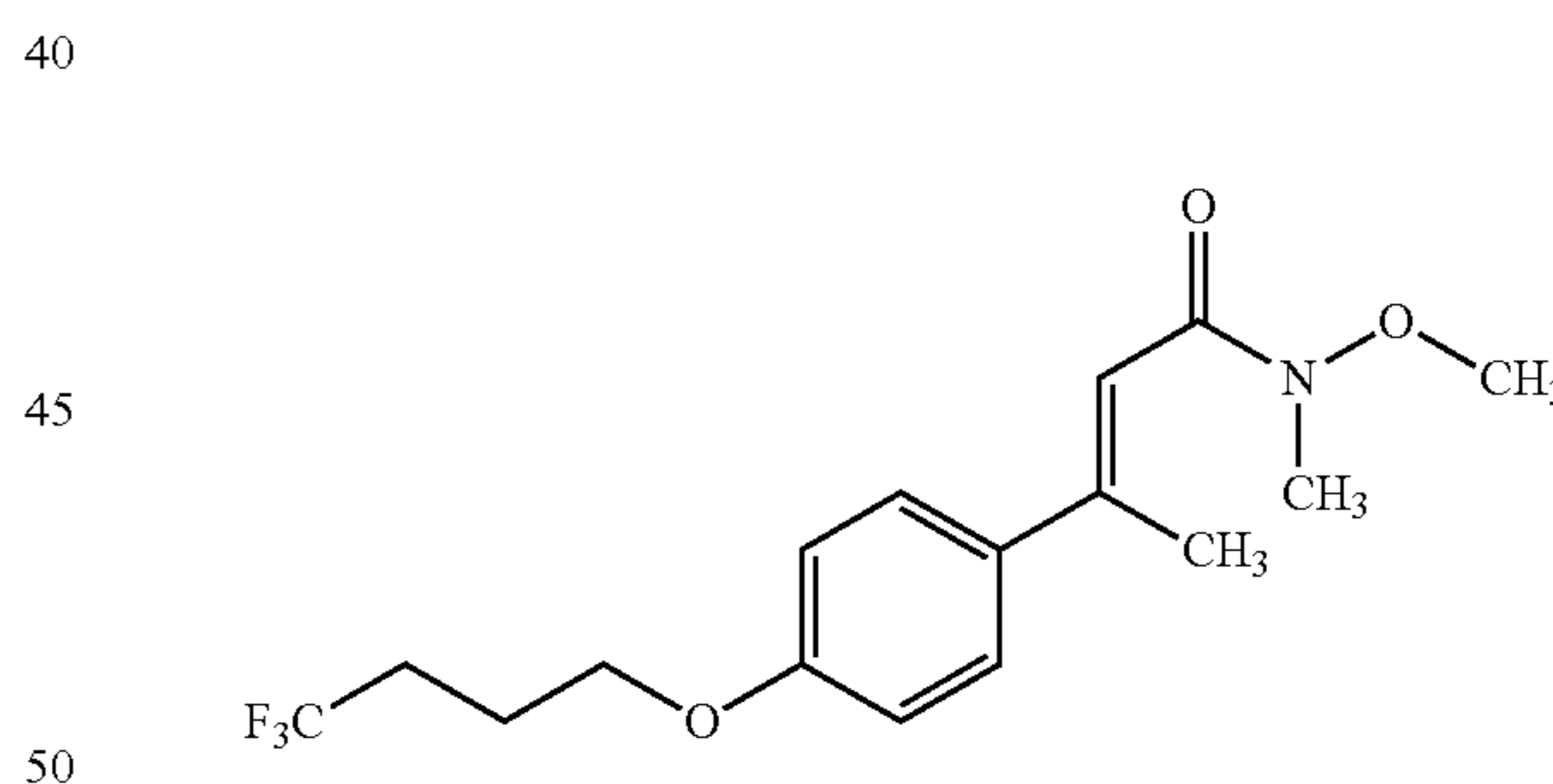
Intermediate 11C. (E)-N-Methoxy-N-methyl-3-(4-(4,4,4-trifluorobutoxy)phenyl)but-2-enamide
