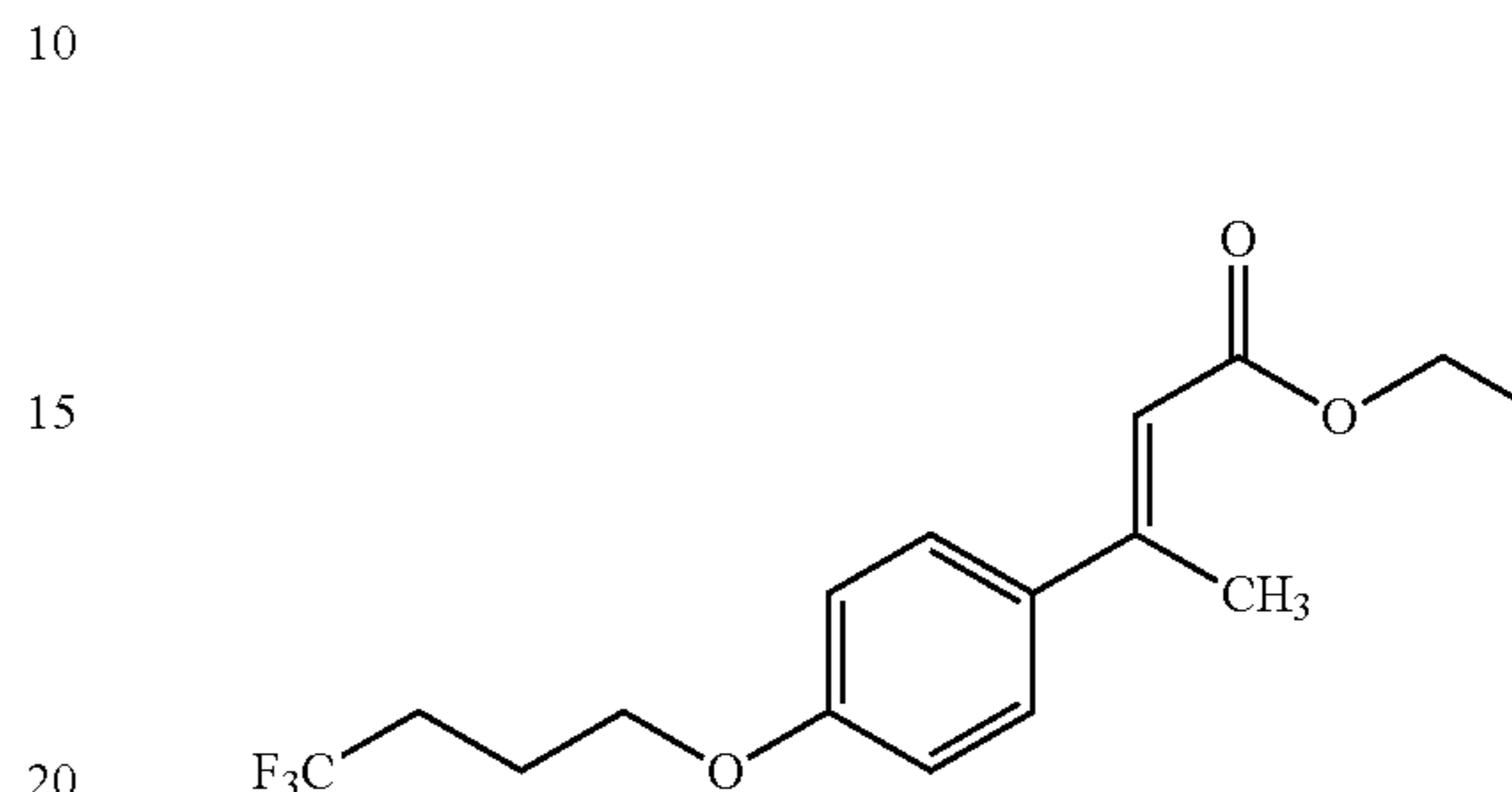
Intermediate 11B. (E)-Ethyl 3-(4-(4,4,4-trifluorobutoxy)phenyl)but-2-enoate
