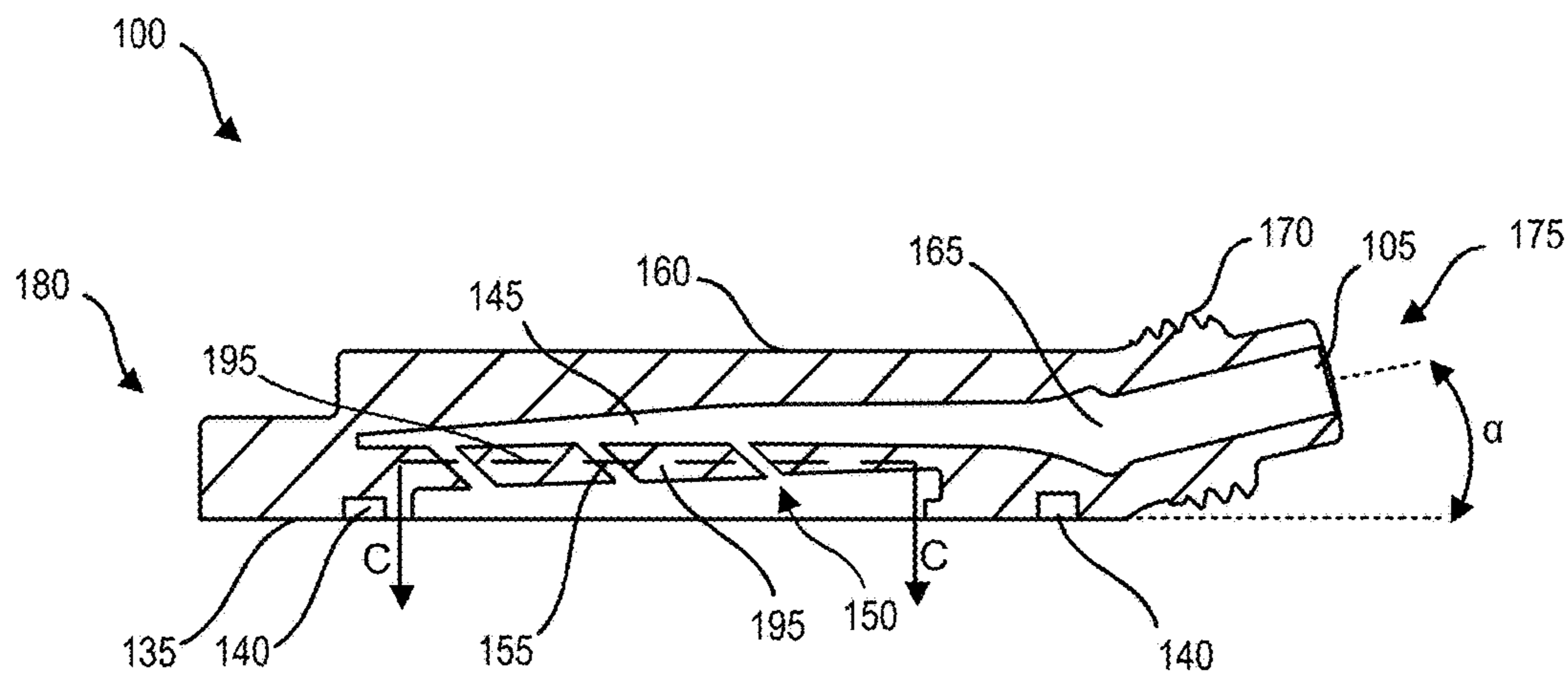
SECTION B-B
