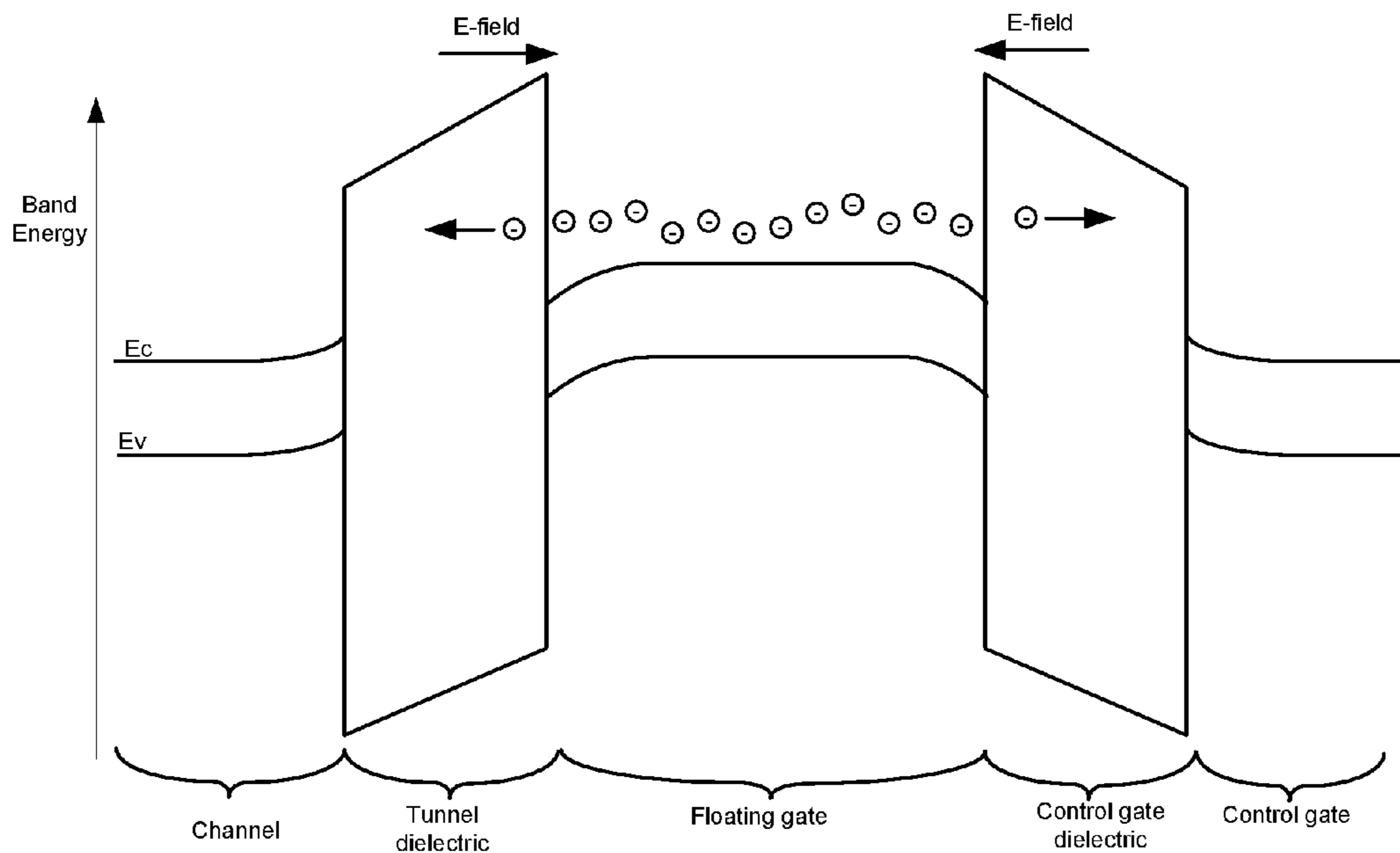
Fig. 5A (Conventional)
