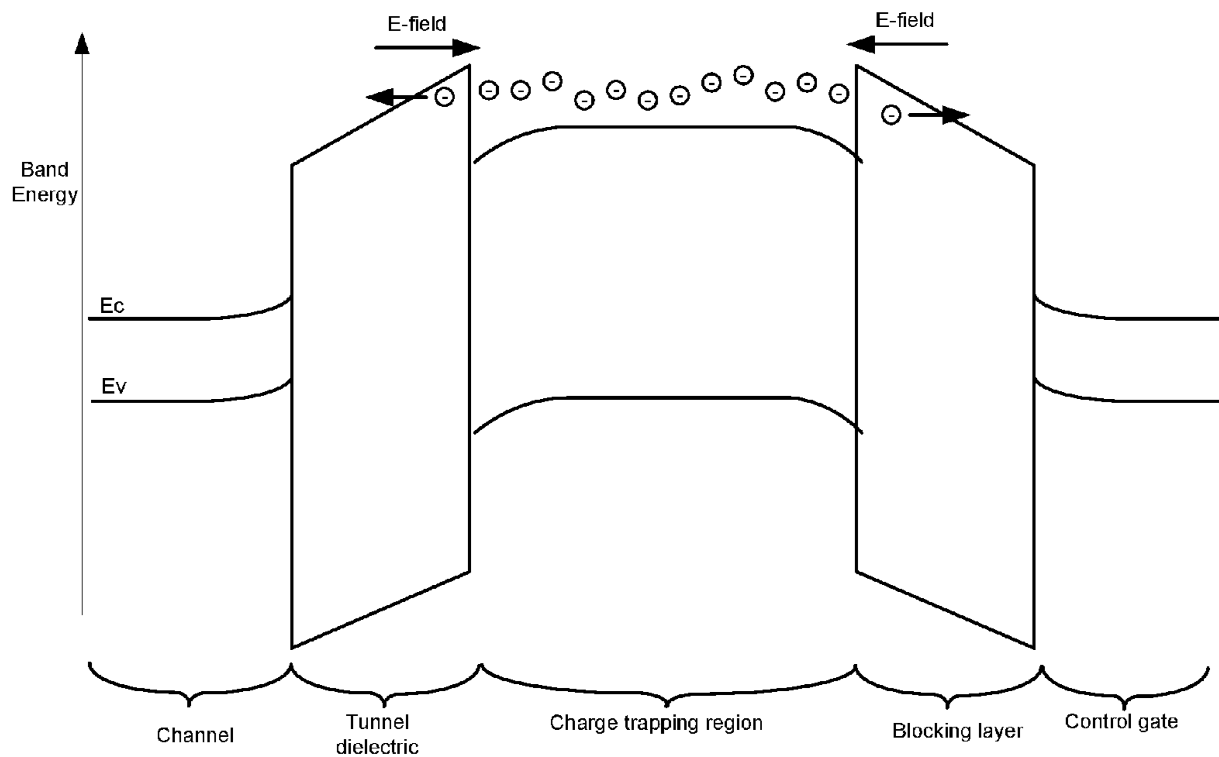
Fig. 5B (Conventional)
