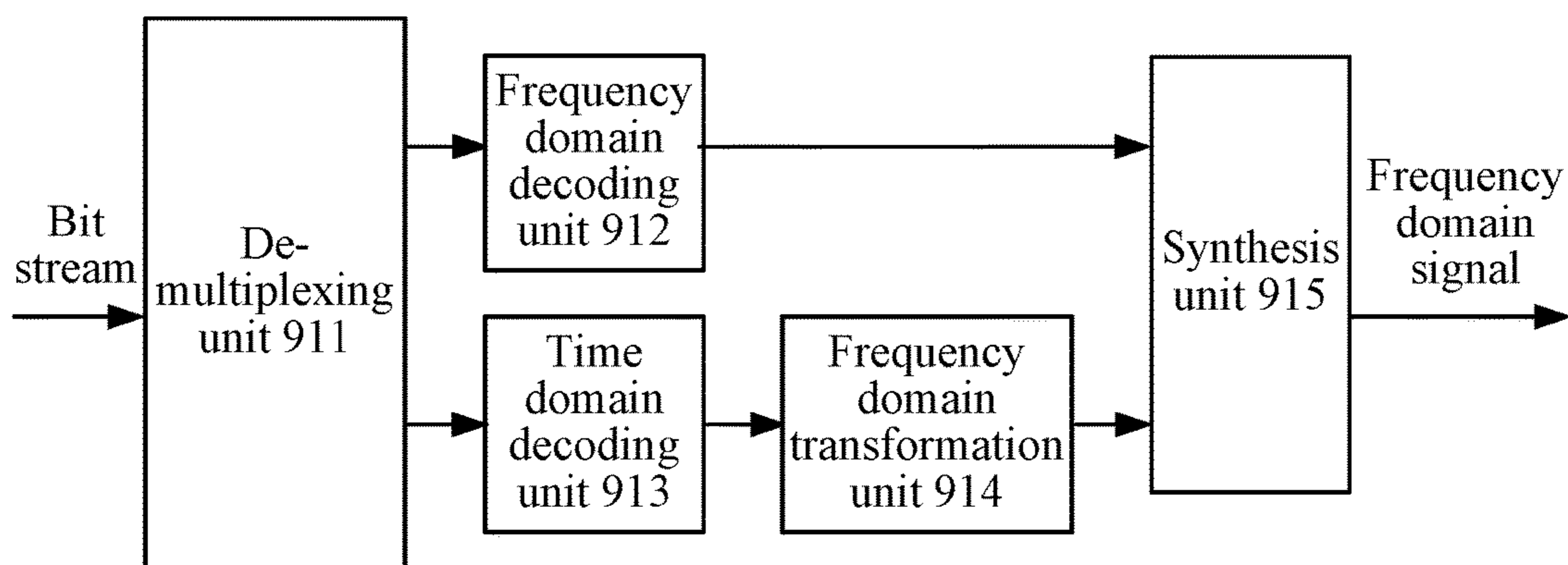
Decoding unit 910
