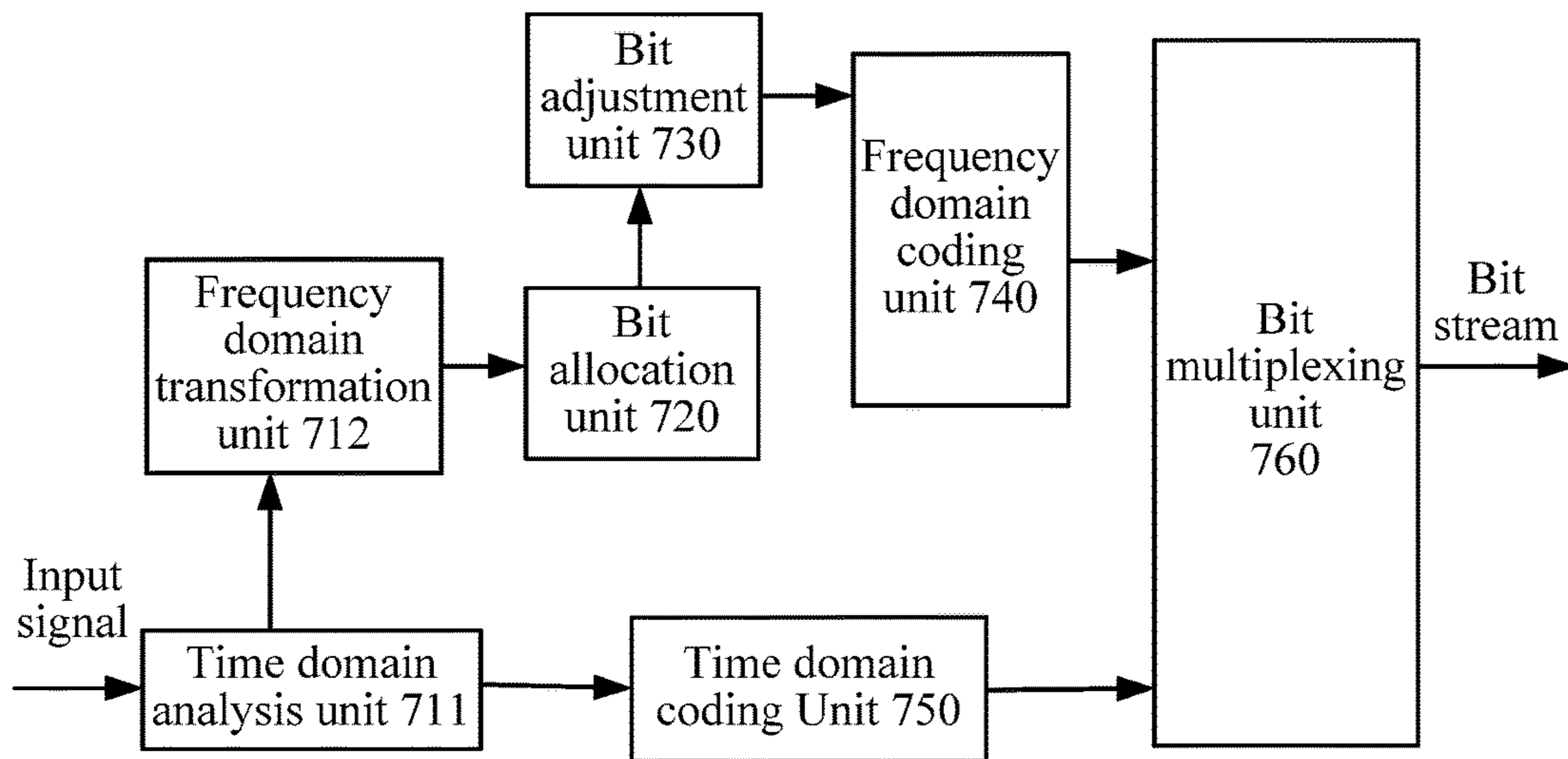
Device 700
