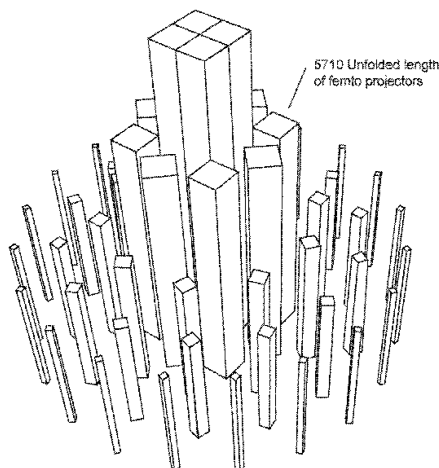
5700 Perspective view of exit pupil envelope femto projectors
