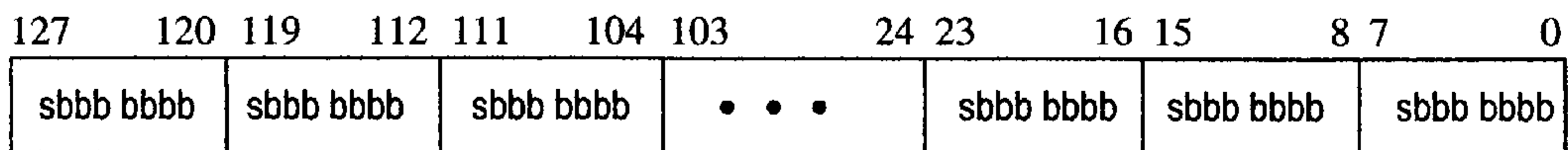
345 SIGNED PACKED BYTE REPRESENTATION
