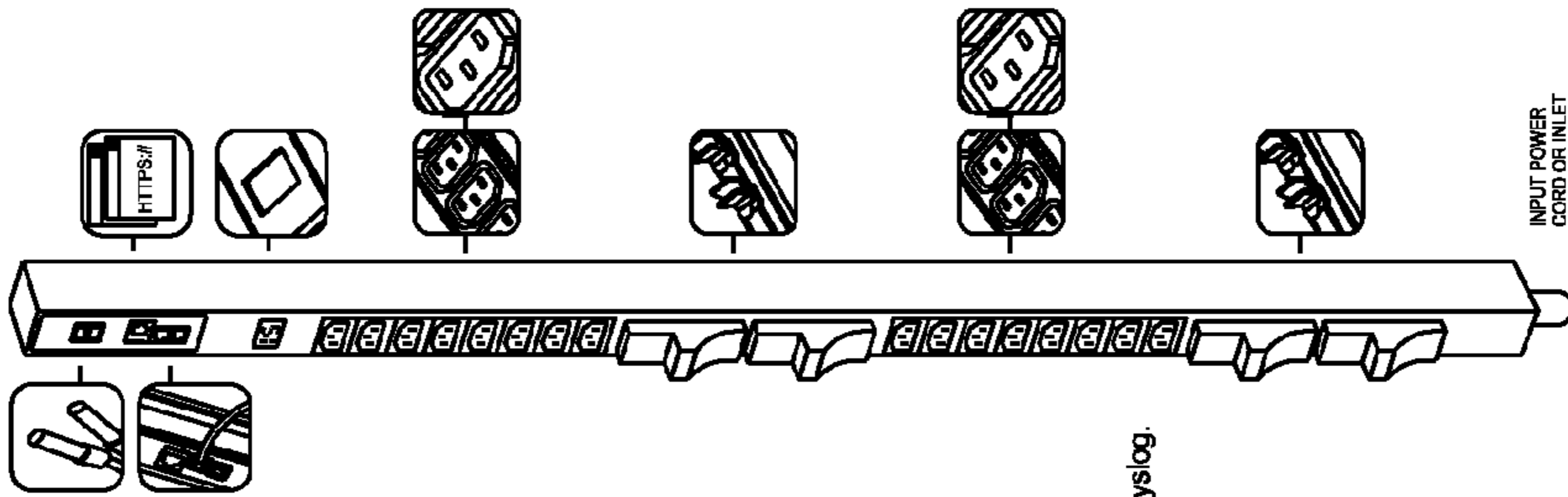
Diagram 2 Switched CDU Anatomy
