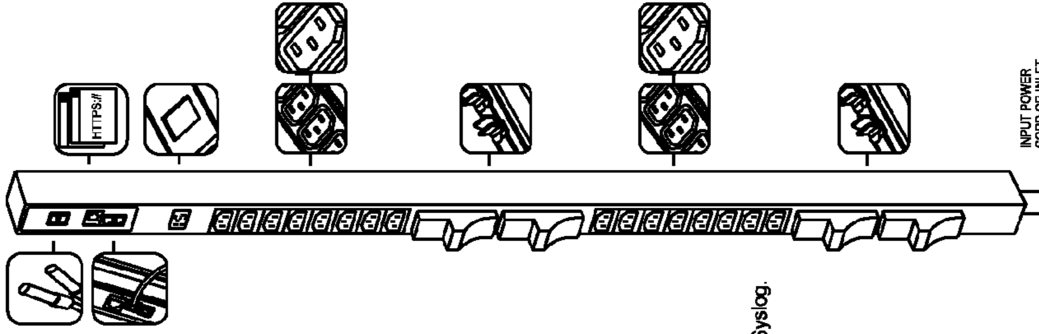
Diagram 2 Switched CDU Anatomy
