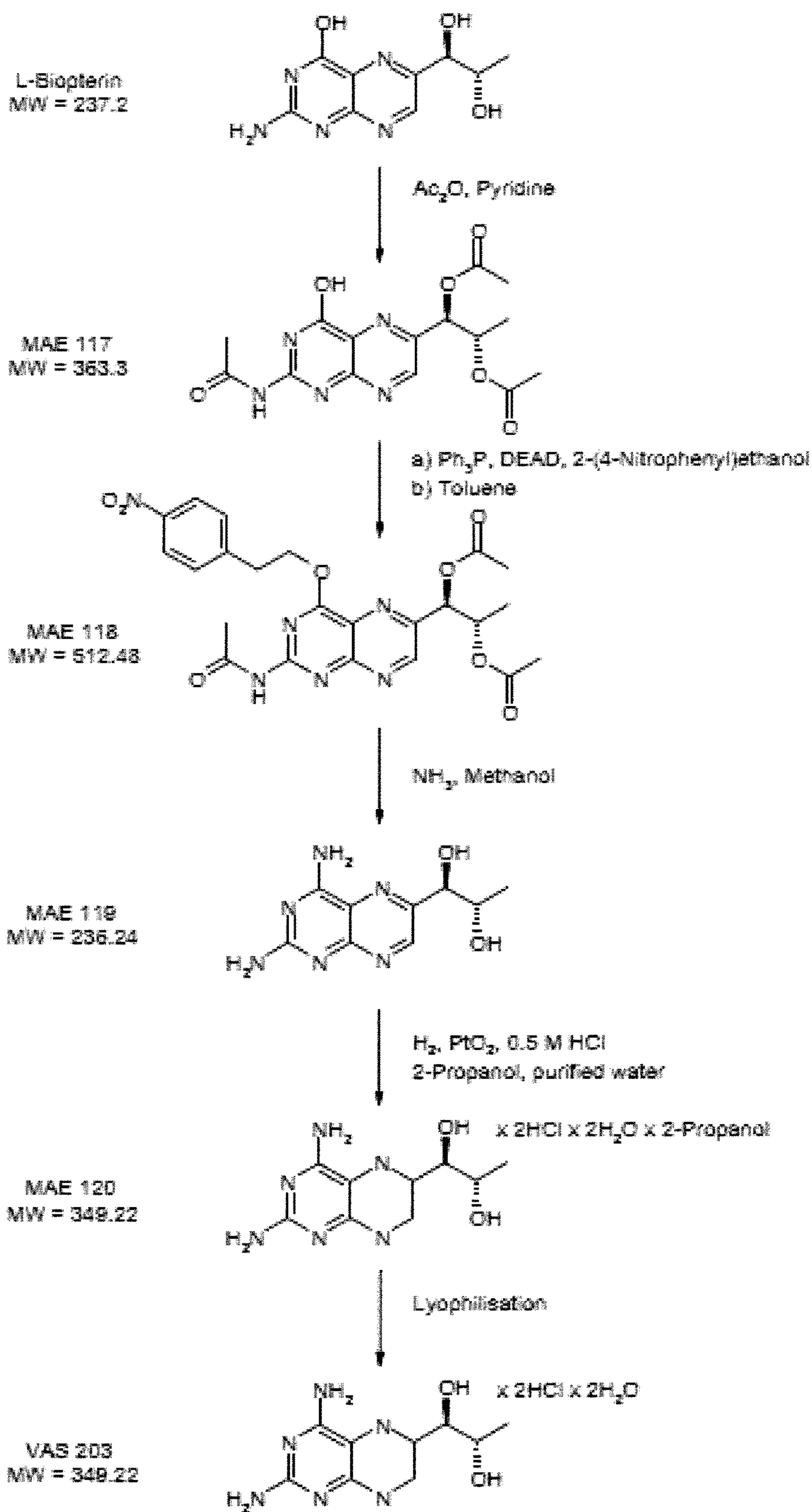
Figure 1: Preparation of VAS203 drug substance
