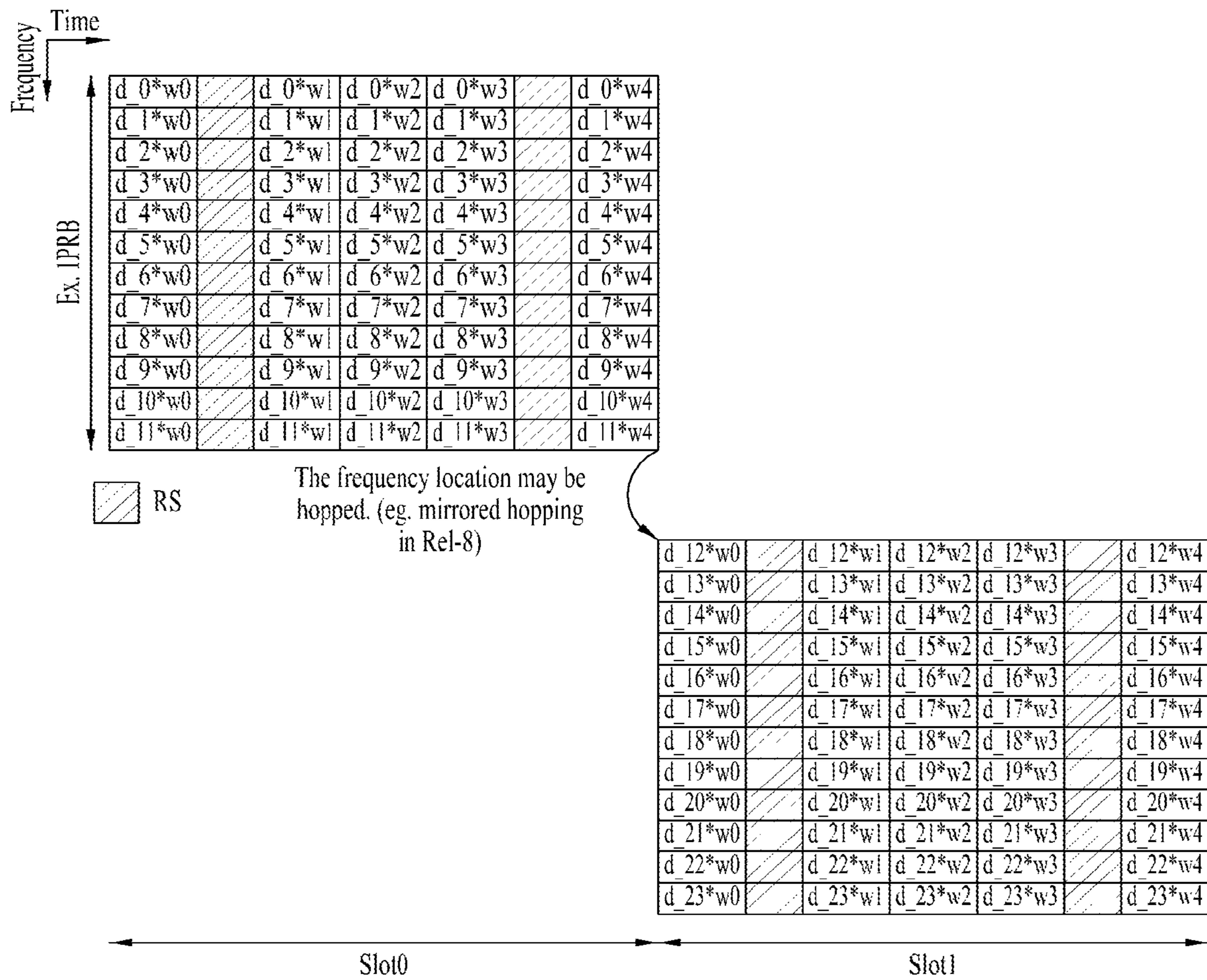
Reuse of LTE PUCCH format 2 structure (normal CP case)
