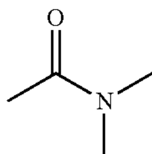
N,N-Dimethylacetamide
