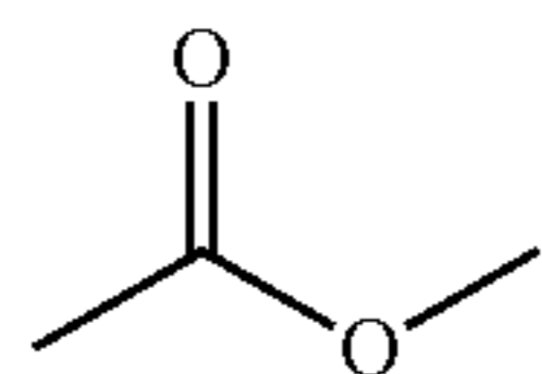
Methyl acetate
