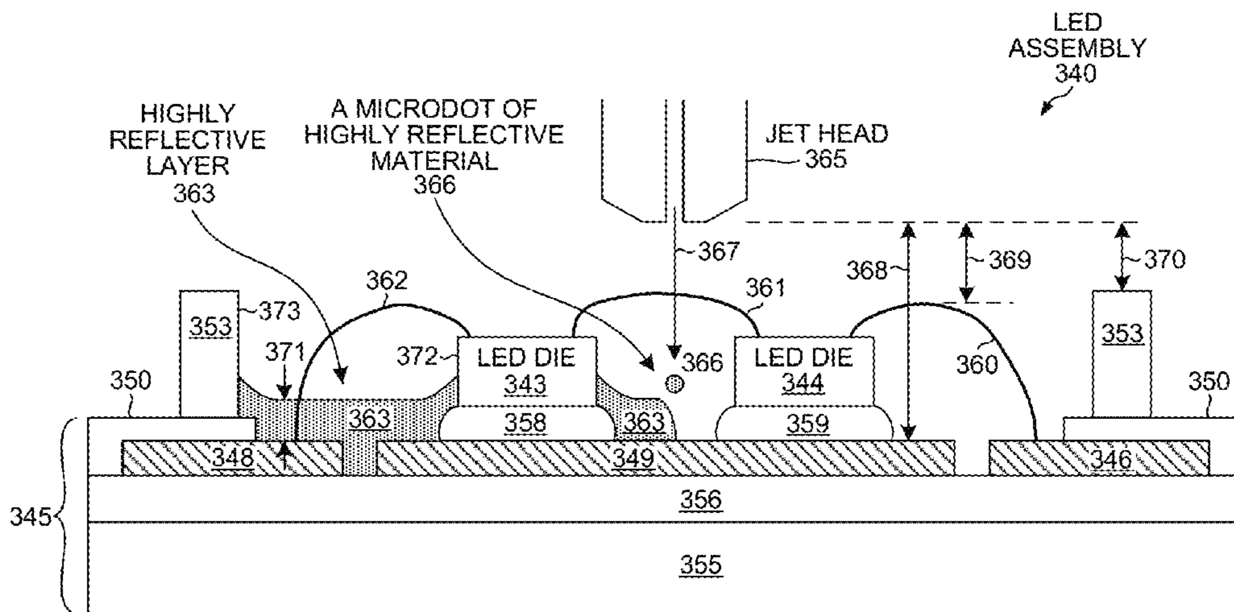
JETTING MICRODOTS OF HR MATERIAL FIG. 56
