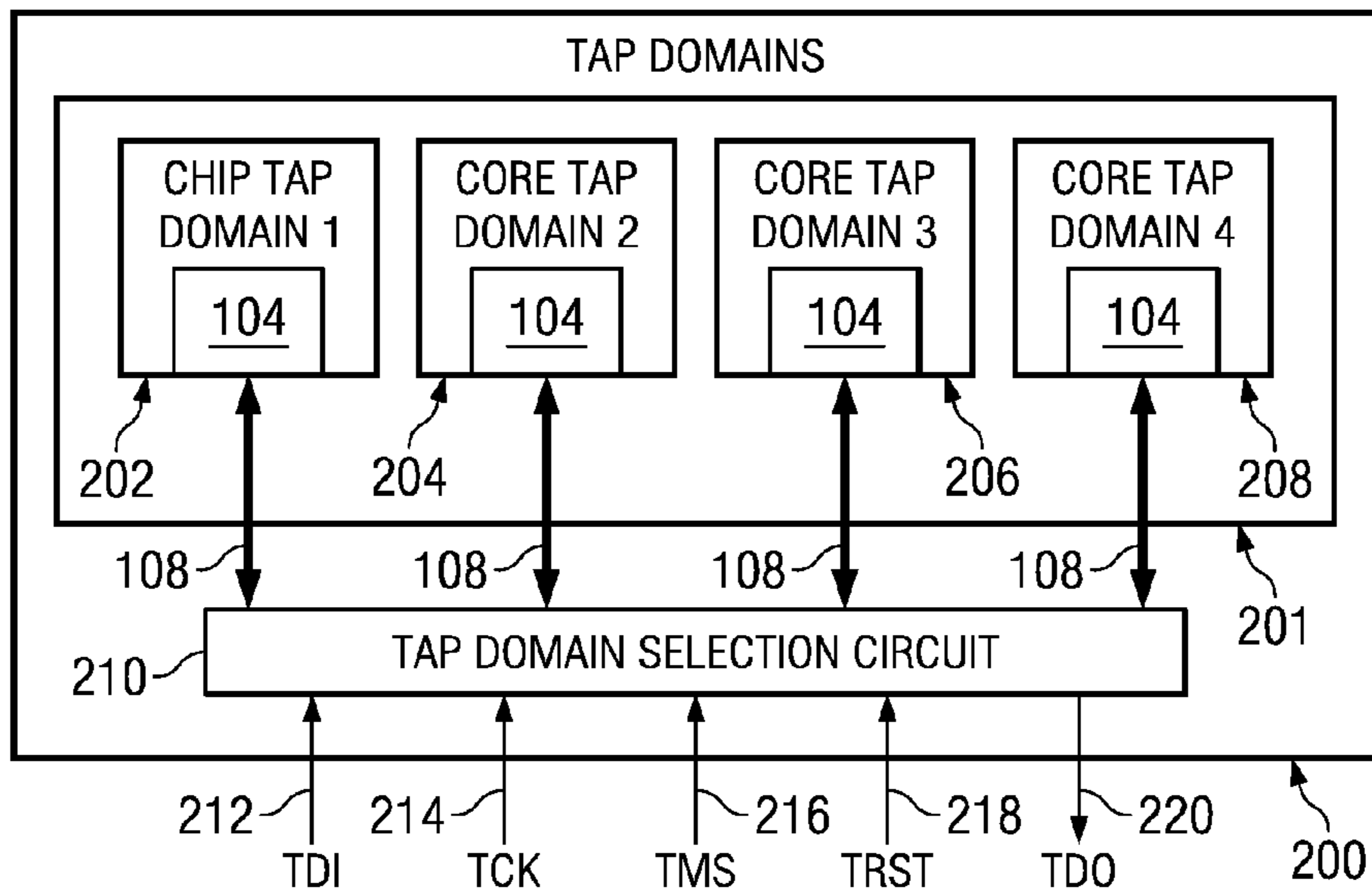
FIG. 2 (PRIOR ART)
