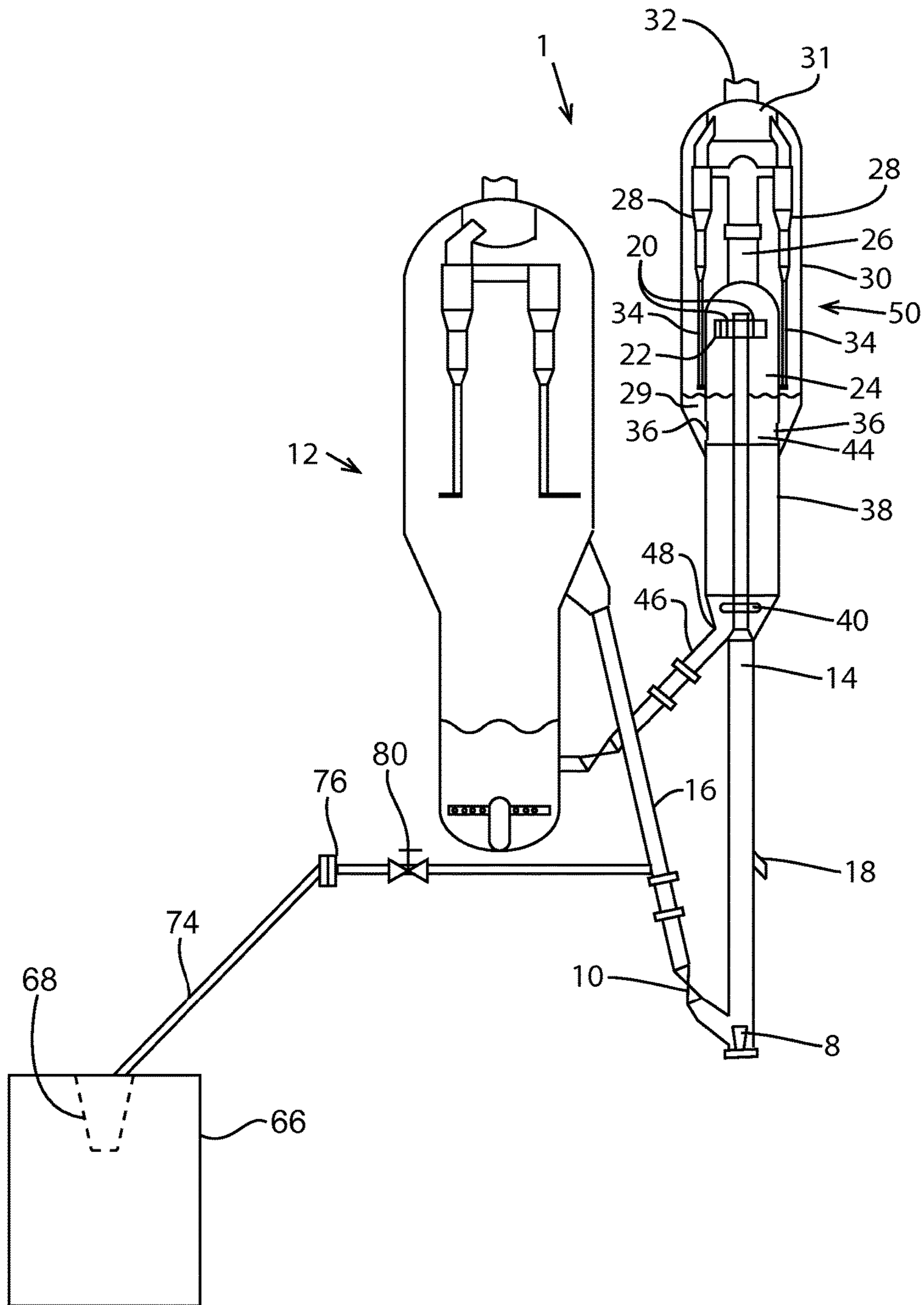
FIG 2 PRIOR ART
